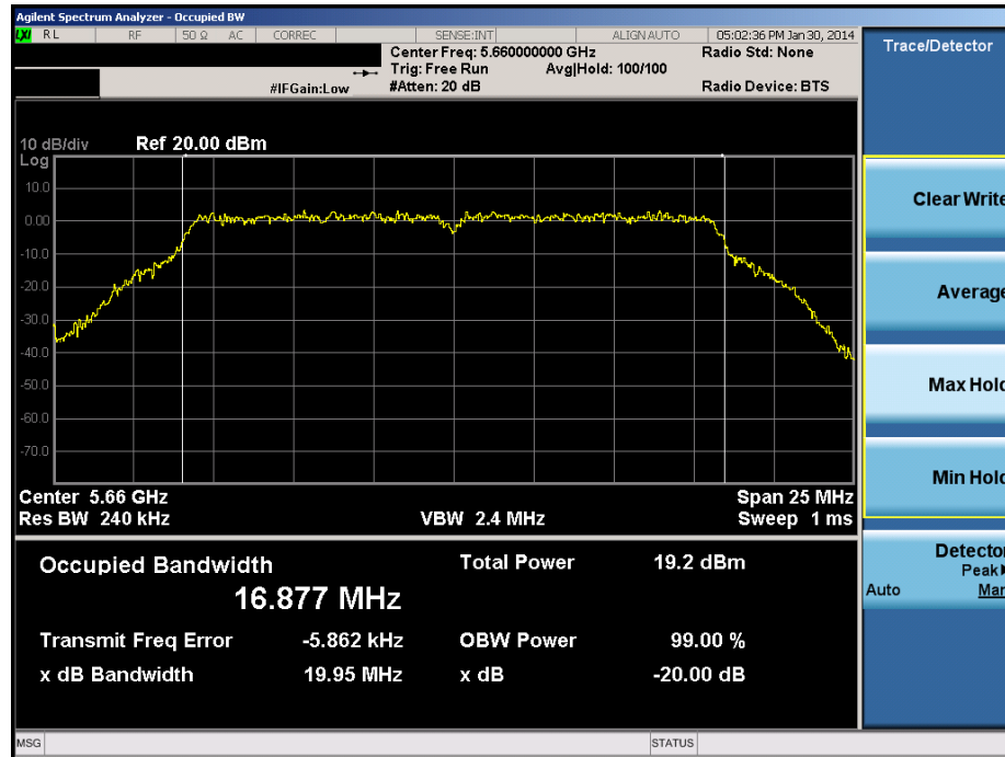
Plot 6-65. 20dB Bandwidth Plot (20MHz BW 802.11a (UNII Band 2C) – Ch. 132)
