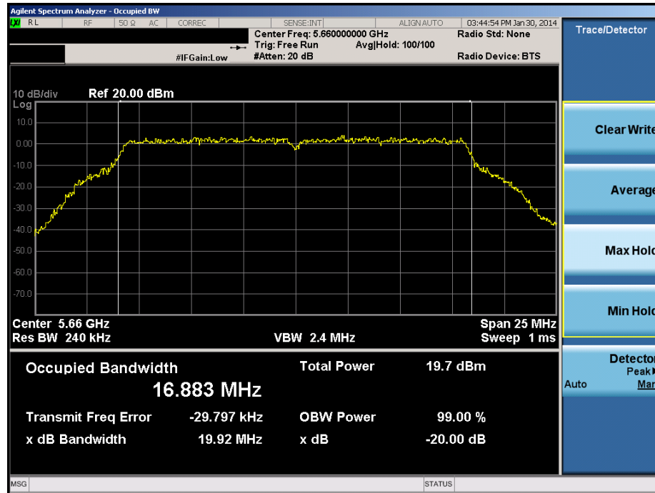
Plot 6-31. 20dB Bandwidth Plot (20MHz BW 802.11a (UNII Band 2C) – Ch. 132)
