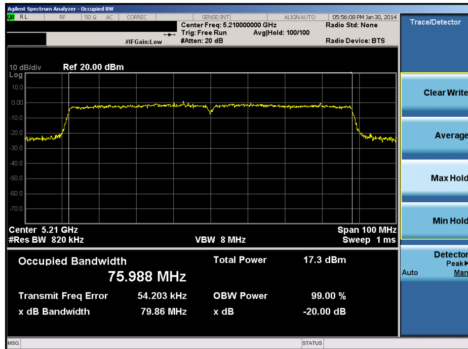
Plot 6-34. 20dB Bandwidth Plot (80MHz BW 802.11a (UNII Band 1) – Ch. 42)
