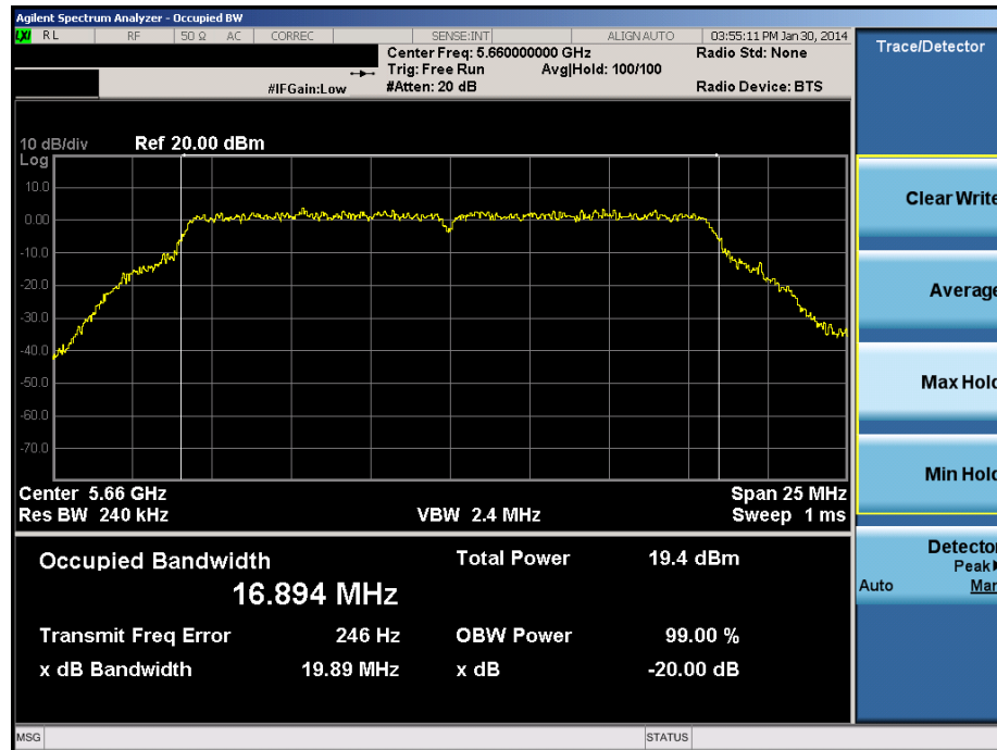
Plot 6-32. 20dB Bandwidth Plot (20MHz BW 802.11n (UNII Band 2C) – Ch. 132)
