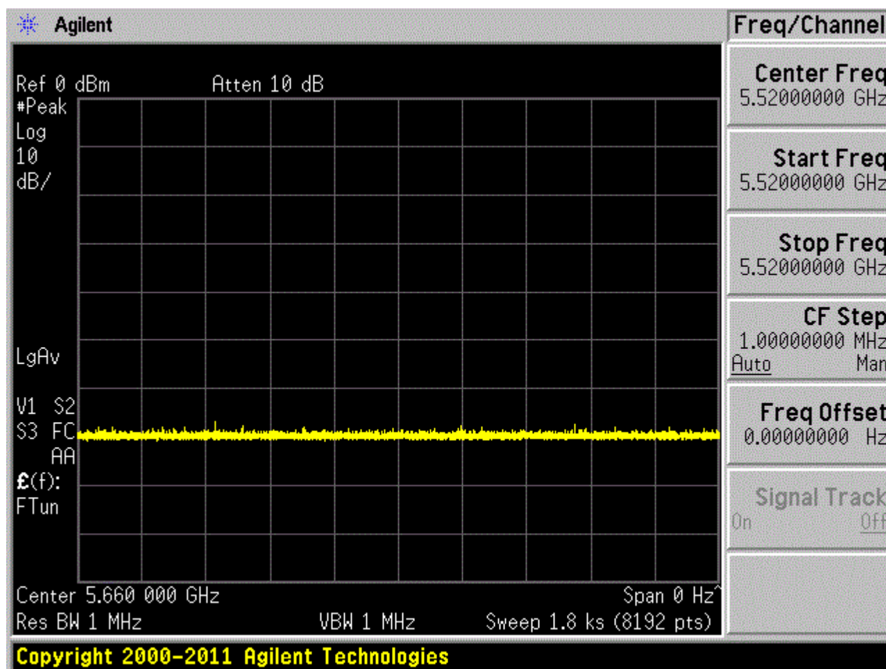
Figure 6-6. Non-Occupancy Period Plot
