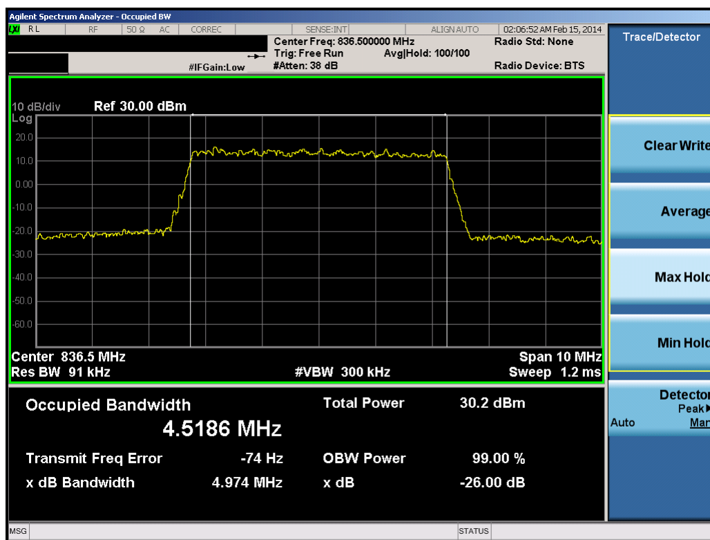
Plot 8-11. Occupied Bandwidth Plot (5.0MHz 16-QAM – RB Size 25)
