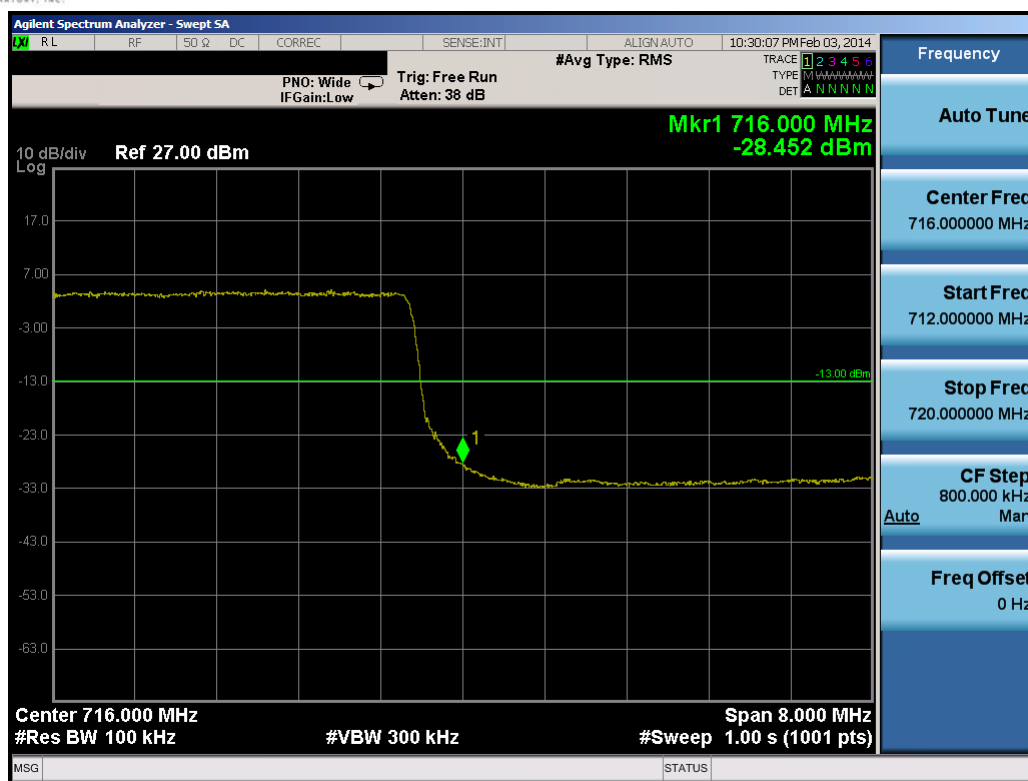
Plot 7-14. Upper Band Edge Plot (10.0MHz QPSK – RB Size 50)
