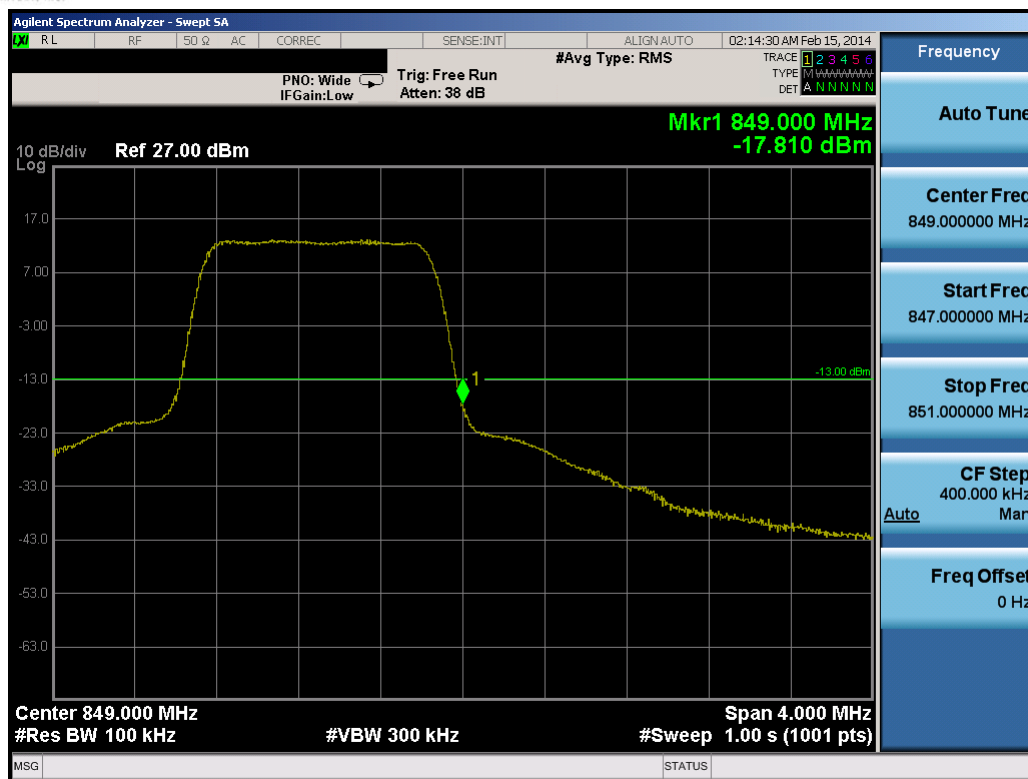
Plot 8-4. Upper Band Edge Plot (1.4MHz QPSK – RB Size 6)
