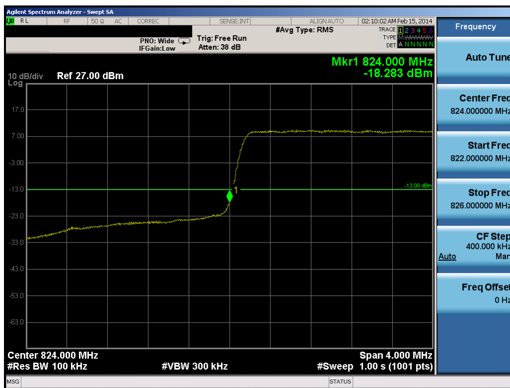
Plot 8-5. Lower Band Edge Plot (3.0MHz QPSK – RB Size 15)
