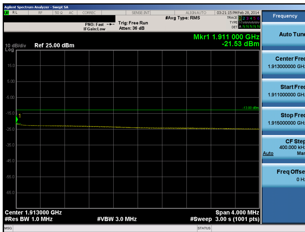
Plot 10-20. Extended Upper Band Edge Plot (10.0MHz QPSK – RB Size 50)
