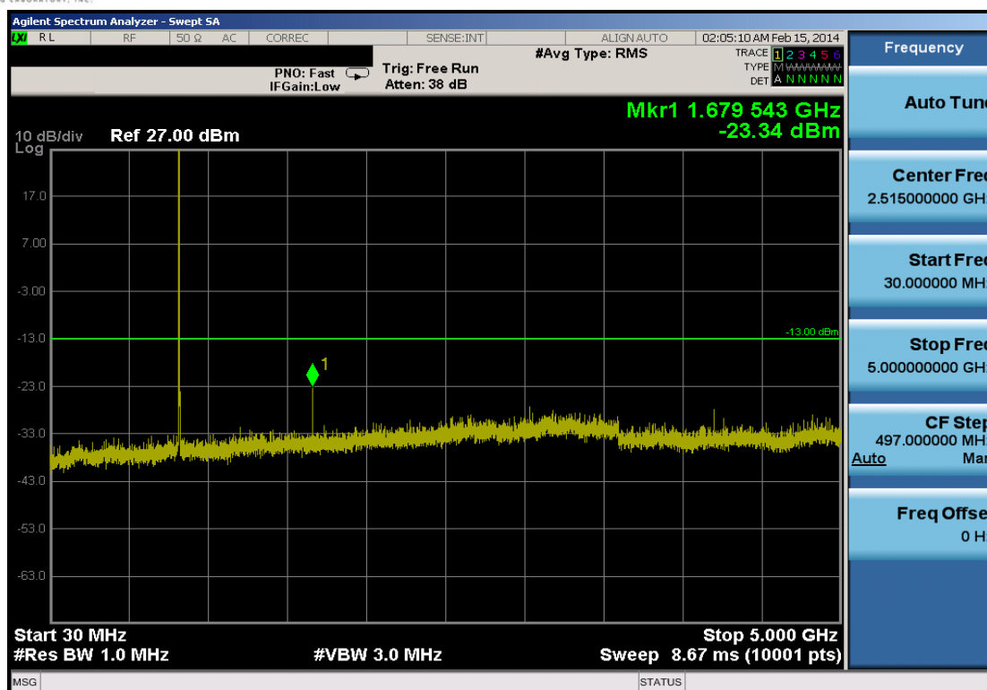
Plot 8-16. Conducted Spurious Plot (5.0MHz QPSK – RB Size 1, RB Offset 0 – High Channel)
