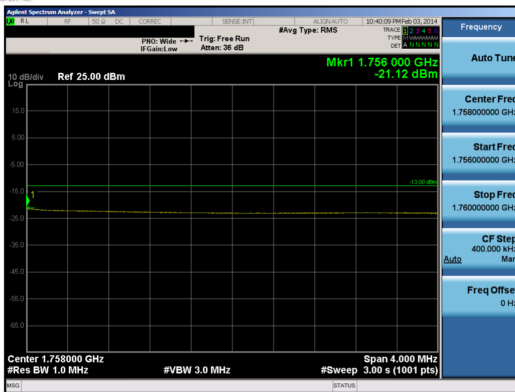
Plot 9-20. Upper Extended Band Edge Plot (10.0MHz QPSK – RB Size 50)
