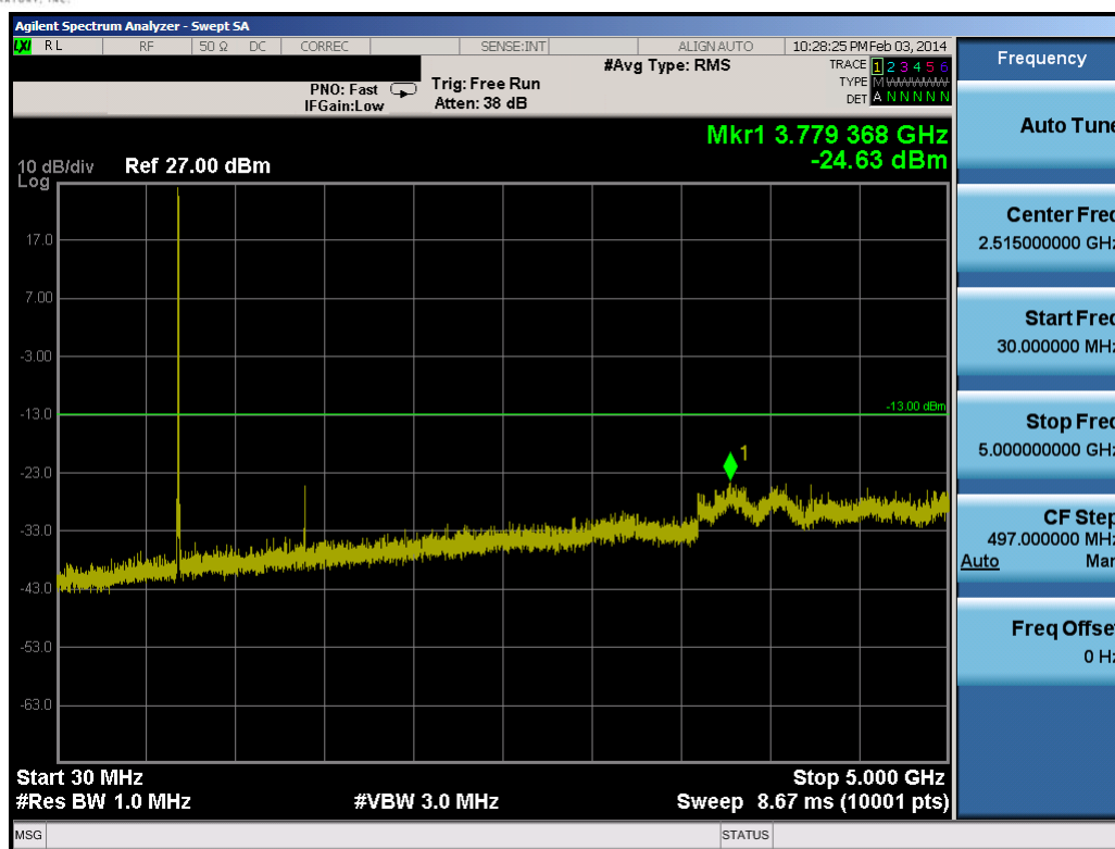
Plot 7-8. Conducted Spurious Plot (10.0MHz QPSK – RB Size 1, RB Offset 0– Low Channel)
