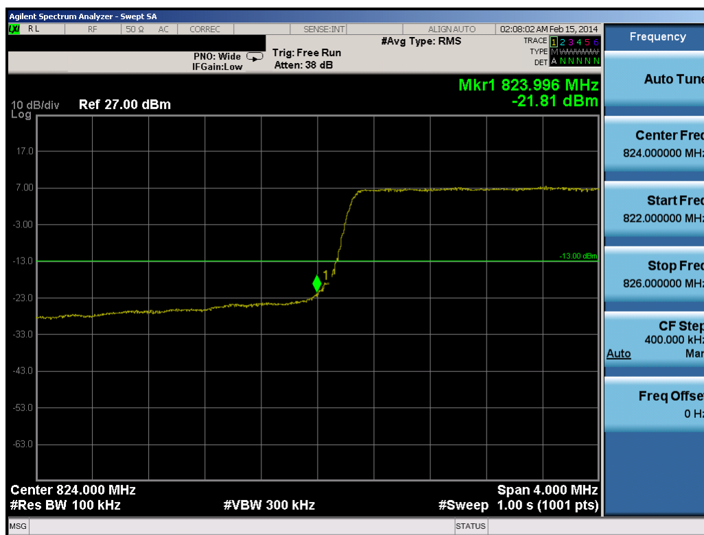
Plot 8-9. Lower Band Edge Plot (5.0MHz QPSK - RB Size 25)
