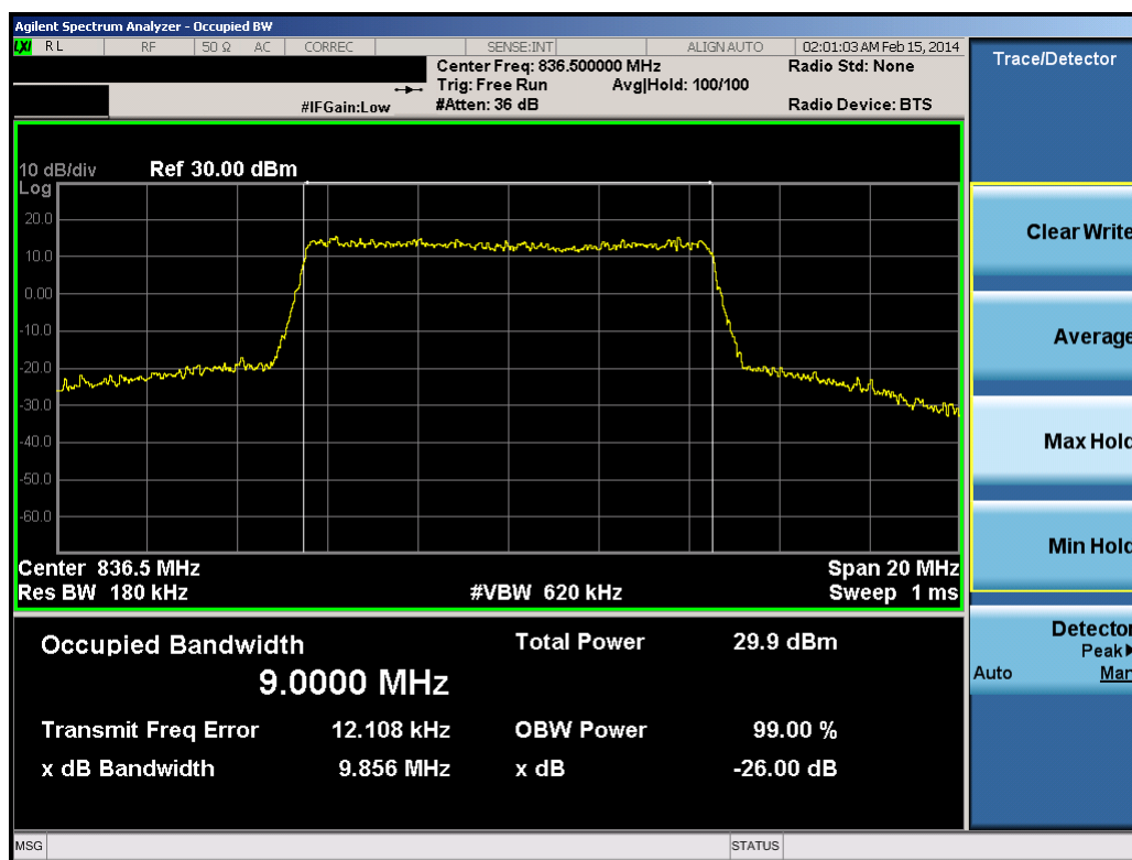
Plot 8-21. Occupied Bandwidth Plot (10.0MHz 16-QAM – RB Size 50)
