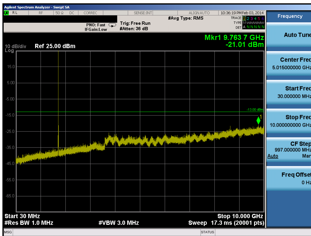
Plot 9-15. Conducted Spurious Plot (10.0MHz QPSK – RB Size 1, RB Offset 0 – Mid Channel)
