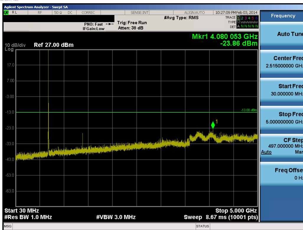
Plot 7-10. Conducted Spurious Plot (10.0MHz QPSK – RB Size 1, RB Offset 0 – Mid Channel)
