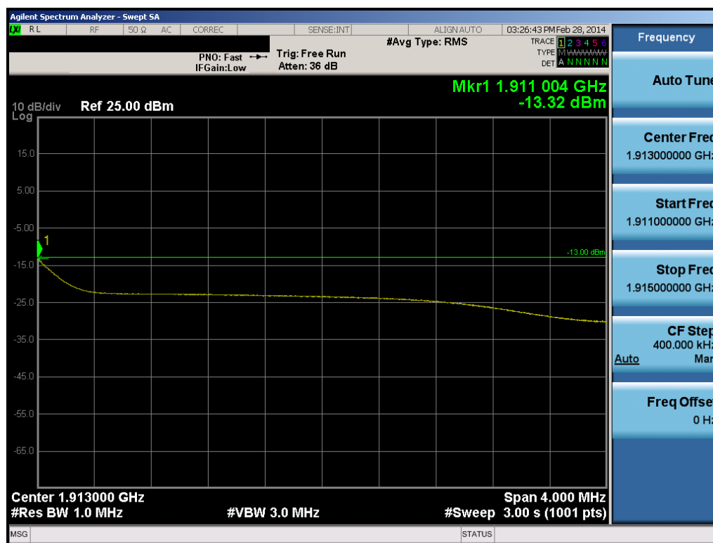
Plot 10-6. Extended Upper Band Edge Plot (5.0MHz QPSK – RB Size 25)
