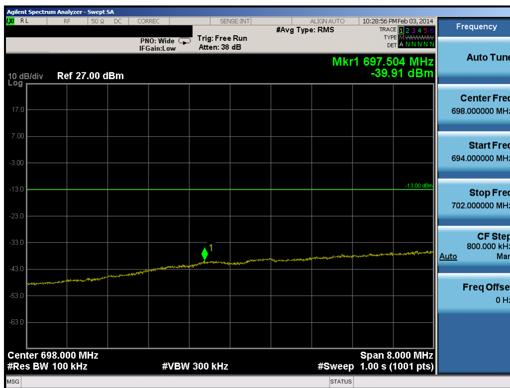
Plot 7-5. Lower Band Edge Plot (10.0MHz QPSK – RB Size 50)
