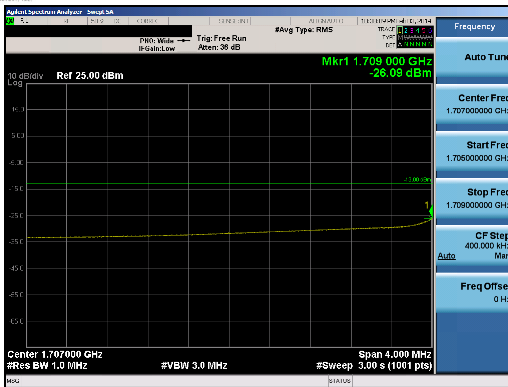
Plot 9-10. Lower Extended Band Edge Plot (10.0MHz QPSK – RB Size 50)
