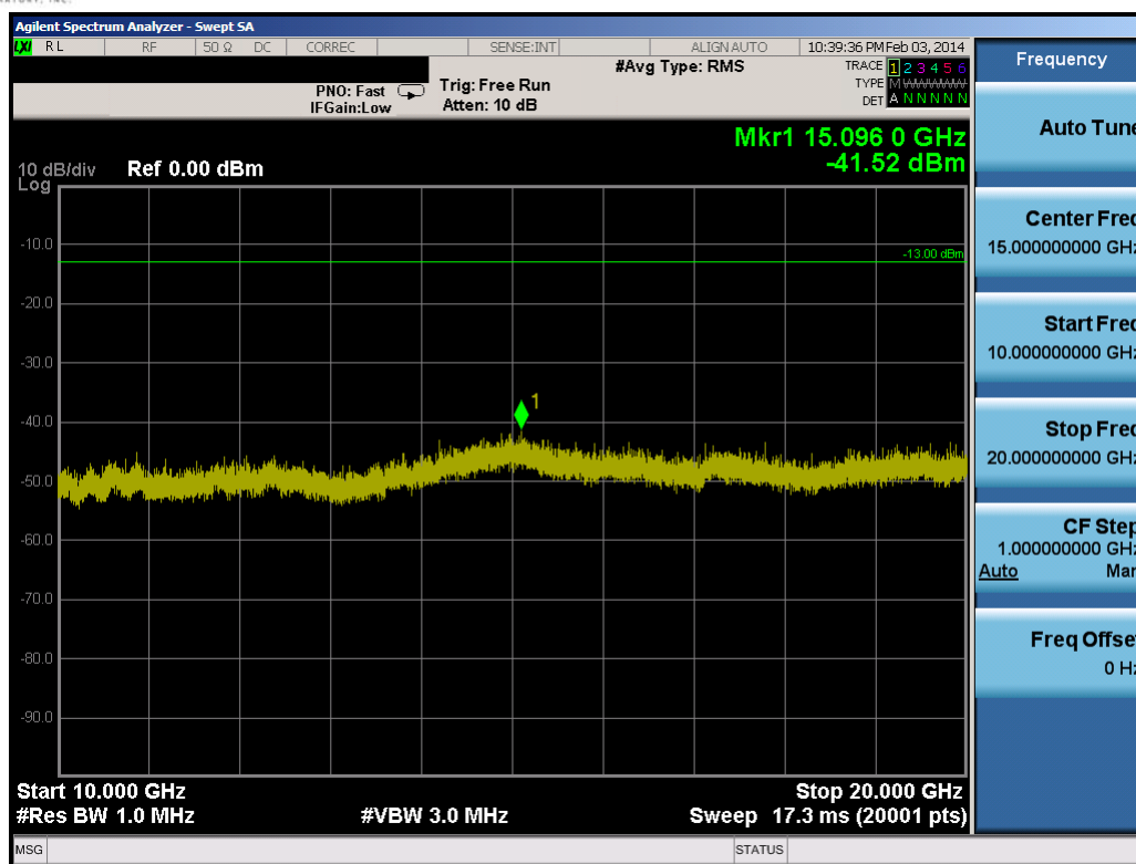
Plot 9-18. Conducted Spurious Plot (10.0MHz QPSK – RB Size 1, RB Offset 0 – High Channel)
