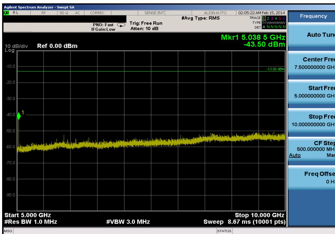
Plot 8-17. Conducted Spurious Plot (5.0MHz QPSK – RB Size 1, RB Offset 0 – High Channel)
