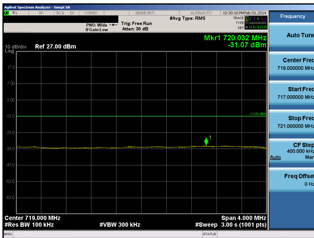
Plot 7-15. Upper Extended Band Edge Plot (10.0MHz QPSK – RB Size 50)
