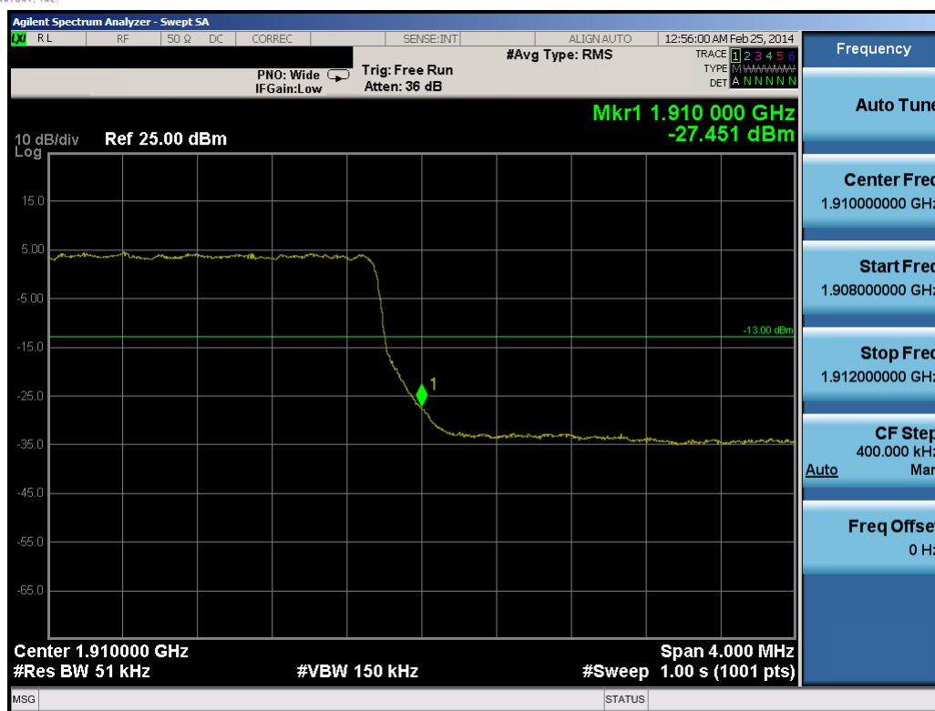
Plot 10-5. Upper Band Edge Plot (5.0MHz QPSK – RB Size 25)
