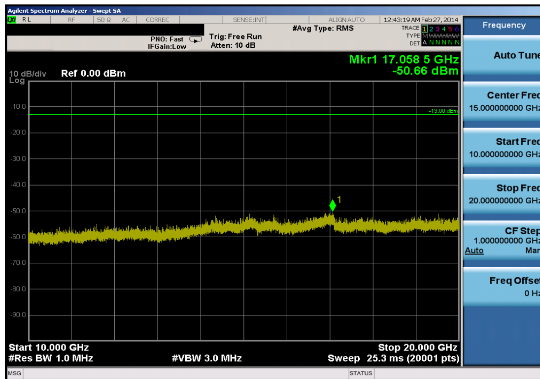
Plot 10-16. Conducted Spurious Plot (10.0MHz QPSK – RB Size 1, RB Offset 0 – Mid Channel)
