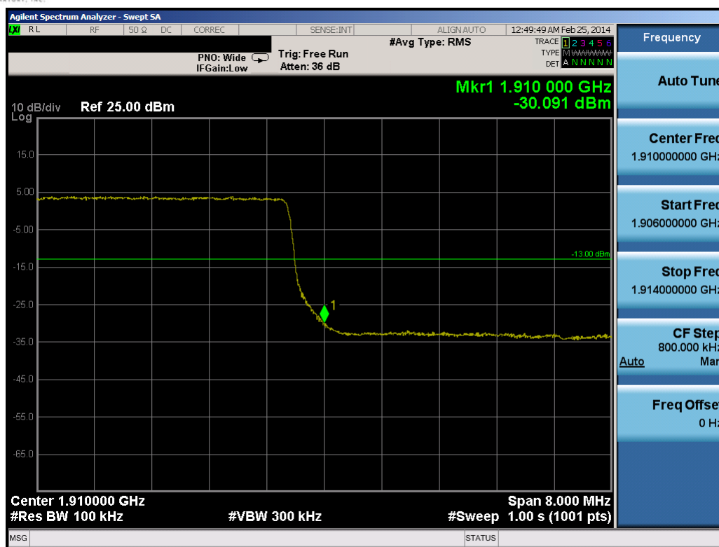
Plot 10-19. Upper Band Edge Plot (10.0MHz QPSK – RB Size 50)
