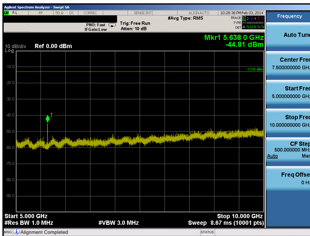
Plot 7-9. Conducted Spurious Plot (10.0MHz QPSK – RB Size 1, RB Offset 0 – Low Channel)
