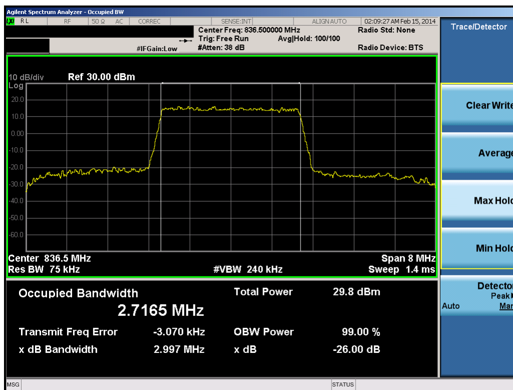
Plot 8-7. Occupied Bandwidth Plot (3.0MHz 16-QAM – RB Size 15)
