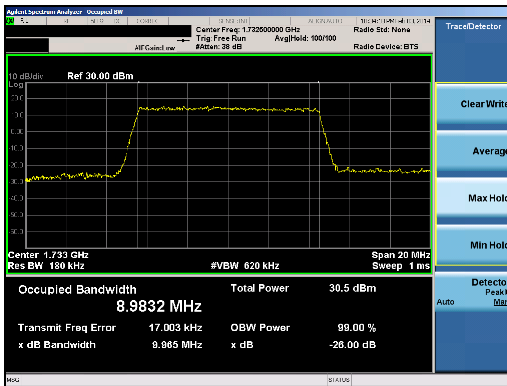
Plot 9-11. Occupied Bandwidth Plot (10.0MHz QPSK – RB Size 50)
