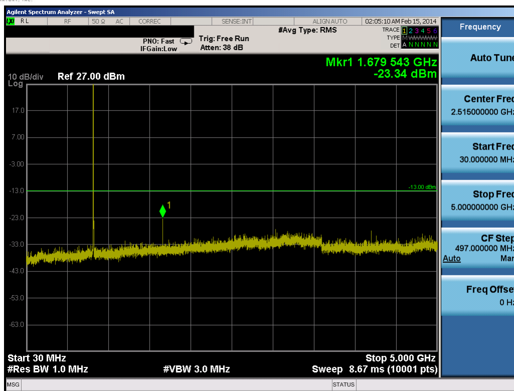
Plot 8-26. Conducted Spurious Plot (10.0MHz QPSK – RB Size 1, RB Offset 0 – High Channel)
