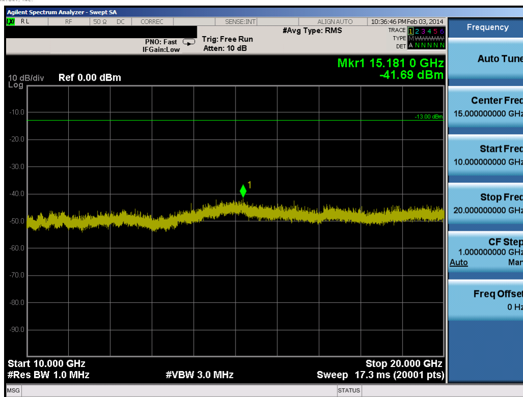
Plot 9-16. Conducted Spurious Plot (10.0MHz QPSK – RB Size 1, RB Offset 0 – Mid Channel)
