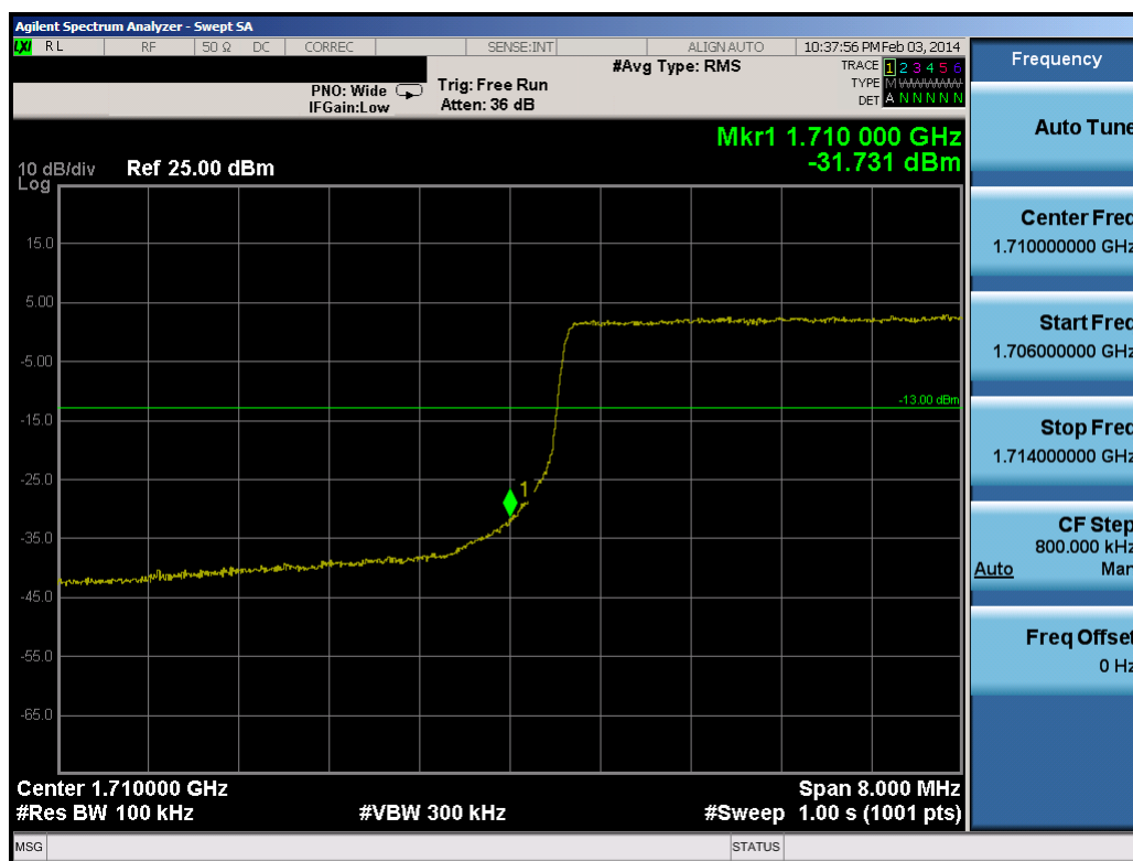
Plot 9-9. Lower Band Edge Plot (10.0MHz QPSK – RB Size 50)
