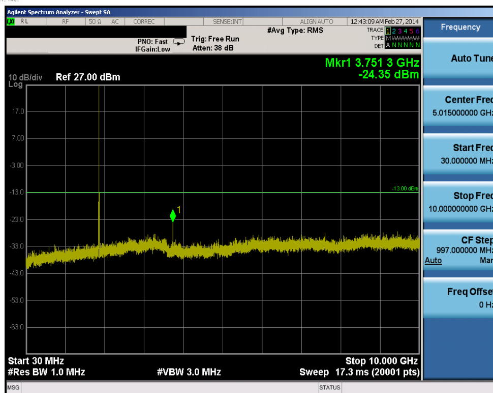
Plot 10-15. Conducted Spurious Plot (10.0MHz QPSK – RB Size 1, RB Offset 0 – Mid Channel)
