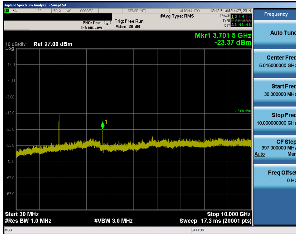
Plot 10-13. Conducted Spurious Plot (10.0MHz QPSK – RB Size 1, RB Offset 0– Low Channel)
