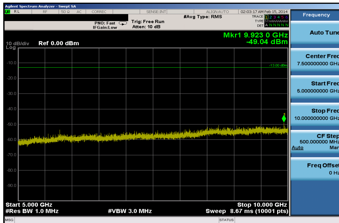
Plot 8-13. Conducted Spurious Plot (5.0MHz QPSK – RB Size 1, RB Offset 0 – Low Channel)
