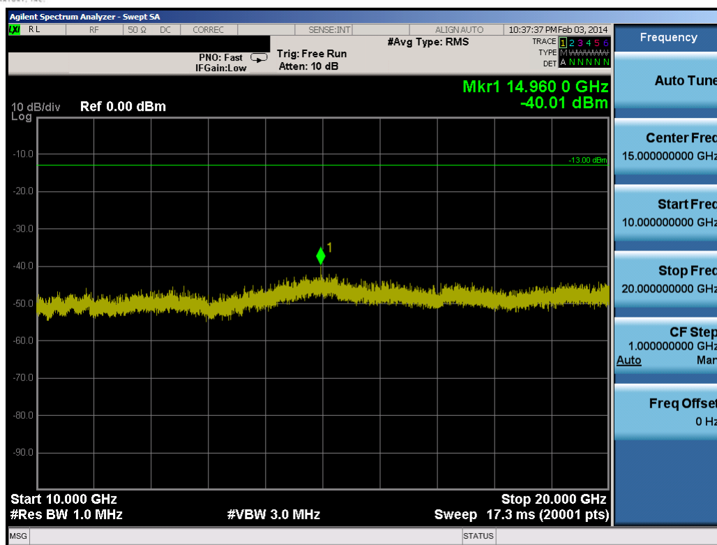
Plot 9-14. Conducted Spurious Plot (10.0MHz QPSK – RB Size 1, RB Offset 0 – Low Channel)
