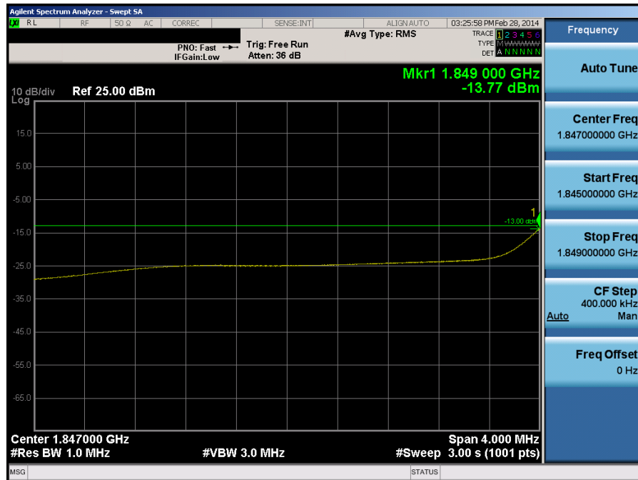
Plot 10-2. Extended Lower Band Edge Plot (5.0MHz QPSK – RB Size 25)
