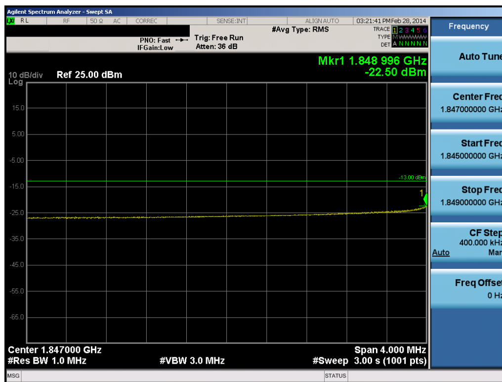
Plot 10-10. Extended Lower Band Edge Plot (10.0MHz QPSK – RB Size 50)
