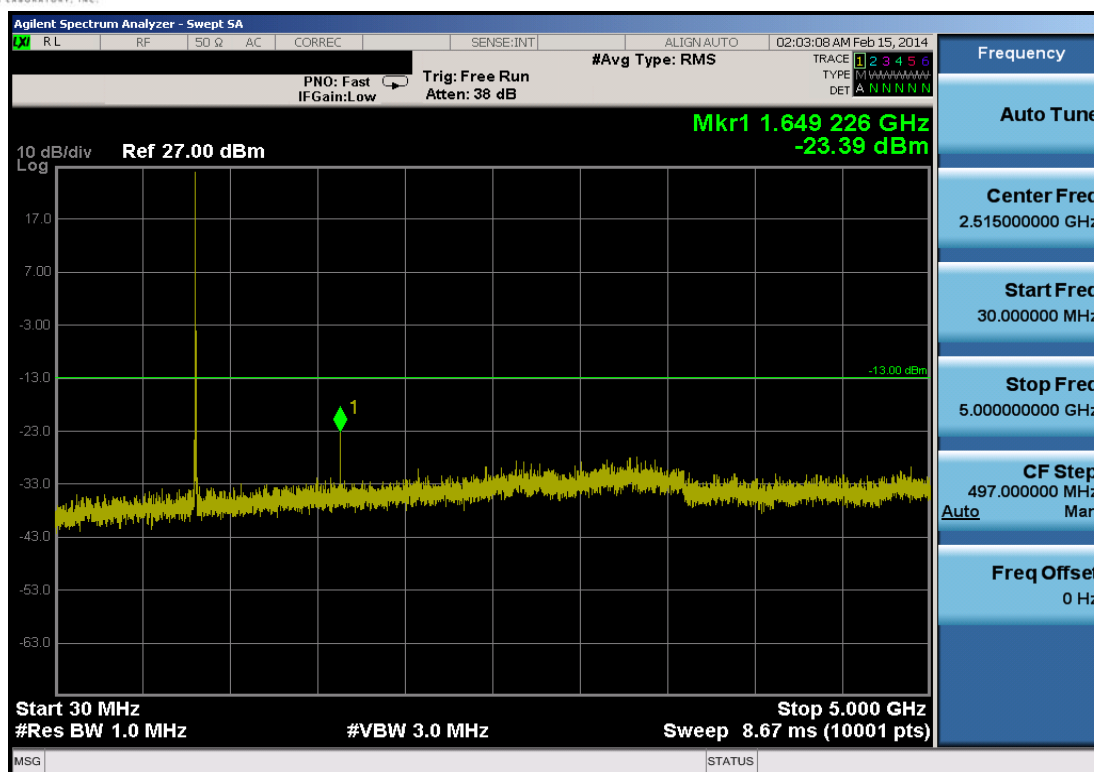
Plot 8-12. Conducted Spurious Plot (5.0MHz QPSK – RB Size 1, RB Offset 0 – Low Channel)
