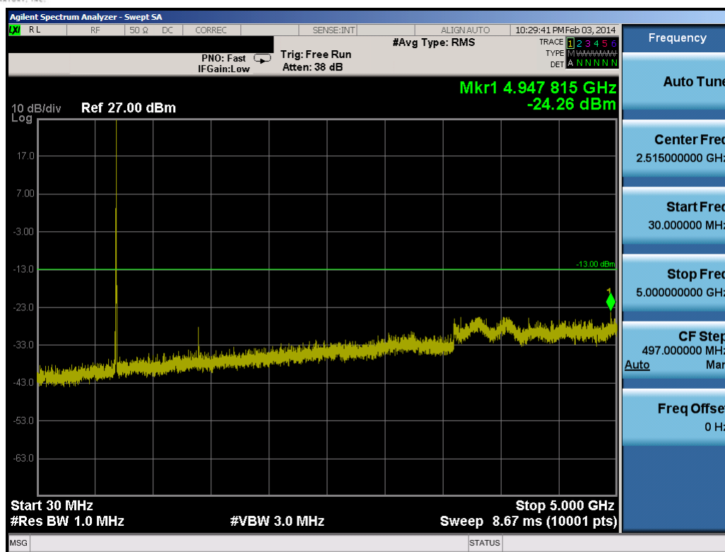
Plot 7-12. Conducted Spurious Plot (10.0MHz QPSK – RB Size 1, RB Offset 0 – High Channel)
