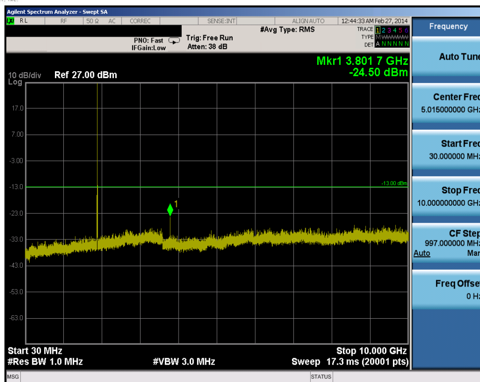
Plot 10-17. Conducted Spurious Plot (10.0MHz QPSK – RB Size 1, RB Offset 0 – High Channel)
