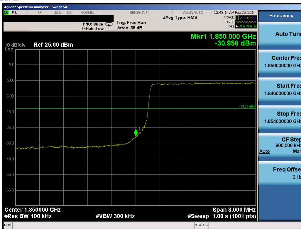
Plot 10-9. Lower Band Edge Plot (10.0MHz QPSK – RB Size 50)
