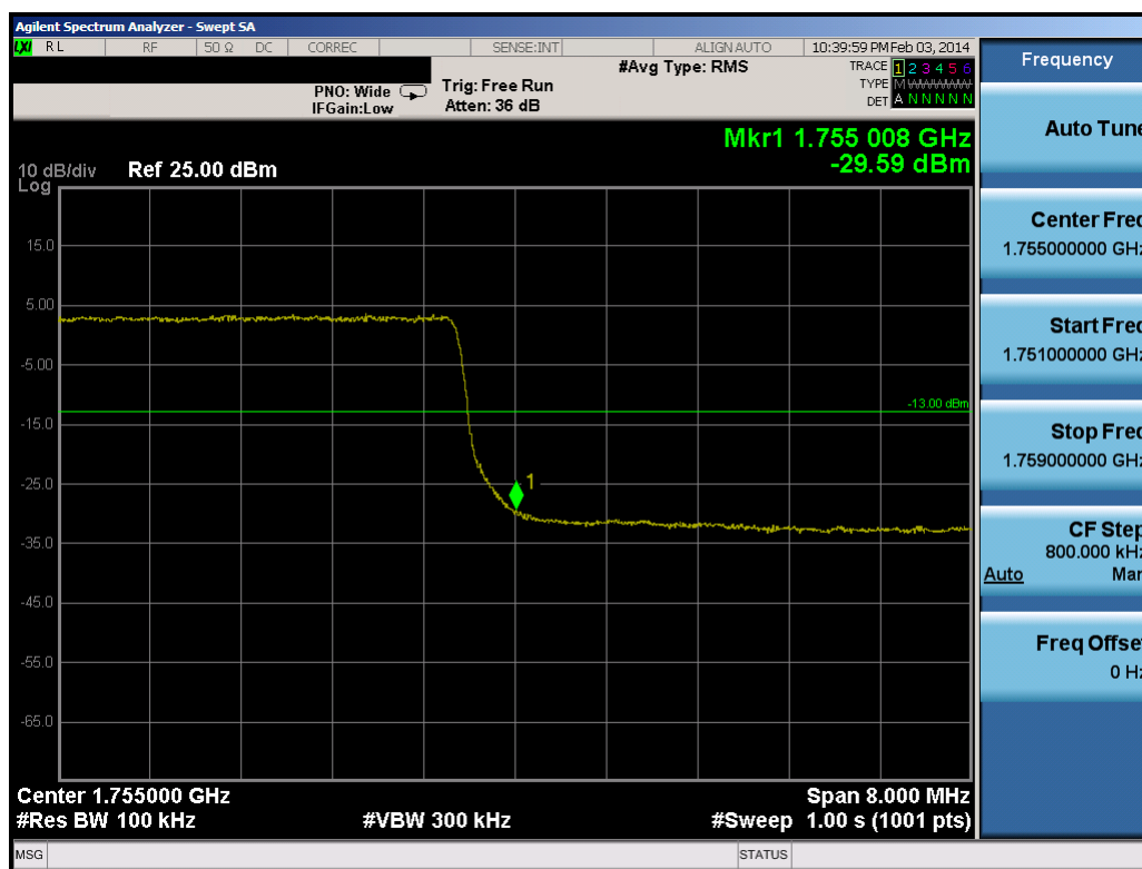
Plot 9-19. Upper Band Edge Plot (10.0MHz QPSK – RB Size 50)
