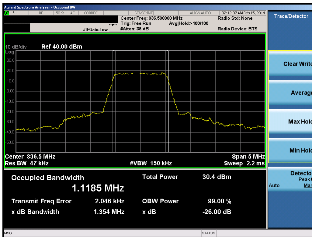
Plot 8-3. Occupied Bandwidth Plot (1.4MHz 16-QAM – RB Size 6)
