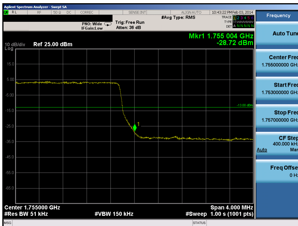
Plot 9-5. Upper Band Edge Plot (5.0MHz QPSK – RB Size 25)
