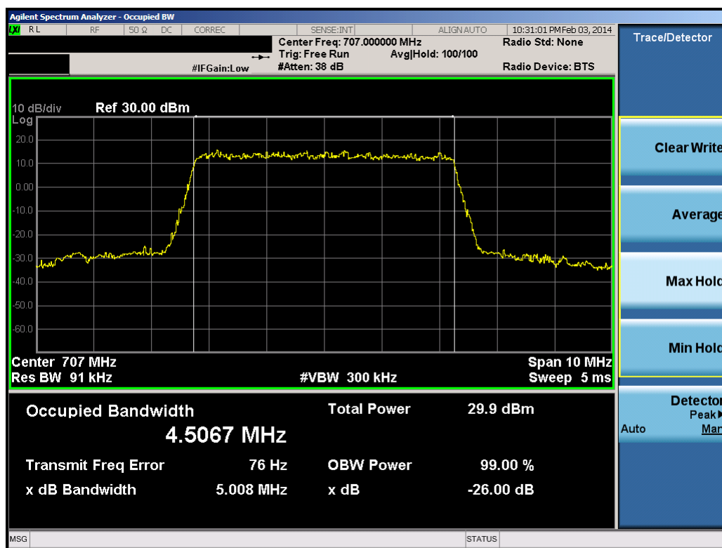
Plot 7-3. Occupied Bandwidth Plot (5.0MHz 16-QAM – RB Size 25)
