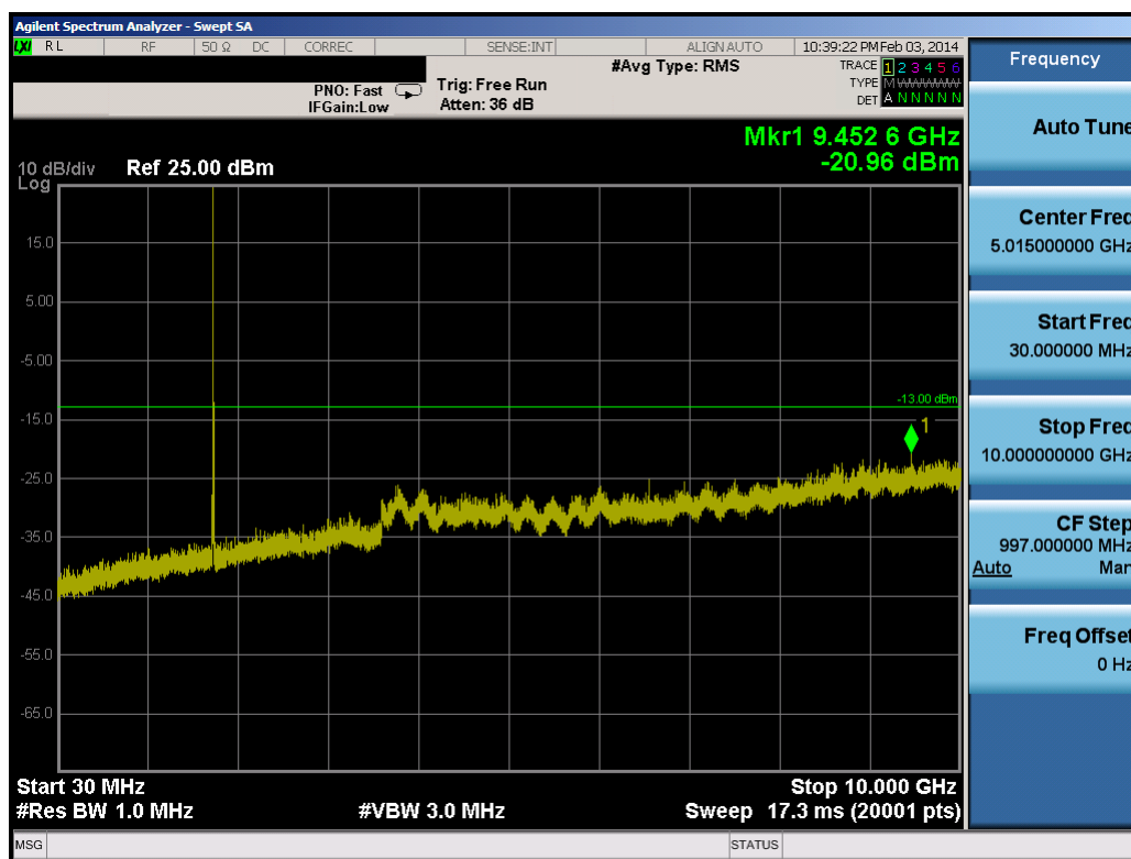
Plot 9-17. Conducted Spurious Plot (10.0MHz QPSK – RB Size 1, RB Offset 0 – High Channel)
