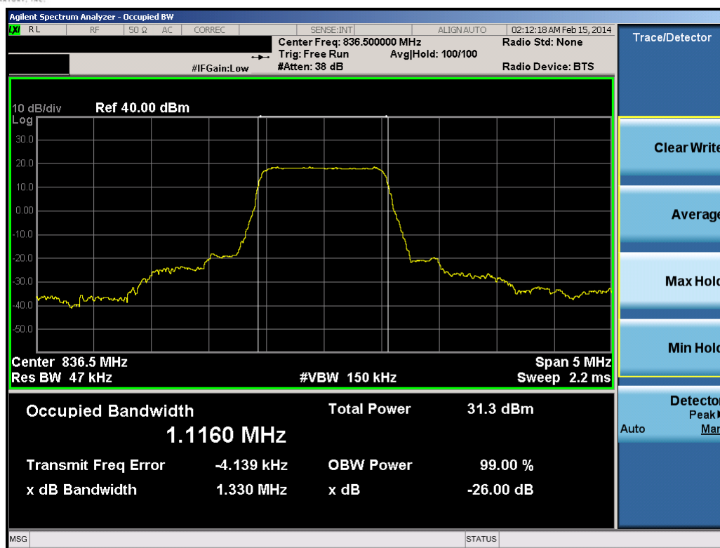
Plot 8-2. Occupied Bandwidth Plot (1.4MHz QPSK – RB Size 6)
