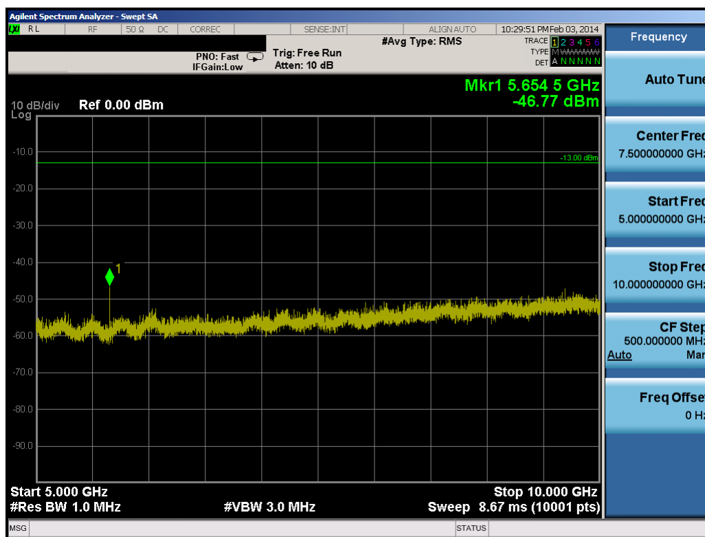
Plot 7-13. Conducted Spurious Plot (10.0MHz QPSK – RB Size 1, RB Offset 0 – High Channel)
