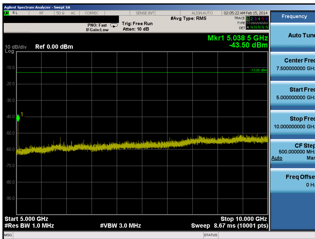
Plot 8-27. Conducted Spurious Plot (10.0MHz QPSK – RB Size 1, RB Offset 0 – High Channel)
