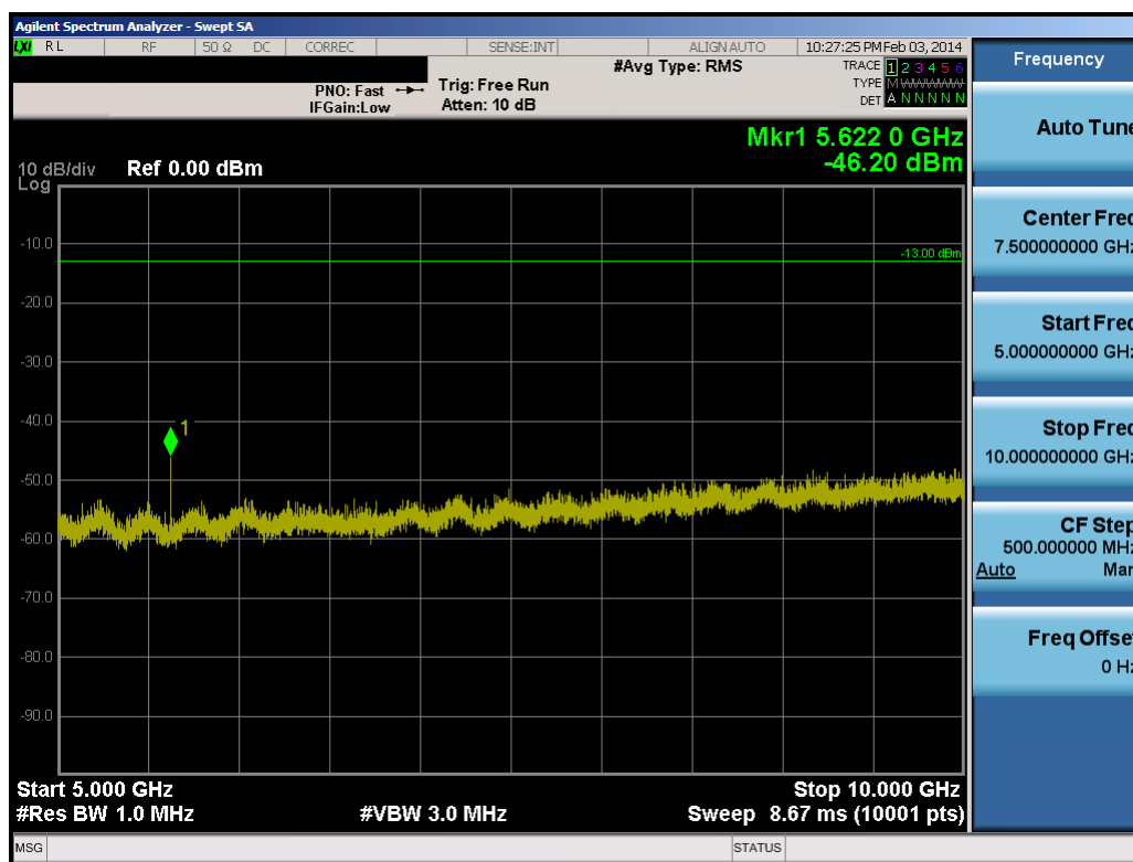
Plot 7-11. Conducted Spurious Plot (10.0MHz QPSK – RB Size 1, RB Offset 0 – Mid Channel)
