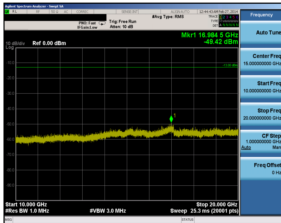
Plot 10-18. Conducted Spurious Plot (10.0MHz QPSK – RB Size 1, RB Offset 0 – High Channel)
