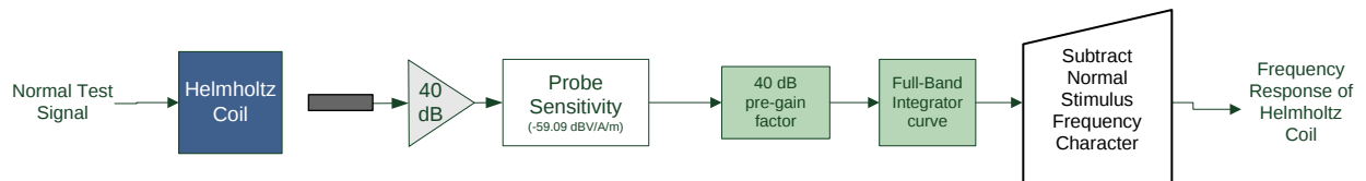
Figure 5-12 Frequency Response Block Diagram
