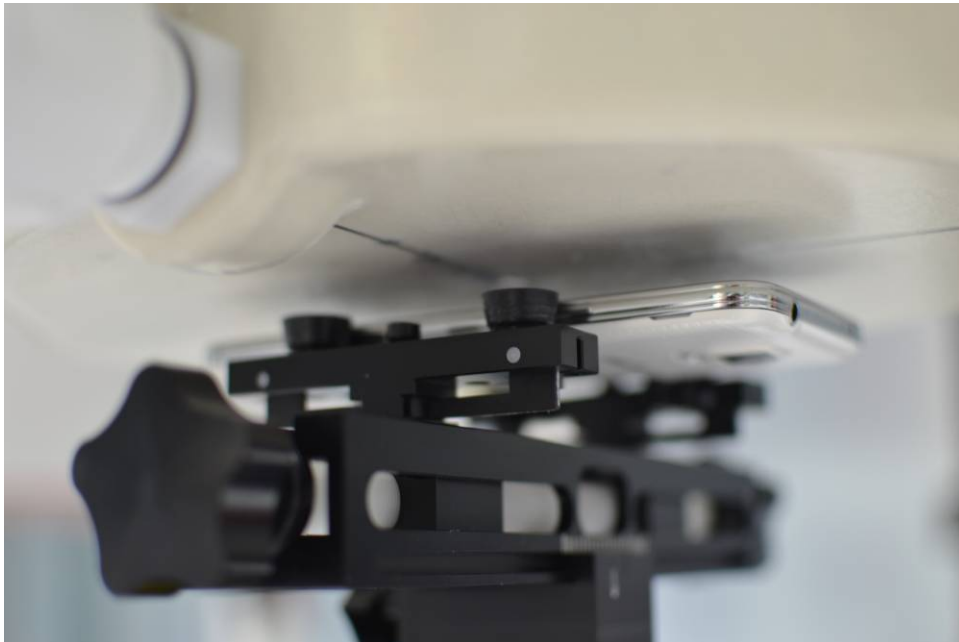
SAR Test Setup Photo 10: Front Side at 1.0 cm with Standard Cover
