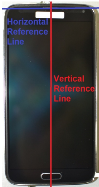
SAR Test Setup Photo 18: Vertical and Horizontal Reference Lines
