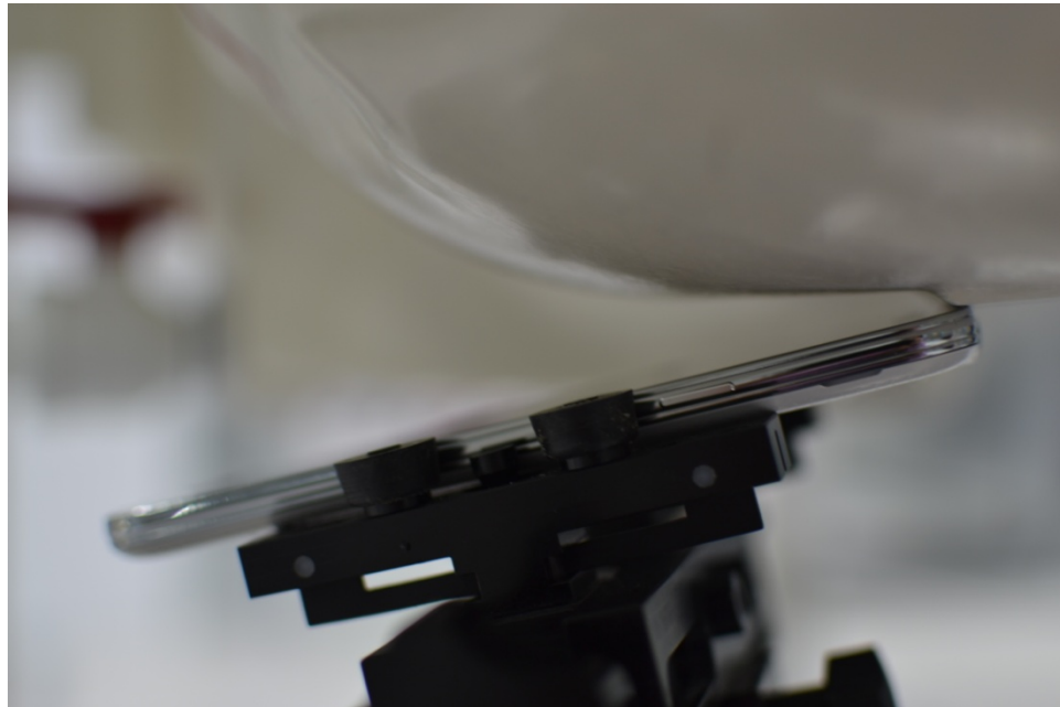
SAR Test Setup Photo 6: Left Tilt with Standard Cover
