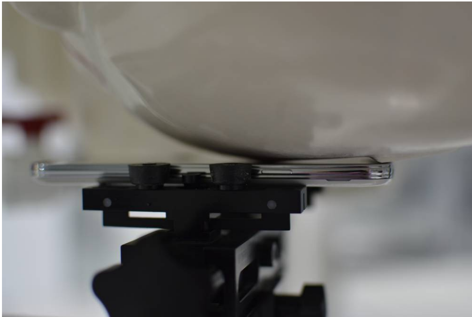
SAR Test Setup Photo 4: Left Cheek with Standard Cover
