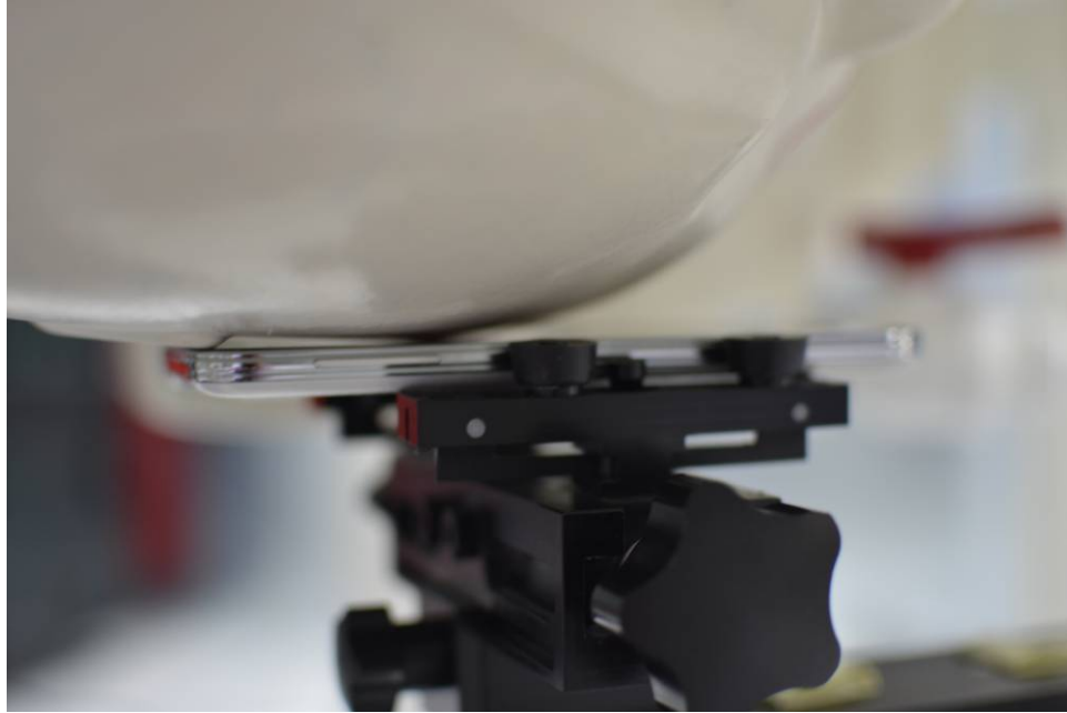
SAR Test Setup Photo 1: Right Cheek with Standard Cover
