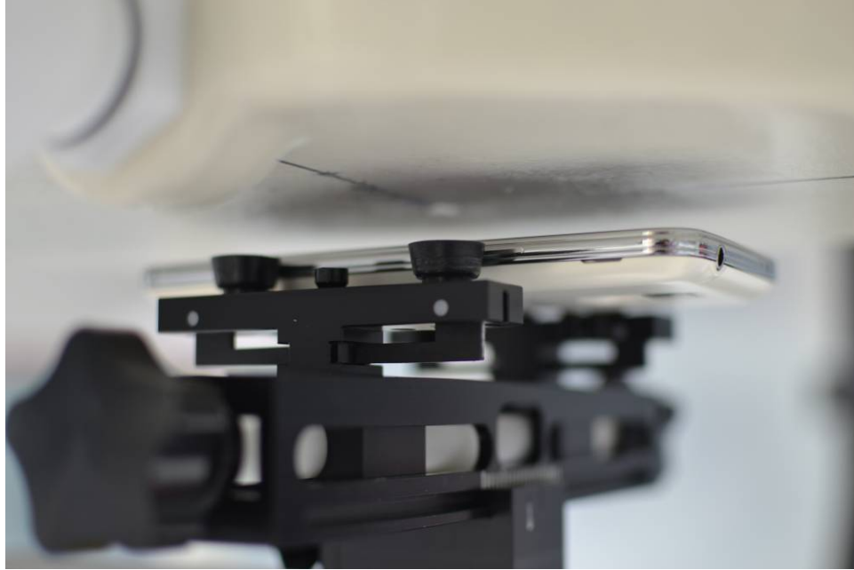
SAR Test Setup Photo 11: Front Side at 1.0 cm with Wireless Charging Cover
