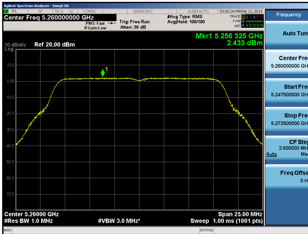
Plot 6-78. Peak Power Spectral Density Plot (802.11a (UNII Band 2A) – Ch. 52)
