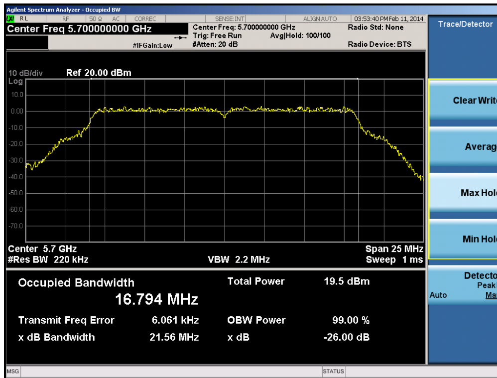
Plot 6-55. 26dB Bandwidth Plot (802.11a (UNII Band 2C) – Ch. 140)
