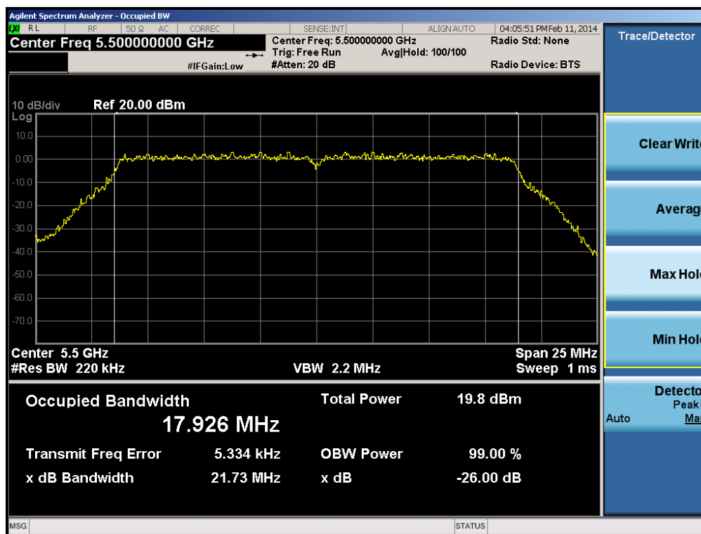
Plot 6-56. 26dB Bandwidth Plot (20MHz BW 802.11n (UNII Band 2C) – Ch. 100)
