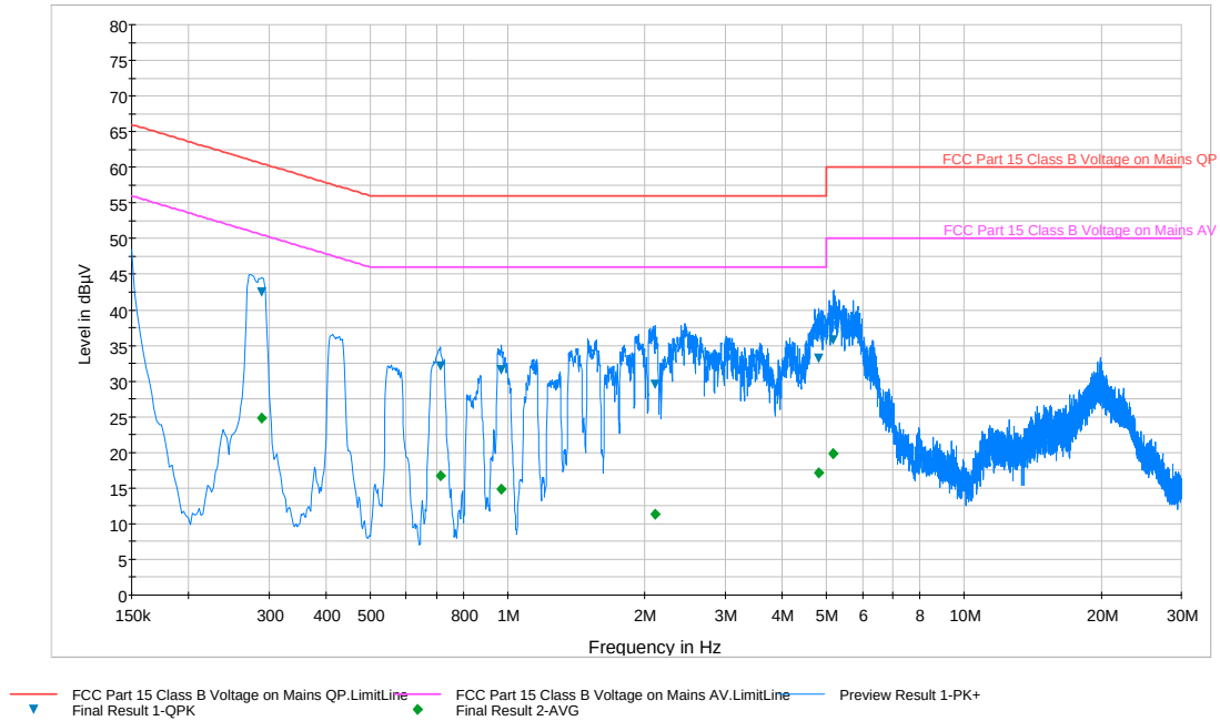
Plot 6-200. Line Conducted Plot with 802.11a UNII Band 1 (N)
