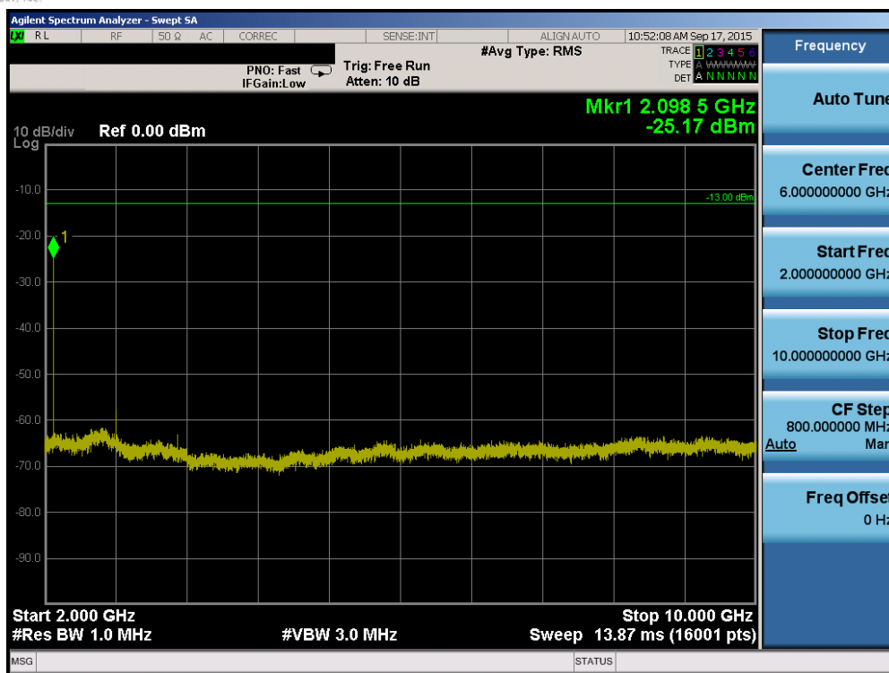
Plot 6-47. Conducted Spurious Plot (Band 12/17 – 5.0MHz QPSK – RB Size 1, RB Offset 0 – Low Channel)
