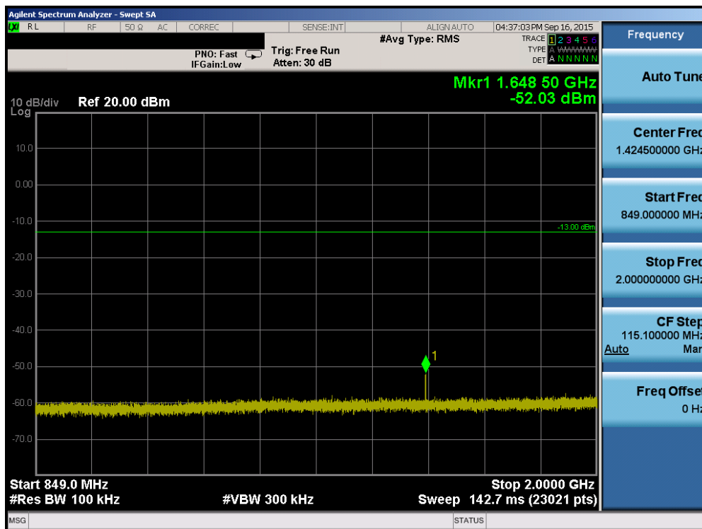
Plot 6-64. Conducted Spurious Plot (Band 5 – 1.4MHz QPSK – RB Size 1, RB Offset 0 – Low Channel)
