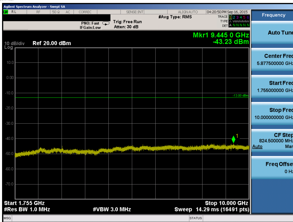
Plot 6-73. Conducted Spurious Plot (Band 4 – 3.0MHz QPSK – RB Size 1, RB Offset 0 – Low Channel)
