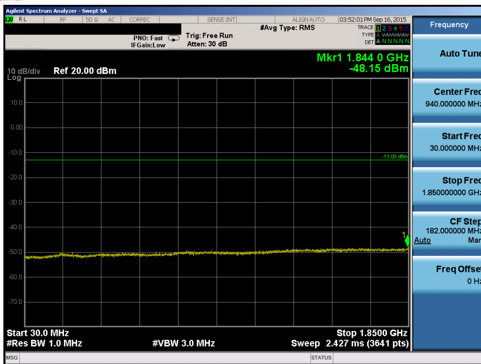
Plot 6-87. Conducted Spurious Plot (Band 2 – 3.0MHz QPSK – RB Size 1, RB Offset 0 – High Channel)
