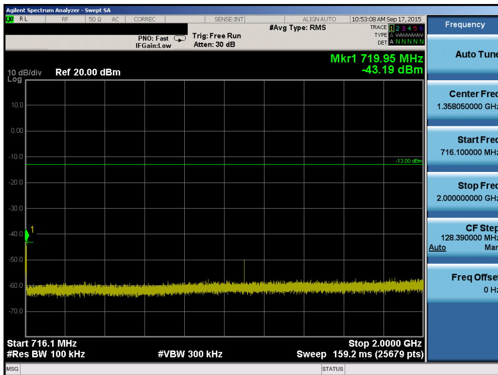
Plot 6-52. Conducted Spurious Plot (Band 12/17 – 5.0MHz QPSK – RB Size 1, RB Offset 0 – High Channel)
