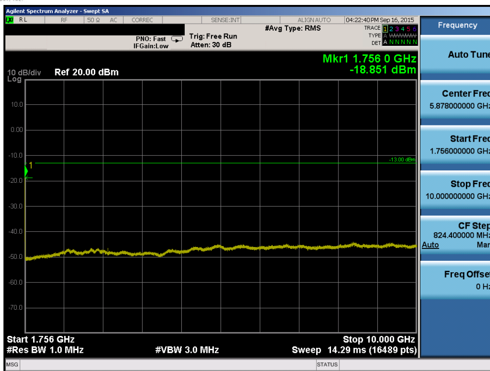
Plot 6-79. Conducted Spurious Plot (Band 4 – 3.0MHz QPSK – RB Size 1, RB Offset 0 – High Channel)
