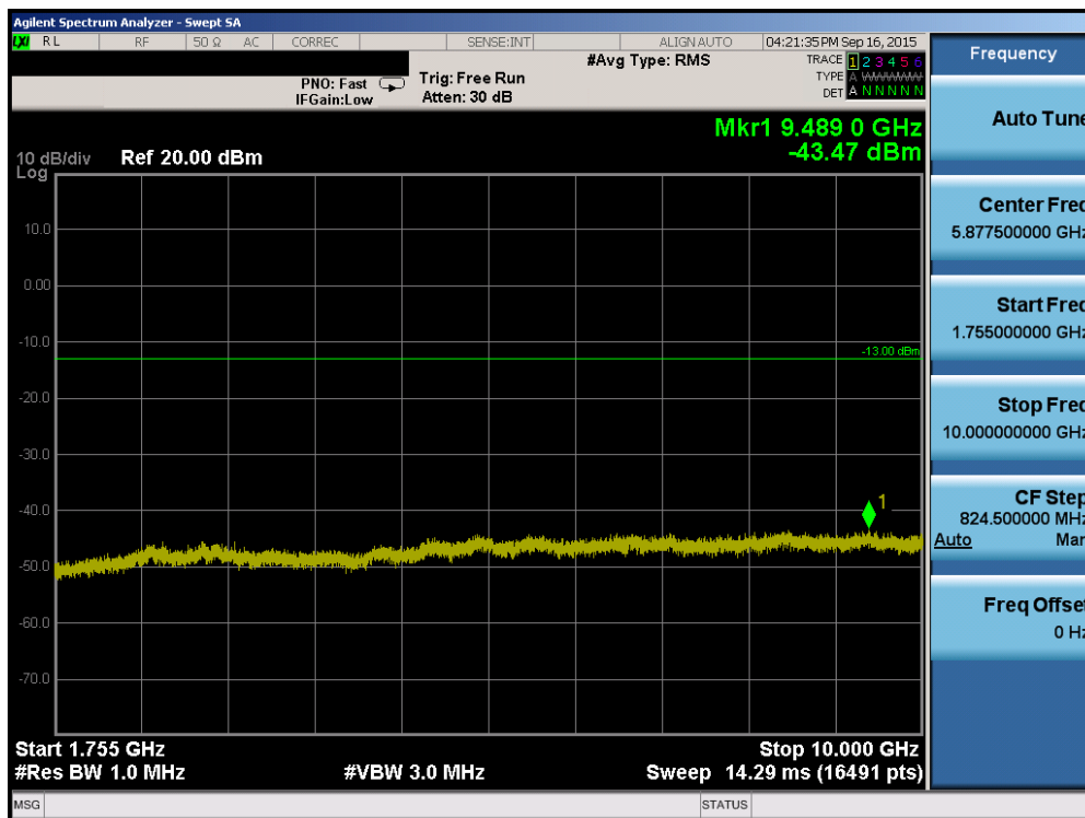
Plot 6-76. Conducted Spurious Plot (Band 4 – 3.0MHz QPSK – RB Size 1, RB Offset 0 – Mid Channel)
