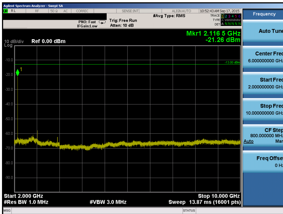
Plot 6-50. Conducted Spurious Plot (Band 12/17 – 5.0MHz QPSK – RB Size 1, RB Offset 0 – Mid Channel)
