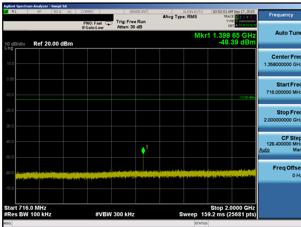
Plot 6-46. Conducted Spurious Plot (Band 12/17 – 5.0MHz QPSK – RB Size 1, RB Offset 0 – Low Channel)
