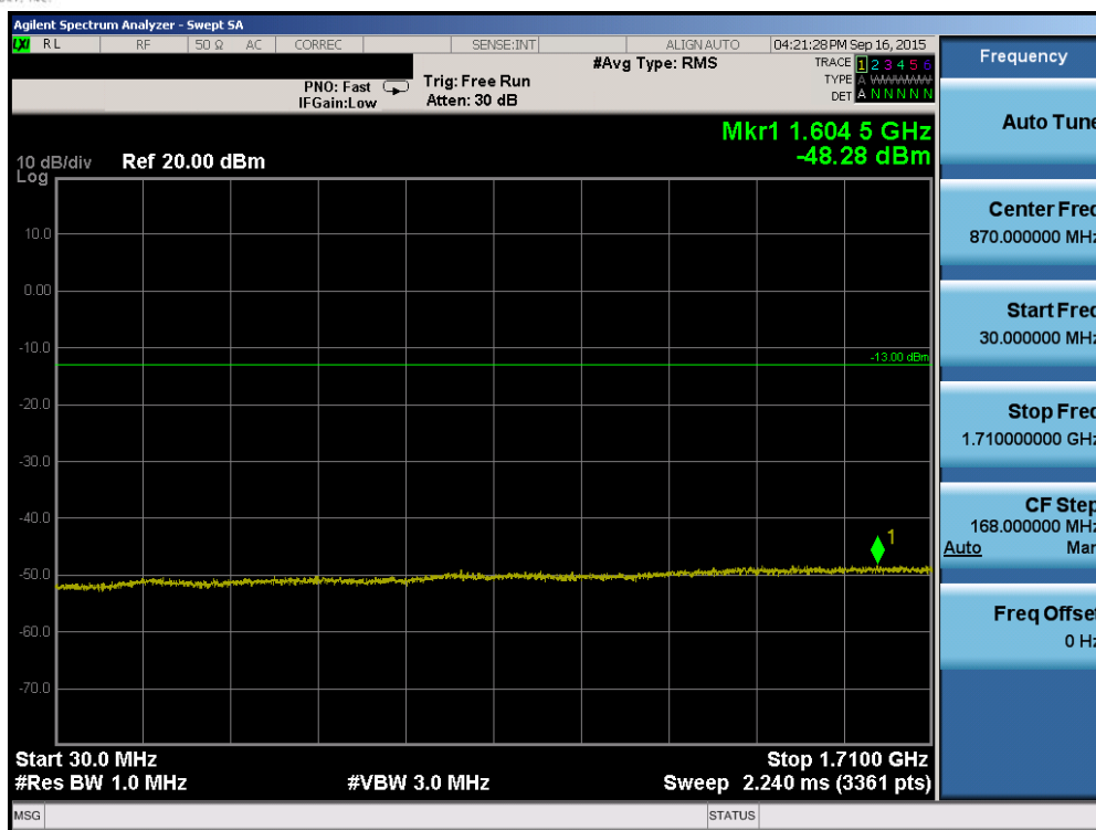
Plot 6-75. Conducted Spurious Plot (Band 4 – 3.0MHz QPSK – RB Size 1, RB Offset 0 – Mid Channel)
