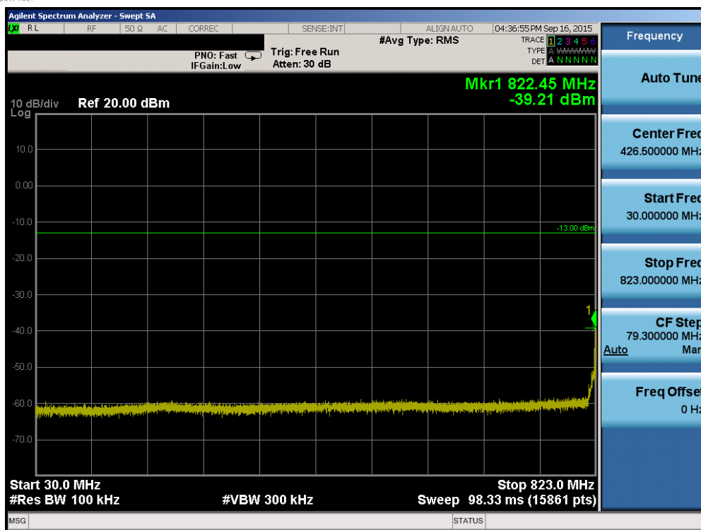
Plot 6-63. Conducted Spurious Plot (Band 5 – 1.4MHz QPSK – RB Size 1, RB Offset 0 – Low Channel)
