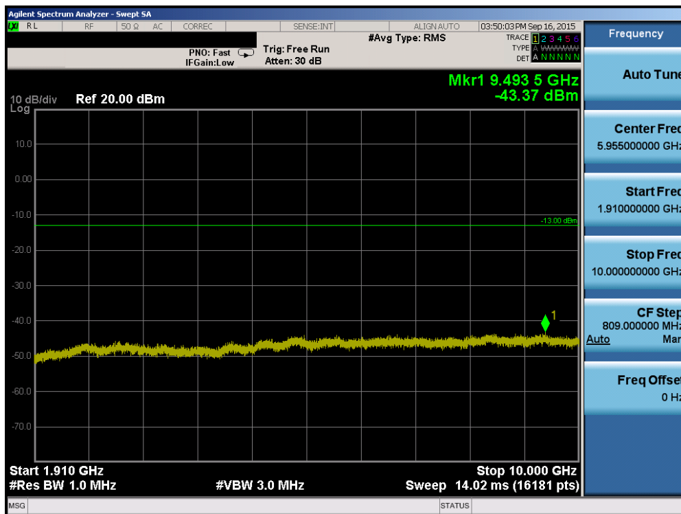
Plot 6-82. Conducted Spurious Plot (Band 2 – 3.0MHz QPSK – RB Size 1, RB Offset 0 – Low Channel)
