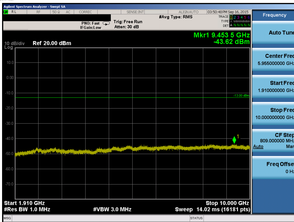
Plot 6-85. Conducted Spurious Plot (Band 2 – 3.0MHz QPSK – RB Size 1, RB Offset 0 – Mid Channel)
