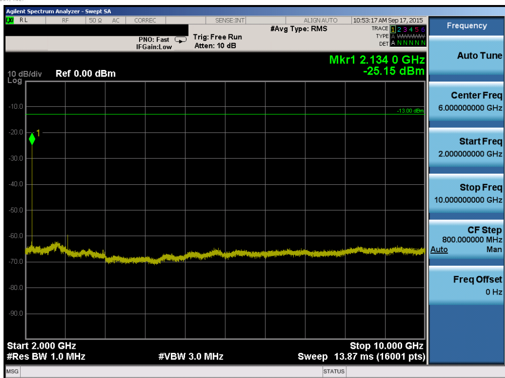
Plot 6-53. Conducted Spurious Plot (Band 12/17 – 5.0MHz QPSK – RB Size 1, RB Offset 0 – High Channel)
