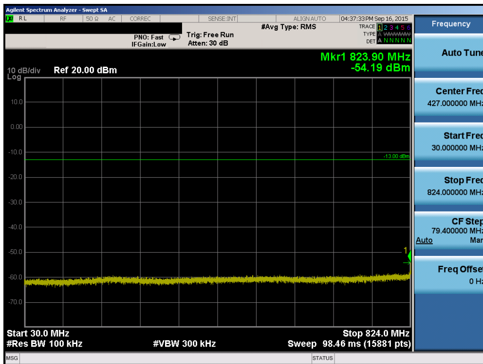
Plot 6-66. Conducted Spurious Plot (Band 5 – 1.4MHz QPSK – RB Size 1, RB Offset 0 – Mid Channel)
