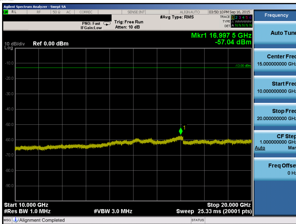
Plot 6-83. Conducted Spurious Plot (Band 2 – 3.0MHz QPSK – RB Size 1, RB Offset 0 – Low Channel)
