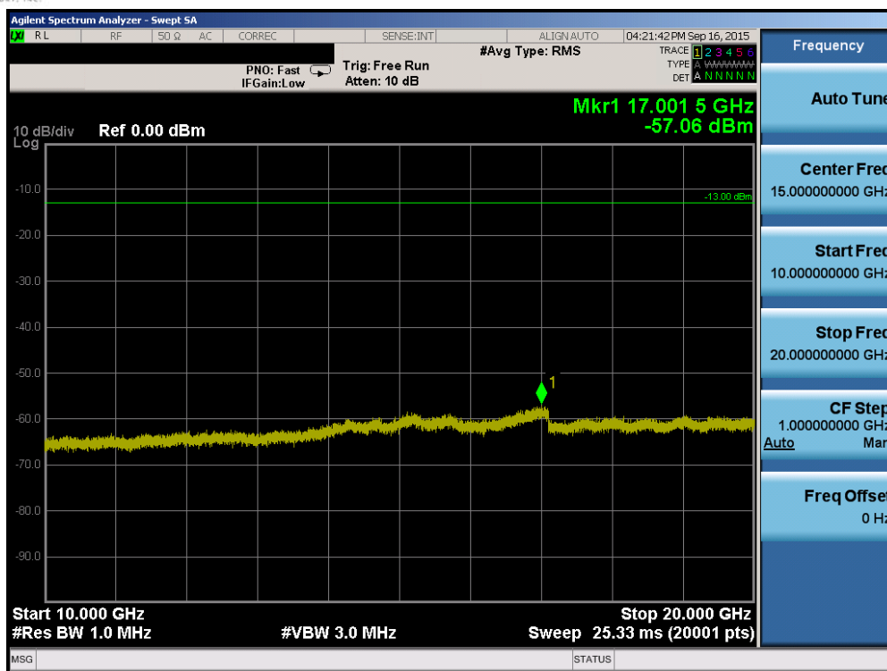
Plot 6-77. Conducted Spurious Plot (Band 4 – 3.0MHz QPSK – RB Size 1, RB Offset 0 – Mid Channel)
