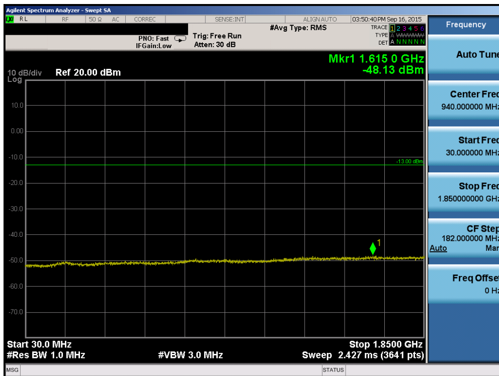
Plot 6-84. Conducted Spurious Plot (Band 2 – 3.0MHz QPSK – RB Size 1, RB Offset 0 – Mid Channel)
