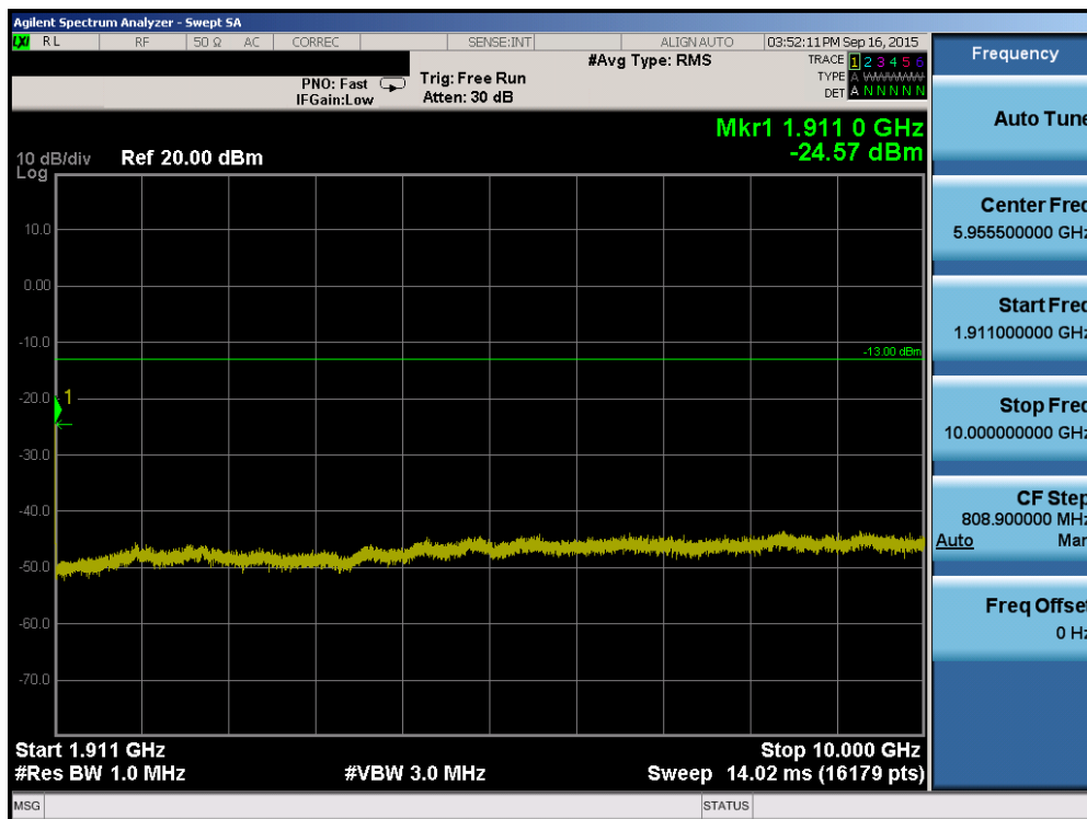
Plot 6-88. Conducted Spurious Plot (Band 2 – 3.0MHz QPSK – RB Size 1, RB Offset 0 – High Channel)
