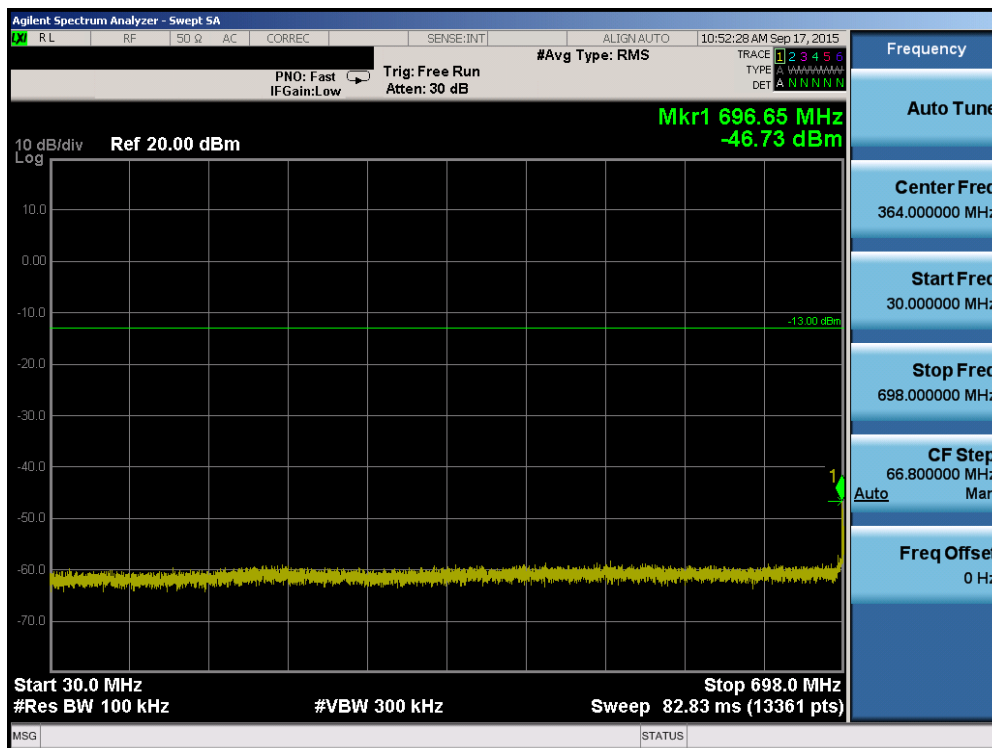
Plot 6-48. Conducted Spurious Plot (Band 12/17 – 5.0MHz QPSK – RB Size 1, RB Offset 0 – Mid Channel)
