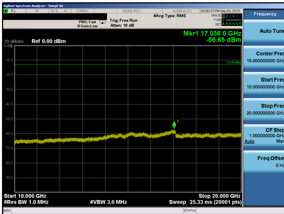
Plot 6-86. Conducted Spurious Plot (Band 2 – 3.0MHz QPSK – RB Size 1, RB Offset 0 – Mid Channel)
