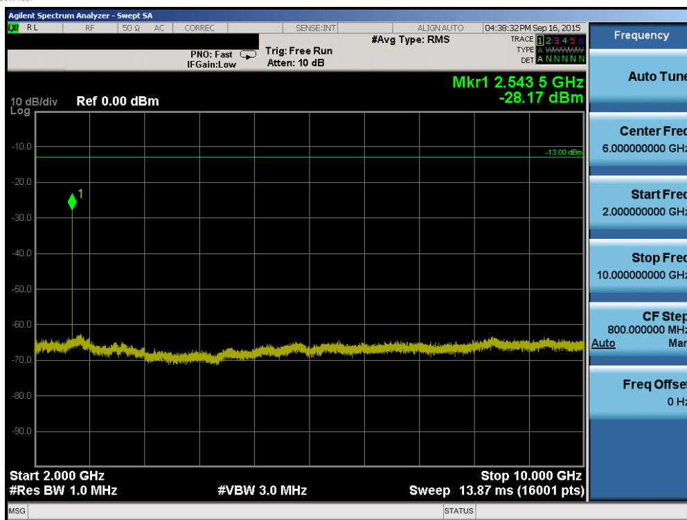
Plot 6-71. Conducted Spurious Plot (Band 5 – 1.4MHz QPSK – RB Size 1, RB Offset 0 – High Channel)
