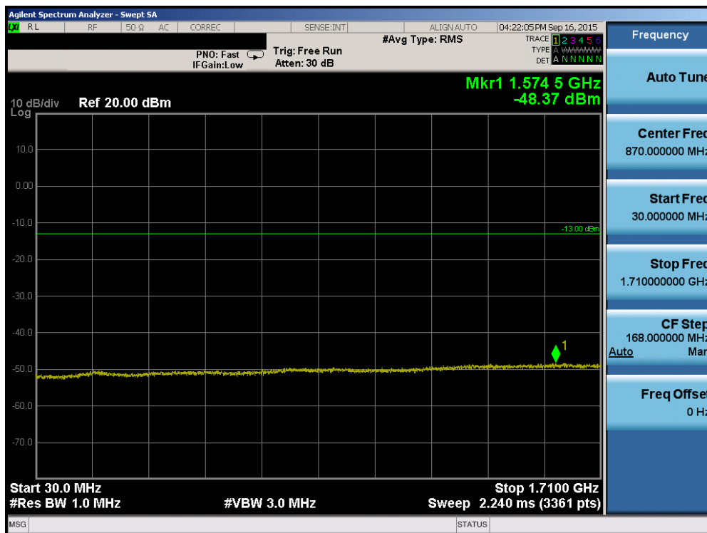
Plot 6-78. Conducted Spurious Plot (Band 4 – 3.0MHz QPSK – RB Size 1, RB Offset 0 – High Channel)
