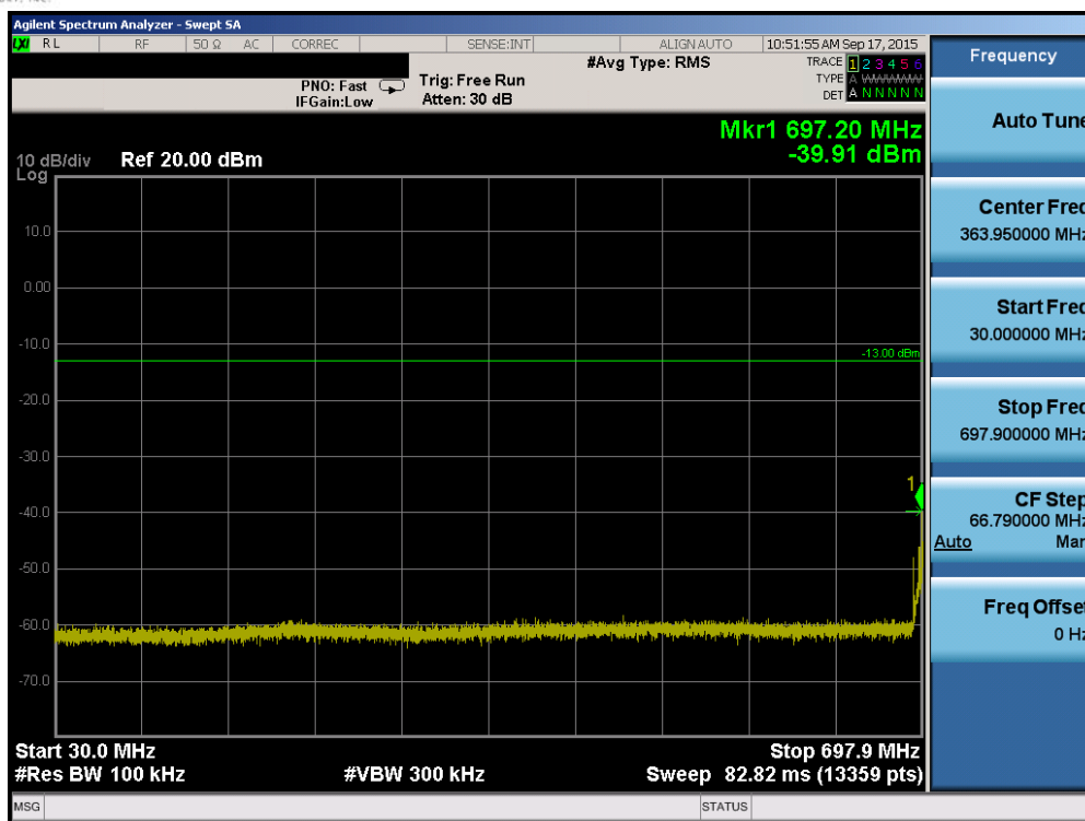
Plot 6-45. Conducted Spurious Plot (Band 12/17 – 5.0MHz QPSK – RB Size 1, RB Offset 0 – Low Channel)
