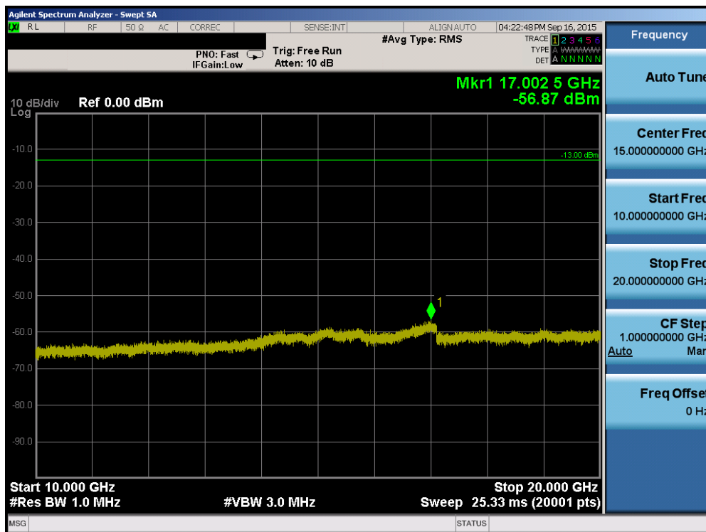
Plot 6-80. Conducted Spurious Plot (Band 4 – 3.0MHz QPSK – RB Size 1, RB Offset 0 – High Channel)
