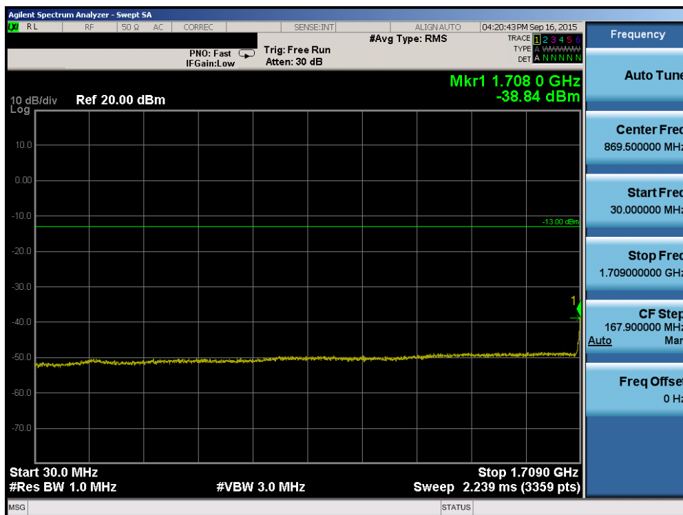
Plot 6-72. Conducted Spurious Plot (Band 4 – 3.0MHz QPSK – RB Size 1, RB Offset 0 – Low Channel)
