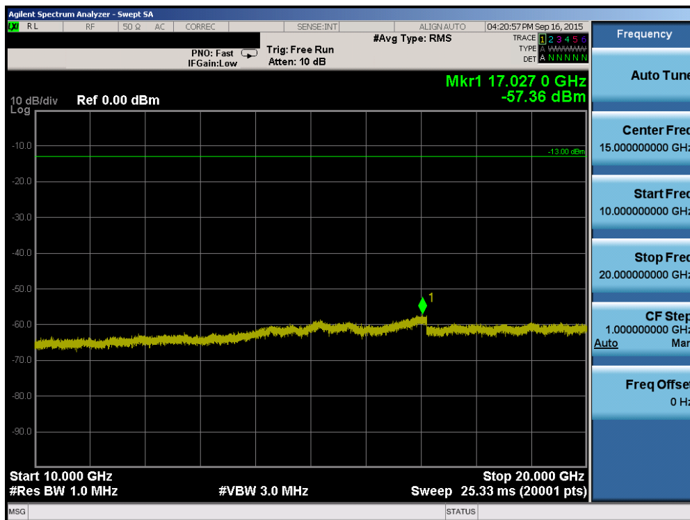
Plot 6-74. Conducted Spurious Plot (Band 4 – 3.0MHz QPSK – RB Size 1, RB Offset 0 – Low Channel)
