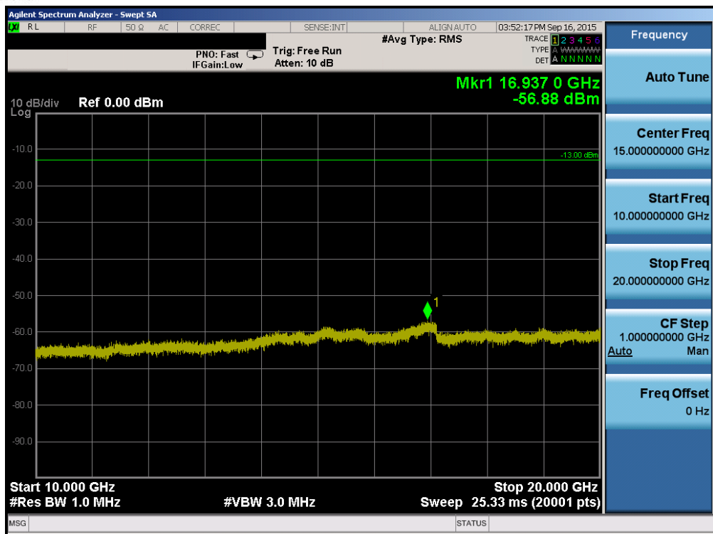
Plot 6-89. Conducted Spurious Plot (Band 2 – 3.0MHz QPSK – RB Size 1, RB Offset 0 – High Channel)
