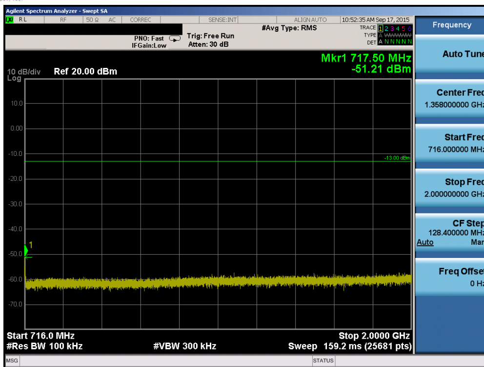
Plot 6-49. Conducted Spurious Plot (Band 12/17 – 5.0MHz QPSK – RB Size 1, RB Offset 0 – Mid Channel)
