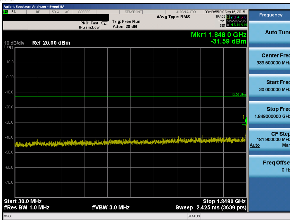
Plot 6-81. Conducted Spurious Plot (Band 2 – 3.0MHz QPSK – RB Size 1, RB Offset 0 – Low Channel)
