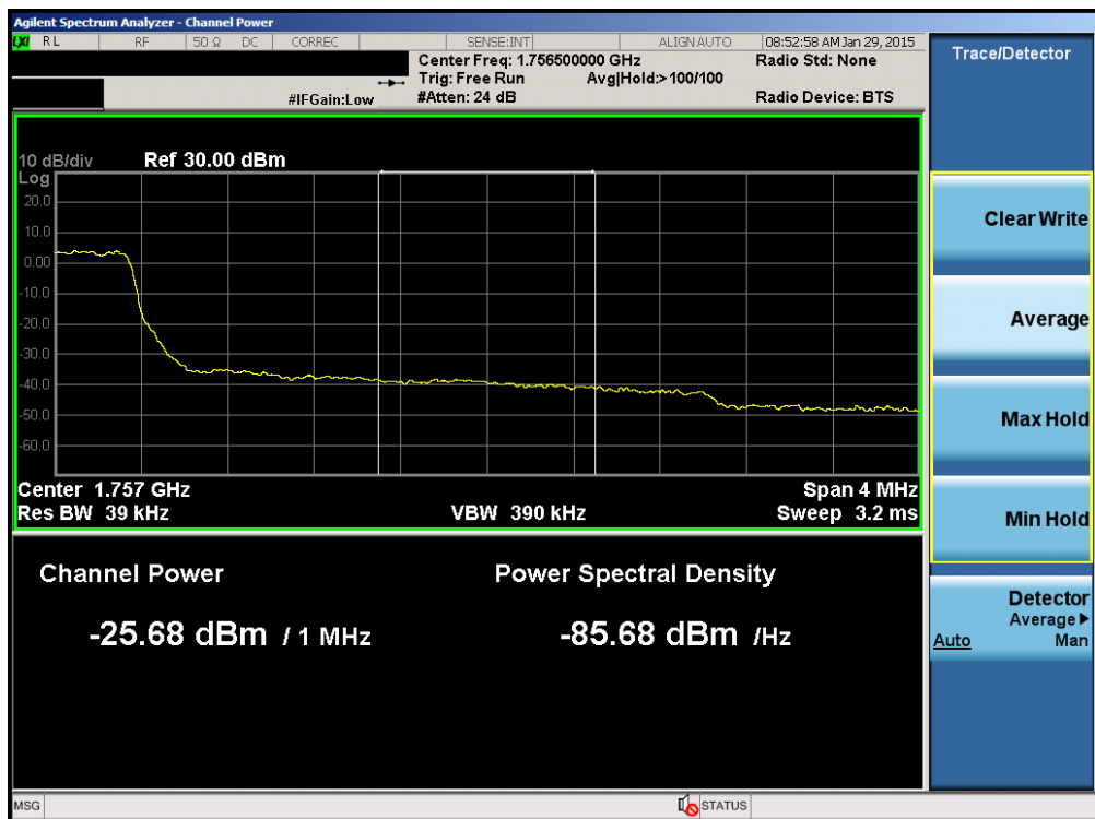
Plot 6-46. Upper Extended Band Edge Plot (Band 4 – 3.0MHz QPSK – RB Size 15)
