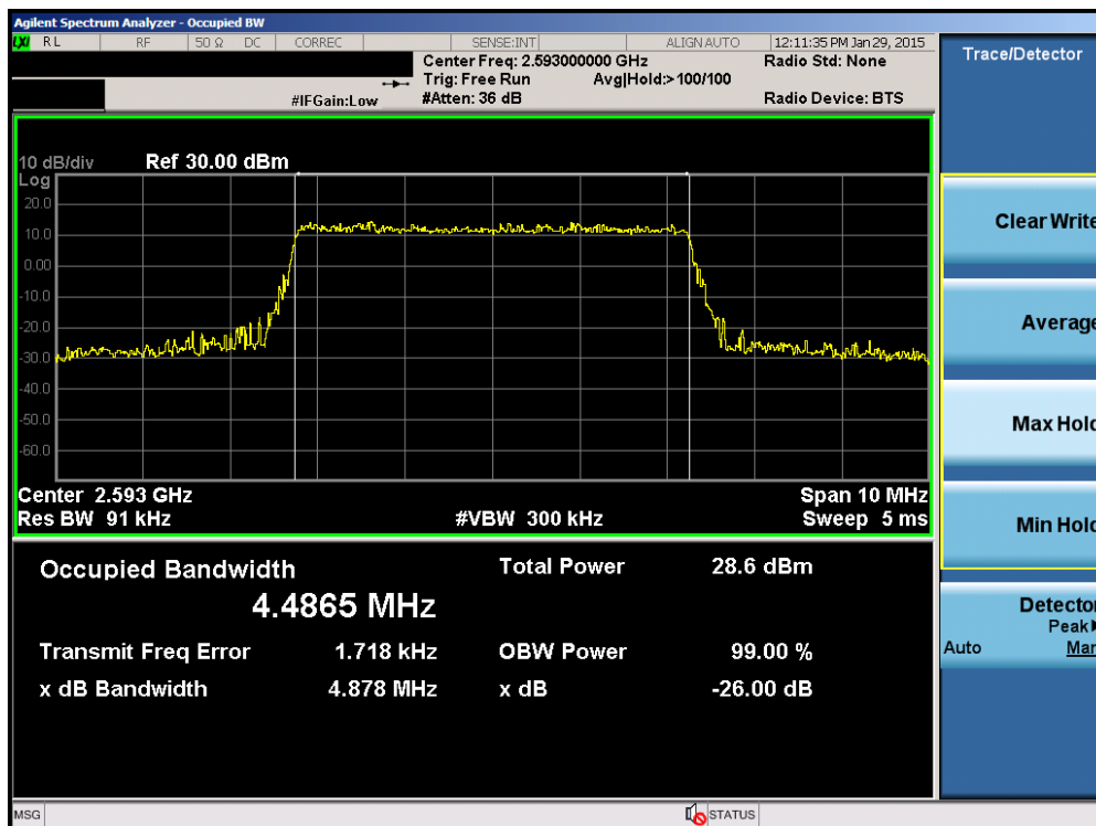
Plot 6-14. Occupied Bandwidth Plot (Band 41 – 5.0MHz 16-QAM – RB Size 25)
