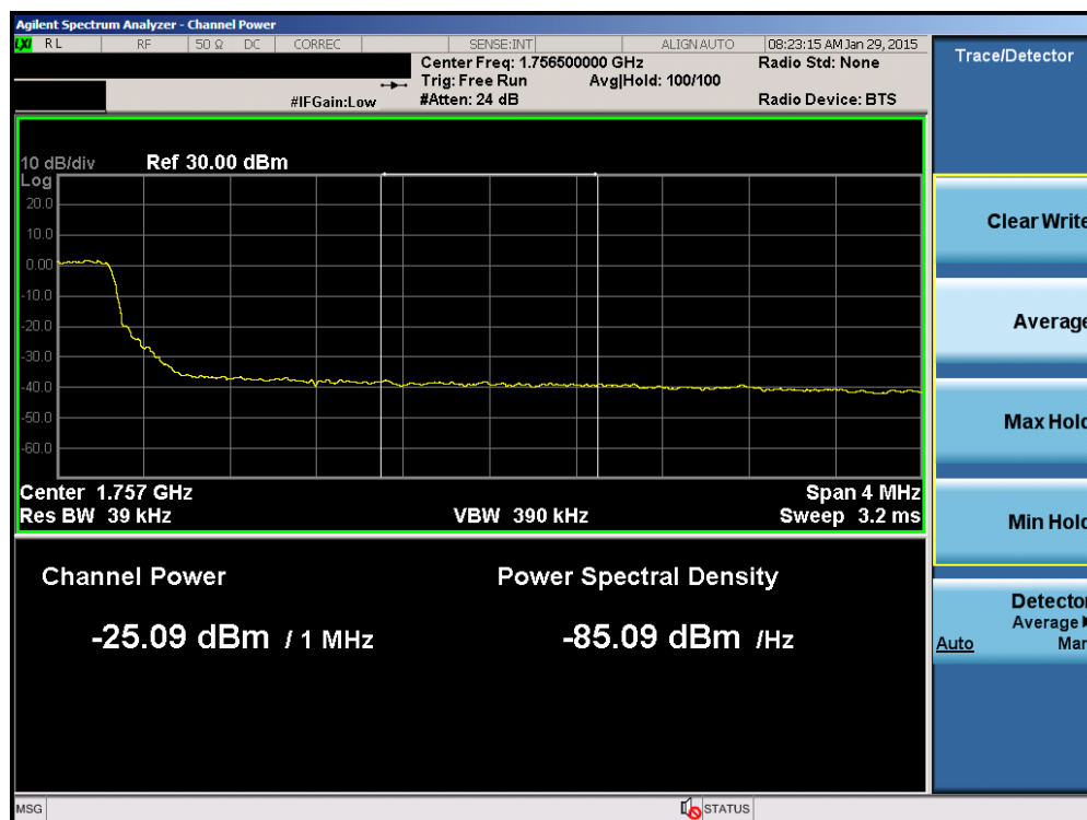
Plot 6-50. Upper Extended Band Edge Plot (Band 4 – 5.0MHz QPSK – RB Size 25)
