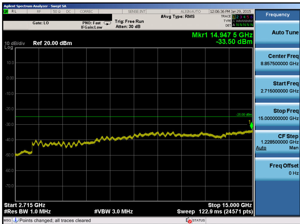
Plot 6-34. Conducted Spurious Plot (Band 41 – 10.0MHz QPSK – RB Size 1, RB Offset 0 – Mid Channel)
