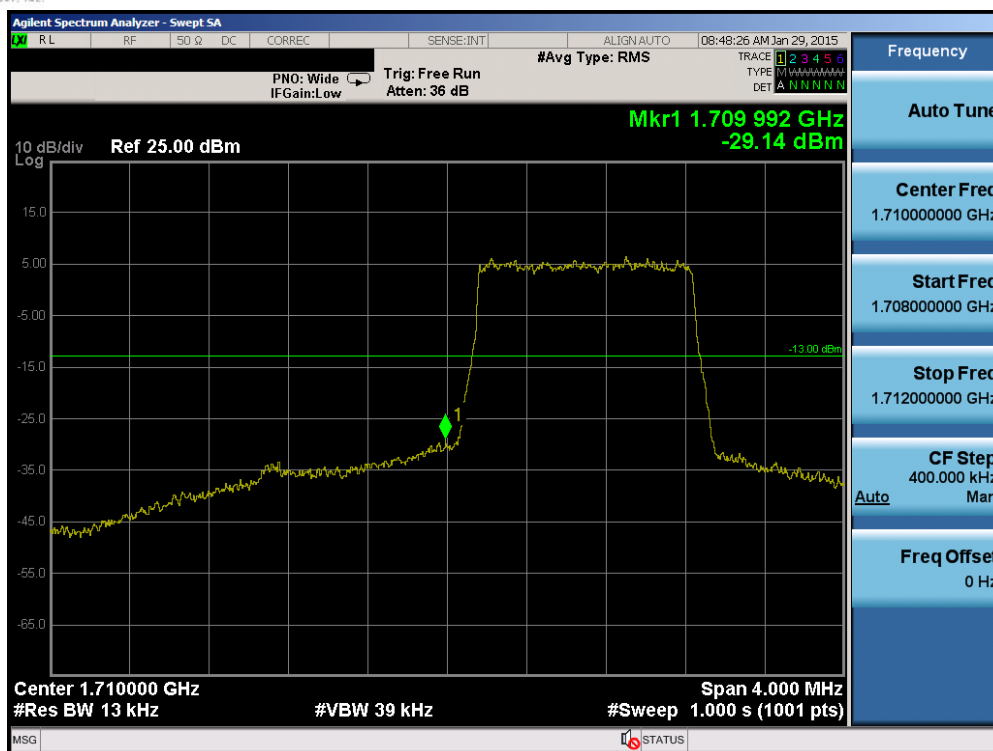
Plot 6-39. Lower Band Edge Plot (Band 4 – 1.4MHz QPSK – RB Size 6)
