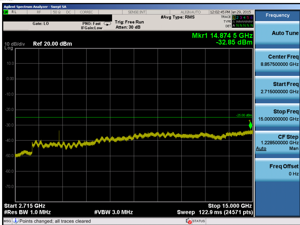
Plot 6-31. Conducted Spurious Plot (Band 41 – 10.0MHz QPSK – RB Size 1, RB Offset 0 – Low Channel)
