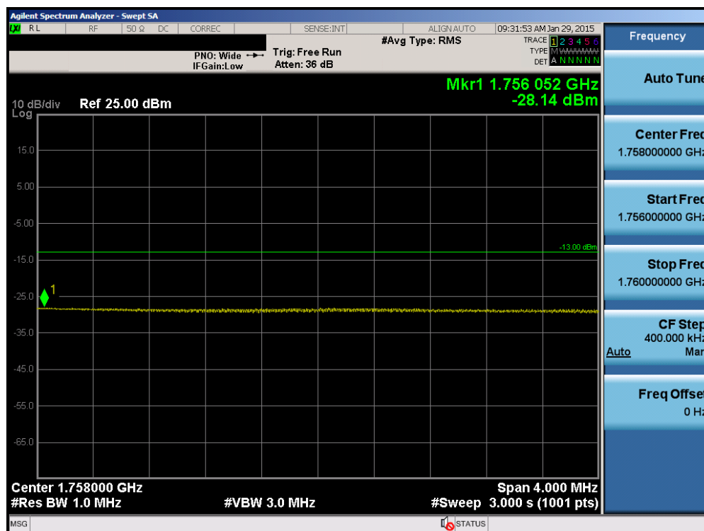
Plot 6-62. Upper Extended Band Edge Plot (Band 4 – 20.0MHz QPSK – RB Size 100)
