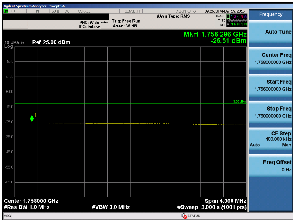
Plot 6-58. Upper Extended Band Edge Plot (Band 4 – 15.0MHz QPSK – RB Size 75)
