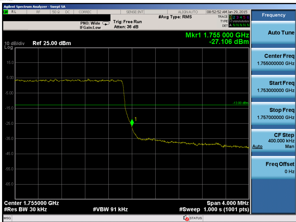
Plot 6-45. Upper Band Edge Plot (Band 4 – 3.0MHz QPSK – RB Size 15)
