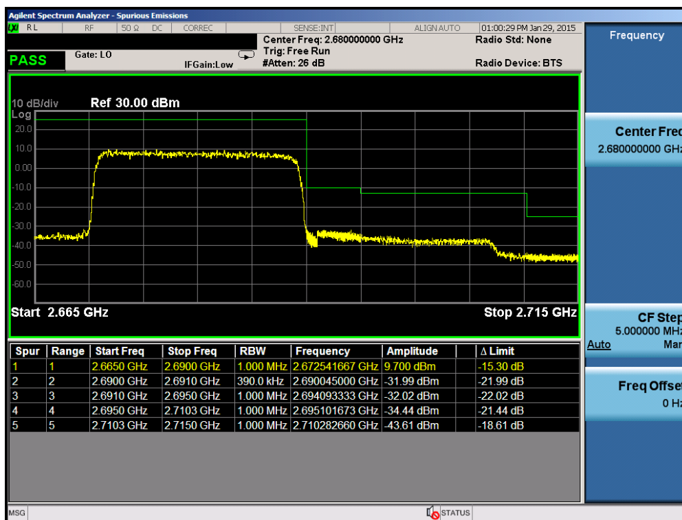
Plot 6-70. Upper Channel Edge Plot (Band 41 – 20.0MHz QPSK – RB Size 100)
