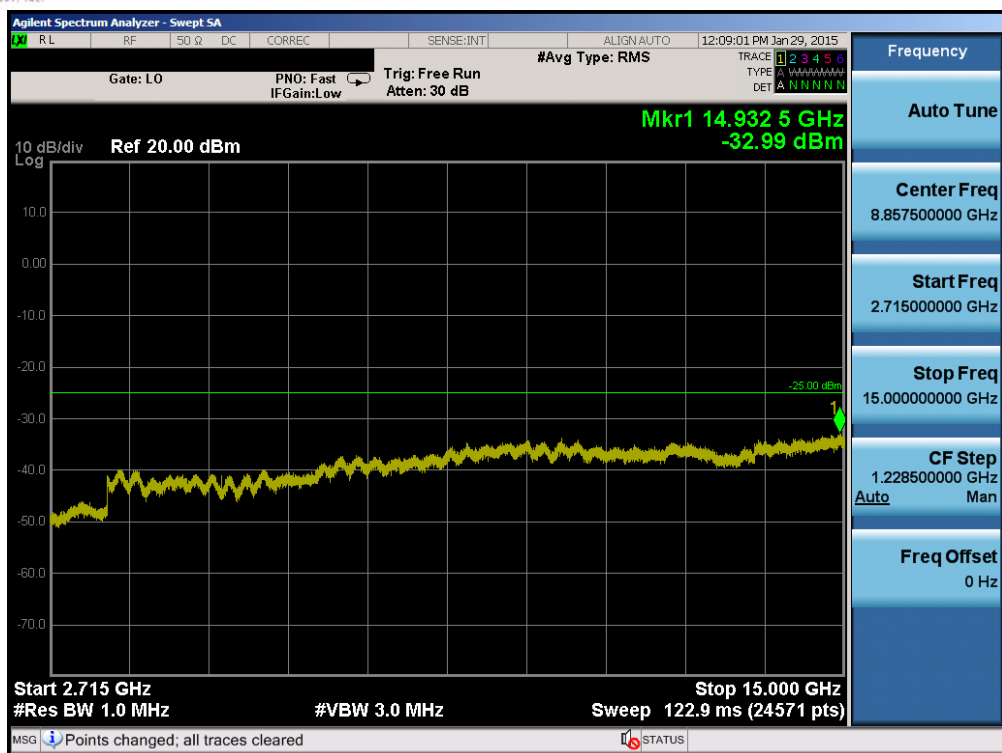
Plot 6-37. Conducted Spurious Plot (Band 41 – 10.0MHz QPSK – RB Size 1, RB Offset 0 – High Channel)
