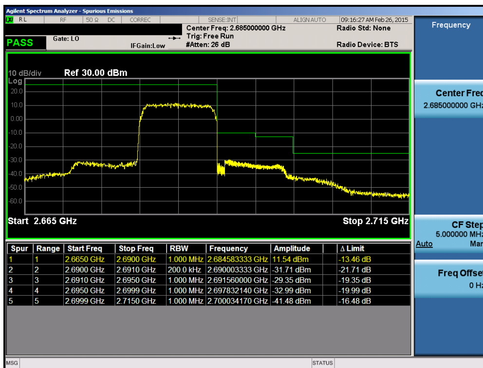
Plot 6-66. Upper Channel Edge Plot (Band 41 – 10.0MHz QPSK – RB Size 50)
