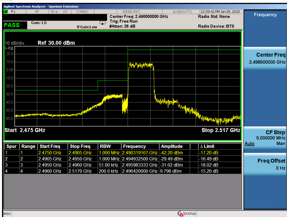
Plot 6-63. Lower Channel Edge Plot (Band 41 – 5.0MHz QPSK – RB Size 25)
