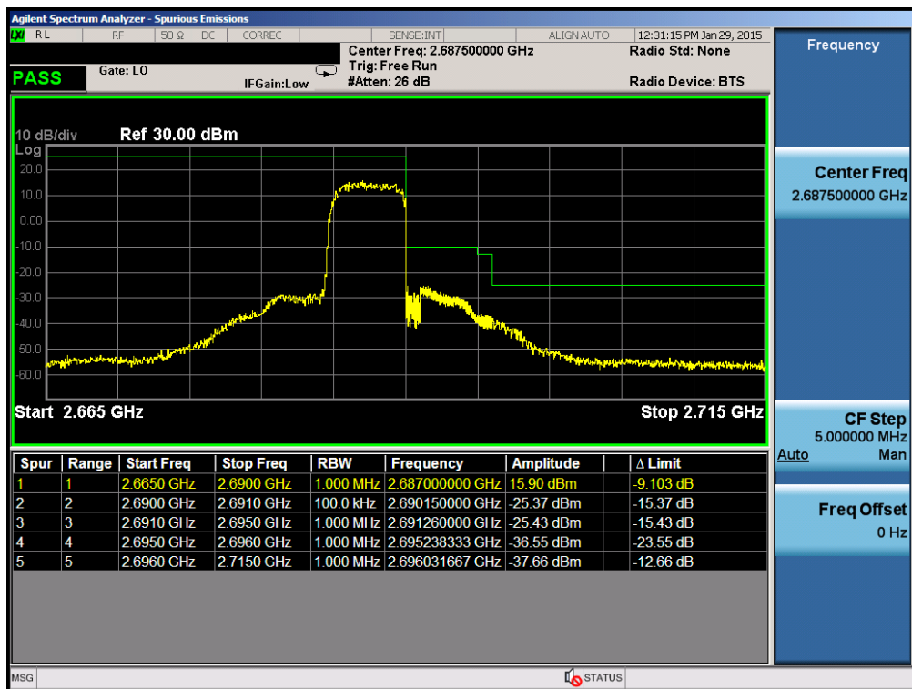
Plot 6-64. Upper Channel Edge Plot (Band 41 – 5.0MHz QPSK – RB Size 25)
