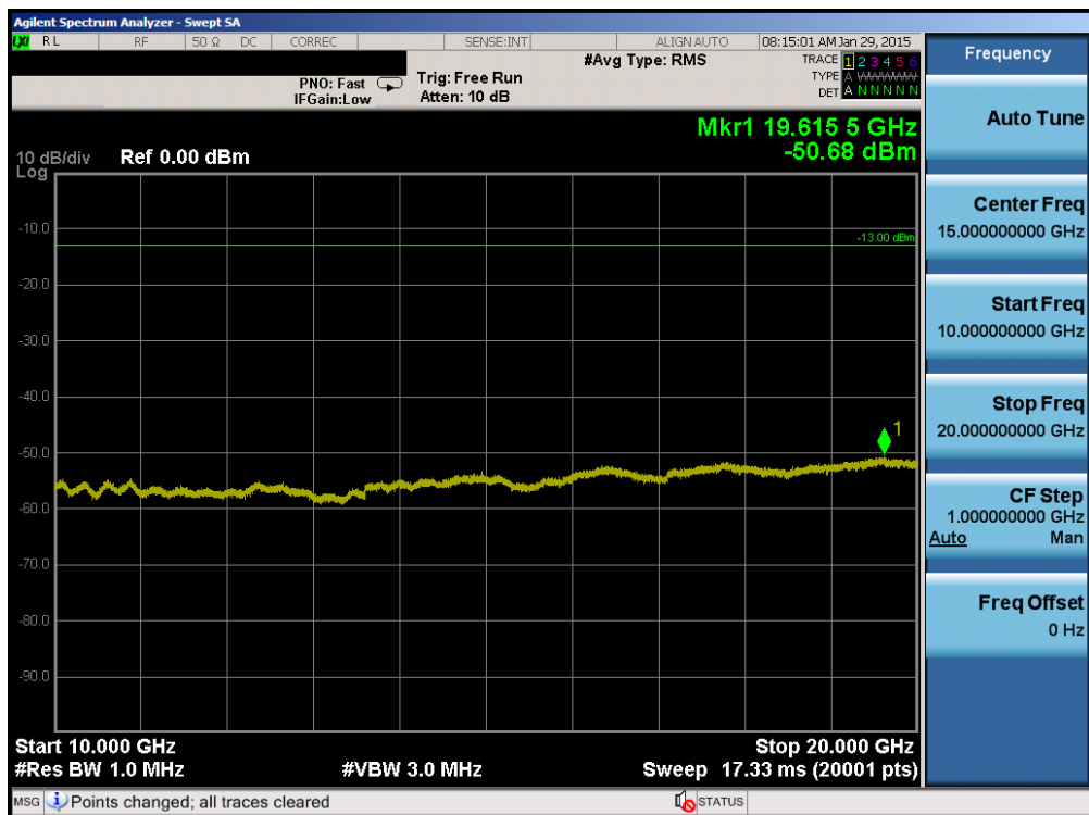
Plot 6-26. Conducted Spurious Plot (Band 4 – 5.0MHz QPSK – RB Size 1, RB Offset 0 – Mid Channel)
