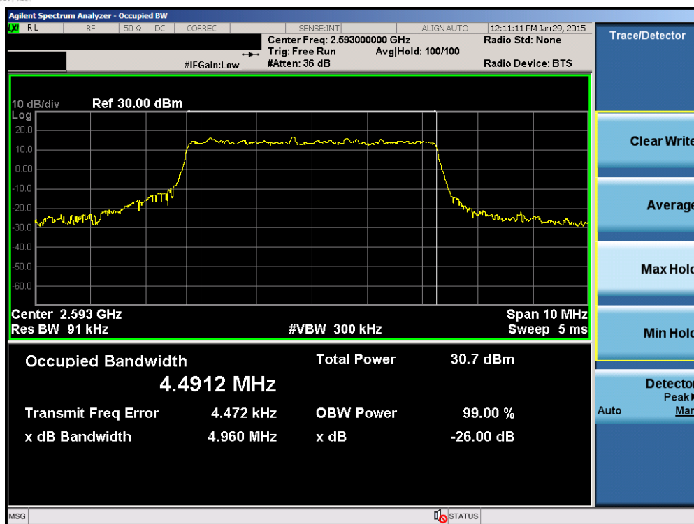
Plot 6-13. Occupied Bandwidth Plot (Band 41 – 5.0MHz QPSK – RB Size 25)
