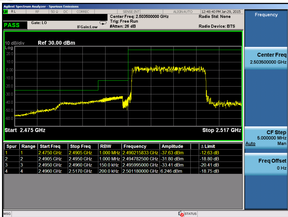
Plot 6-67. Lower Channel Edge Plot (Band 41 – 15.0MHz QPSK – RB Size 75)
