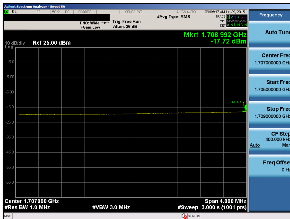
Plot 6-52. Lower Extended Band Edge Plot (Band 4 – 10.0MHz QPSK – RB Size 50)
