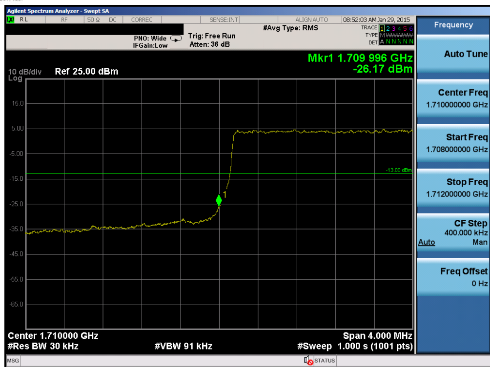
Plot 6-43. Lower Band Edge Plot (Band 4 – 3.0MHz QPSK – RB Size 15)
