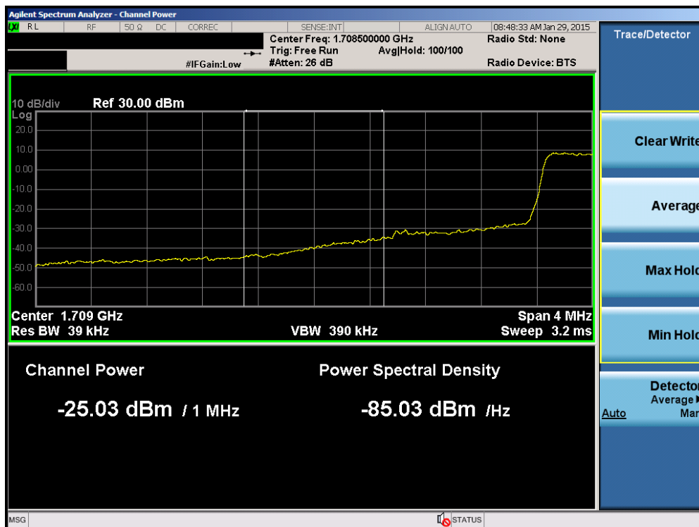
Plot 6-40. Lower Extended Band Edge Plot (Band 4 – 1.4MHz QPSK – RB Size 6)
