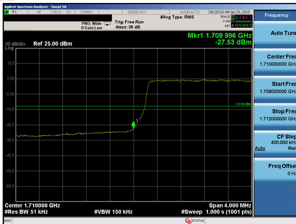
Plot 6-47. Lower Band Edge Plot (Band 4 – 5.0MHz QPSK – RB Size 25)
