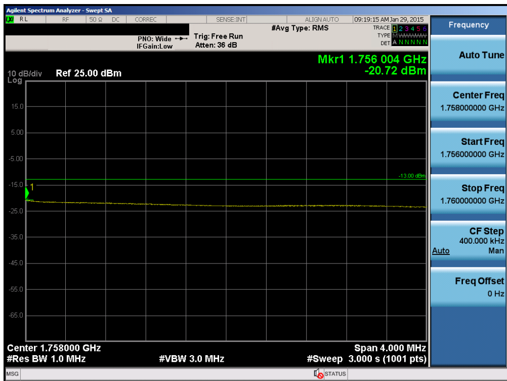
Plot 6-54. Upper Extended Band Edge Plot (Band 4 - 10.0MHz QPSK - RB Size 50)
