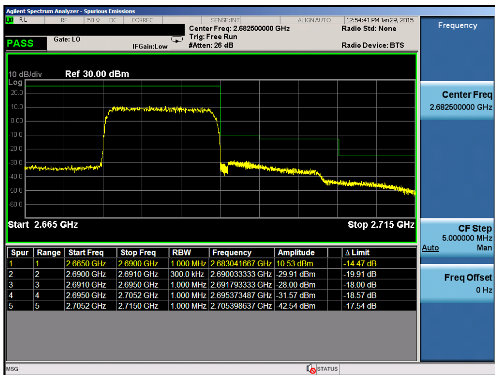
Plot 6-68. Upper Channel Edge Plot (Band 41 – 15.0MHz QPSK – RB Size 75)
