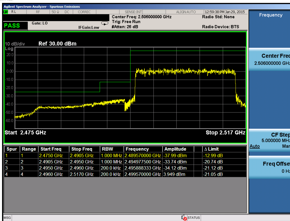
Plot 6-69. Lower Channel Edge Plot (Band 41 – 20.0MHz QPSK – RB Size 100)
