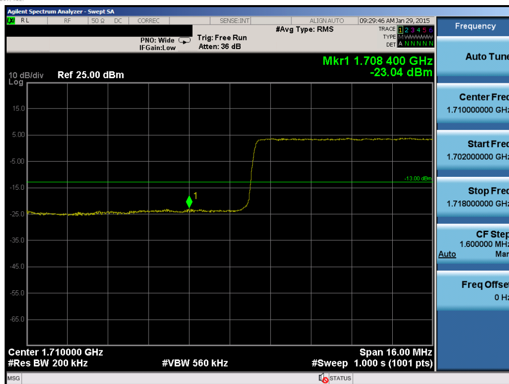
Plot 6-59. Lower Band Edge Plot (Band 4 - 20.0MHz QPSK - RB Size 100)
