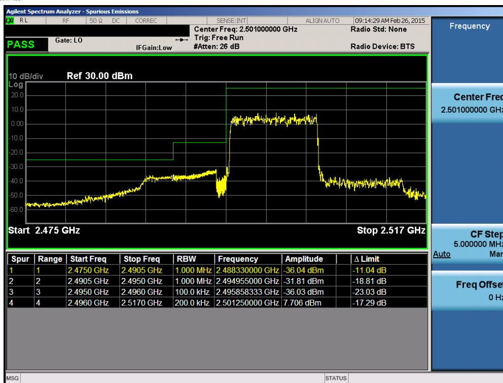
Plot 6-65. Lower Channel Edge Plot (Band 41 – 10.0MHz QPSK – RB Size 50)
