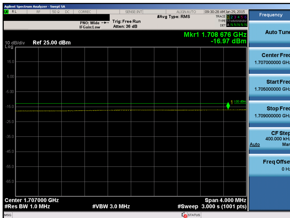
Plot 6-60. Lower Extended Band Edge Plot (Band 4 - 20.0MHz QPSK - RB Size 100)
