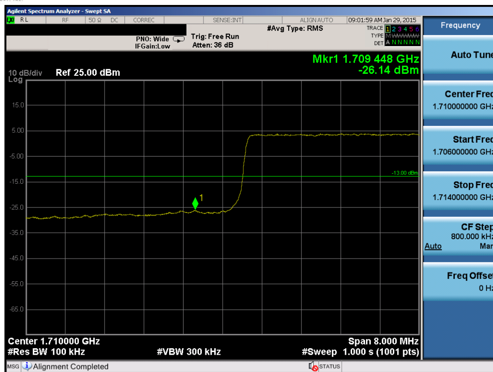
Plot 6-51. Lower Band Edge Plot (Band 4 – 10.0MHz QPSK – RB Size 50)
