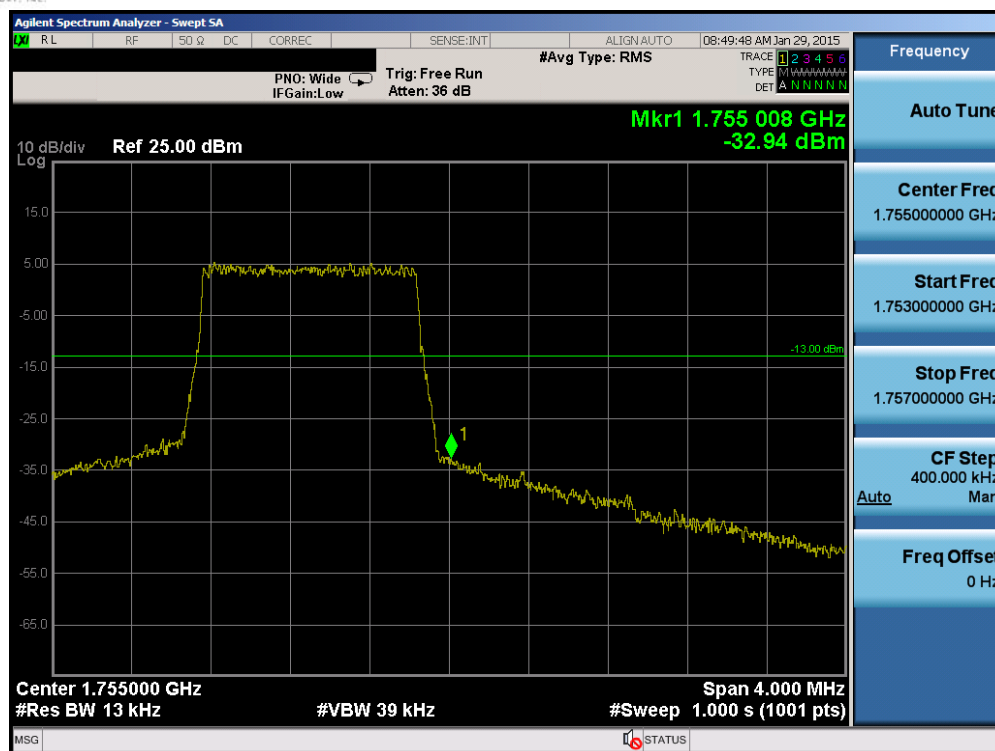
Plot 6-41. Upper Band Edge Plot (Band 4 – 1.4MHz QPSK – RB Size 6)
