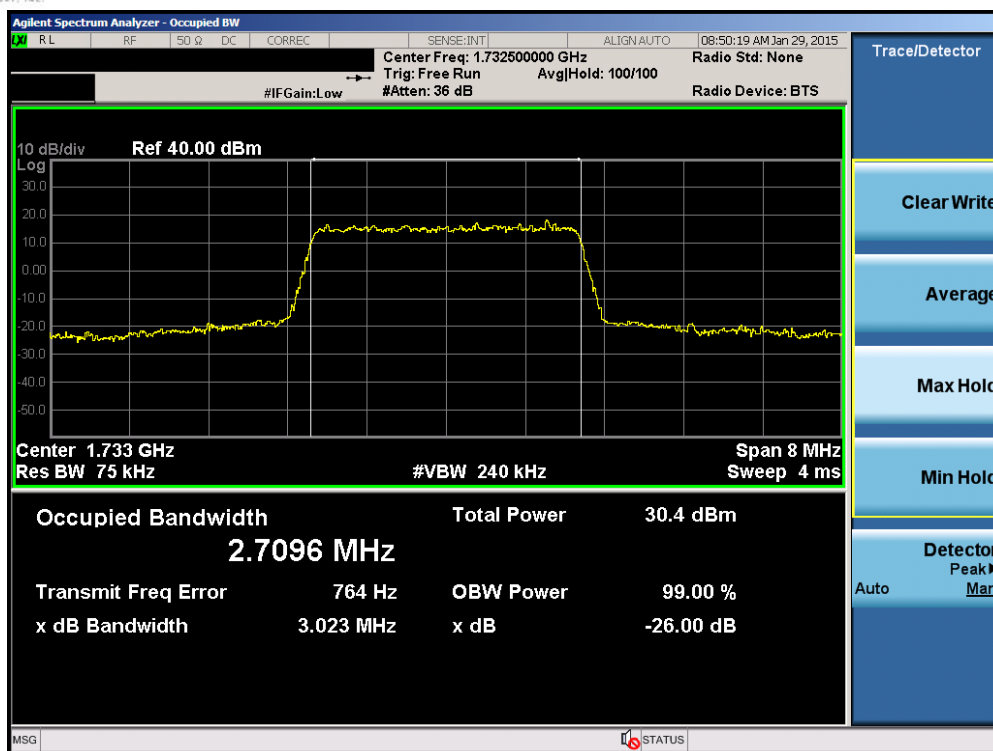
Plot 6-3. Occupied Bandwidth Plot (Band 4 – 3.0MHz QPSK – RB Size 15)
