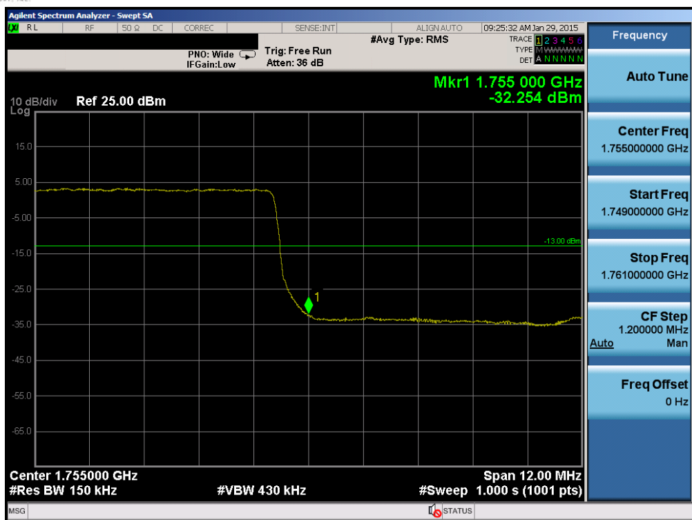
Plot 6-57. Upper Band Edge Plot (Band 4 – 15.0MHz QPSK – RB Size 75)
