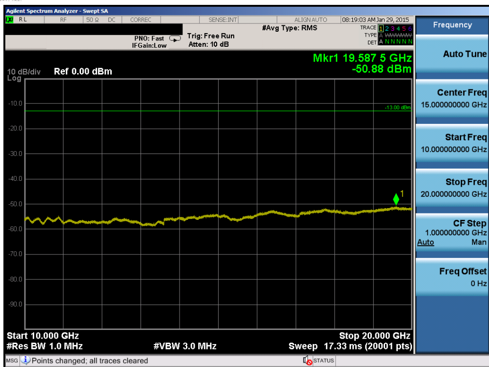
Plot 6-23. Conducted Spurious Plot (Band 4 – 5.0MHz QPSK – RB Size 1, RB Offset 0 – Low Channel)
