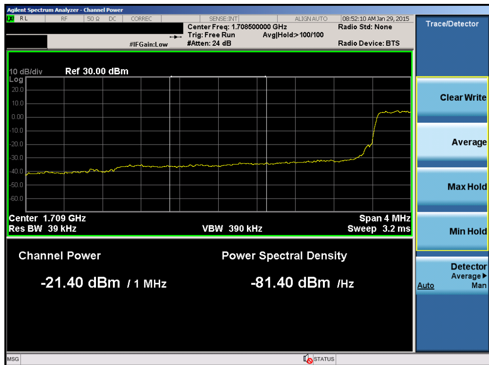
Plot 6-44. Lower Extended Band Edge Plot (Band 4 – 3.0MHz QPSK – RB Size 15)
