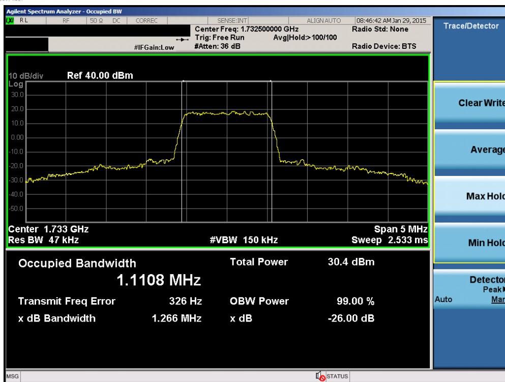
Plot 6-1. Occupied Bandwidth Plot (Band 4 – 1.4MHz QPSK – RB Size 6)
