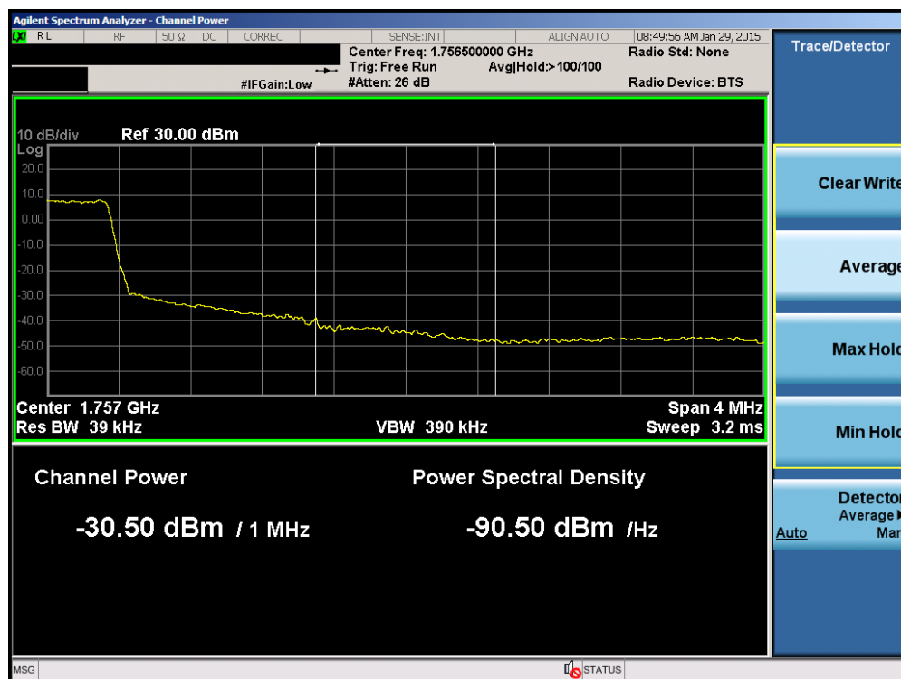
Plot 6-42. Upper Extended Band Edge Plot (Band 4 – 1.4MHz QPSK – RB Size 6)
