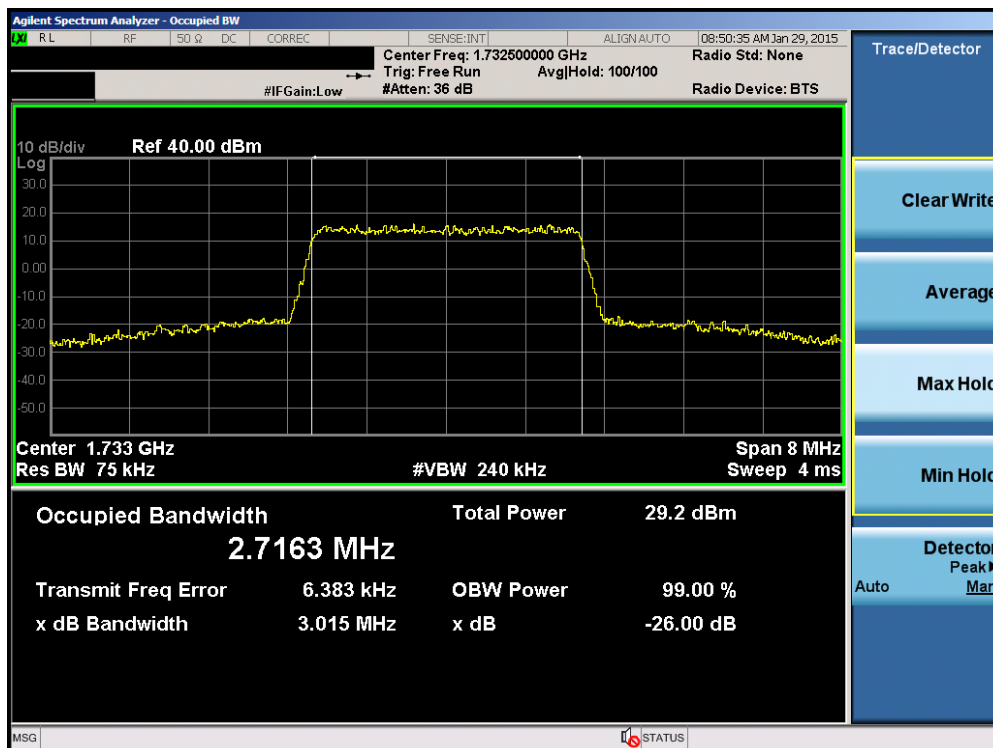
Plot 6-4. Occupied Bandwidth Plot (Band 4 – 3.0MHz 16-QAM – RB Size 15)
