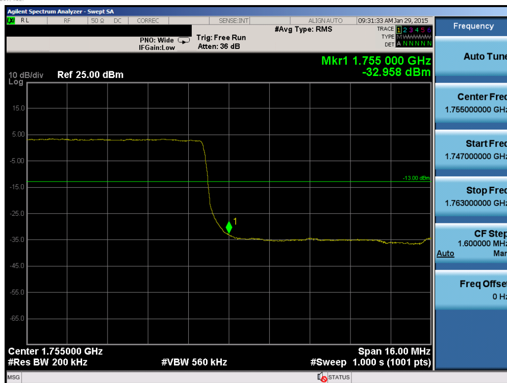
Plot 6-61. Upper Band Edge Plot (Band 4 – 20.0MHz QPSK – RB Size 100)
