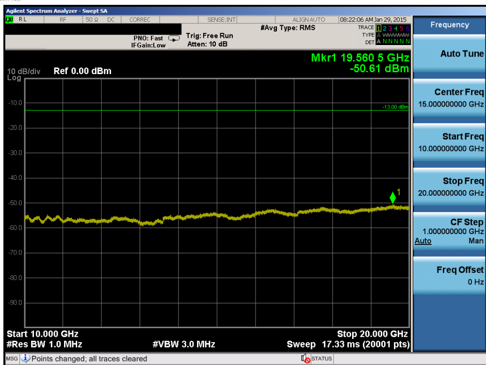
Plot 6-29. Conducted Spurious Plot (Band 4 – 5.0MHz QPSK – RB Size 1, RB Offset 0 – High Channel)
