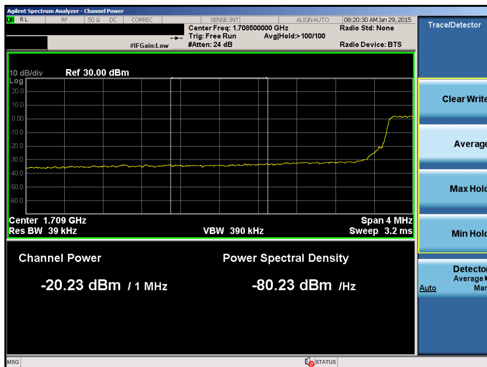
Plot 6-48. Lower Extended Band Edge Plot (Band 4 – 5.0MHz QPSK – RB Size 25)
