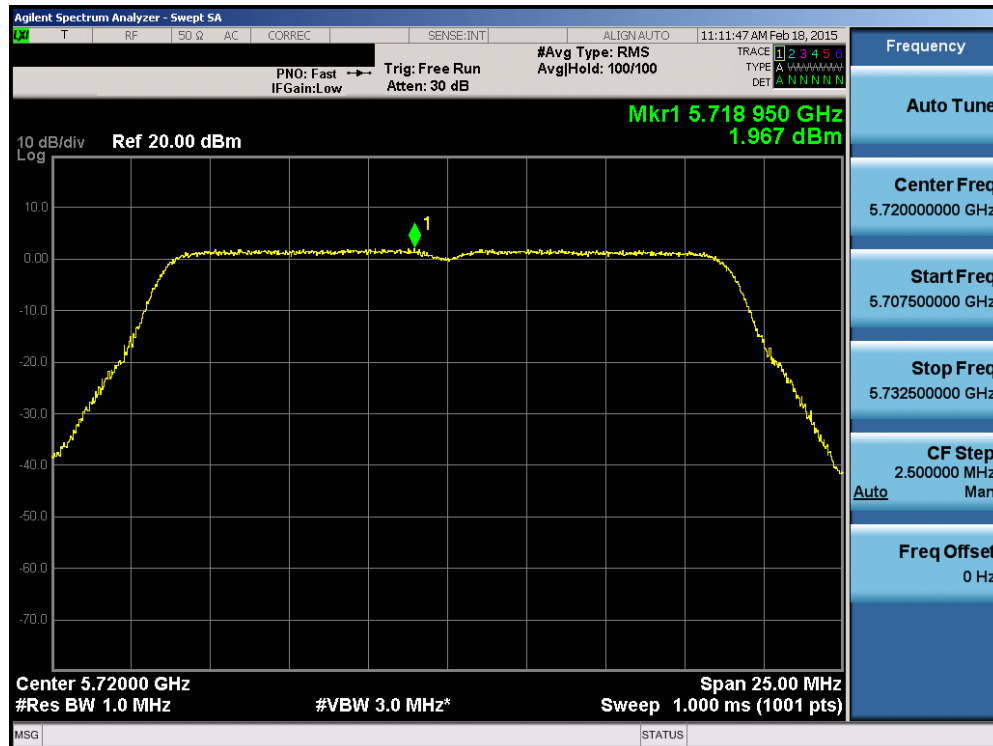
Plot 6-100. Power Spectral Density Plot (20MHz BW 802.11n (UNII Band Gap) – Ch. 144)
