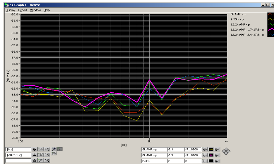
Figure 5-2 UMTS Audio Band Magnetic Noise
