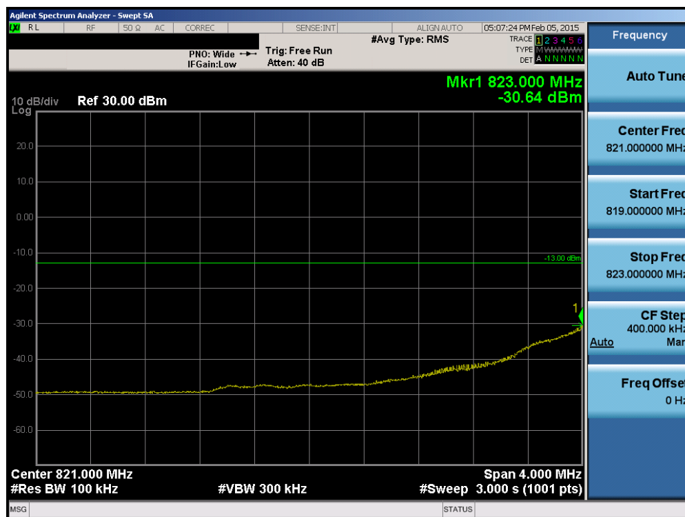
Plot 6-92. Lower Extended Band Edge Plot (Band 5 – 1.4MHz QPSK – RB Size 6)
