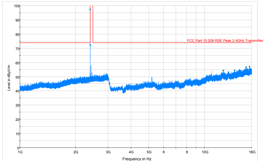
Plot 6-42. Radiated Spurious Plot above 1GHz (BT – Ch. 0, Ant. Pol. H)
