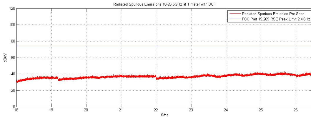
Plot 6-48. Radiated Spurious Plot above 18GHz (Pol. H)
