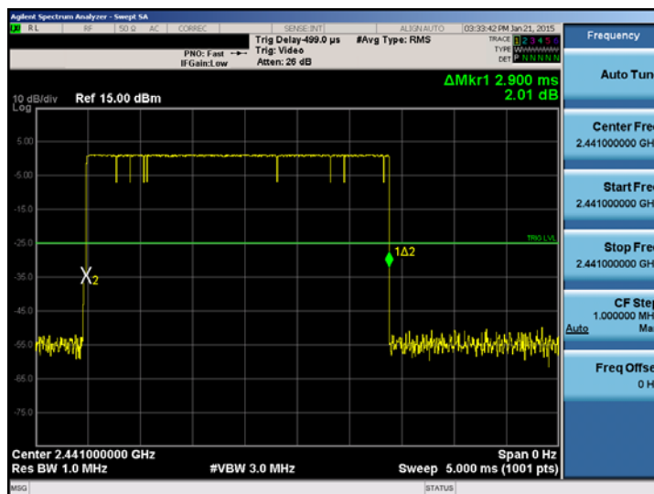
Plot 6-33. Time of Occupancy Plot (Bluetooth)
