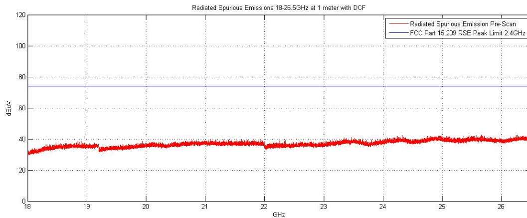
Plot 6-49. Radiated Spurious Plot above 18GHz (Pol. V)
