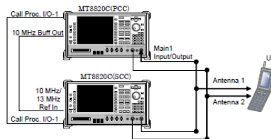
Figure 9-4 Power Measurement Setup
