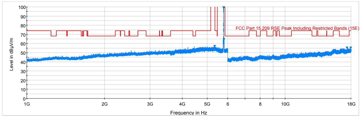
Plot 6-159. Radiated Spurious Plot above 1GHz (802.11a – U3, Ant. Pol. H)
