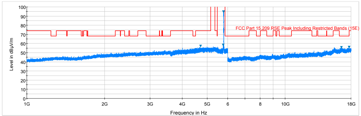
Plot 6-169. Radiated Spurious Plot above 1GHz (802.11a – U3, Ant. Pol. H)
