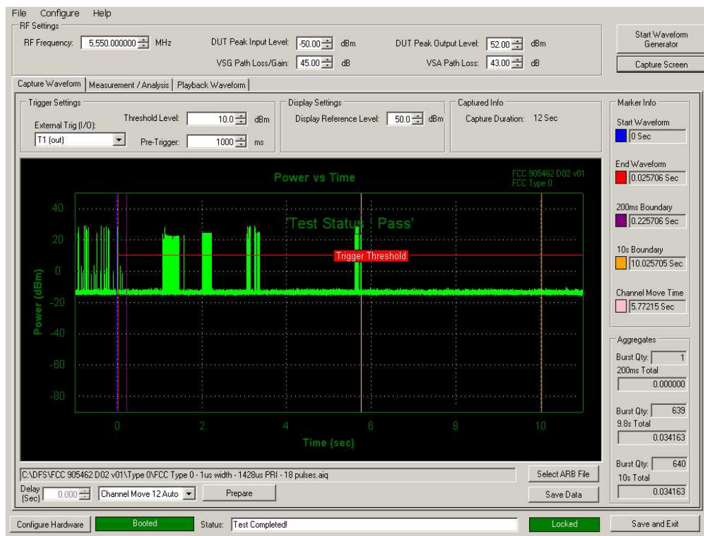
Figure 5-6. Band 2C Move Time and Aggregate Time
