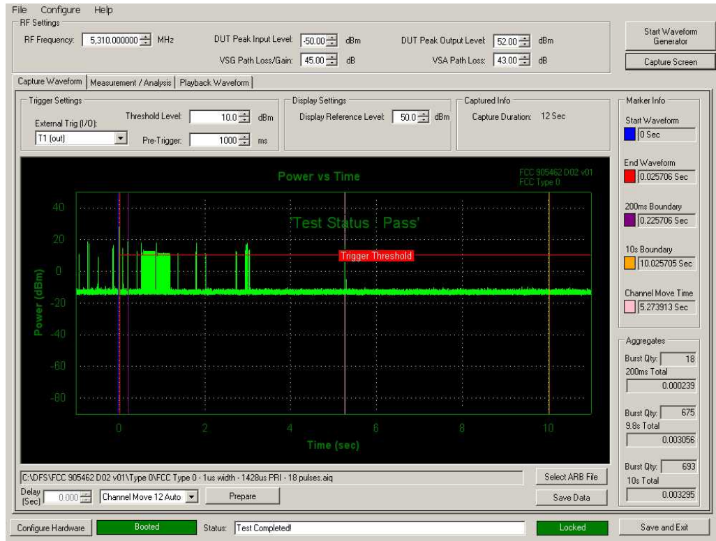
Figure 5-5. Band 2A Move Time and Aggregate Time
