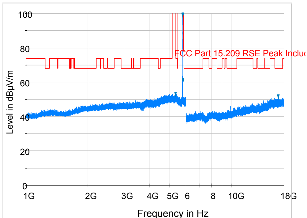
Plot 6-170. Radiated Spurious Plot above 1GHz (802.11a – U3 Ch. 157, Ant. Pol. V)
