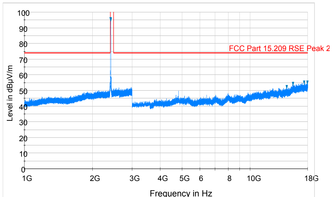
Plot 6-56. Radiated Spurious Plot above 1GHz (802.11b – Ch. 1, Ant. Pol. V)
