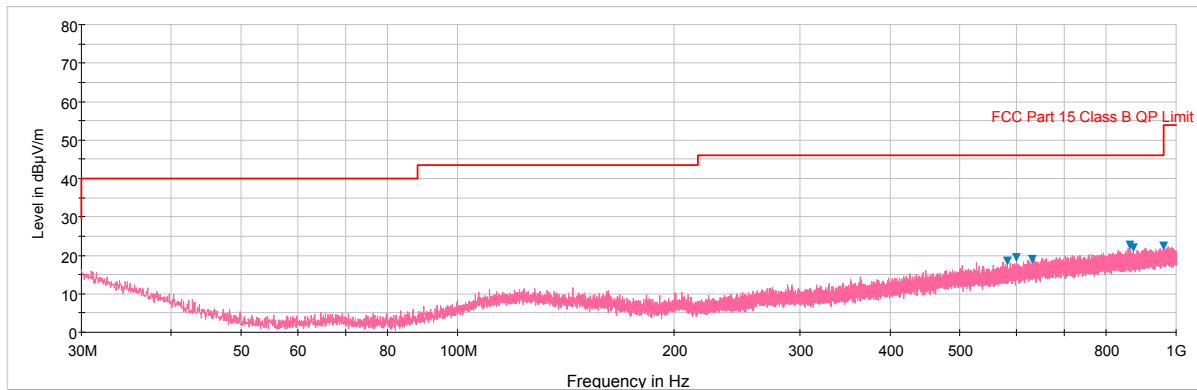
Plot 6-83. Radiated Spurious Plot below 1GHz (Pol. H)
