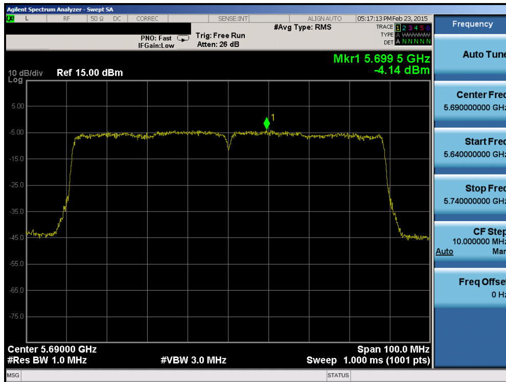
Plot 6-105. Power Spectral Density Plot (80MHz BW 802.11ac (UNII Band Gap) – Ch. 138)
