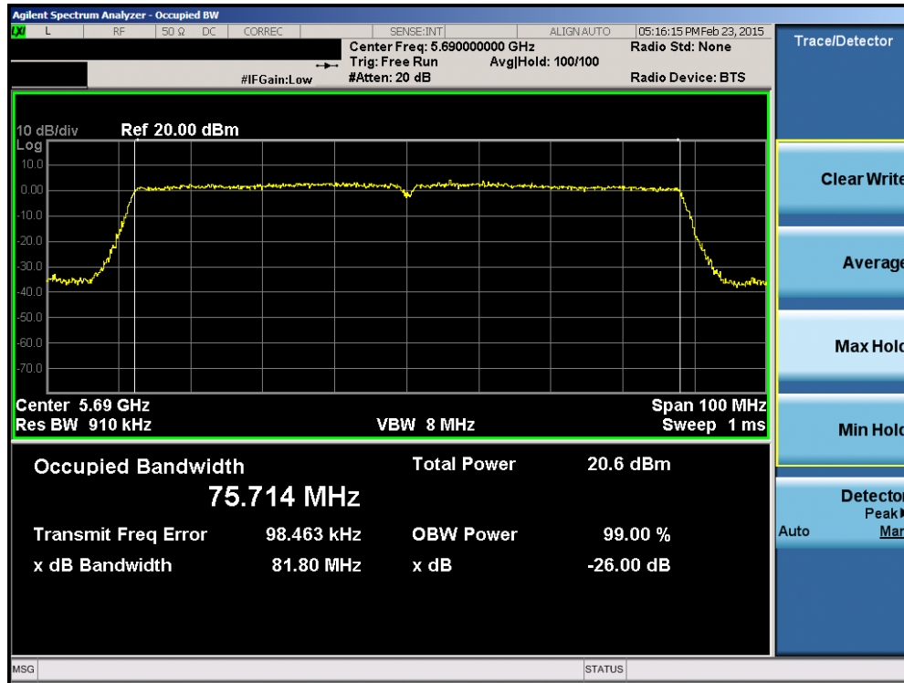
Plot 6-29. 26dB Bandwidth Plot (80MHz BW 802.11ac (UNII Band Gap) – Ch. 138)
