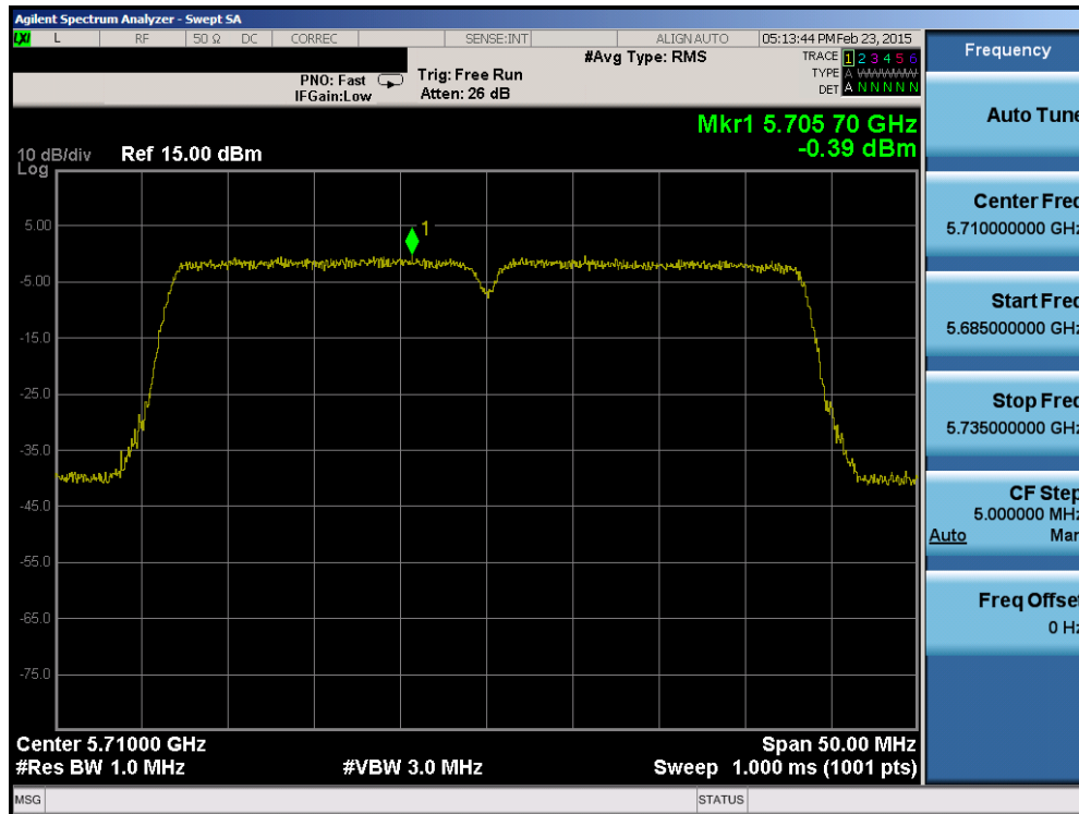
Plot 6-103. Power Spectral Density Plot (40MHz BW 802.11n (UNII Band Gap) – Ch. 142)
