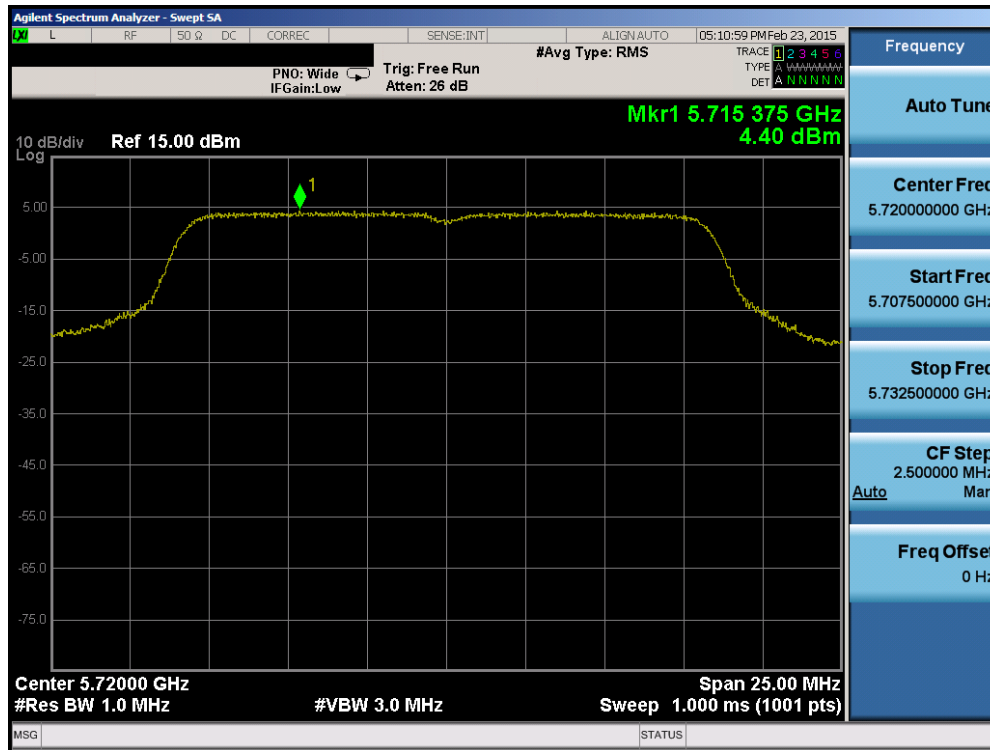
Plot 6-97. Power Spectral Density Plot (802.11a (UNII Band Gap) – Ch. 144)
