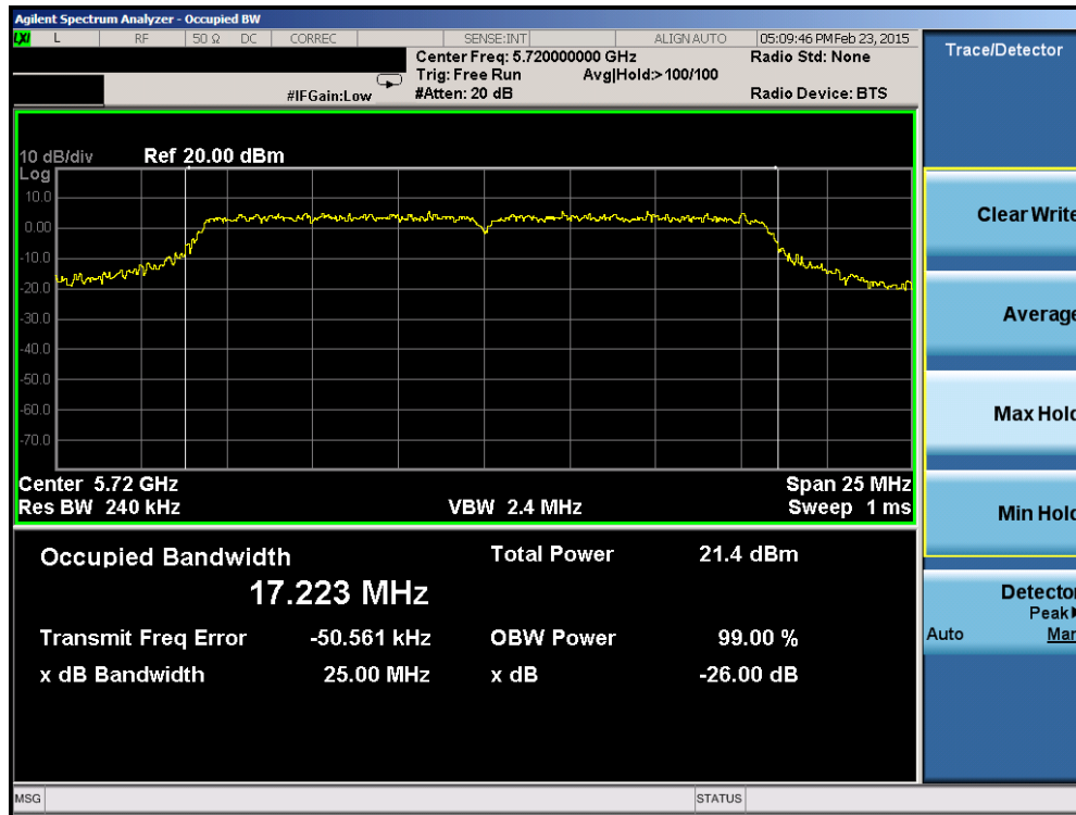
Plot 6-21. 26dB Bandwidth Plot (802.11a (UNII Band Gap) – Ch. 144)
