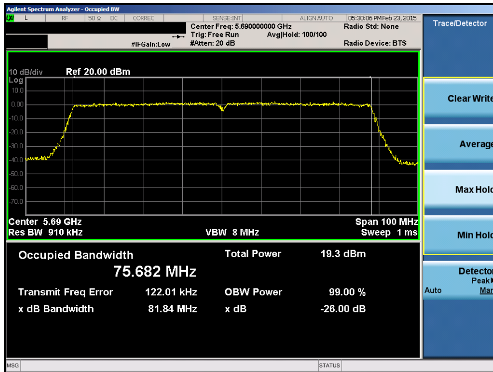
Plot 6-58. 26dB Bandwidth Plot (80MHz BW 802.11ac (UNII Band Gap) – Ch. 138)
