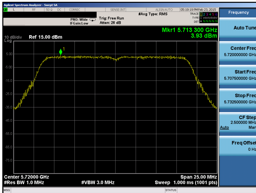
Plot 6-100. Power Spectral Density Plot (20MHz 802.11n (UNII Band Gap) – Ch. 144)
