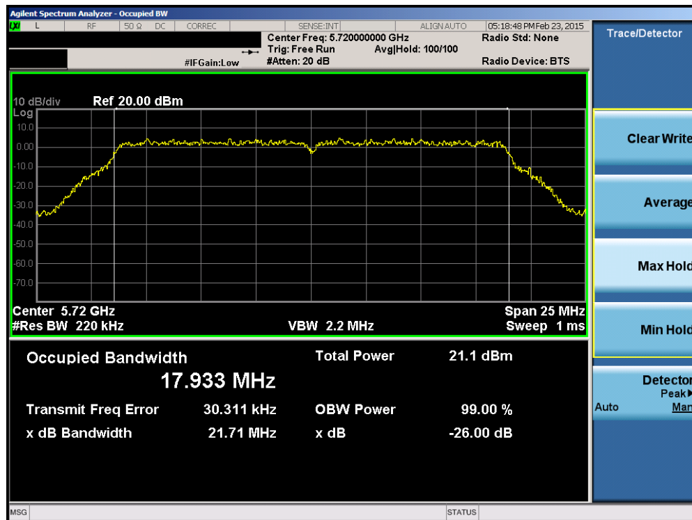
Plot 6-24. 26dB Bandwidth Plot (20MHz BW 802.11n (UNII Band Gap) – Ch. 144)
