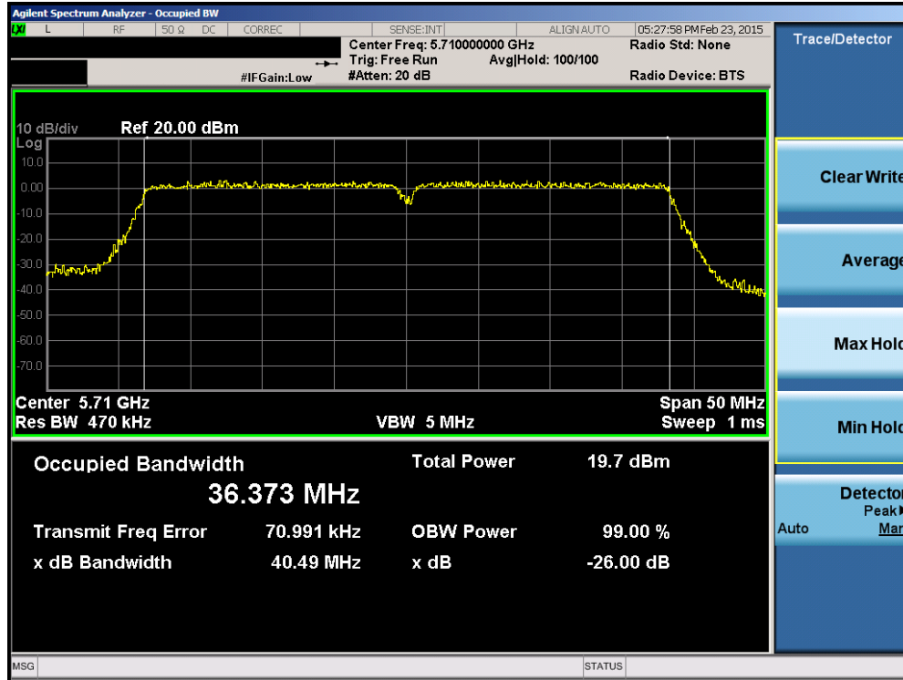
Plot 6-56. 26dB Bandwidth Plot (40MHz BW 802.11n (UNII Band Gap) – Ch. 142)
