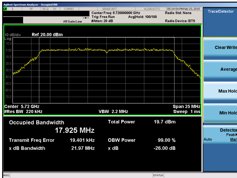
Plot 6-53. 26dB Bandwidth Plot (20MHz BW 802.11n (UNII Band Gap) – Ch. 144)
