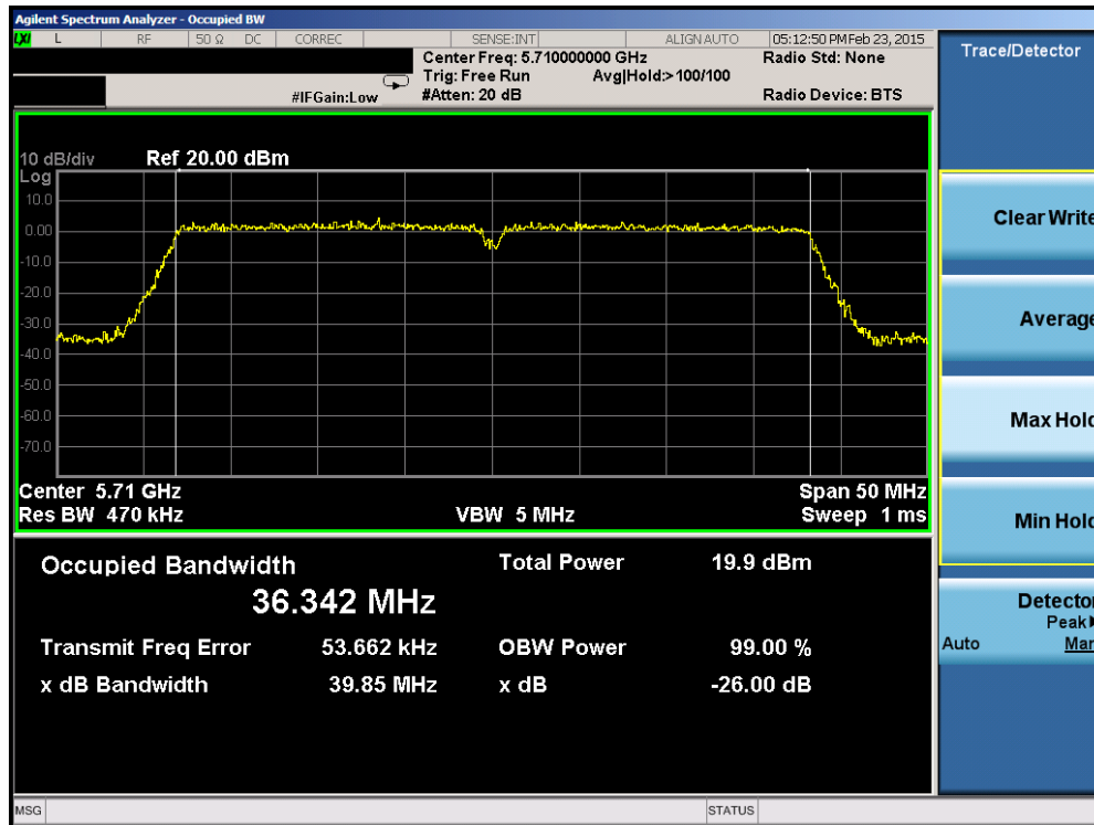
Plot 6-27. 26dB Bandwidth Plot (40MHz BW 802.11n (UNII Band Gap) – Ch. 142)
