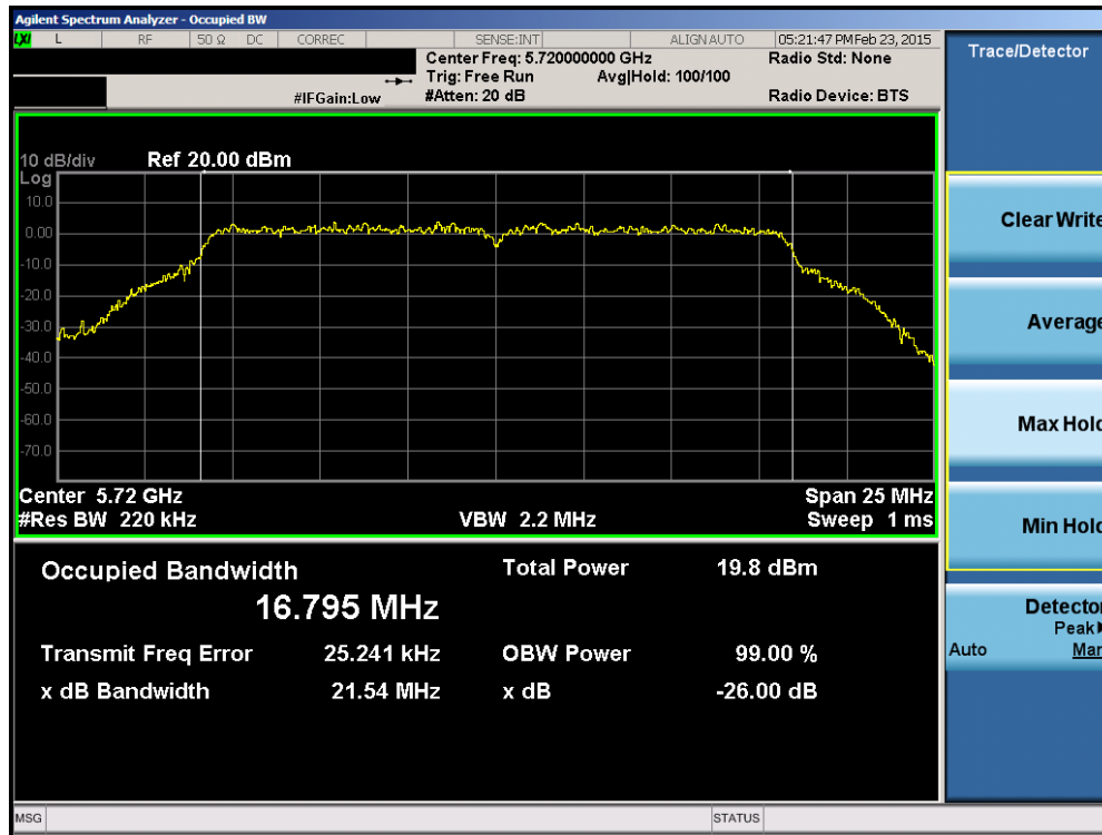
Plot 6-50. 26dB Bandwidth Plot (802.11a (UNII Band Gap) – Ch. 144)
