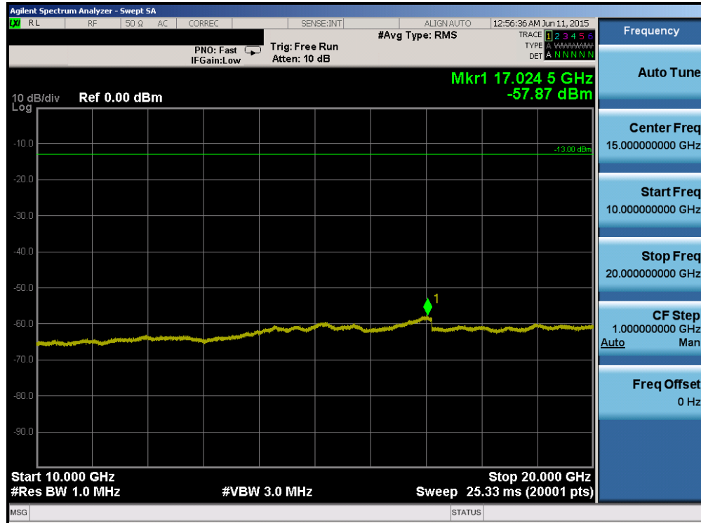
Plot 6-71. Conducted Spurious Plot (Band 4 – 10.0MHz QPSK – RB Size 1, RB Offset 0 – High Channel)
