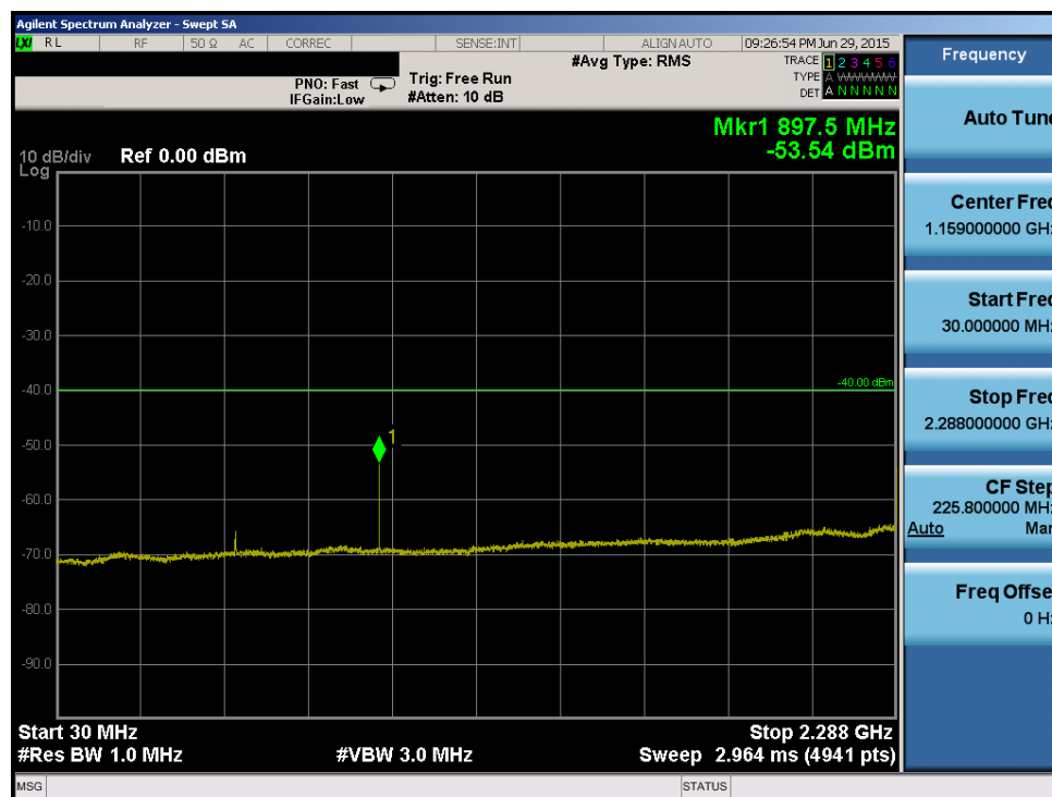
Plot 6-81. Conducted Spurious Plot (Band 30 – 10.0MHz QPSK – RB Size 1, RB Offset 0 – Mid Channel)
