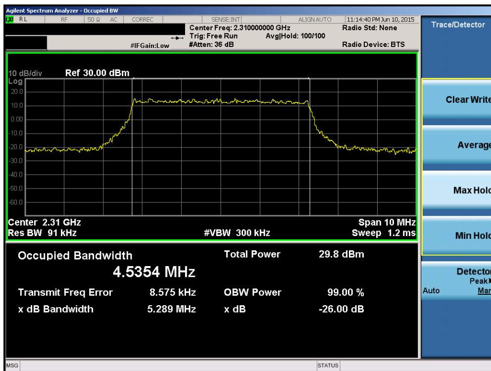
Plot 6-42. Occupied Bandwidth Plot (Band 30 – 5.0MHz 16-QAM – RB Size 25)
