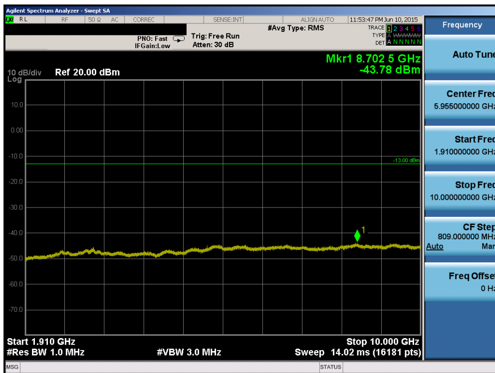
Plot 6-76. Conducted Spurious Plot (Band 2 – 10.0MHz QPSK – RB Size 1, RB Offset 0 – Mid Channel)
