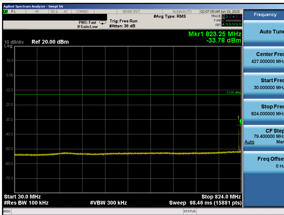
Plot 6-57. Conducted Spurious Plot (Band 5 – 10.0MHz QPSK – RB Size 1, RB Offset 0 – Mid Channel)
