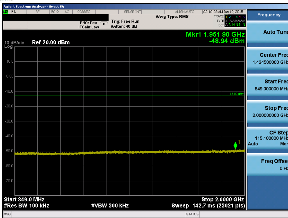
Plot 6-55. Conducted Spurious Plot (Band 5 – 10.0MHz QPSK – RB Size 1, RB Offset 0 – Low Channel)
