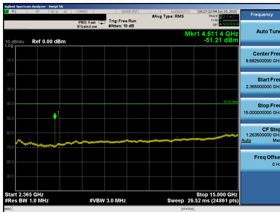
Plot 6-82. Conducted Spurious Plot (Band 30 – 10.0MHz QPSK – RB Size 1, RB Offset 0 – Mid Channel)
