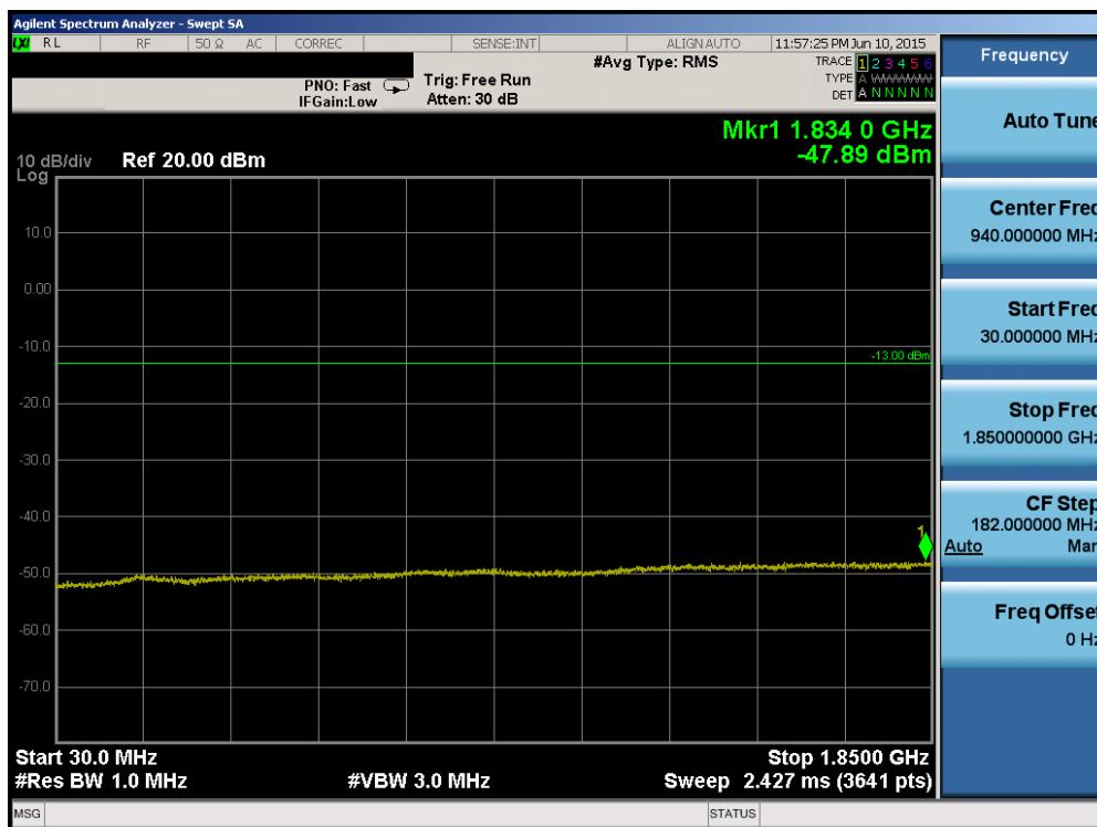
Plot 6-78. Conducted Spurious Plot (Band 2 – 10.0MHz QPSK – RB Size 1, RB Offset 0 – High Channel)
