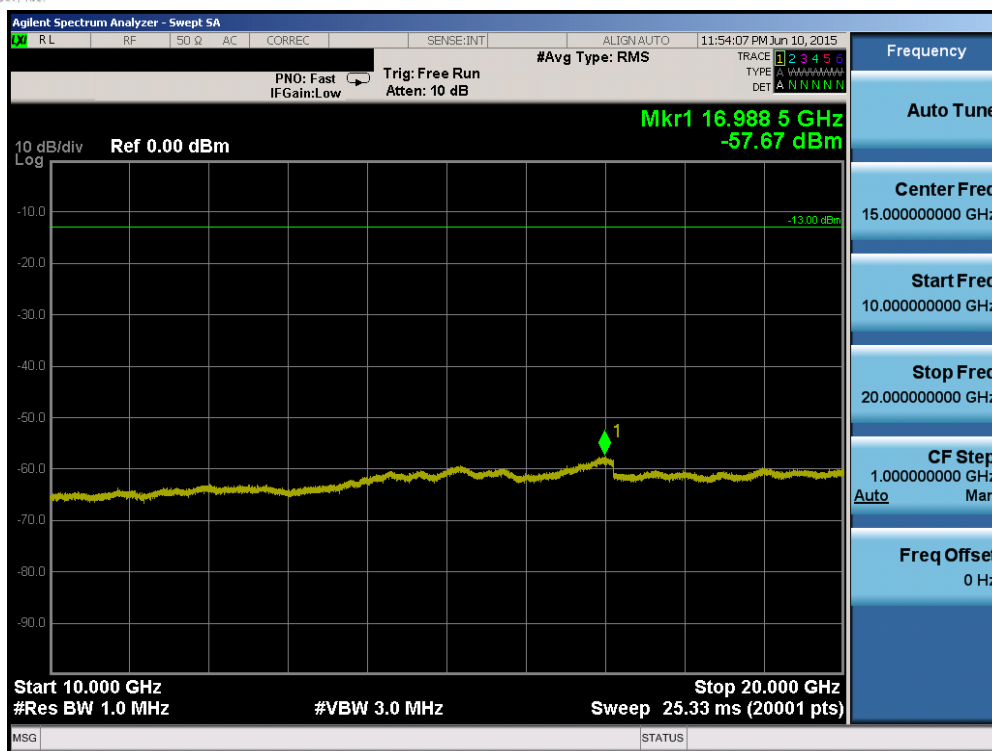
Plot 6-77. Conducted Spurious Plot (Band 2 – 10.0MHz QPSK – RB Size 1, RB Offset 0 – Mid Channel)
