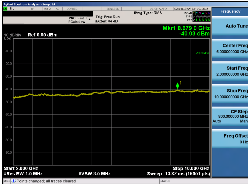
Plot 6-62. Conducted Spurious Plot (Band 5 – 10.0MHz QPSK – RB Size 1, RB Offset 0 – High Channel)
