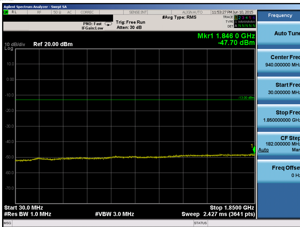
Plot 6-75. Conducted Spurious Plot (Band 2 – 10.0MHz QPSK – RB Size 1, RB Offset 0 – Mid Channel)
