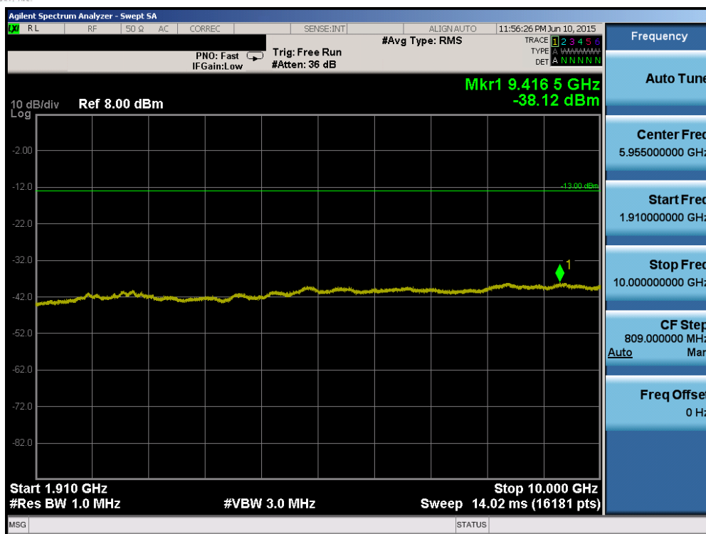
Plot 6-73. Conducted Spurious Plot (Band 2 – 10.0MHz QPSK – RB Size 1, RB Offset 0 – Low Channel)
