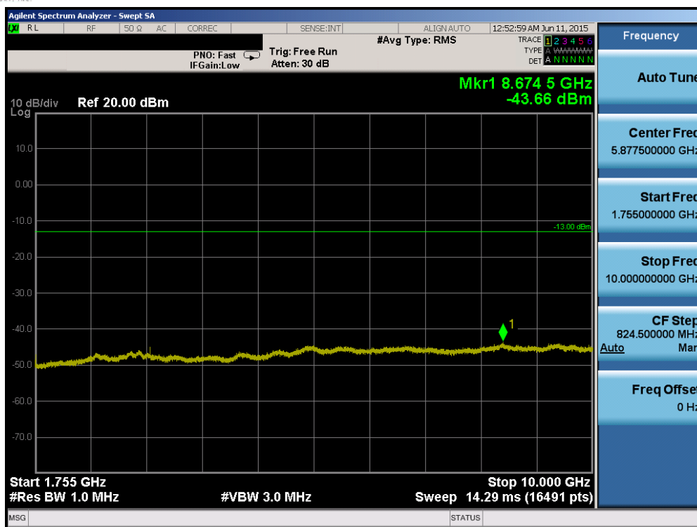
Plot 6-67. Conducted Spurious Plot (Band 4 – 10.0MHz QPSK – RB Size 1, RB Offset 0 – Mid Channel)
