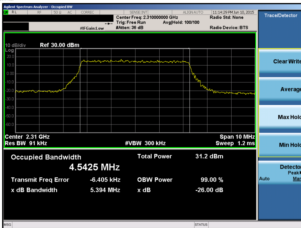
Plot 6-41. Occupied Bandwidth Plot (Band 30 – 5.0MHz QPSK – RB Size 25)
