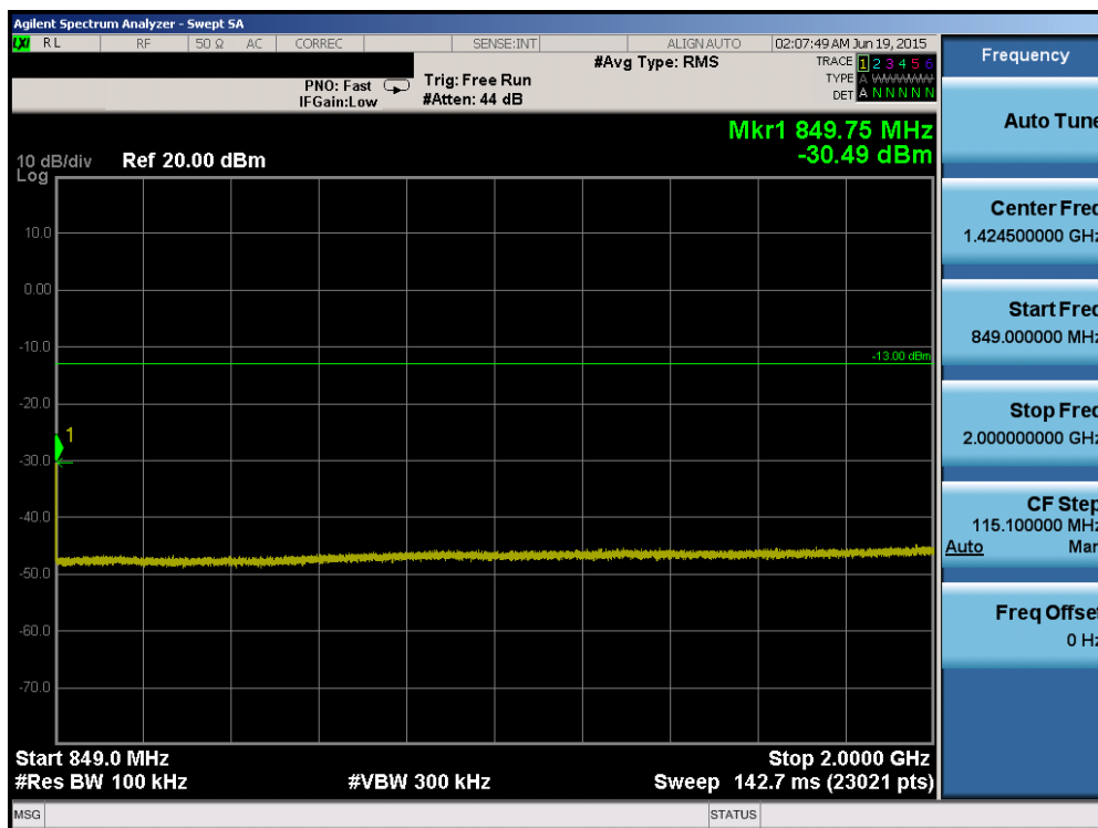
Plot 6-58. Conducted Spurious Plot (Band 5 – 10.0MHz QPSK – RB Size 1, RB Offset 0 – Mid Channel)
