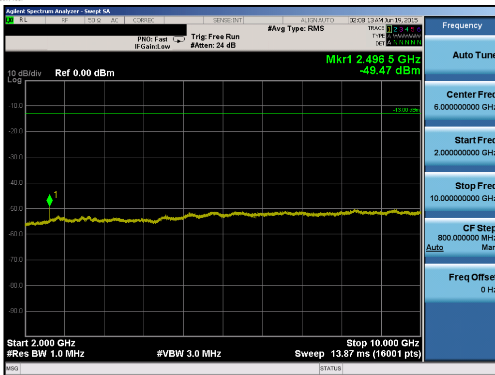
Plot 6-59. Conducted Spurious Plot (Band 5 – 10.0MHz QPSK – RB Size 1, RB Offset 0 – Mid Channel)
