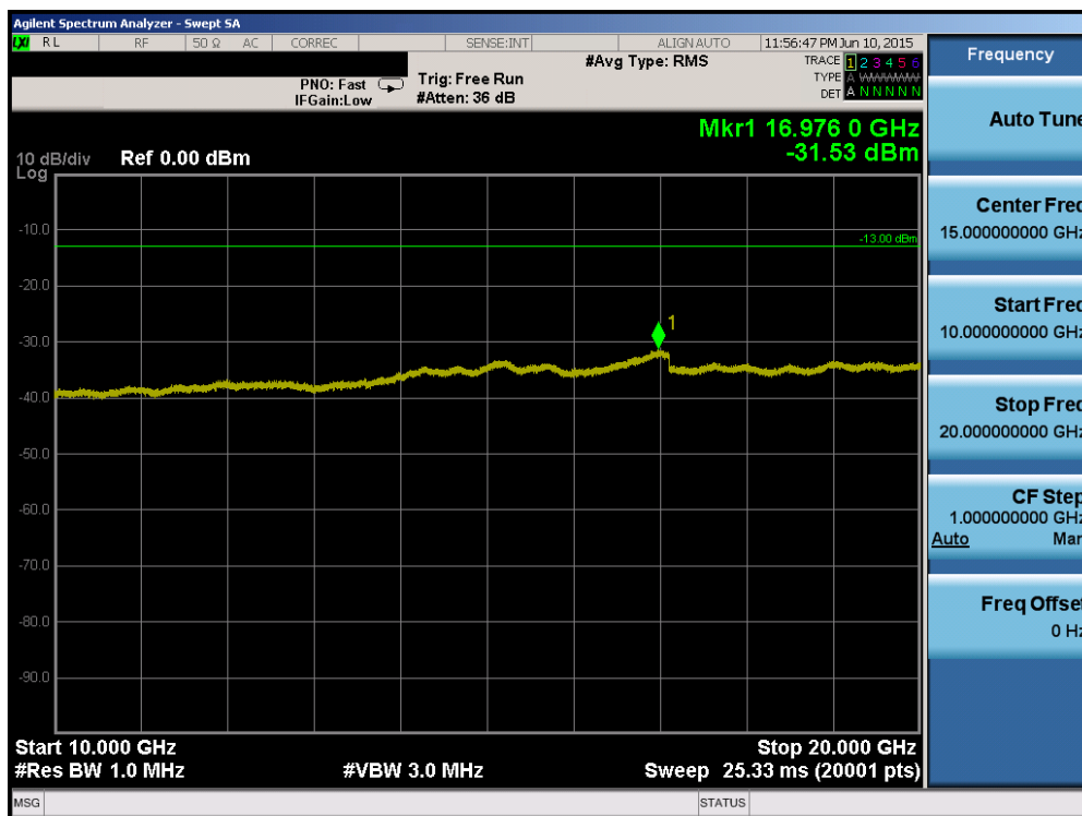
Plot 6-74. Conducted Spurious Plot (Band 2 – 10.0MHz QPSK – RB Size 1, RB Offset 0 – Low Channel)
