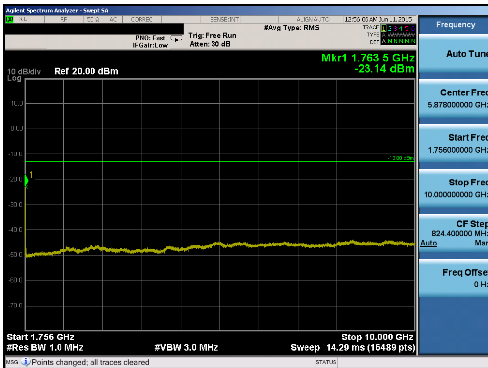
Plot 6-70. Conducted Spurious Plot (Band 4 – 10.0MHz QPSK – RB Size 1, RB Offset 0 – High Channel)
