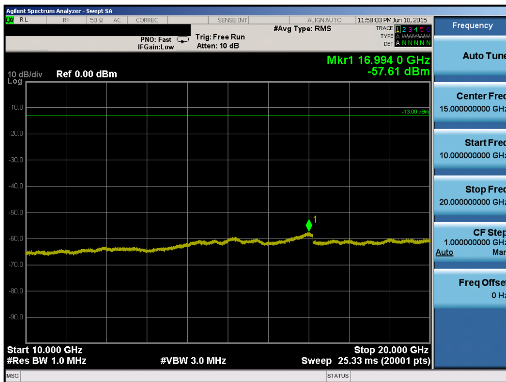
Plot 6-80. Conducted Spurious Plot (Band 2 – 10.0MHz QPSK – RB Size 1, RB Offset 0 – High Channel)
