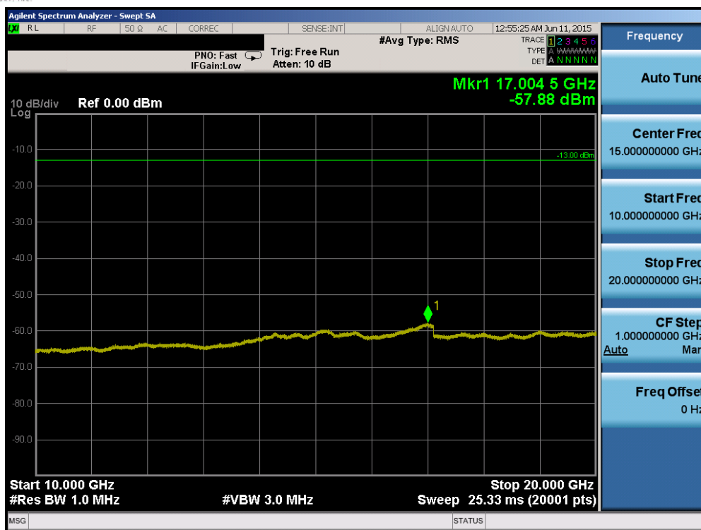
Plot 6-65. Conducted Spurious Plot (Band 4 – 10.0MHz QPSK – RB Size 1, RB Offset 0 – Low Channel)
