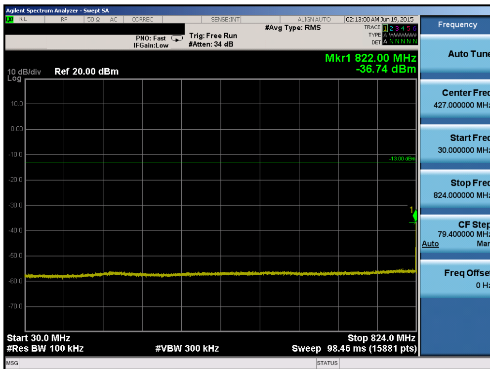
Plot 6-60. Conducted Spurious Plot (Band 5 – 10.0MHz QPSK – RB Size 1, RB Offset 0 – High Channel)
