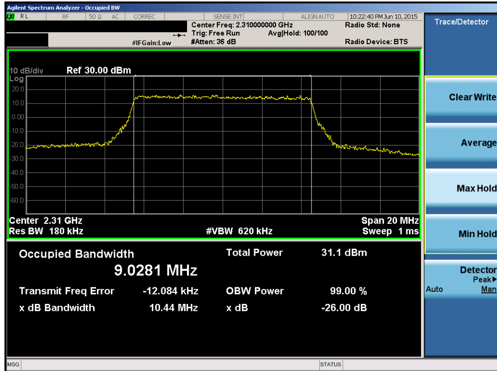
Plot 6-43. Occupied Bandwidth Plot (Band 30 – 10.0MHz QPSK – RB Size 50)
