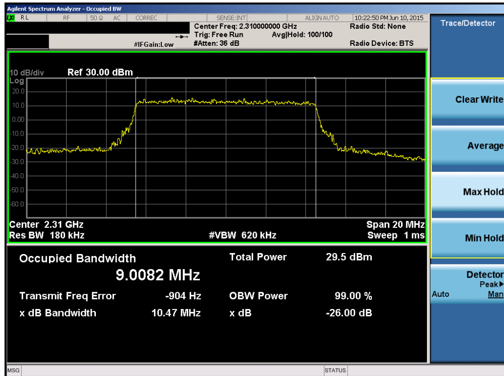
Plot 6-44. Occupied Bandwidth Plot (Band 30 – 10.0MHz 16-QAM – RB Size 50)
