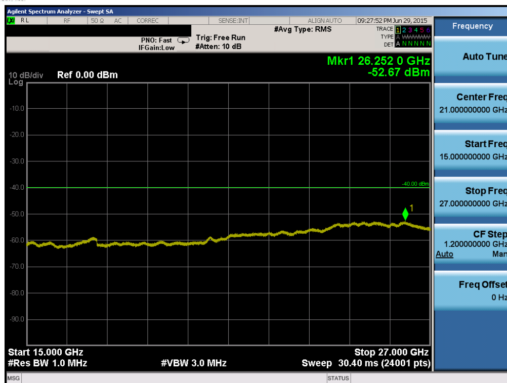
Plot 6-83. Conducted Spurious Plot (Band 30 – 10.0MHz QPSK – RB Size 1, RB Offset 0 – Mid Channel)
