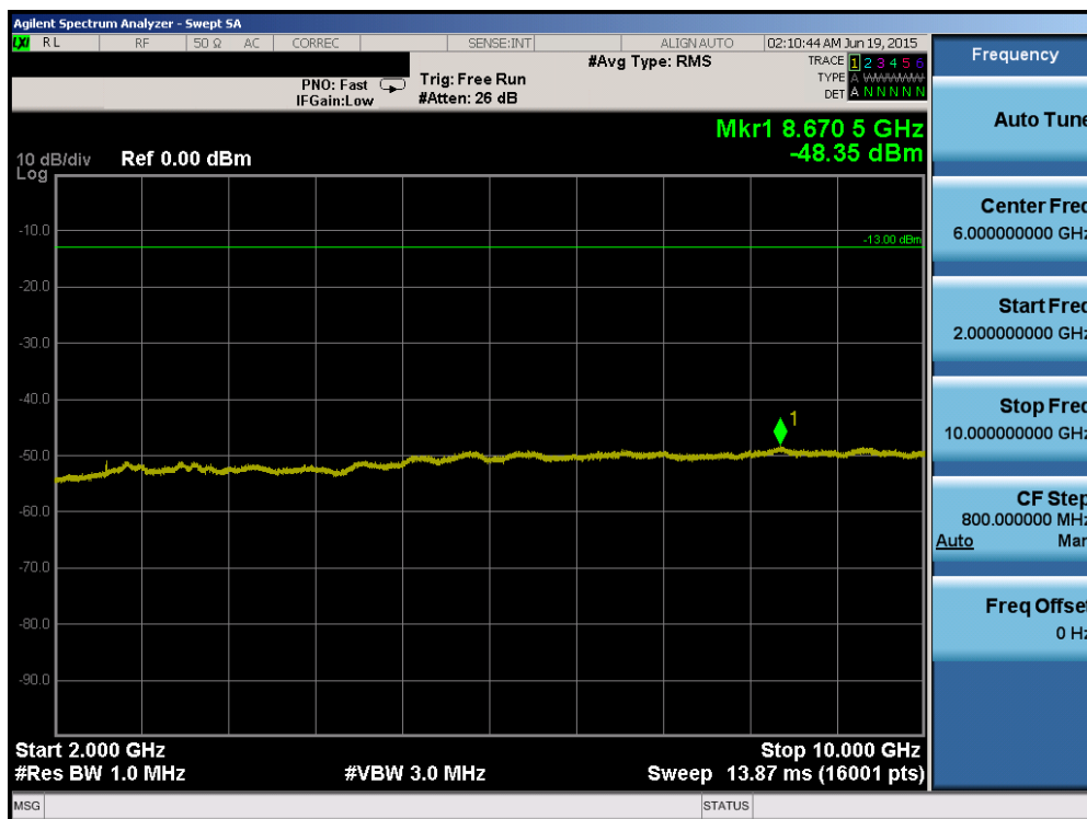
Plot 6-56. Conducted Spurious Plot (Band 5 – 10.0MHz QPSK – RB Size 1, RB Offset 0 – Low Channel)
