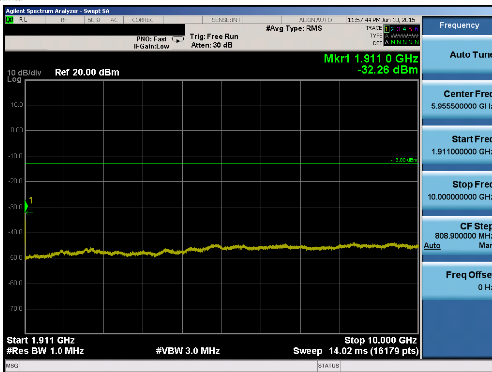
Plot 6-79. Conducted Spurious Plot (Band 2 – 10.0MHz QPSK – RB Size 1, RB Offset 0 – High Channel)
