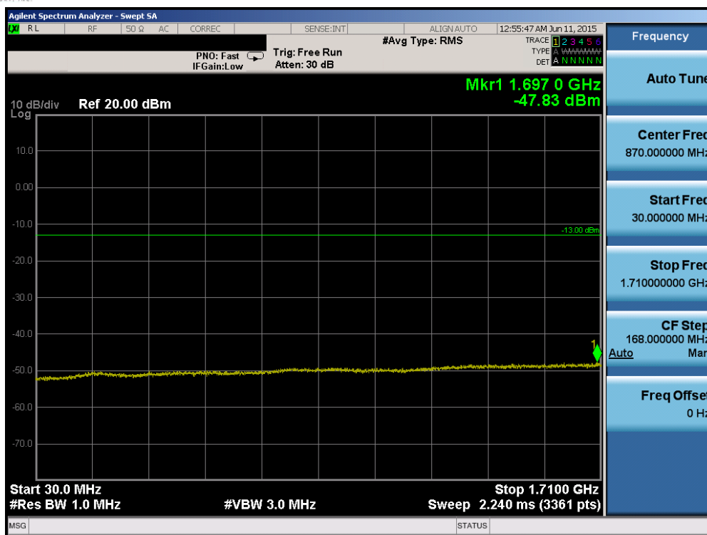
Plot 6-69. Conducted Spurious Plot (Band 4 – 10.0MHz QPSK – RB Size 1, RB Offset 0 – High Channel)
