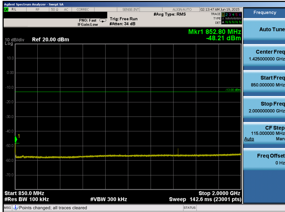
Plot 6-61. Conducted Spurious Plot (Band 5 – 10.0MHz QPSK – RB Size 1, RB Offset 0 – High Channel)
