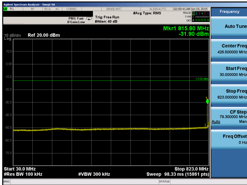
Plot 6-54. Conducted Spurious Plot (Band 5 – 10.0MHz QPSK – RB Size 1, RB Offset 0– Low Channel)
