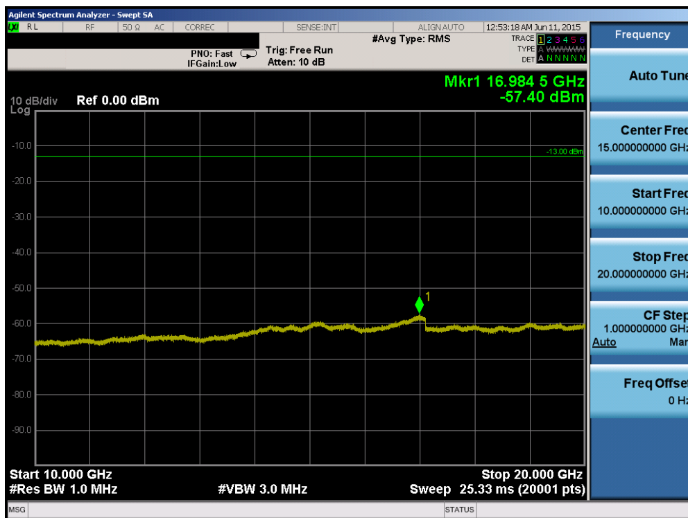
Plot 6-68. Conducted Spurious Plot (Band 4 – 10.0MHz QPSK – RB Size 1, RB Offset 0 – Mid Channel)
