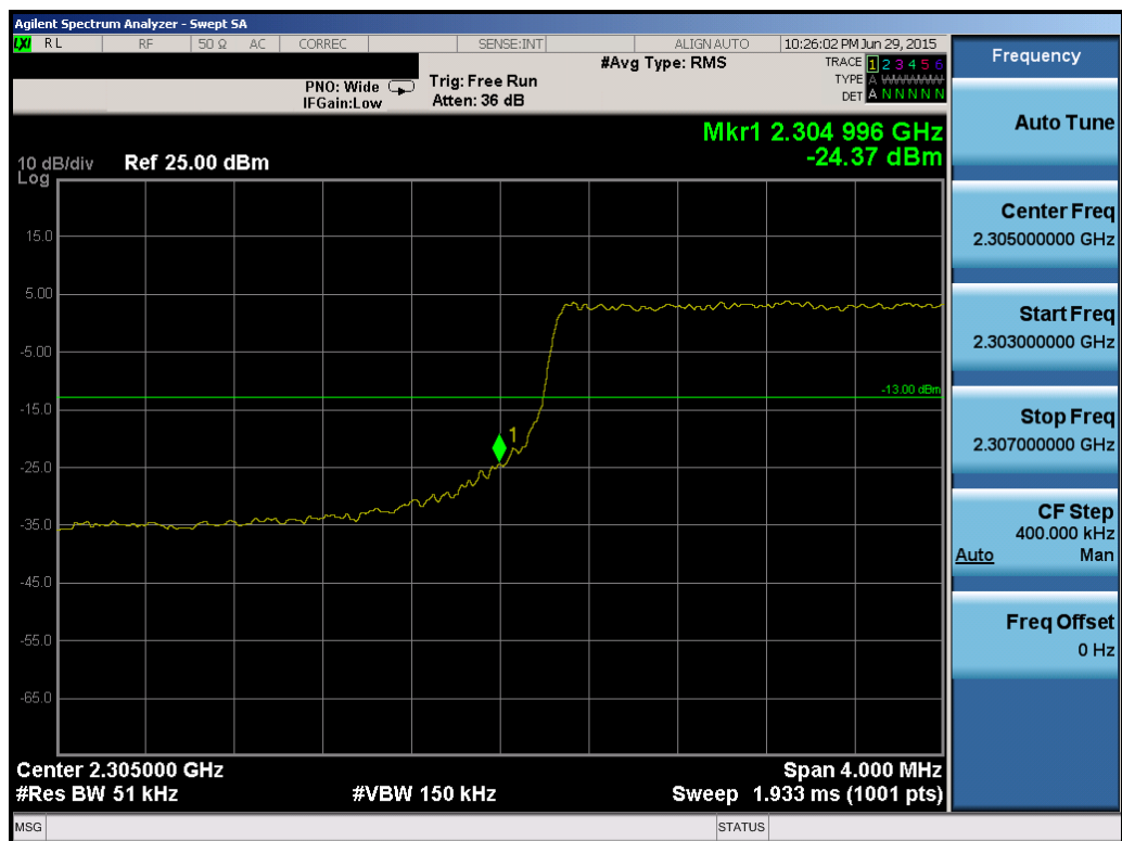
Plot 6-160. Lower Band Edge Plot (Band 30 – 5.0MHz QPSK – RB Size 25)
