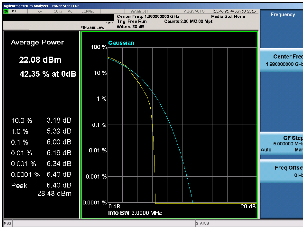
Plot 6-170. PAR Plot (Band 2 – 1.4MHz 16-QAM – RB Size 6)
