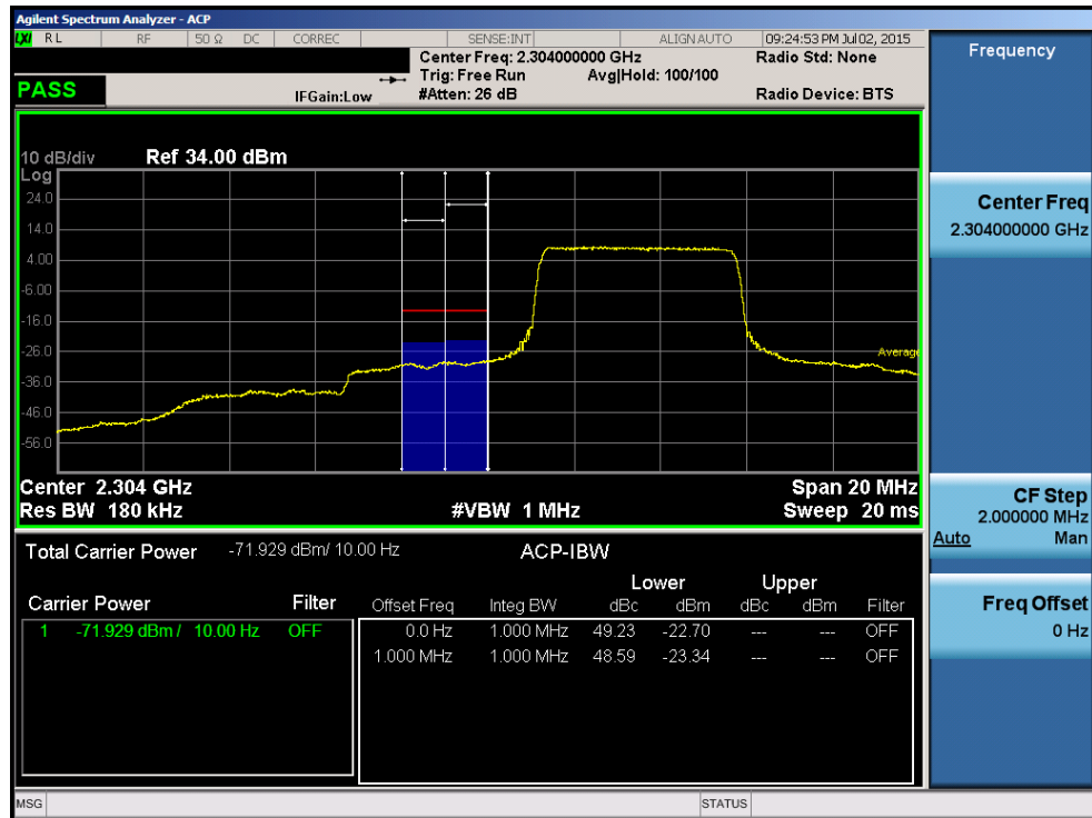
Plot 6-162. Lower Extended Band Edge Plot (Band 30 – 5.0MHz QPSK – RB Size 25)
