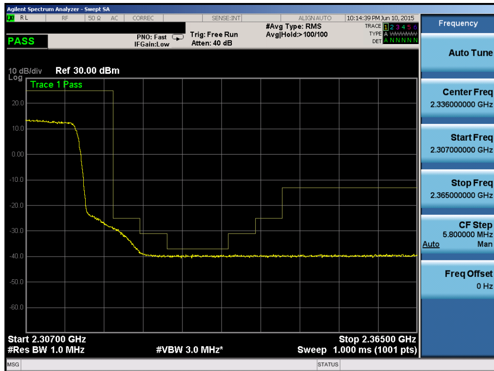
Plot 6-168. Upper Extended Band Edge Plot (Band 30 – 10.0MHz QPSK – RB Size 50)
