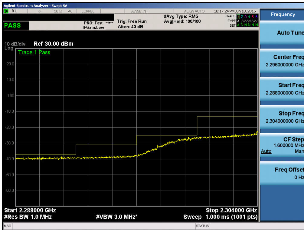
Plot 6-166. Lower Extended Band Edge Plot (Band 30 – 10.0MHz QPSK – RB Size 50)
