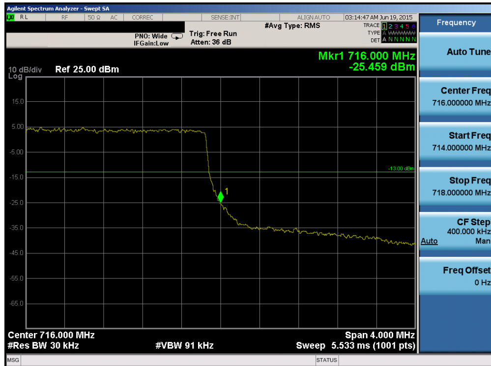
Plot 6-90. Upper Band Edge Plot (Band 12 - 3.0MHz QPSK - RB Size 15)
