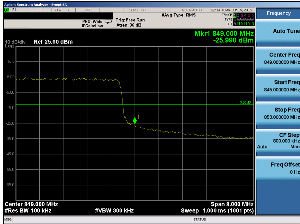
Plot 6-111. Upper Band Edge Plot (Band 5 – 10.0MHz QPSK – RB Size 50)
