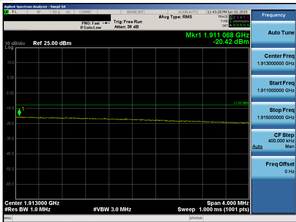
Plot 6-159. Upper Extended Band Edge Plot (Band 2 – 20.0MHz QPSK – RB Size 100)
