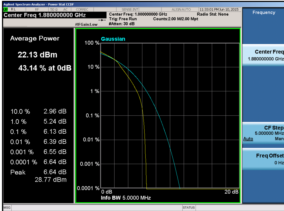
Plot 6-174. PAR Plot (Band 2 – 5.0MHz 16-QAM – RB Size 25)
