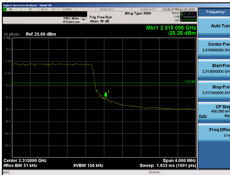
Plot 6-163. Upper Band Edge Plot (Band 30 – 5.0MHz QPSK – RB Size 25)
