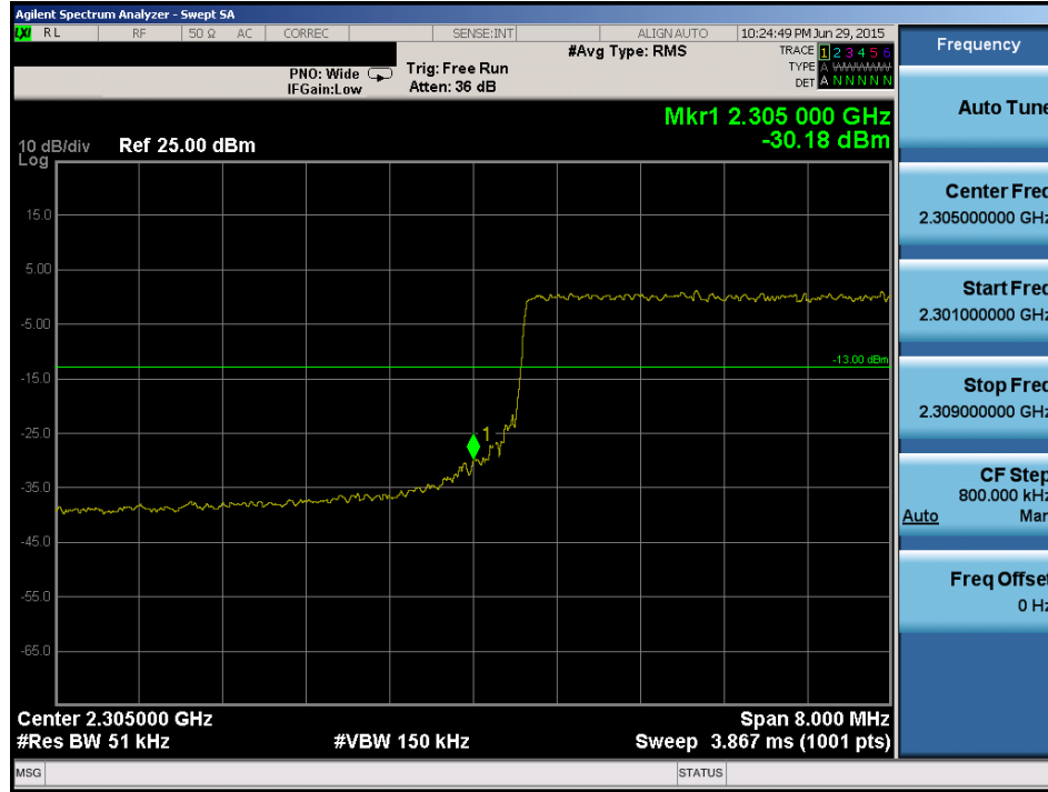
Plot 6-165. Lower Band Edge Plot (Band 30 – 10.0MHz QPSK – RB Size 50)
