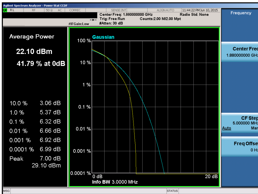
Plot 6-172. PAR Plot (Band 2 – 3.0MHz 16-QAM – RB Size 15)
