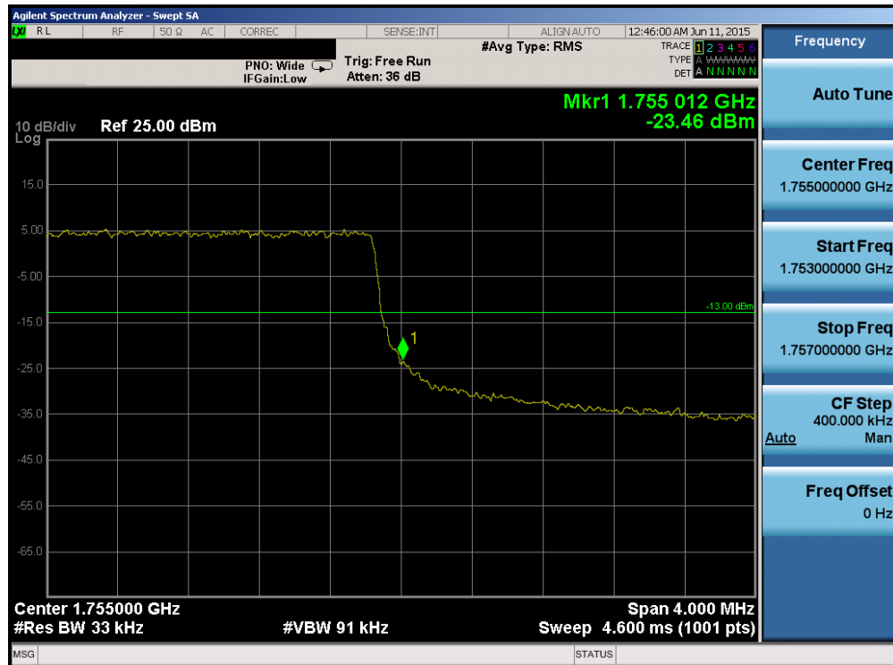
Plot 6-118. Upper Band Edge Plot (Band 4 – 3.0MHz QPSK – RB Size 15)
