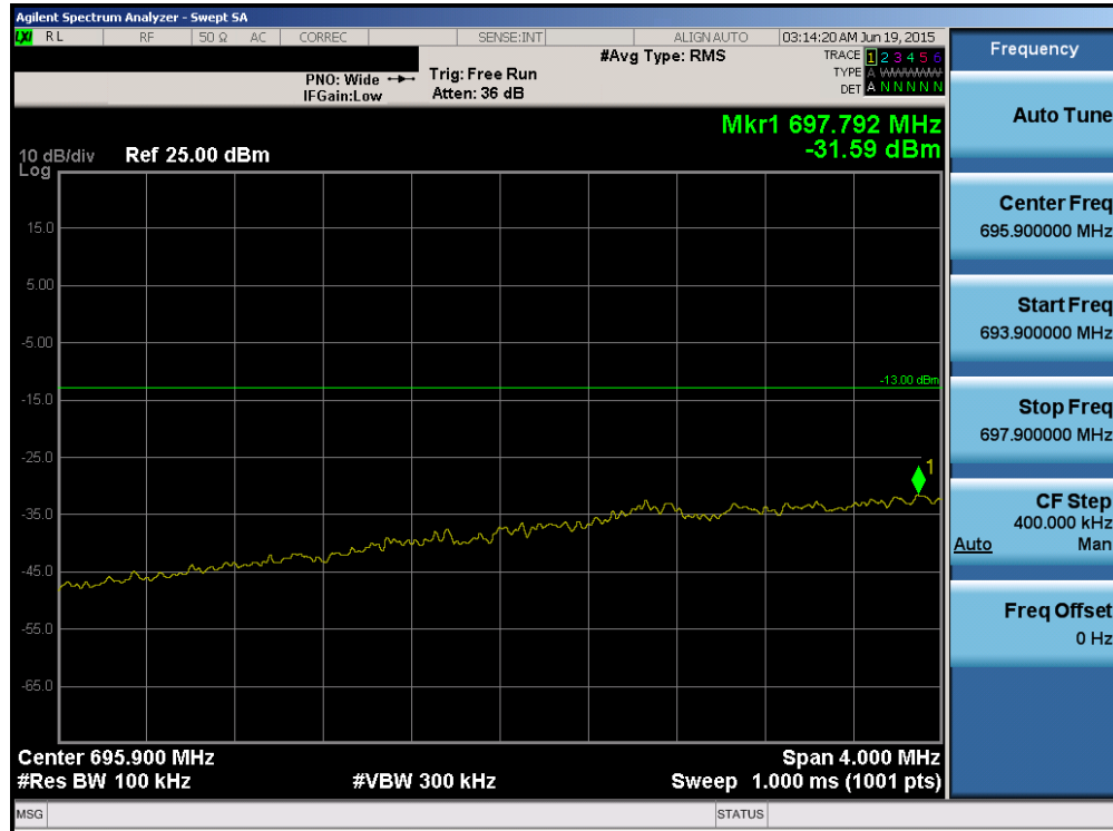
Plot 6-89. Lower Extended Band Edge Plot (Band 12 - 3.0MHz QPSK - RB Size 15)
