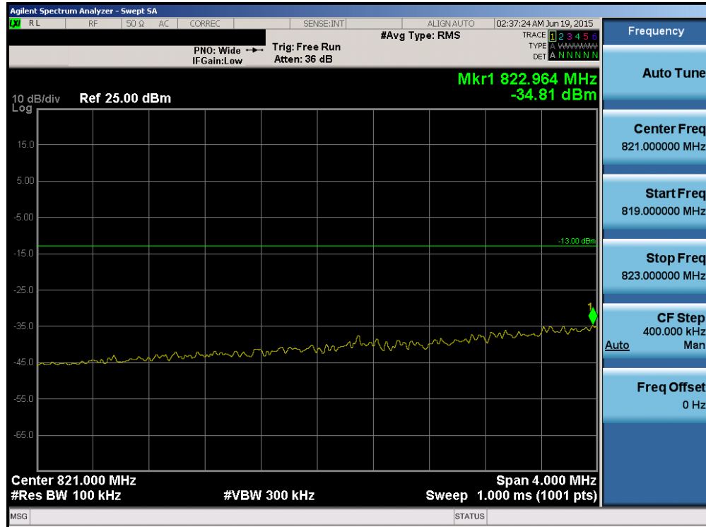
Plot 6-103. Lower Extended Band Edge Plot (Band 5 – 3.0MHz QPSK – RB Size 15)
