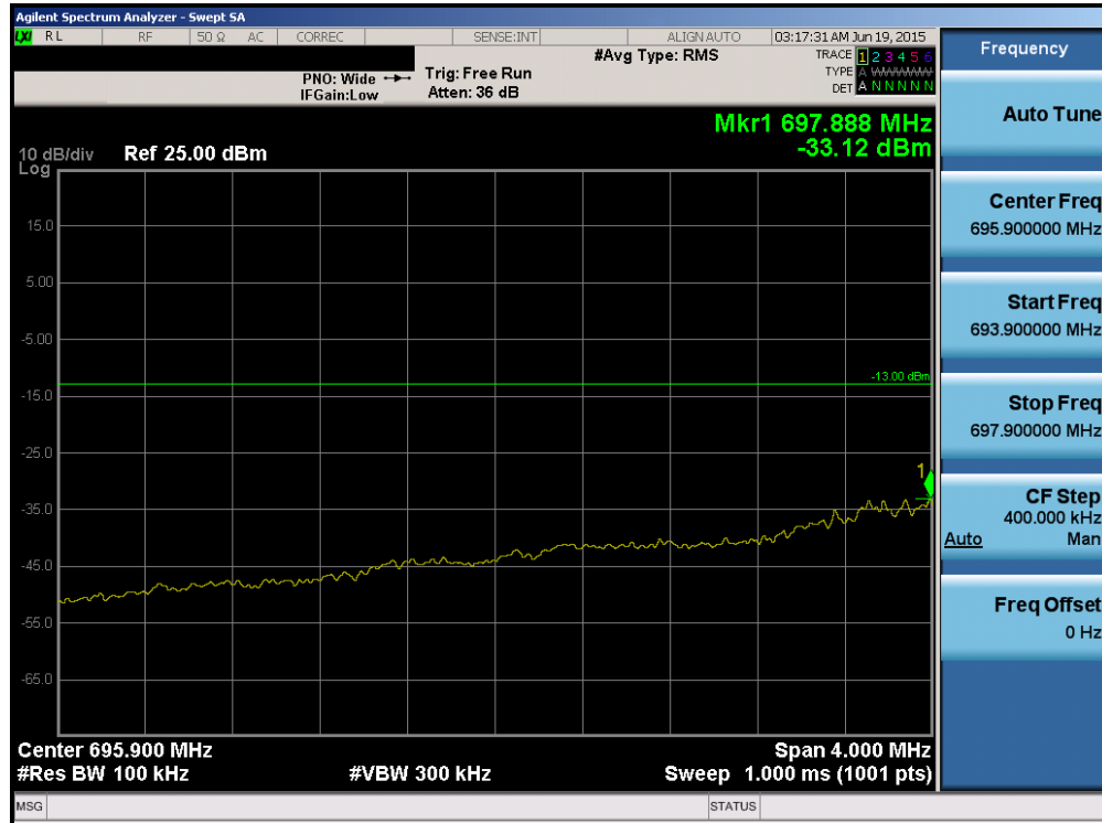
Plot 6-85. Lower Extended Band Edge Plot (Band 12 – 1.4MHz QPSK – RB Size 6)
