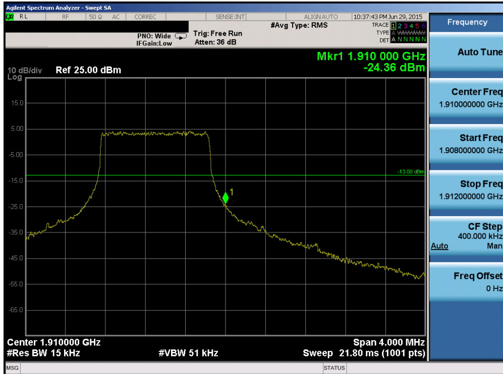
Plot 6-138. Upper Band Edge Plot (Band 2 – 1.4MHz QPSK – RB Size 6)
