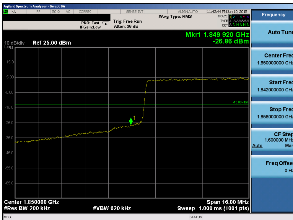
Plot 6-156. Lower Band Edge Plot (Band 2 – 20.0MHz QPSK – RB Size 100)
