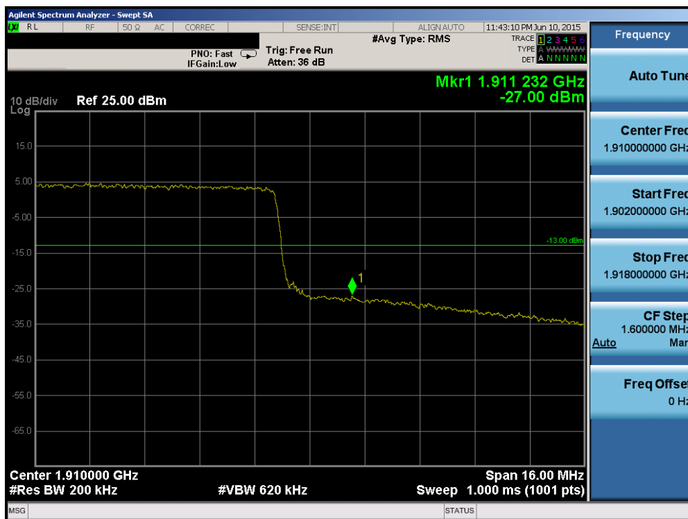
Plot 6-158. Upper Band Edge Plot (Band 2 – 20.0MHz QPSK – RB Size 100)
