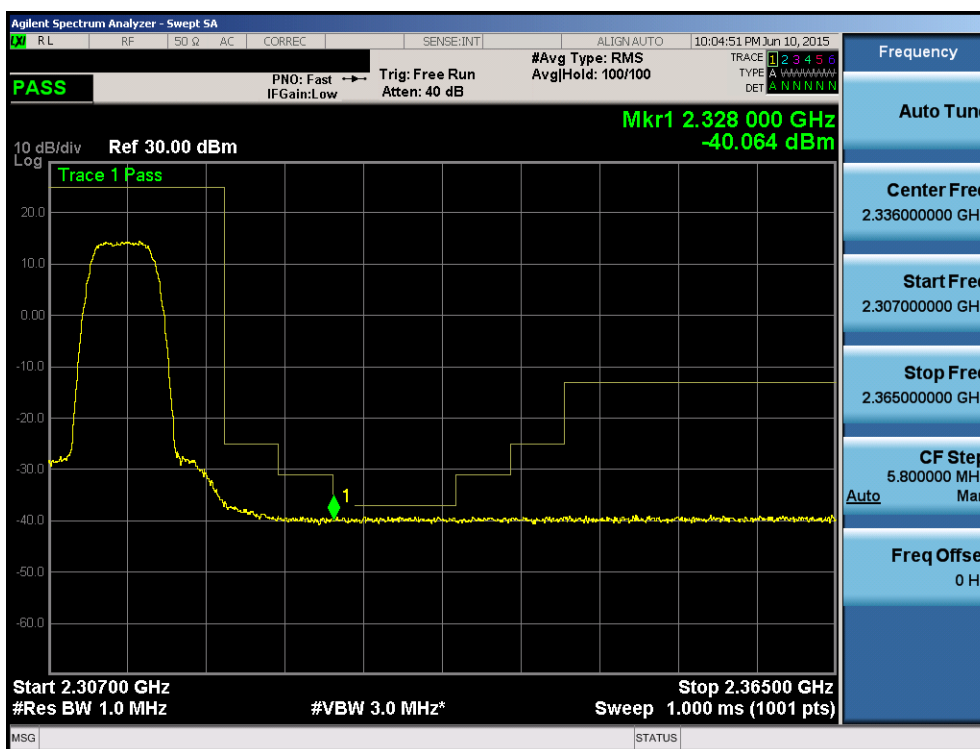
Plot 6-164. Upper Extended Band Edge Plot (Band 30 – 5.0MHz QPSK – RB Size 25)
