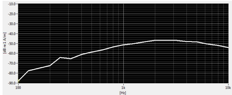
Figure 8-4 Worst-case ABM2 Plot for LTE
