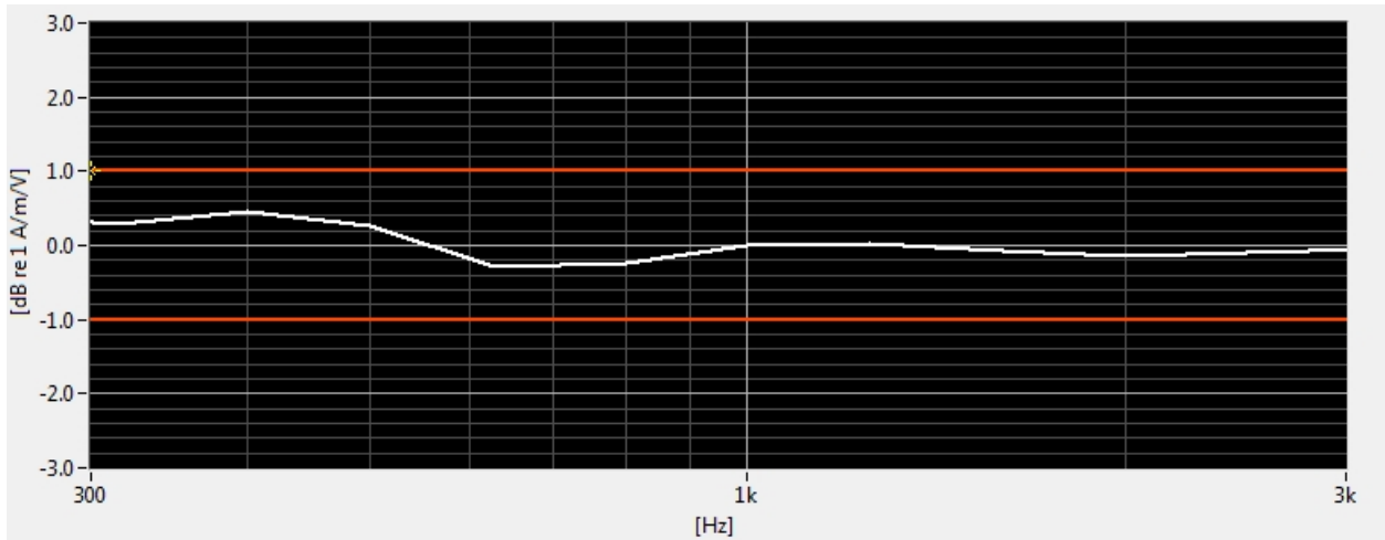
Figure 8-5 Helmholtz Coil Validation for Frequency Response
