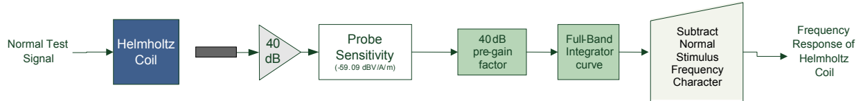
Figure 5-6 Frequency Response Validation
