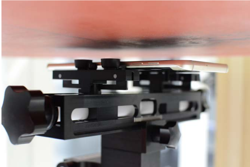
SAR Test Setup Photo 5: Back at 15 mm
