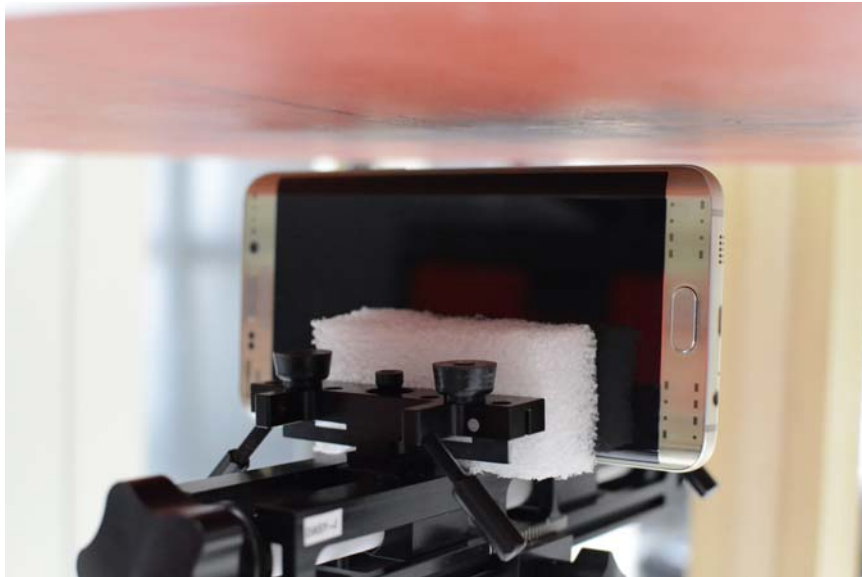
SAR Test Setup Photo 10: Right at 10 mm
