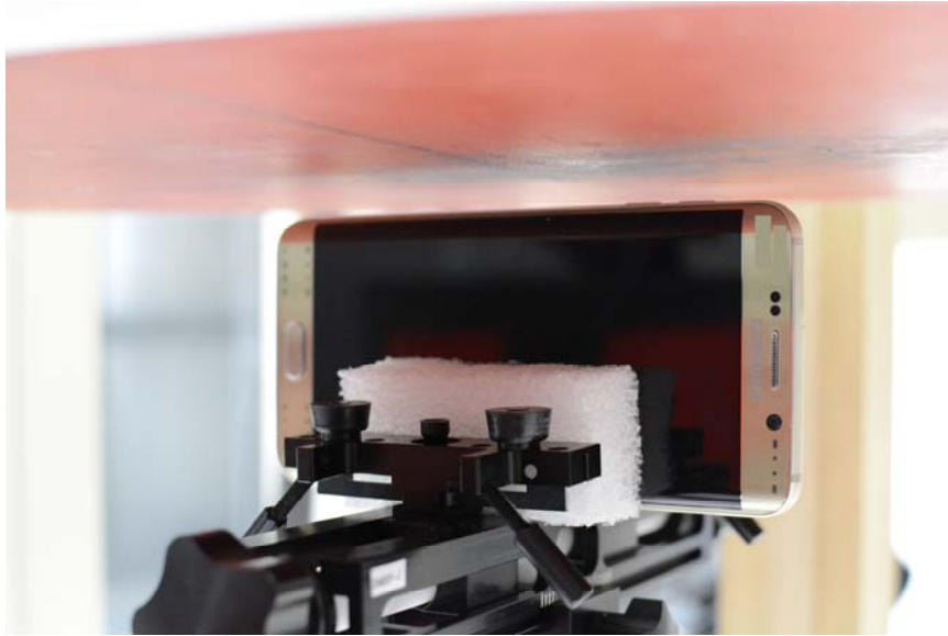
SAR Test Setup Photo 11: Left at 10 mm
