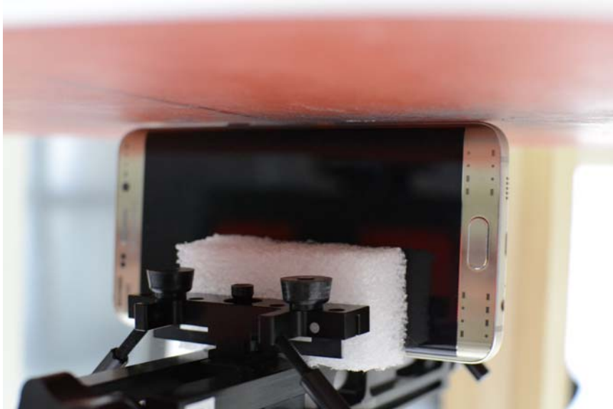
SAR Test Setup Photo 19: Right at 0 mm
