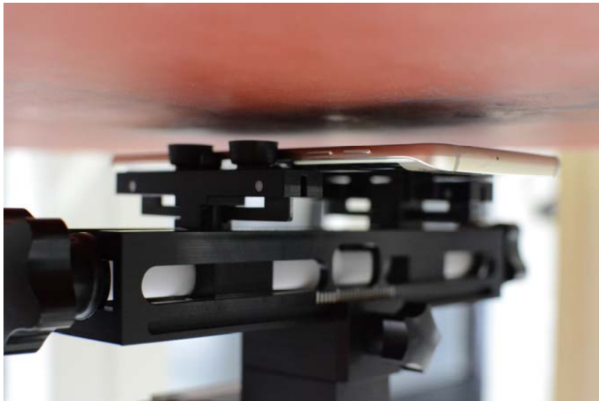
SAR Test Setup Photo 6: Back at 10 mm
