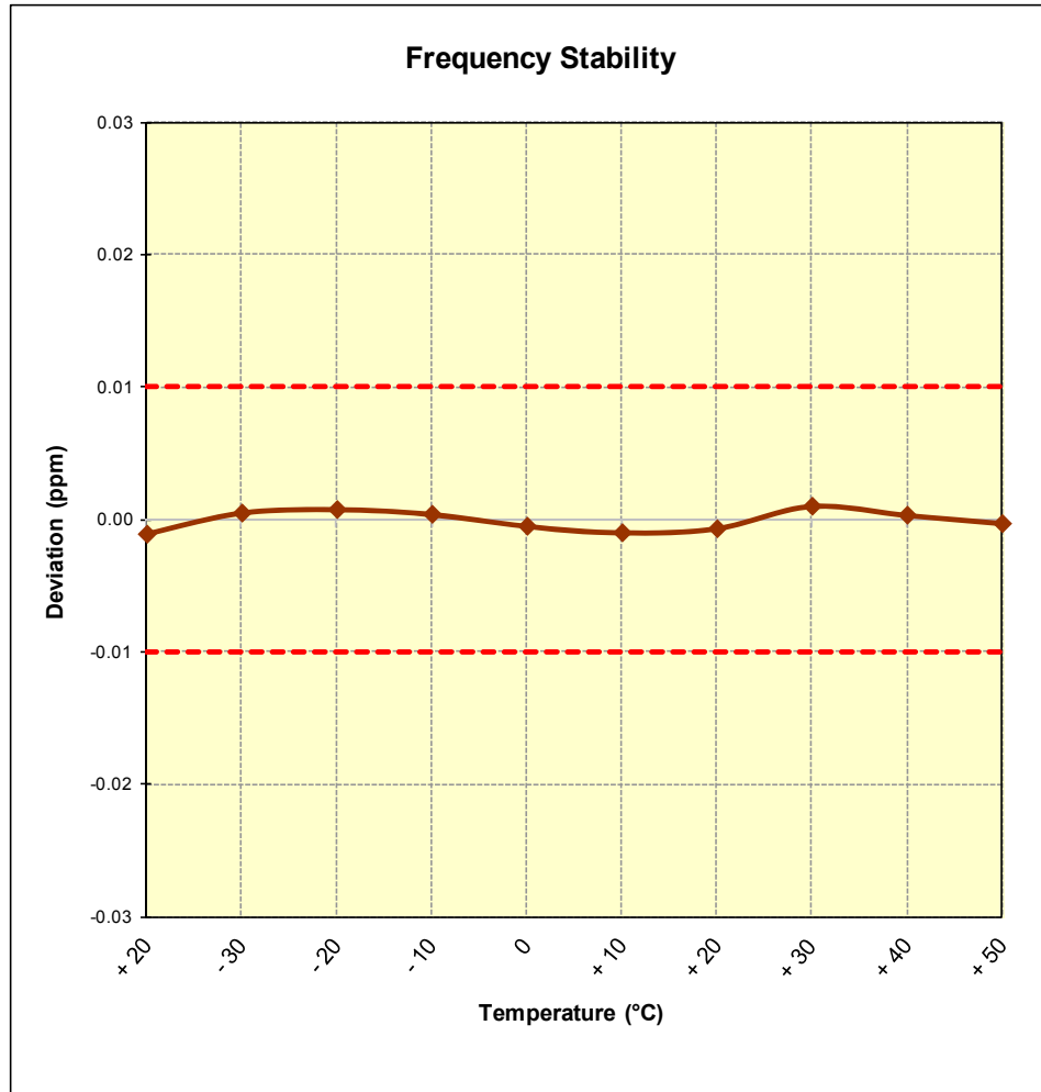
Figure 7-4. Frequency Stability Plot
