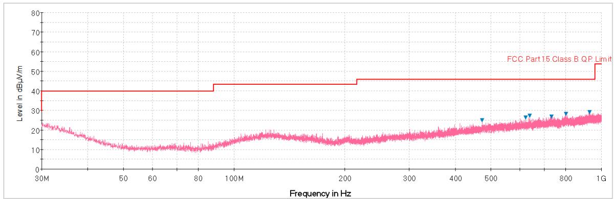
Plot 6-222. Radiated Spurious Plot below 1GHz (802.11a – U3 Ch. 157, Ant. Pol. H)
