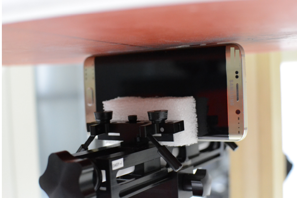
SAR Test Setup Photo 9– Left Edge at 0.0 cm
