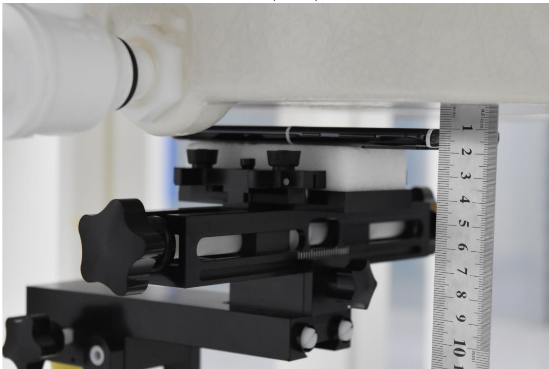
Front (10 mm)
