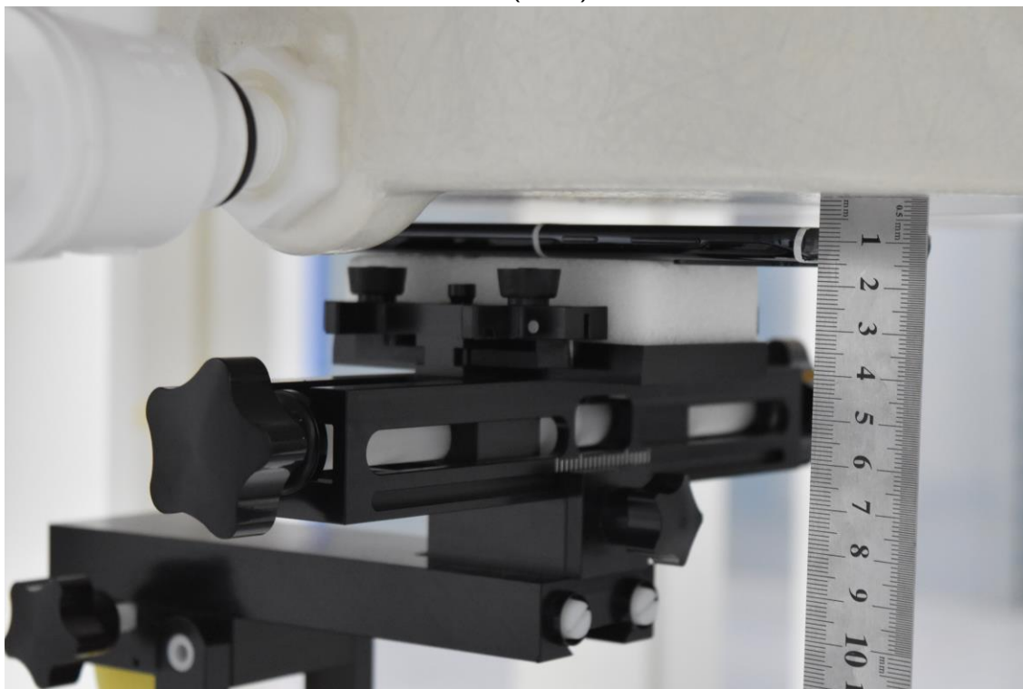
Front (7 mm)
