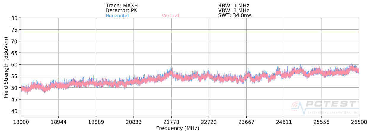
Plot 7-45. Radiated Spurious Plot above 18GHz
