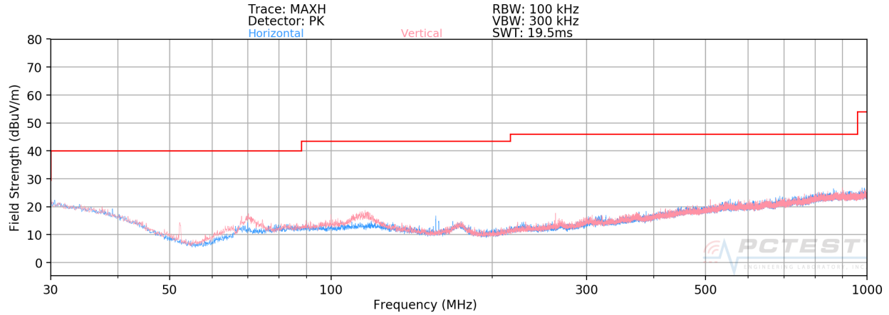
Plot 7-48. Radiated Spurious Plot below 1GHz
