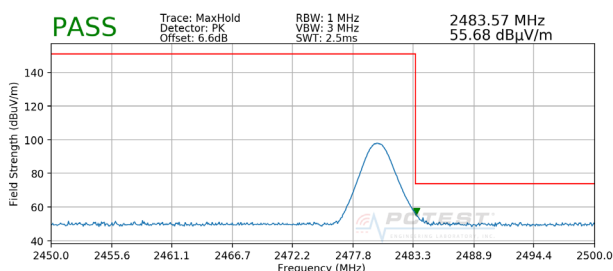
Plot 7-47. Radiated Restricted Upper Band Edge Measurement (Peak)
