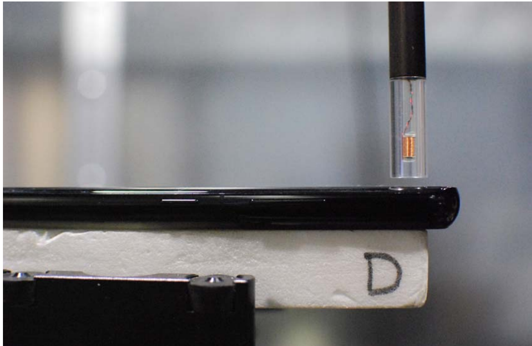
Figure 16-2 Test Setup for Wireless Device
