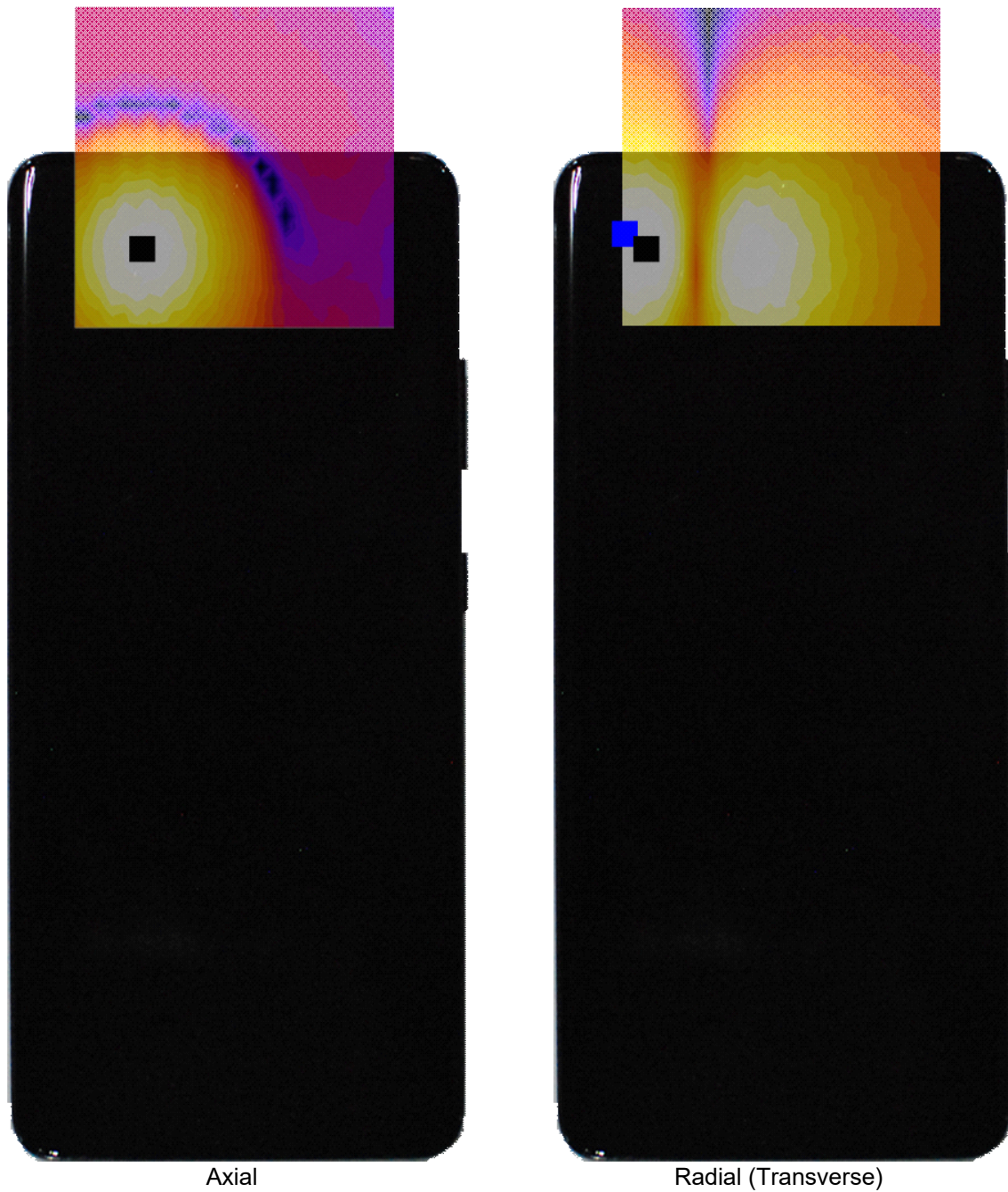
Figure 16-3 T-Coil Scan Overlay Magnetic Field Distributions
