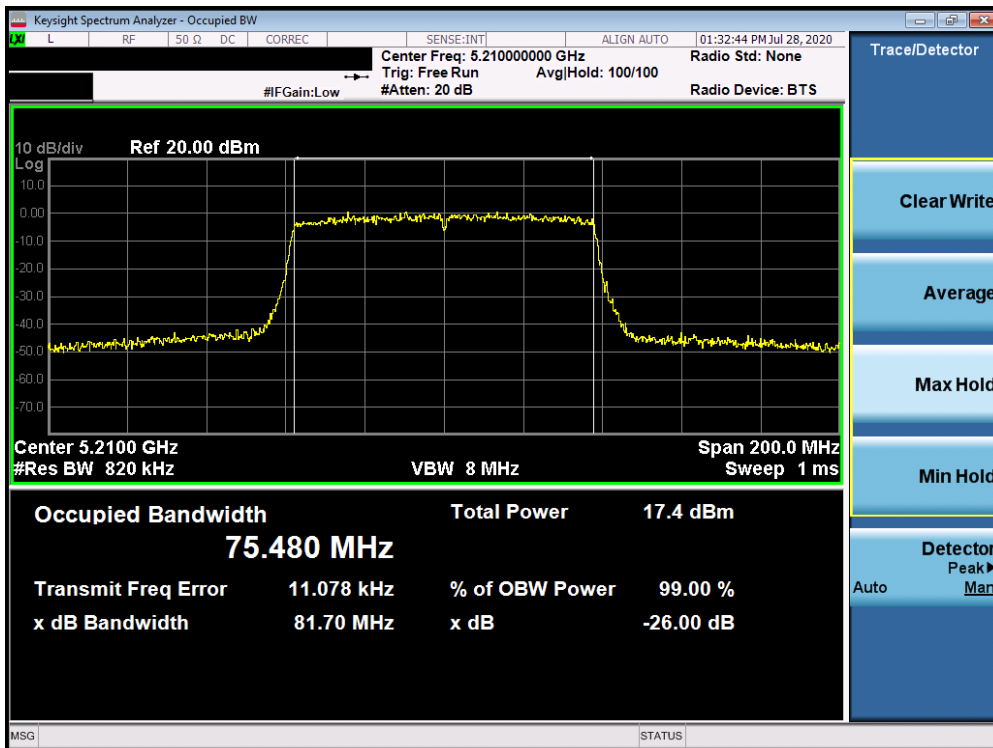
Plot 7-14. 26dB Bandwidth Plot ANT3 (80MHz BW 802.11ac (UNII Band 1) – Ch. 42)
