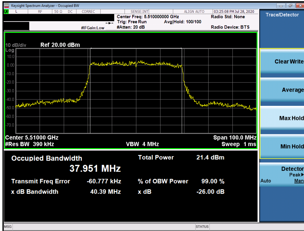
Plot 7-43. 26dB Bandwidth Plot ANT3 (40MHz BW 802.11ax (UNII Band 2C) – Ch. 102)
