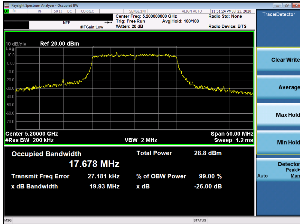
Plot 7-56. 26dB Bandwidth Plot ANT4 (20MHz BW 802.11n (UNII Band 1) – Ch. 40)
