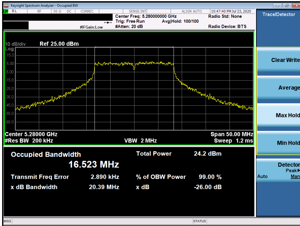
Plot 7-68. 26dB Bandwidth Plot ANT4 (802.11a (UNII Band 2A) – Ch. 56)
