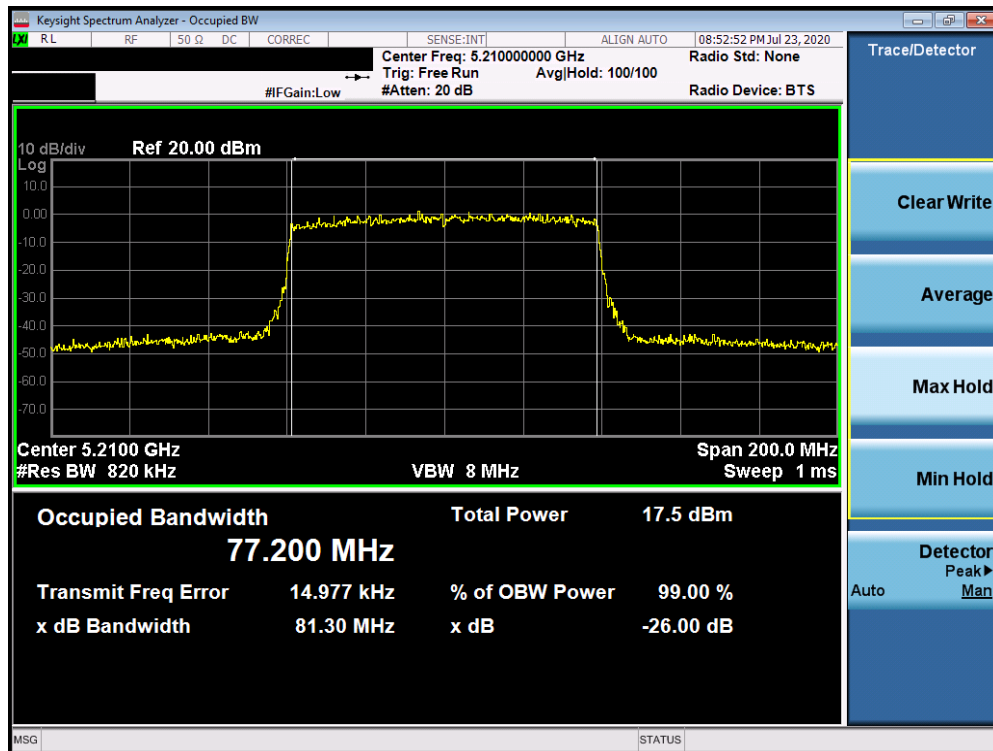
Plot 7-15. 26dB Bandwidth Plot ANT3 (80MHz BW 802.11ax (UNII Band 1) – Ch. 42)
