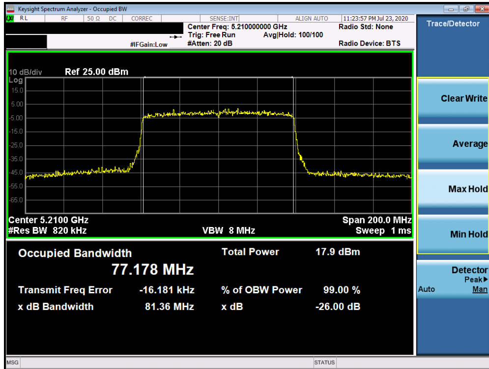
Plot 7-66. 26dB Bandwidth Plot ANT4 (80MHz BW 802.11ax (UNII Band 1) – Ch. 42)
