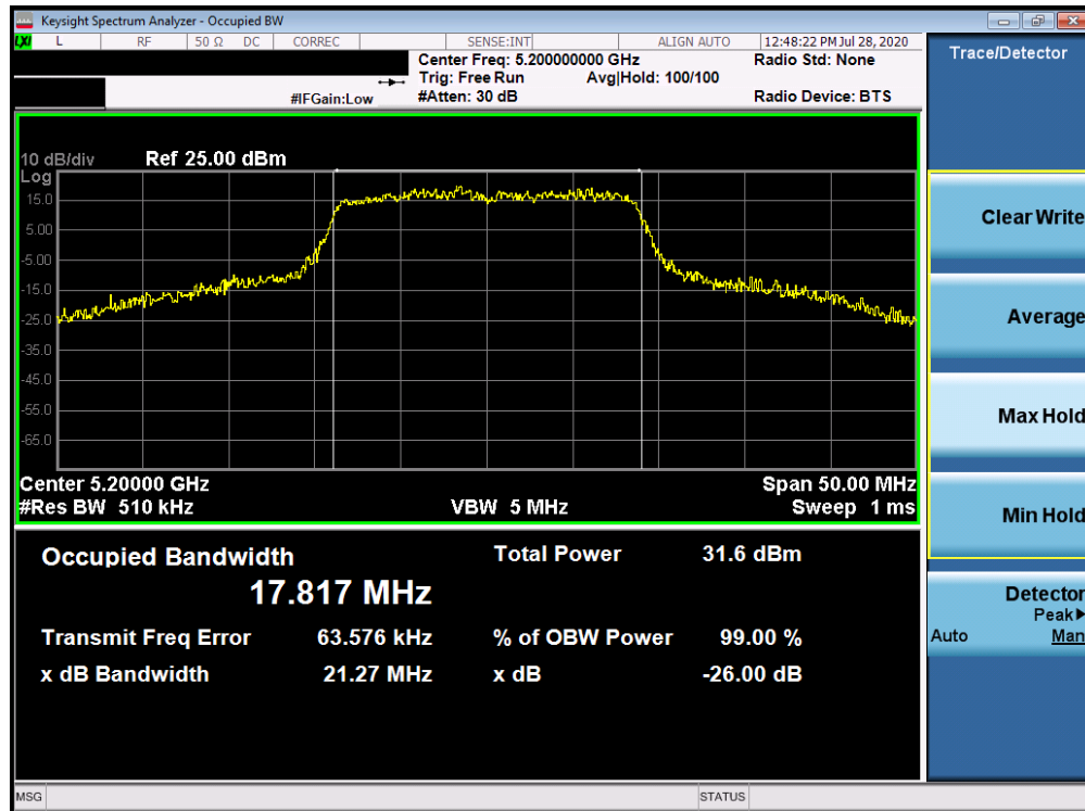
Plot 7-5. 26dB Bandwidth Plot ANT3 (20MHz BW 802.11n (UNII Band 1) – Ch. 40)
