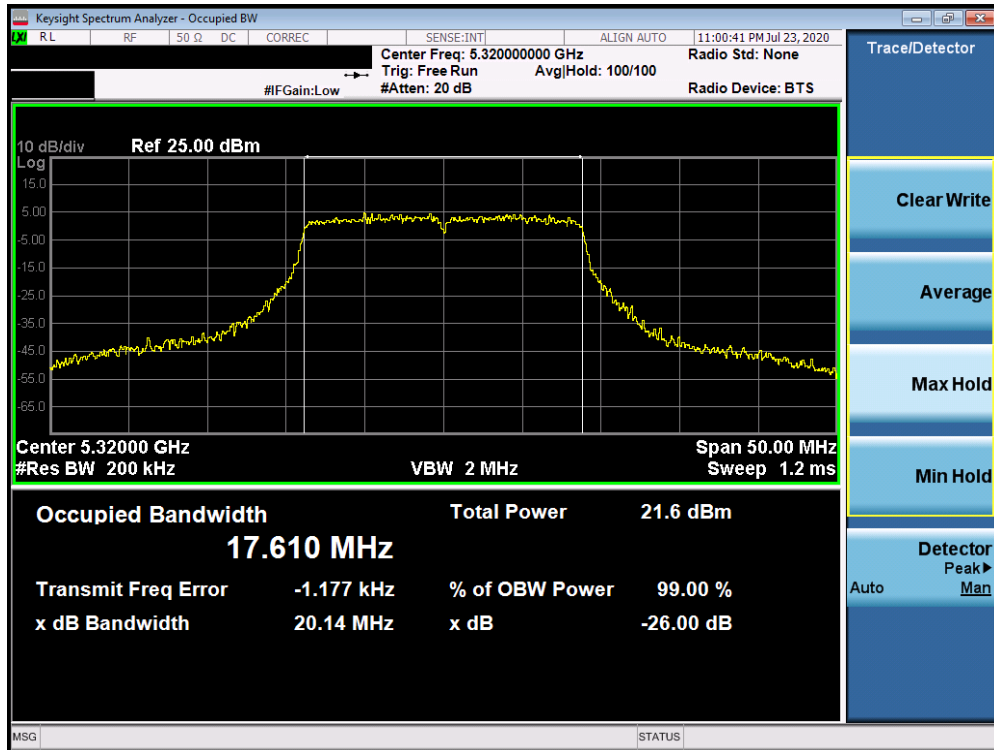
Plot 7-75. 26dB Bandwidth Plot ANT4 (20MHz BW 802.11ax (UNII Band 2A) – Ch. 64)
