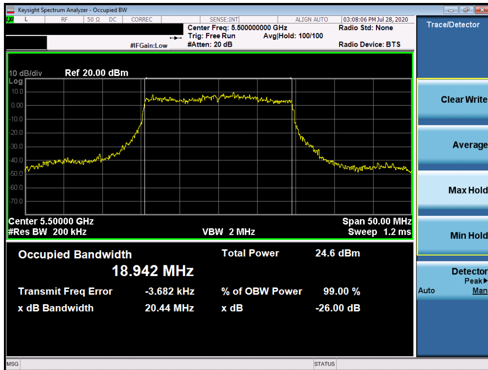
Plot 7-37. 26dB Bandwidth Plot ANT3 (20MHz BW 802.11ax (UNII Band 2C) – Ch. 100)
