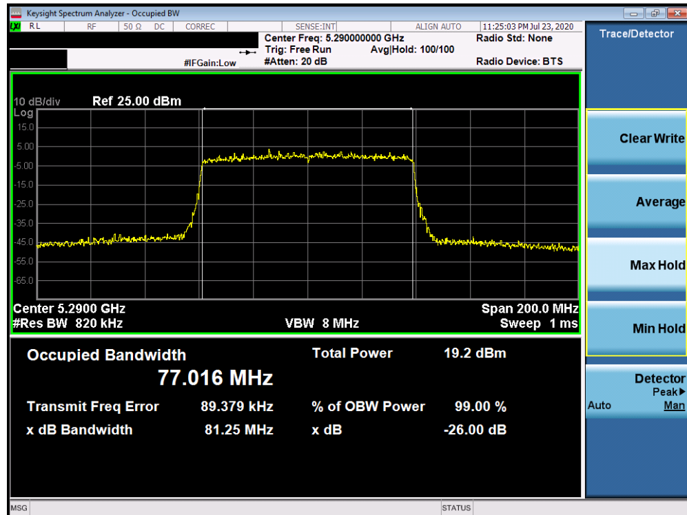
Plot 7-81. 26dB Bandwidth Plot ANT4 (80MHz BW 802.11ax (UNII Band 2A) – Ch. 58)
