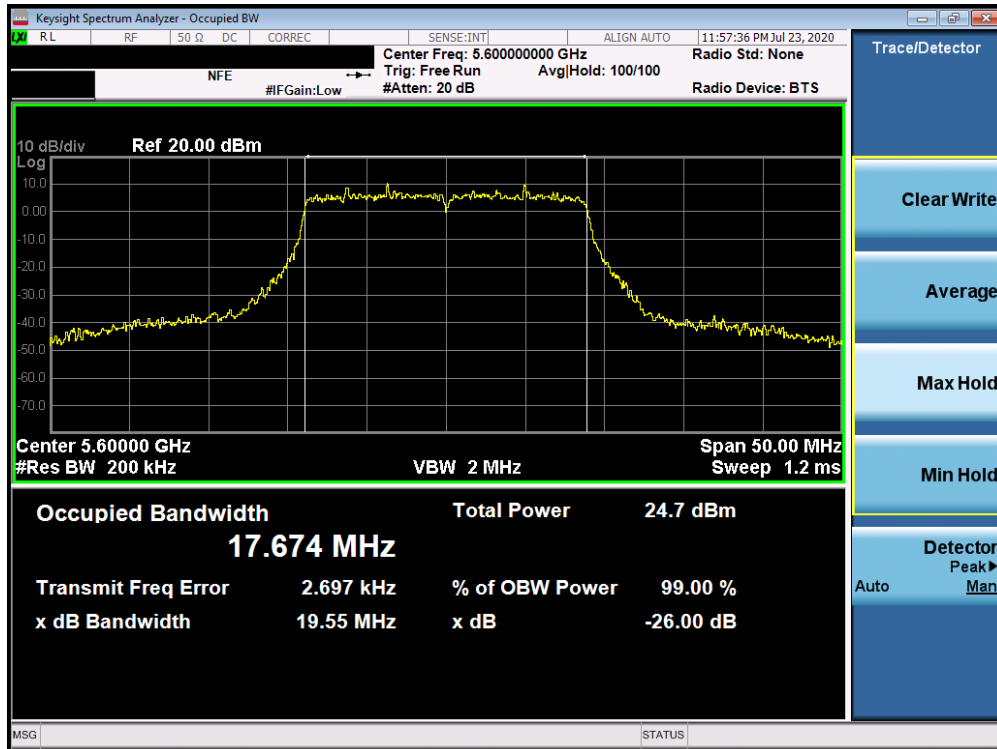
Plot 7-86. 26dB Bandwidth Plot ANT4 (20MHz BW 802.11n (UNII Band 2C) – Ch. 120)
