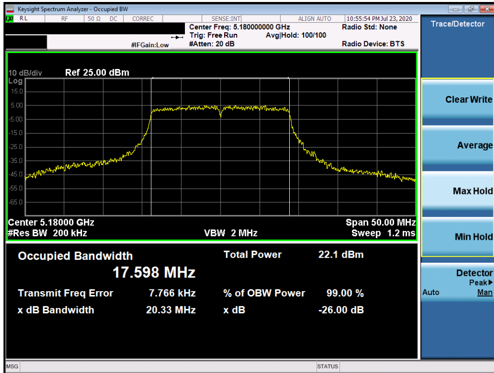
Plot 7-58. 26dB Bandwidth Plot ANT4 (20MHz BW 802.11ax (UNII Band 1) – Ch. 36)
