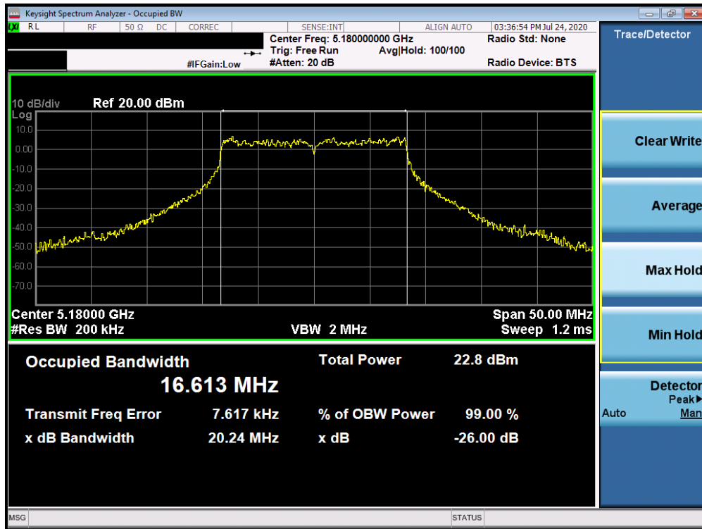
Plot 7-103. 26dB Bandwidth Plot ANT5 (802.11a (UNII Band 1) – Ch. 36)
