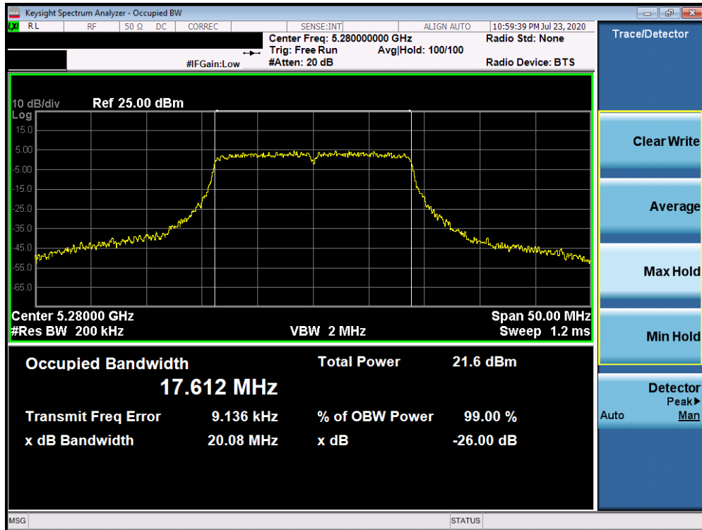
Plot 7-74. 26dB Bandwidth Plot ANT4 (20MHz BW 802.11ax (UNII Band 2A) – Ch. 56)
