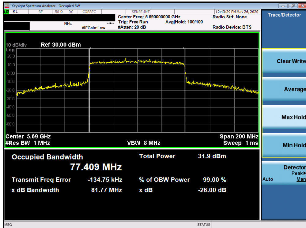
Plot 7-99. 26dB Bandwidth Plot ANT4 (80MHz BW 802.11ac (UNII Band 2C) – Ch. 138)
