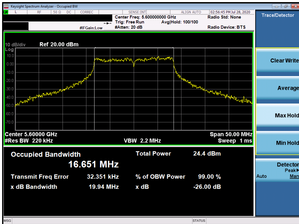
Plot 7-32. 26dB Bandwidth Plot ANT3 (802.11a (UNII Band 2C) – Ch. 120)
