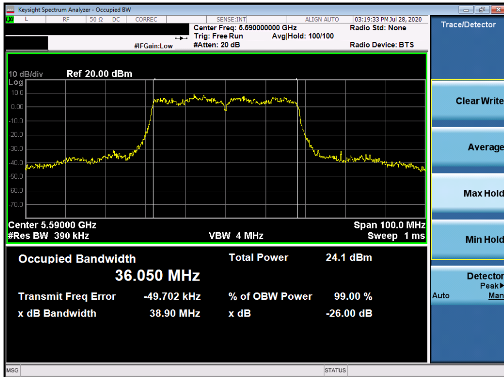
Plot 7-41. 26dB Bandwidth Plot ANT3 (40MHz BW 802.11n (UNII Band 2C) – Ch. 118)
