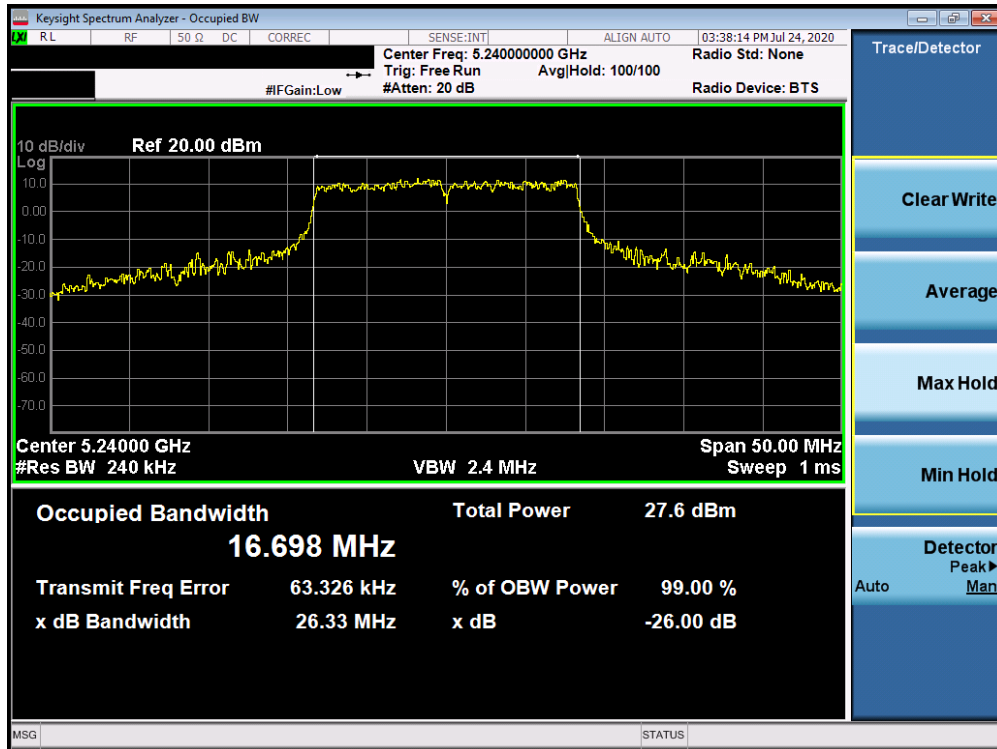
Plot 7-105. 26dB Bandwidth Plot ANT5 (802.11a (UNII Band 1) – Ch. 48)
