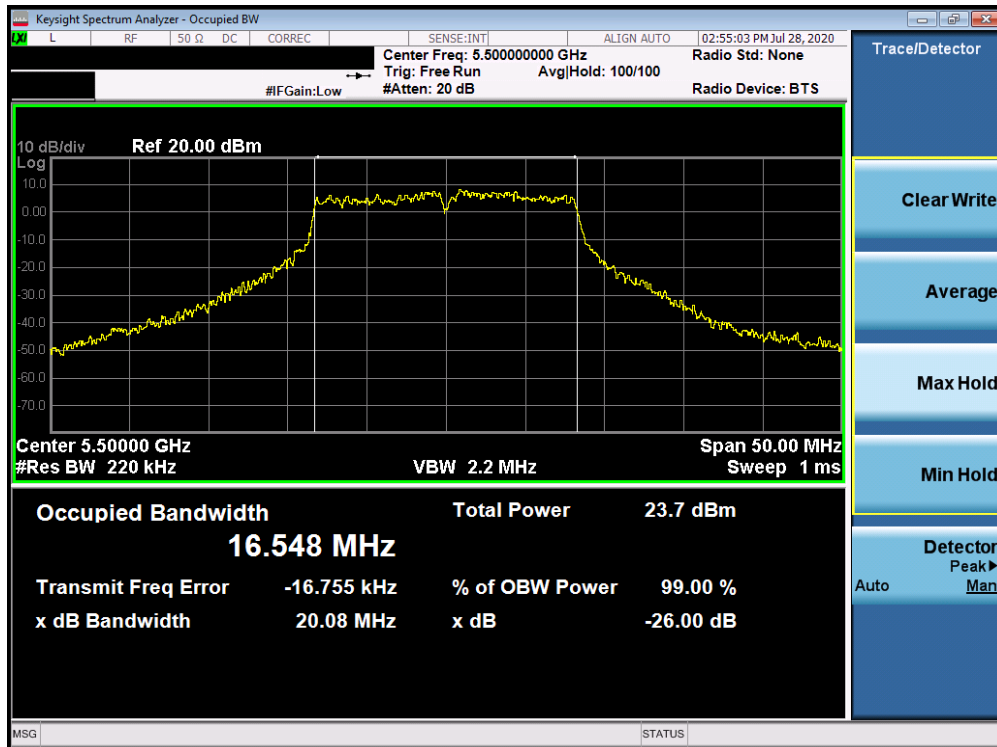
Plot 7-31. 26dB Bandwidth Plot ANT3 (802.11a (UNII Band 2C) – Ch. 100)
