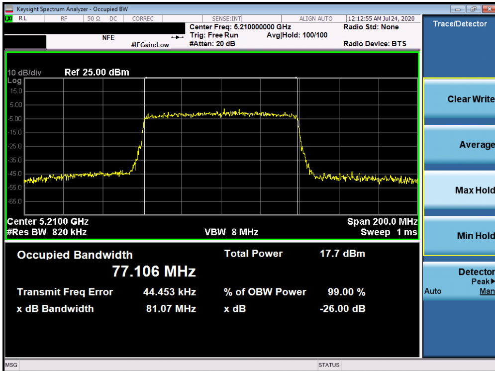
Plot 7-65. 26dB Bandwidth Plot ANT4 (80MHz BW 802.11ac (UNII Band 1) – Ch. 42)
