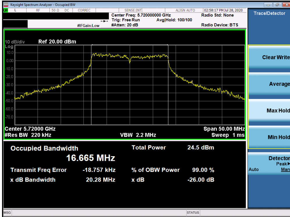
Plot 7-33. 26dB Bandwidth Plot ANT3 (802.11a (UNII Band 2C) – Ch. 144)
