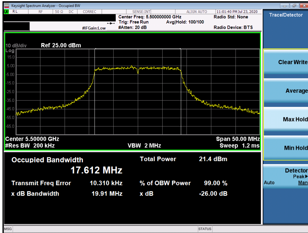
Plot 7-88. 26dB Bandwidth Plot ANT4 (20MHz BW 802.11ax (UNII Band 2C) – Ch. 100)
