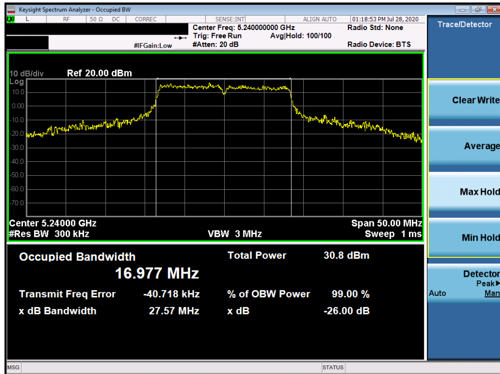
Plot 7-3. 26dB Bandwidth Plot ANT3 (802.11a (UNII Band 1) – Ch. 48)
