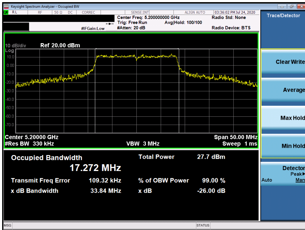
Plot 7-104. 26dB Bandwidth Plot ANT5 (802.11a (UNII Band 1) – Ch. 40)
