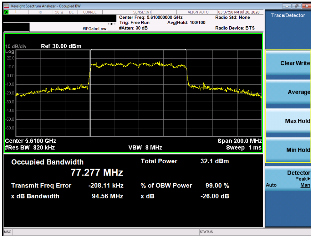
Plot 7-50. 26dB Bandwidth Plot ANT3 (80MHz BW 802.11ax (UNII Band 2C) – Ch. 122)
