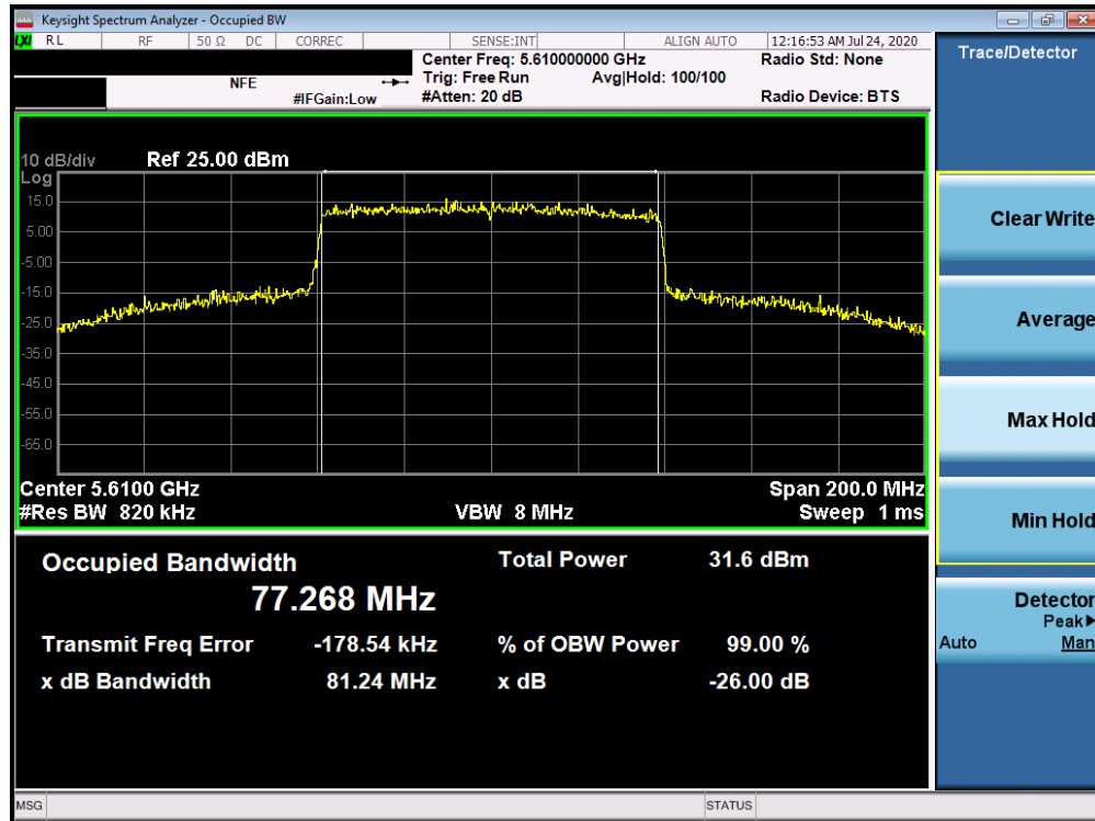
Plot 7-98. 26dB Bandwidth Plot ANT4 (80MHz BW 802.11ac (UNII Band 2C) – Ch. 122)
