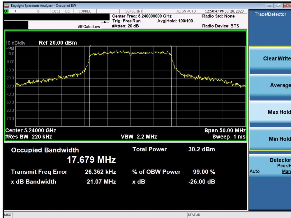
Plot 7-6. 26dB Bandwidth Plot ANT3 (20MHz BW 802.11n (UNII Band 1) – Ch. 48)
