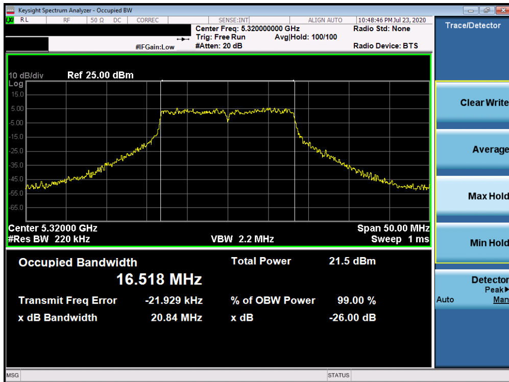
Plot 7-69. 26dB Bandwidth Plot ANT4 (802.11a (UNII Band 2A) – Ch. 64)
