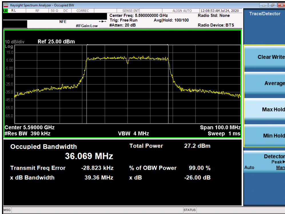
Plot 7-92. 26dB Bandwidth Plot ANT4 (40MHz BW 802.11n (UNII Band 2C) – Ch. 118)
