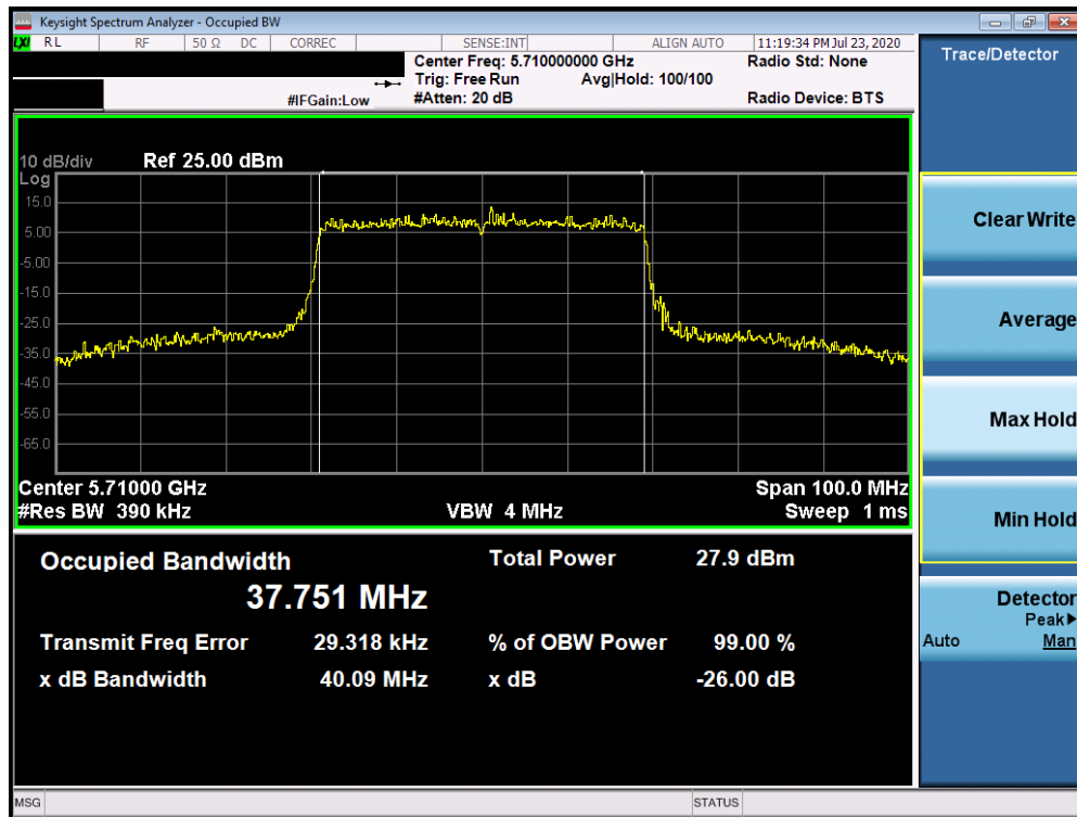
Plot 7-96. 26dB Bandwidth Plot ANT4 (40MHz BW 802.11ax (UNII Band 2C) – Ch. 142)
