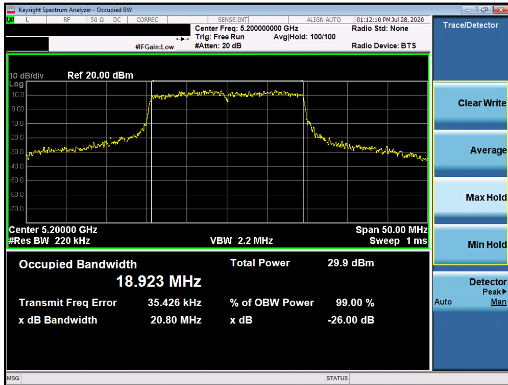
Plot 7-8. 26dB Bandwidth Plot ANT3 (20MHz BW 802.11ax (UNII Band 1) – Ch. 40)
