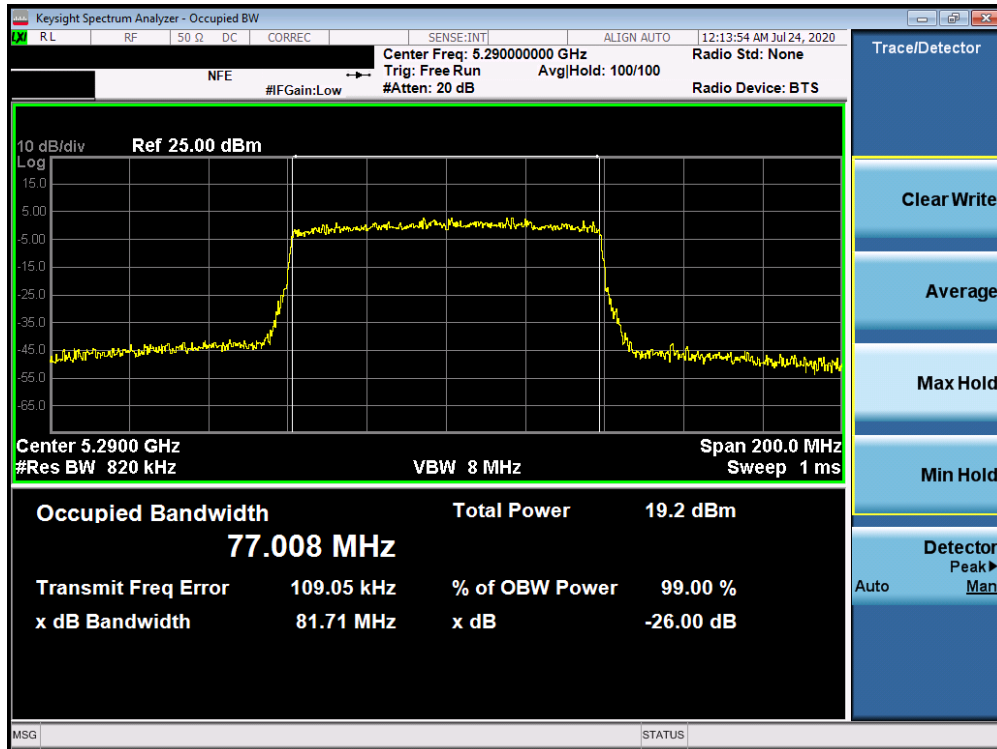
Plot 7-80. 26dB Bandwidth Plot ANT4 (80MHz BW 802.11ac (UNII Band 2A) – Ch. 58)
