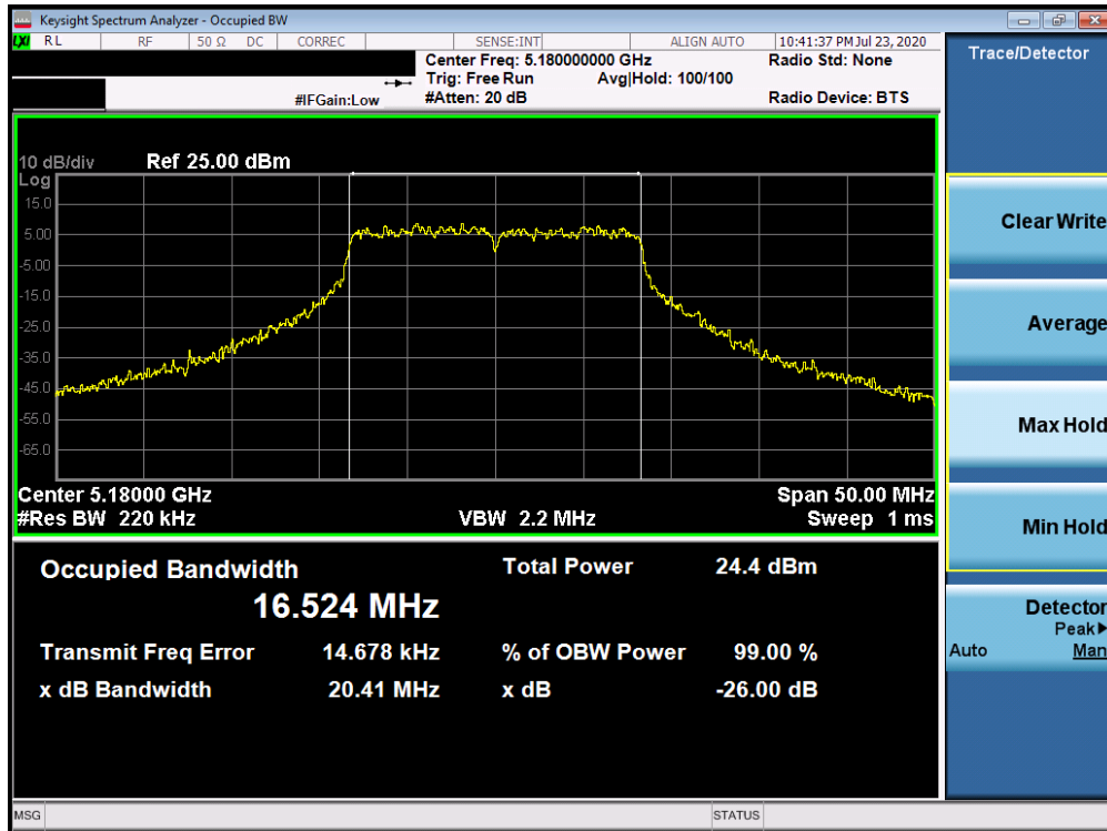
Plot 7-52. 26dB Bandwidth Plot ANT4 (802.11a (UNII Band 1) – Ch. 36)
