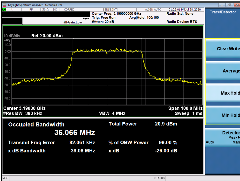
Plot 7-10. 26dB Bandwidth Plot ANT3 (40MHz BW 802.11n (UNII Band 1) – Ch. 38)
