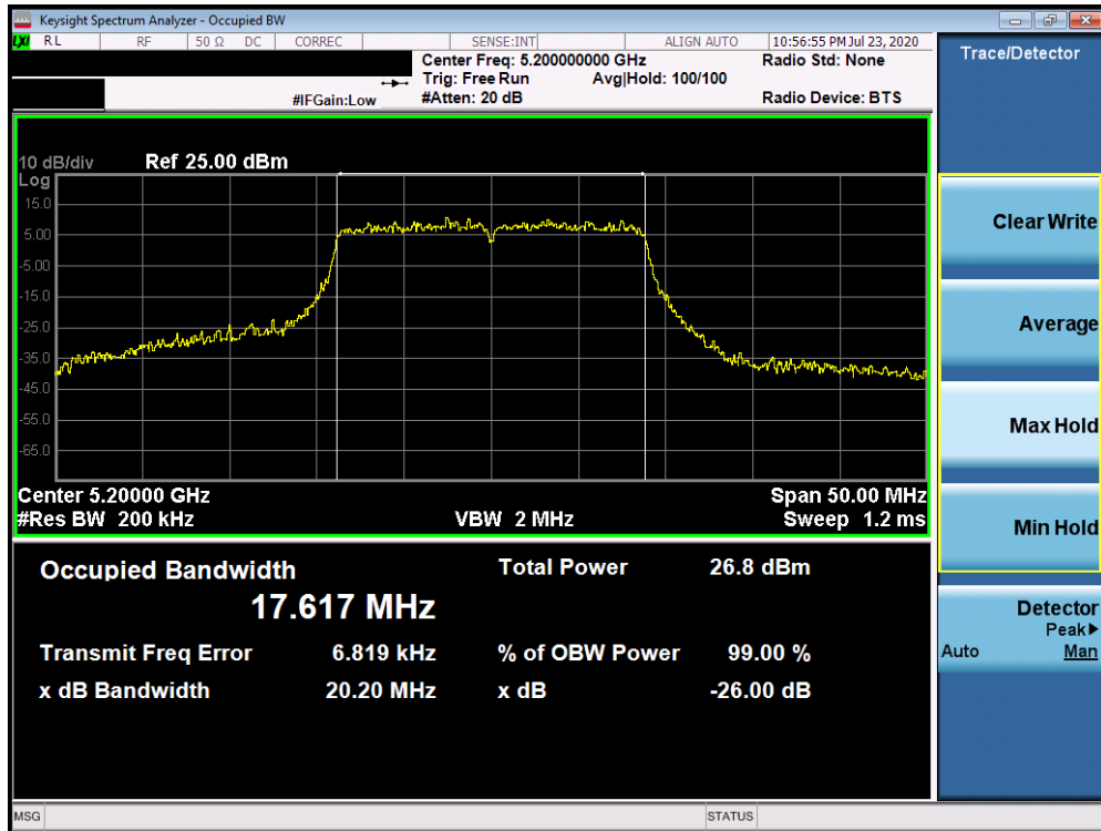
Plot 7-59. 26dB Bandwidth Plot ANT4 (20MHz BW 802.11ax (UNII Band 1) – Ch. 40)
