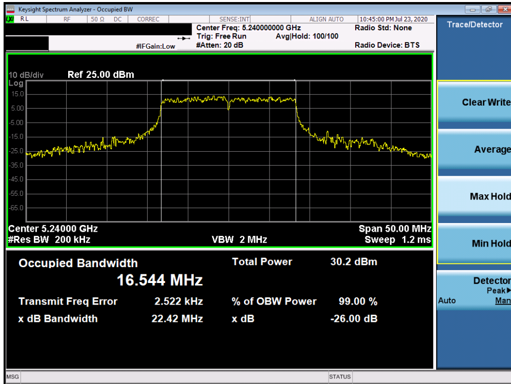
Plot 7-54. 26dB Bandwidth Plot ANT4 (802.11a (UNII Band 1) – Ch. 48)
