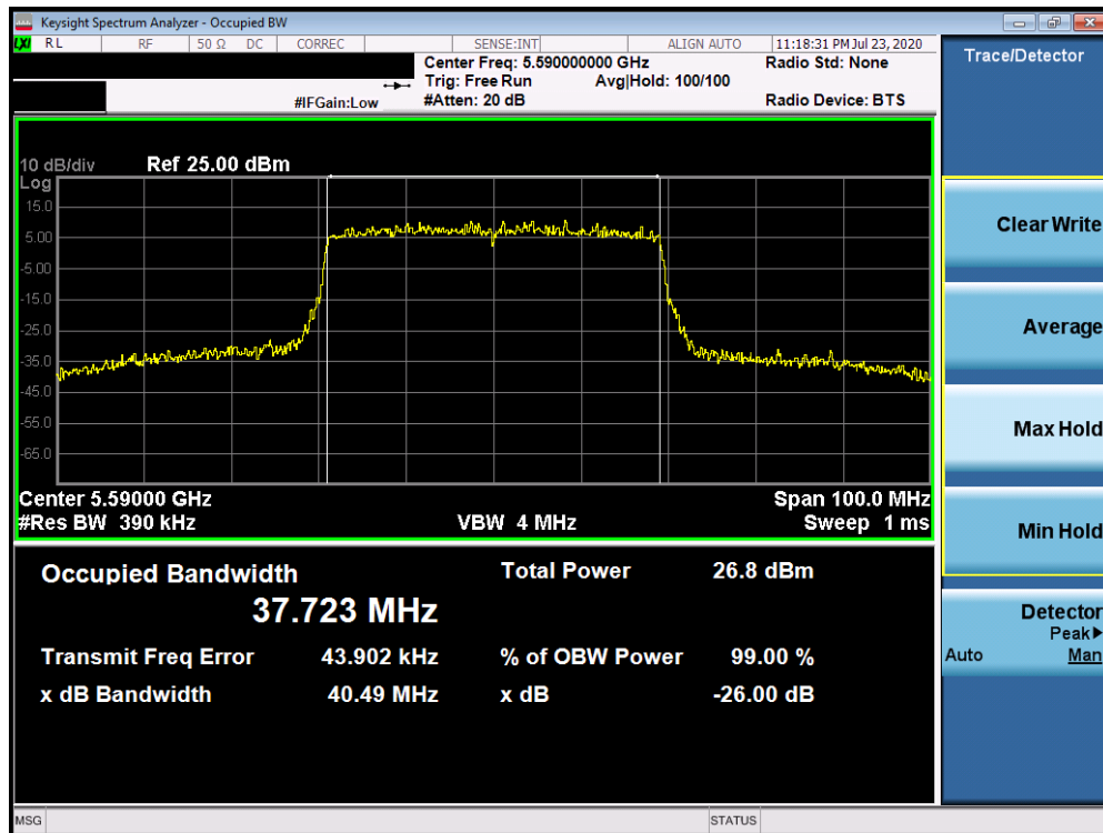
Plot 7-95. 26dB Bandwidth Plot ANT4 (40MHz BW 802.11ax (UNII Band 2C) – Ch. 118)
