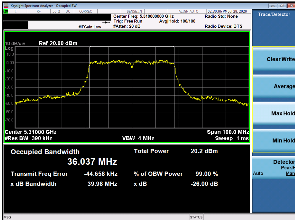
Plot 7-26. 26dB Bandwidth Plot ANT3 (40MHz BW 802.11n (UNII Band 2A) – Ch. 62)
