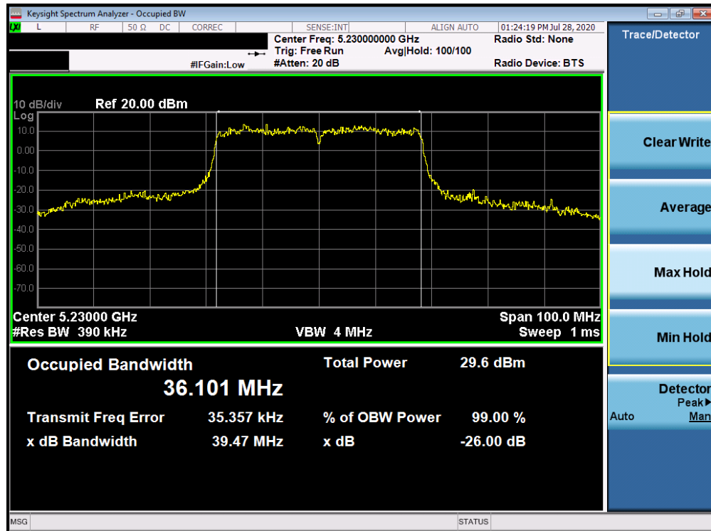
Plot 7-11. 26dB Bandwidth Plot ANT3 (40MHz BW 802.11n (UNII Band 1) – Ch. 46)
