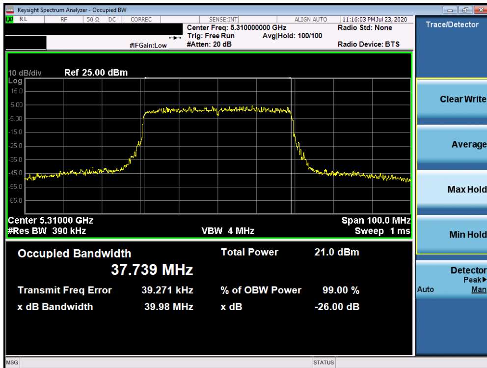
Plot 7-79. 26dB Bandwidth Plot ANT4 (40MHz BW 802.11ax (UNII Band 2a) – Ch. 62)
