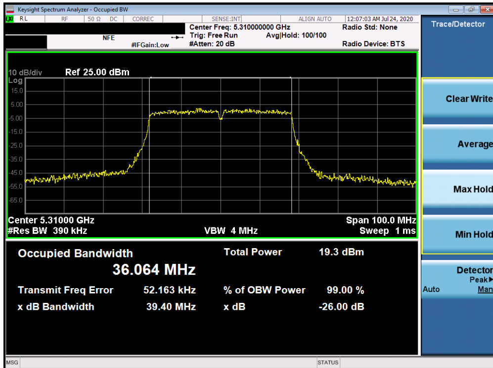
Plot 7-77. 26dB Bandwidth Plot ANT4 (40MHz BW 802.11n (UNII Band 2A) – Ch. 62)
