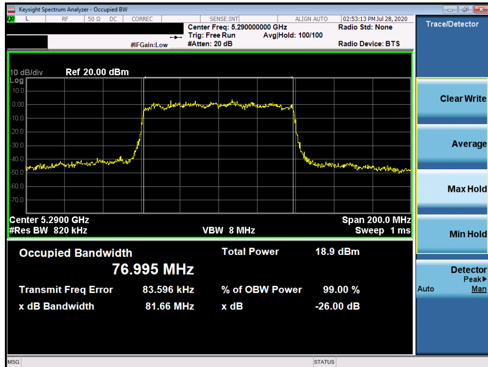
Plot 7-30. 26dB Bandwidth Plot ANT3 (80MHz BW 802.11ax (UNII Band 2A) – Ch. 58)
