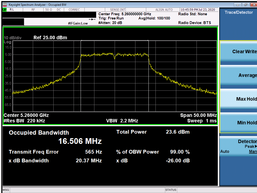
Plot 7-67. 26dB Bandwidth Plot ANT4 (802.11a (UNII Band 2A) – Ch. 52)
