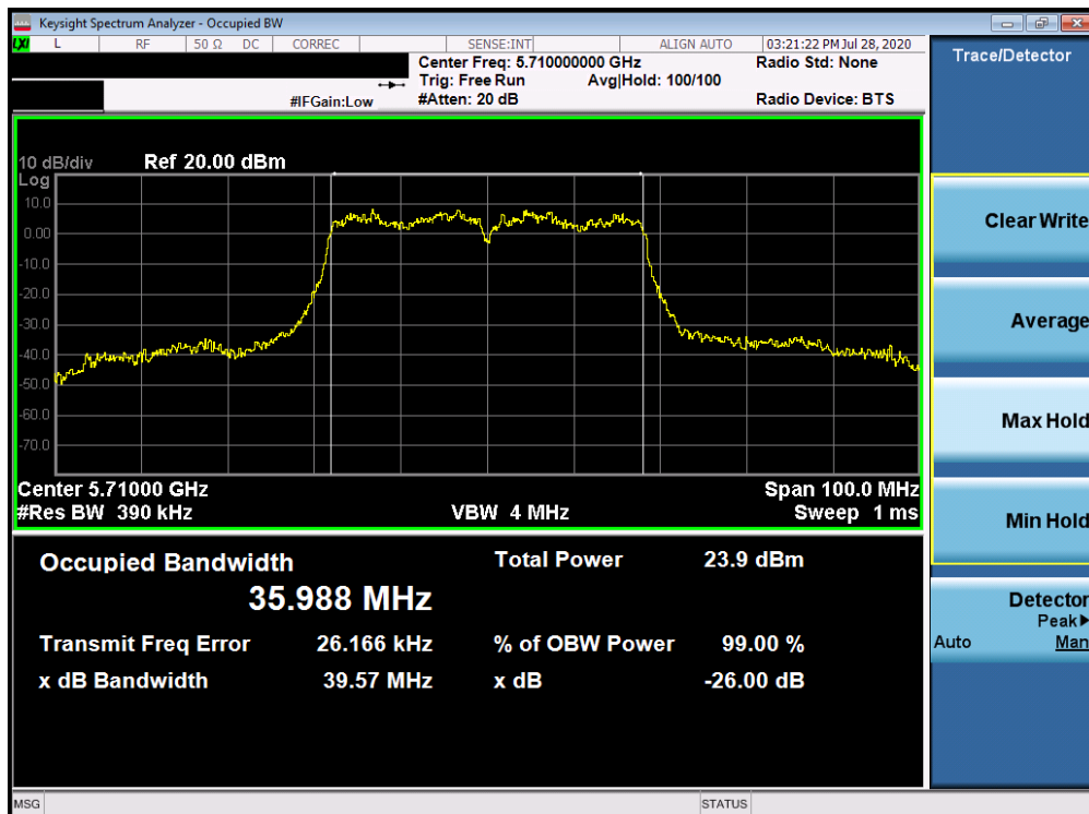
Plot 7-42. 26dB Bandwidth Plot ANT3 (40MHz BW 802.11n (UNII Band 2C) – Ch. 142)
