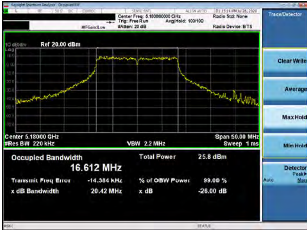
Plot 7-1. 26dB Bandwidth Plot ANT3 (802.11a (UNII Band 1) – Ch. 36)
