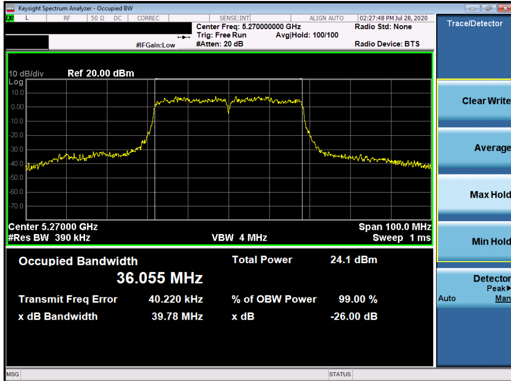
Plot 7-25. 26dB Bandwidth Plot ANT3 (40MHz BW 802.11n (UNII Band 2A) – Ch. 54)
