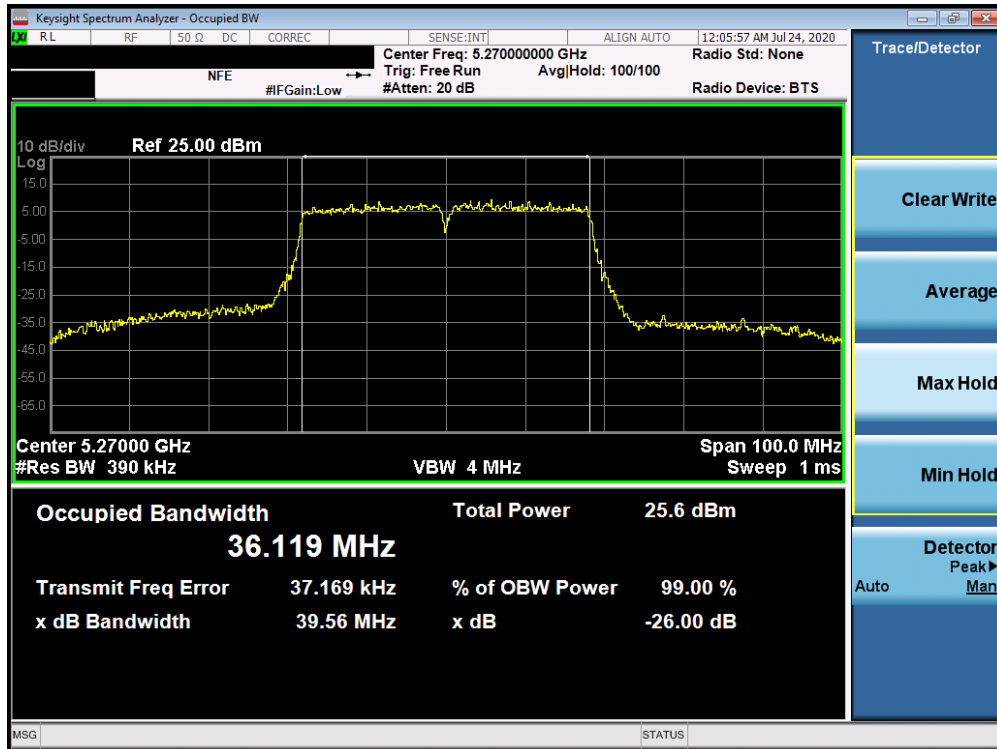
Plot 7-76. 26dB Bandwidth Plot ANT4 (40MHz BW 802.11n (UNII Band 2A) – Ch. 54)
