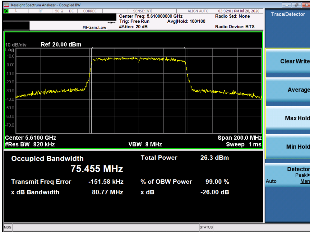
Plot 7-47. 26dB Bandwidth Plot ANT3 (80MHz BW 802.11ac (UNII Band 2C) – Ch. 122)
