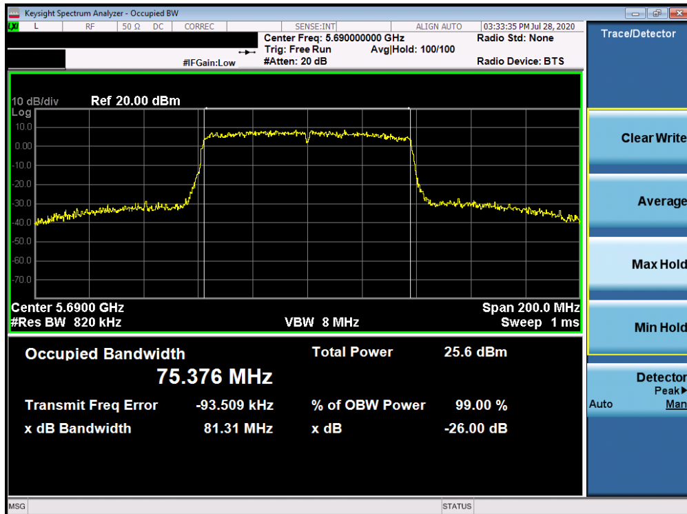
Plot 7-48. 26dB Bandwidth Plot ANT3 (80MHz BW 802.11ac (UNII Band 2C) – Ch. 138)
