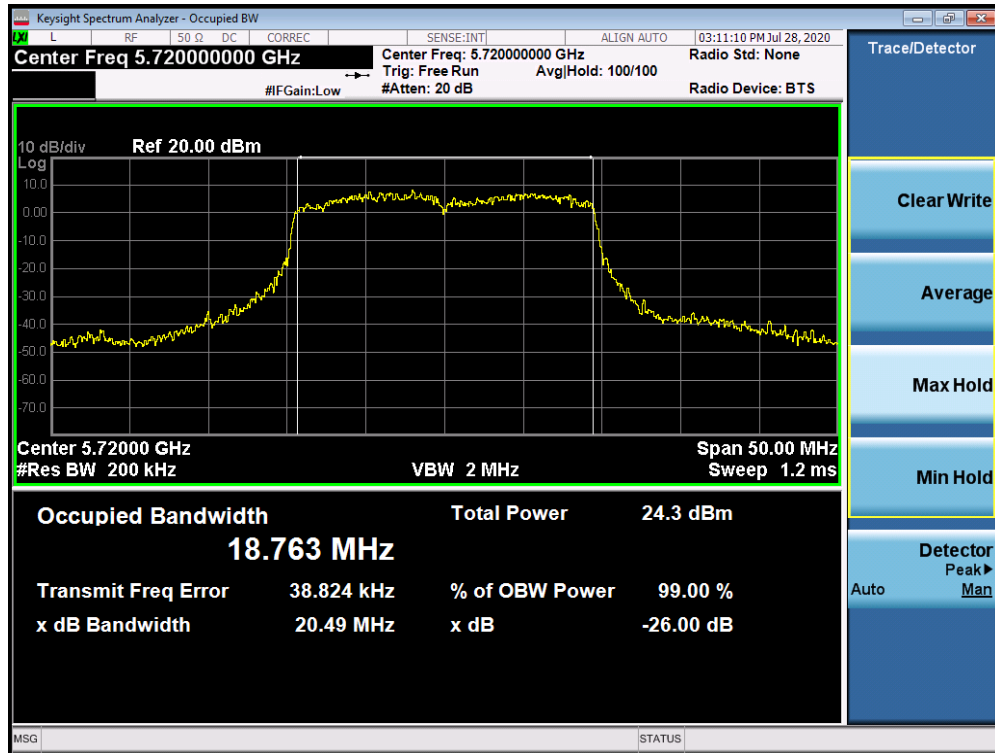
Plot 7-39. 26dB Bandwidth Plot ANT3 (20MHz BW 802.11ax (UNII Band 2C) – Ch. 144)
