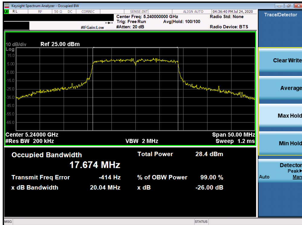
Plot 7-108. 26dB Bandwidth Plot ANT5 (20MHz BW 802.11n (UNII Band 1) – Ch. 48)
