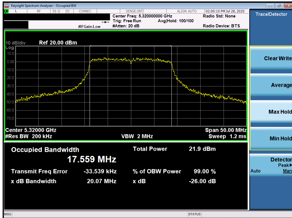
Plot 7-21. 26dB Bandwidth Plot ANT3 (20MHz BW 802.11n (UNII Band 2A) – Ch. 64)
