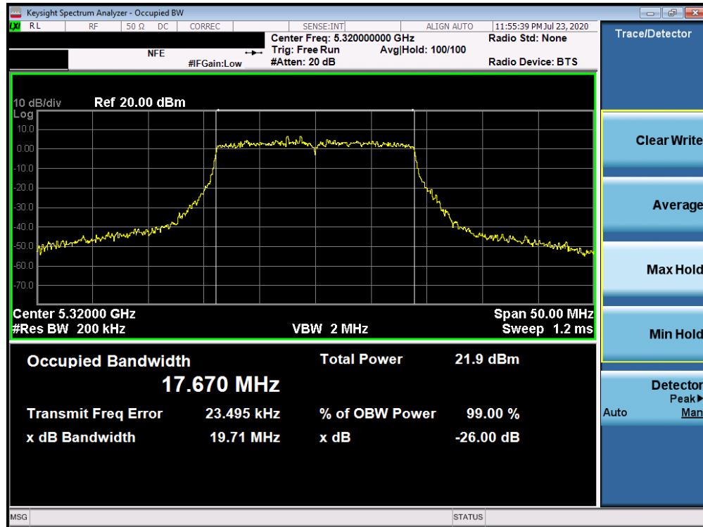
Plot 7-72. 26dB Bandwidth Plot ANT4 (20MHz BW 802.11n (UNII Band 2A) – Ch. 64)
