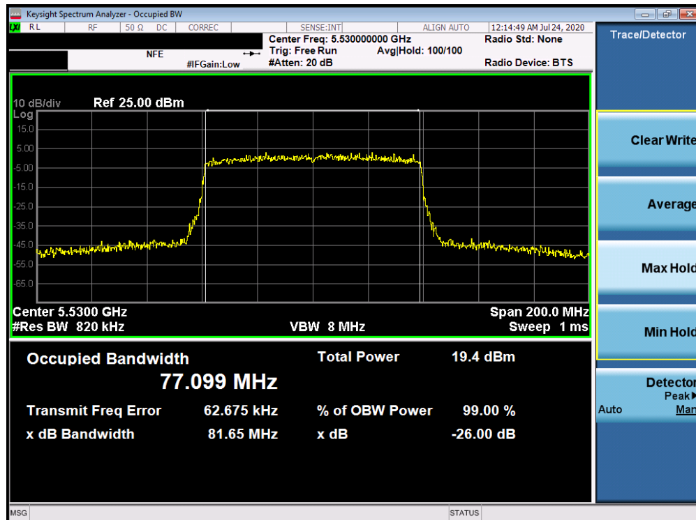
Plot 7-97. 26dB Bandwidth Plot ANT4 (80MHz BW 802.11ac (UNII Band 2C) – Ch. 106)
