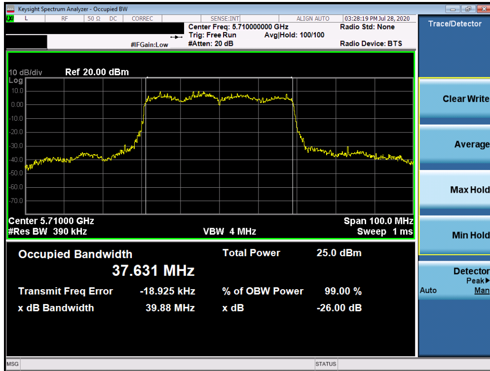
Plot 7-45. 26dB Bandwidth Plot ANT3 (40MHz BW 802.11ax (UNII Band 2C) – Ch. 142)
