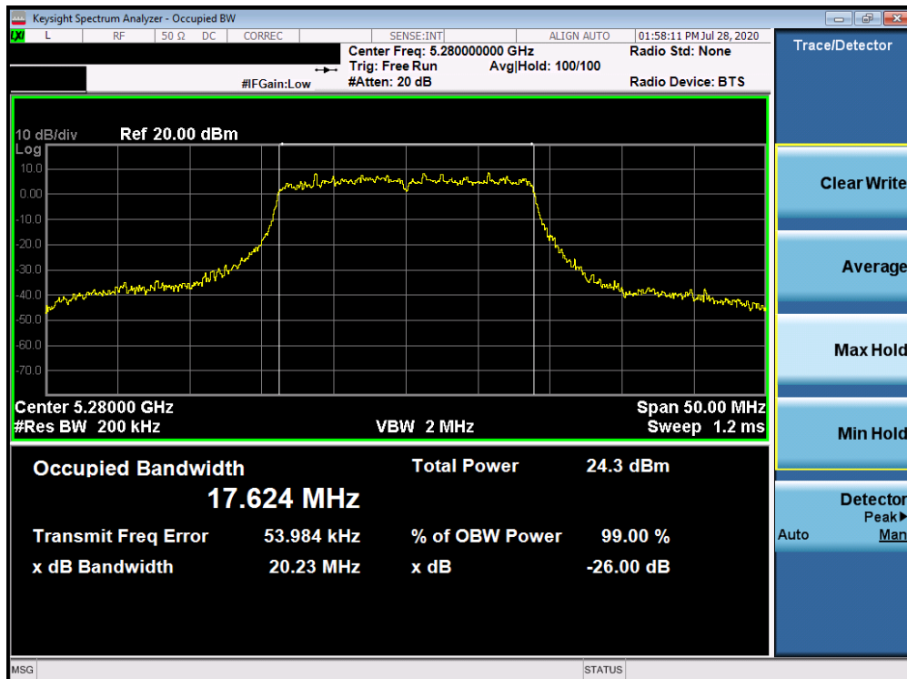
Plot 7-20. 26dB Bandwidth Plot ANT3 (20MHz BW 802.11n (UNII Band 2A) – Ch. 56)
