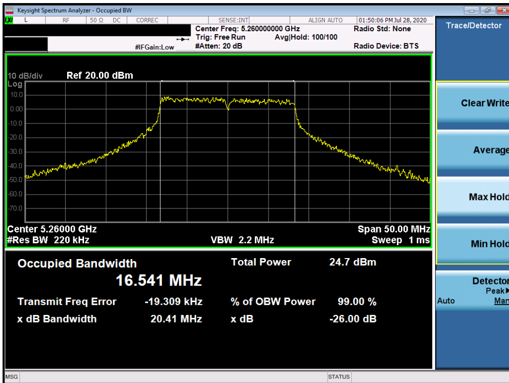
Plot 7-16. 26dB Bandwidth Plot ANT3 (802.11a (UNII Band 2A) – Ch. 52)
