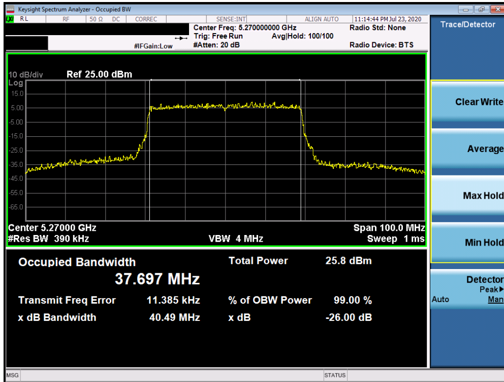
Plot 7-78. 26dB Bandwidth Plot ANT4 (40MHz BW 802.11ax (UNII Band 2a) – Ch. 54)
