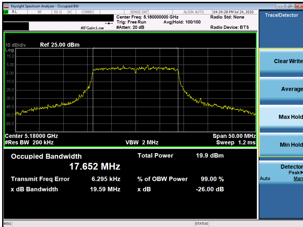
Plot 7-106. 26dB Bandwidth Plot ANT5 (20MHz BW 802.11n (UNII Band 1) – Ch. 36)
