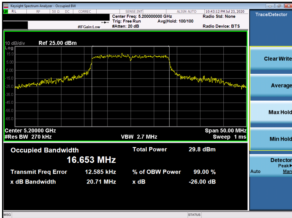
Plot 7-53. 26dB Bandwidth Plot ANT4 (802.11a (UNII Band 1) – Ch. 40)
