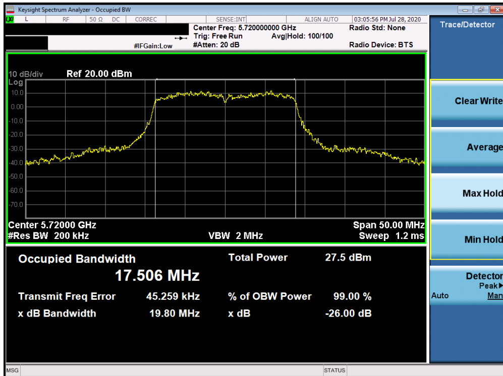
Plot 7-36. 26dB Bandwidth Plot ANT3 (20MHz BW 802.11n (UNII Band 2C) – Ch. 144)
