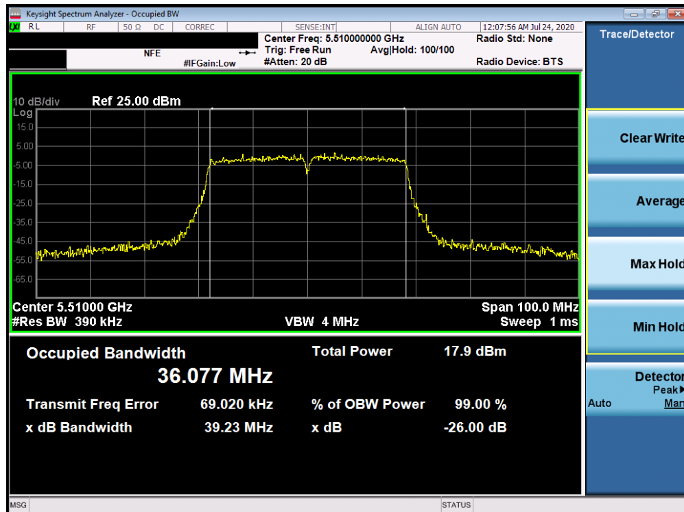
Plot 7-91. 26dB Bandwidth Plot ANT4 (40MHz BW 802.11n (UNII Band 2C) – Ch. 102)
