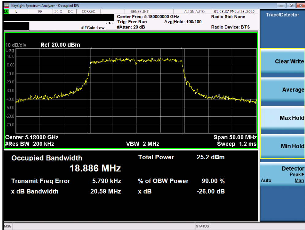
Plot 7-7. 26dB Bandwidth Plot ANT3 (20MHz BW 802.11ax (UNII Band 1) – Ch. 36)
