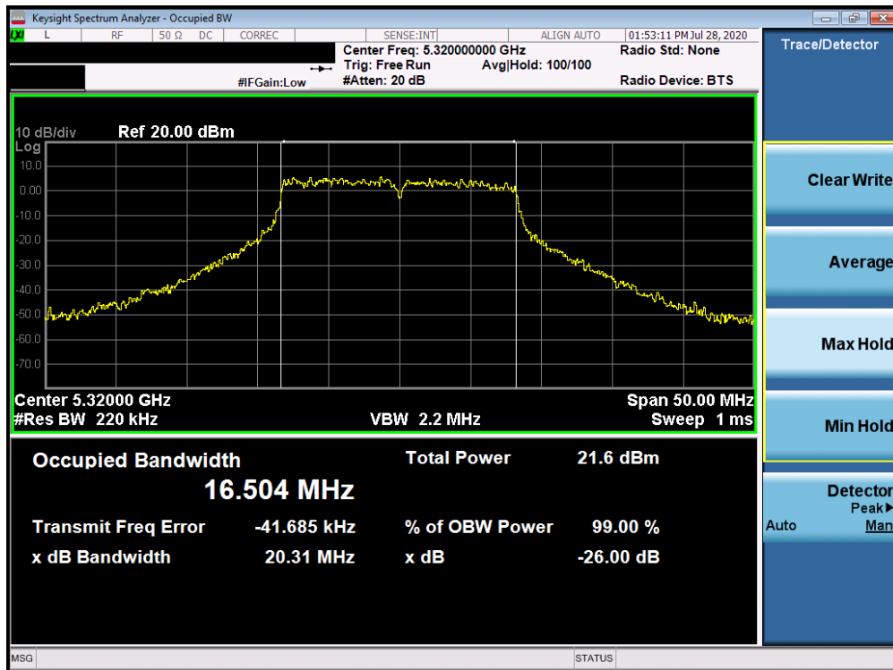
Plot 7-18. 26dB Bandwidth Plot ANT3 (802.11a (UNII Band 2A) – Ch. 64)
