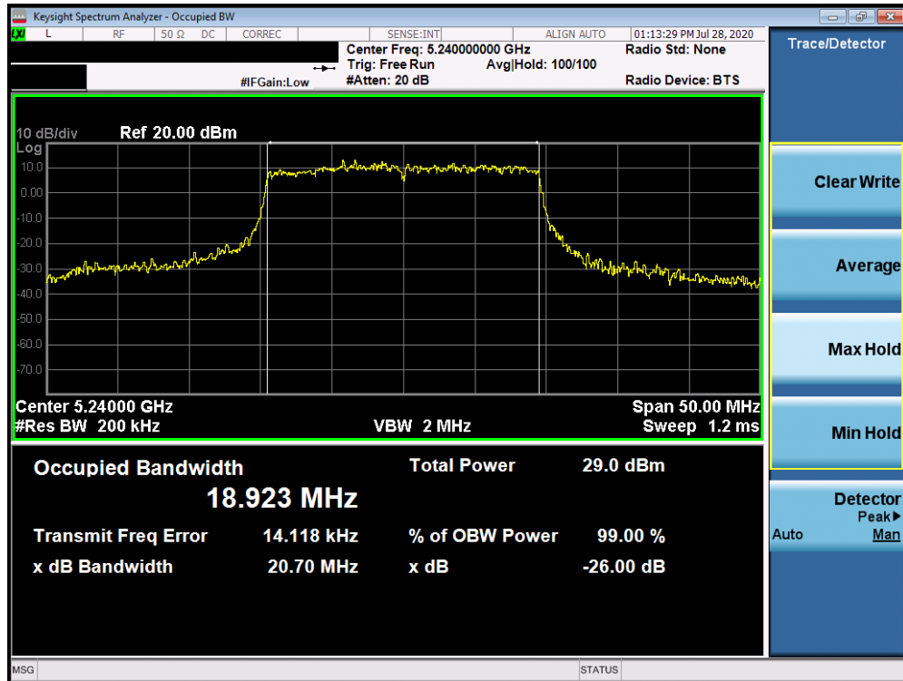
Plot 7-9. 26dB Bandwidth Plot ANT3 (20MHz BW 802.11ax (UNII Band 1) – Ch. 48)
