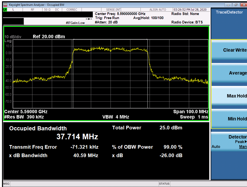
Plot 7-44. 26dB Bandwidth Plot ANT3 (40MHz BW 802.11ax (UNII Band 2C) – Ch. 118)
