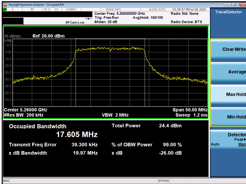
Plot 7-19. 26dB Bandwidth Plot ANT3 (20MHz BW 802.11n (UNII Band 2A) – Ch. 52)
