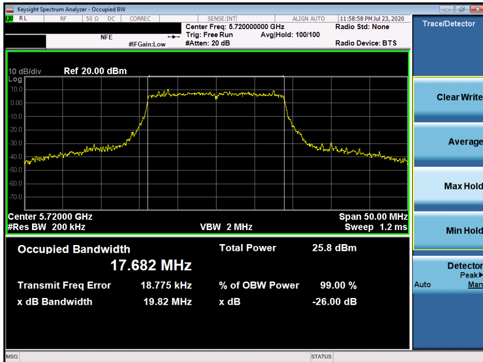
Plot 7-87. 26dB Bandwidth Plot ANT4 (20MHz BW 802.11n (UNII Band 2C) – Ch. 144)
