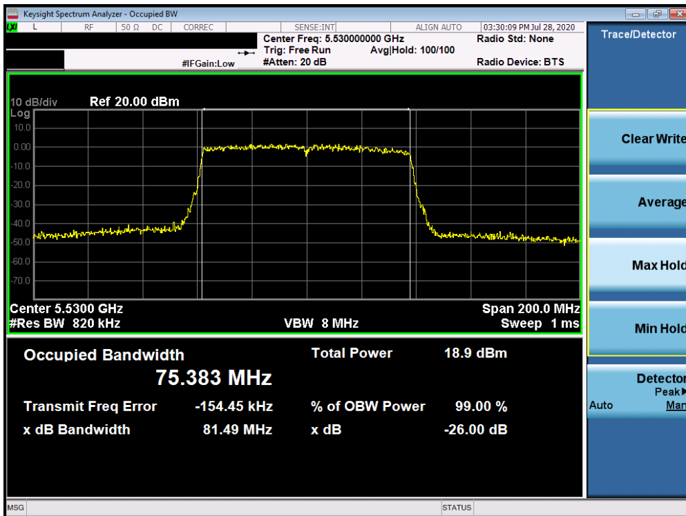
Plot 7-46. 26dB Bandwidth Plot ANT3 (80MHz BW 802.11ac (UNII Band 2C) – Ch. 106)
