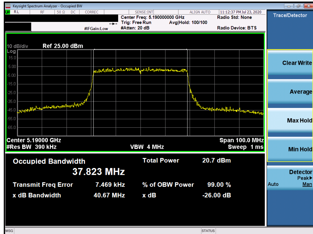
Plot 7-63. 26dB Bandwidth Plot ANT4 (40MHz BW 802.11ax (UNII Band 1) – Ch. 38)
