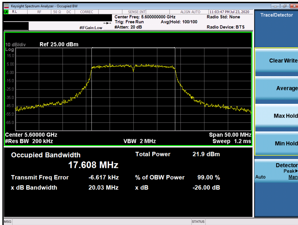
Plot 7-89. 26dB Bandwidth Plot ANT4 (20MHz BW 802.11ax (UNII Band 2C) – Ch. 120)
