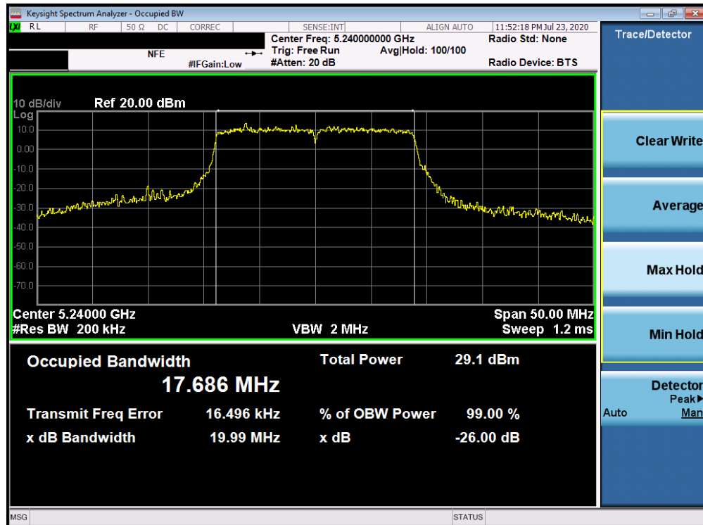
Plot 7-57. 26dB Bandwidth Plot ANT4 (20MHz BW 802.11n (UNII Band 1) – Ch. 48)
