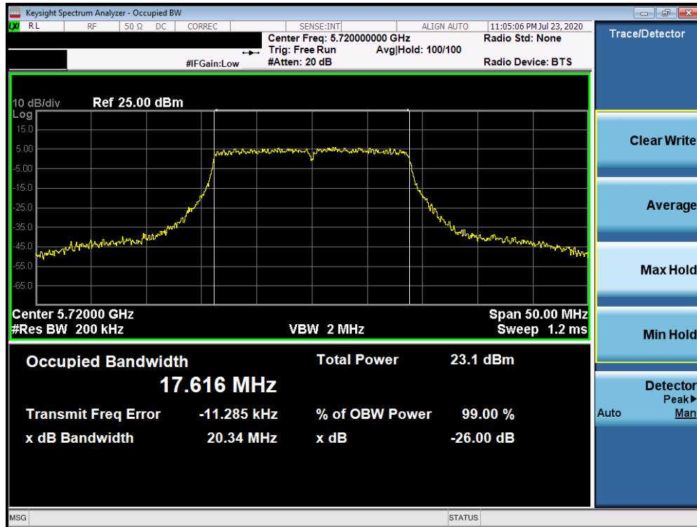
Plot 7-90. 26dB Bandwidth Plot ANT4 (20MHz BW 802.11ax (UNII Band 2C) – Ch. 144)
