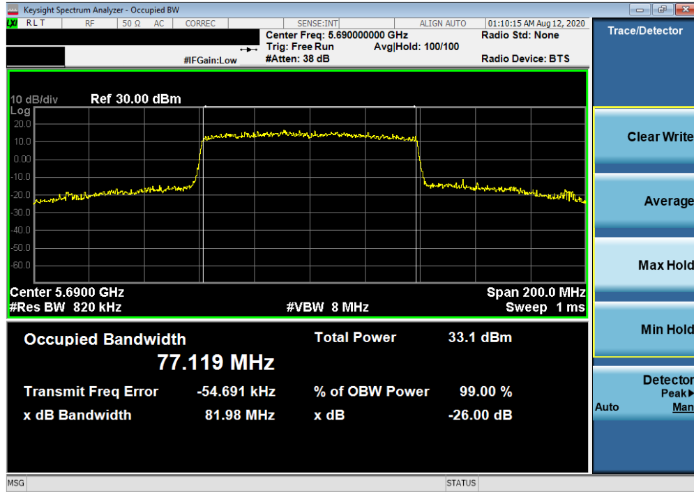
Plot 7-102. 26dB Bandwidth Plot ANT4 (80MHz BW 802.11ax (UNII Band 2C) – Ch. 138)
