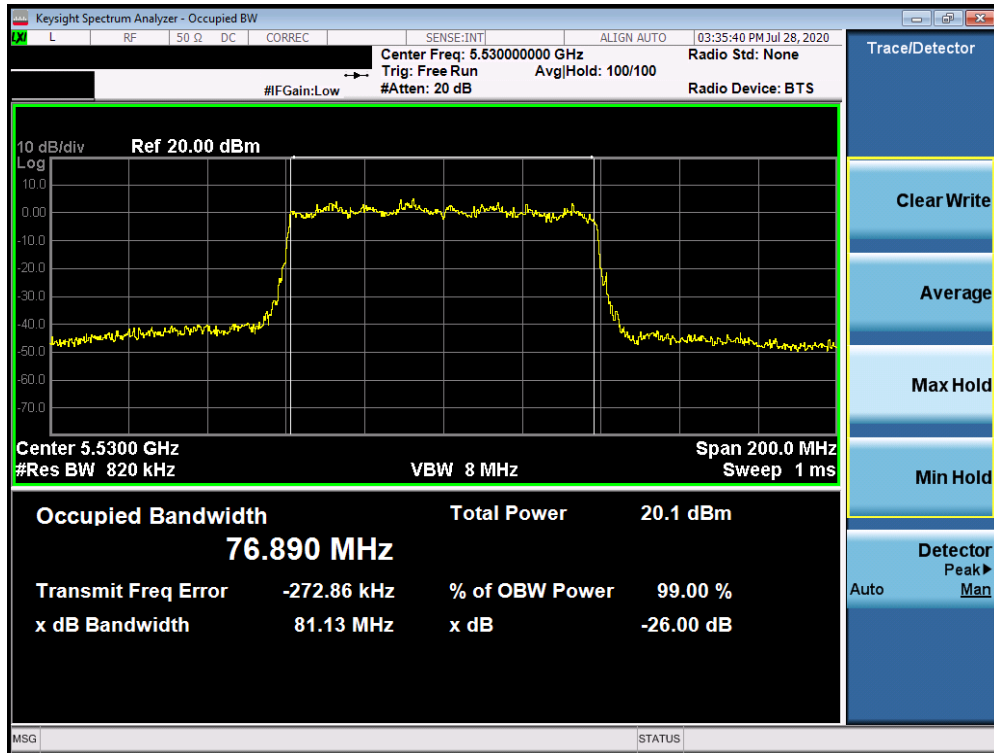
Plot 7-49. 26dB Bandwidth Plot ANT3 (80MHz BW 802.11ax (UNII Band 2C) – Ch. 106)
