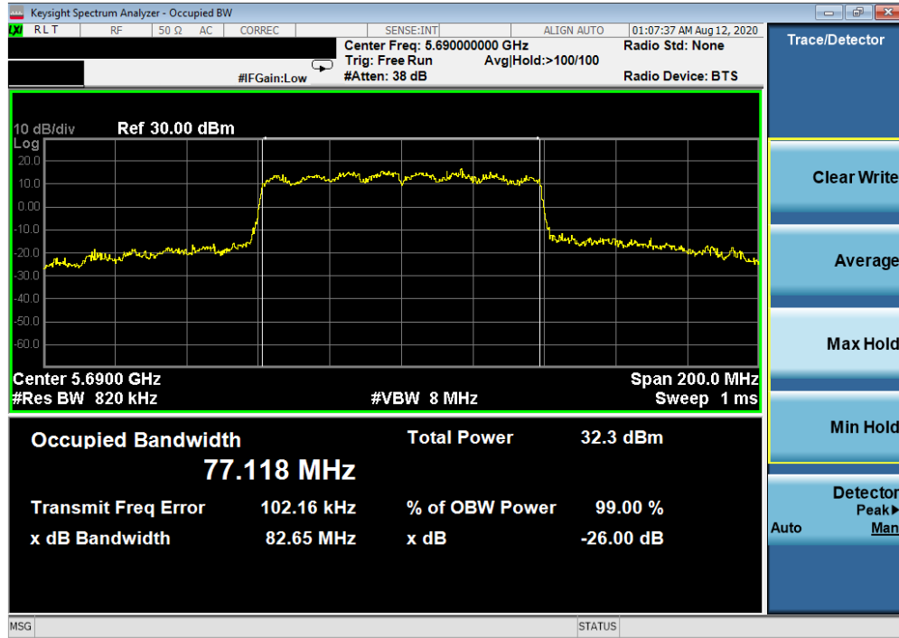
Plot 7-51. 26dB Bandwidth Plot ANT3 (80MHz BW 802.11ax (UNII Band 2C) – Ch. 138)
