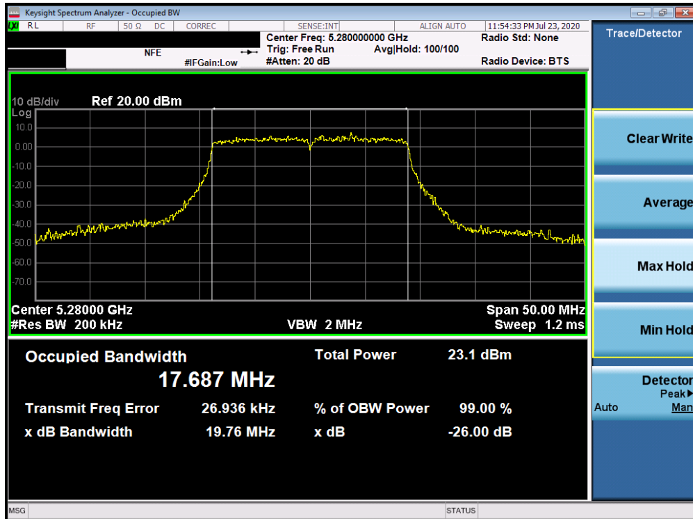
Plot 7-71. 26dB Bandwidth Plot ANT4 (20MHz BW 802.11n (UNII Band 2A) – Ch. 56)
