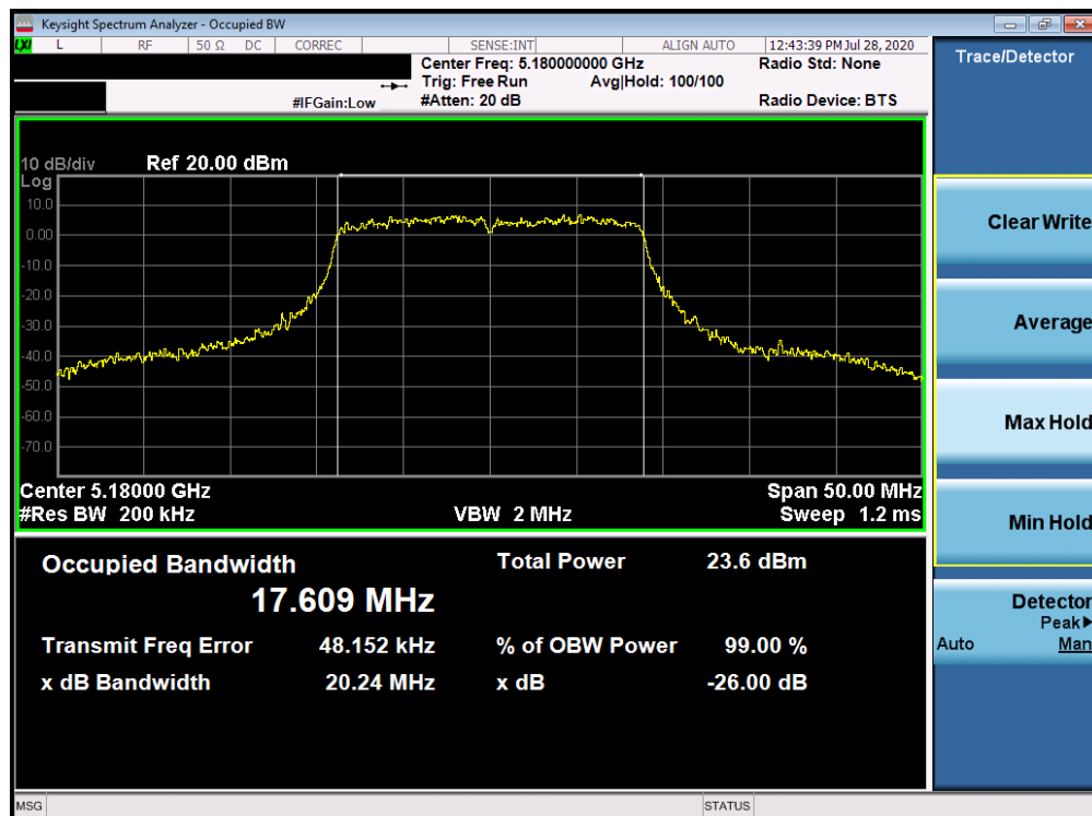
Plot 7-4. 26dB Bandwidth Plot ANT3 (20MHz BW 802.11n (UNII Band 1) – Ch. 36)
