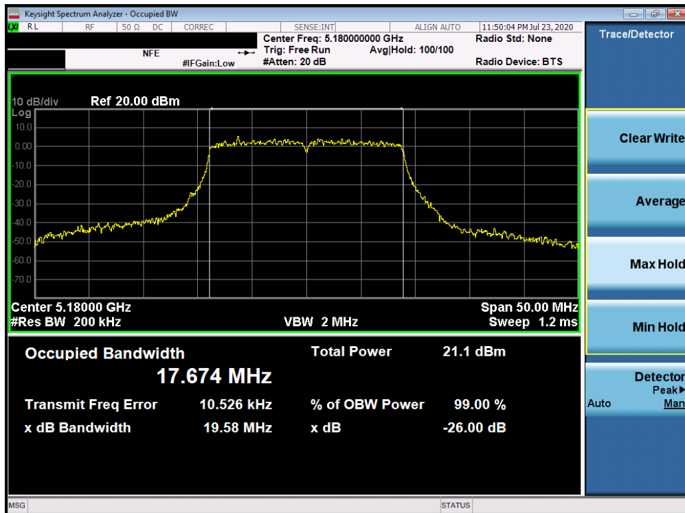
Plot 7-55. 26dB Bandwidth Plot ANT4 (20MHz BW 802.11n (UNII Band 1) – Ch. 36)
