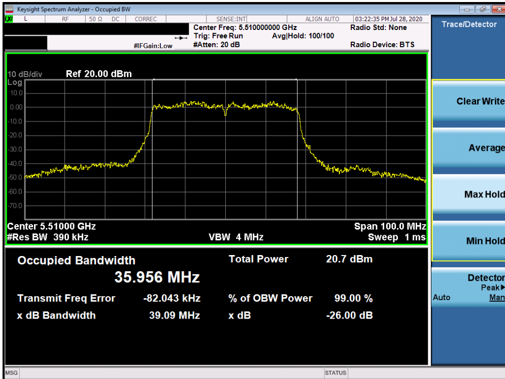
Plot 7-40. 26dB Bandwidth Plot ANT3 (40MHz BW 802.11n (UNII Band 2C) – Ch. 102)
