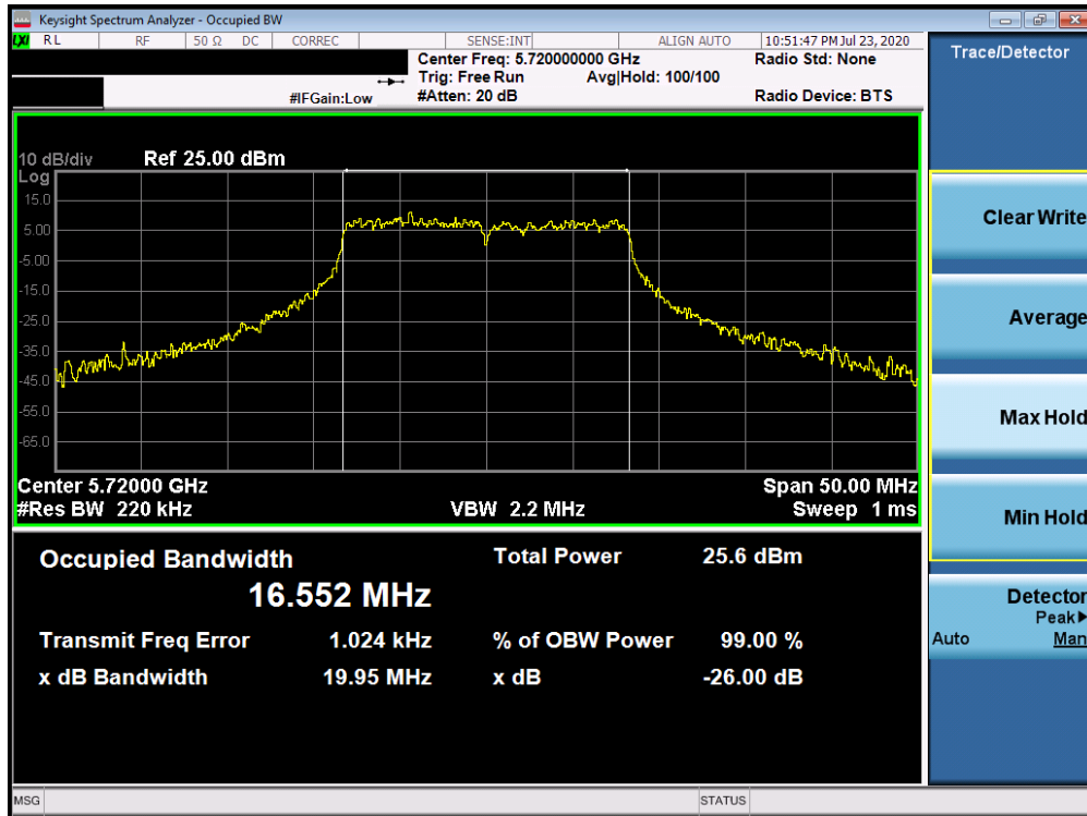
Plot 7-84. 26dB Bandwidth Plot ANT4 (802.11a (UNII Band 2C) – Ch. 144)
