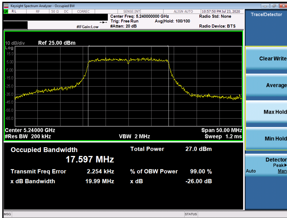
Plot 7-60. 26dB Bandwidth Plot ANT4 (20MHz BW 802.11ax (UNII Band 1) – Ch. 48)
