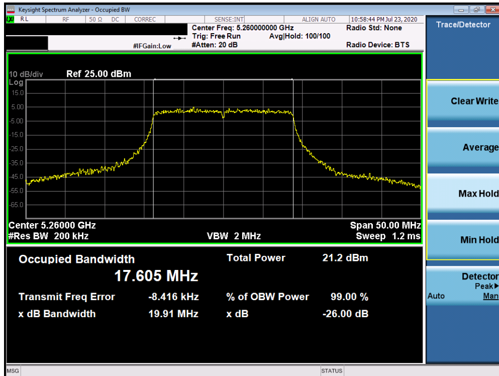
Plot 7-73. 26dB Bandwidth Plot ANT4 (20MHz BW 802.11ax (UNII Band 2A) – Ch. 52)
