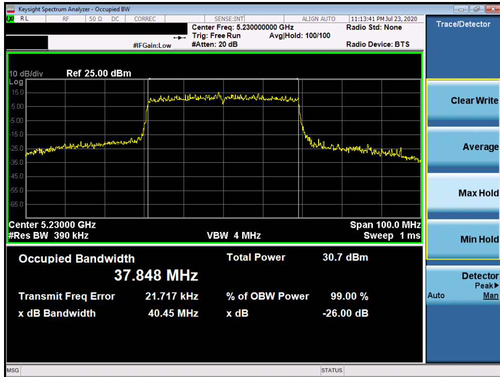
Plot 7-64. 26dB Bandwidth Plot ANT4 (40MHz BW 802.11ax (UNII Band 1) – Ch. 46)
