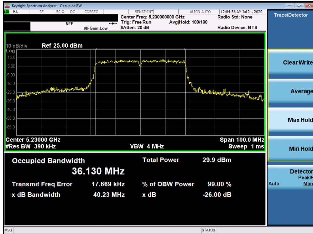
Plot 7-62. 26dB Bandwidth Plot ANT4 (40MHz BW 802.11n (UNII Band 1) – Ch. 46)
