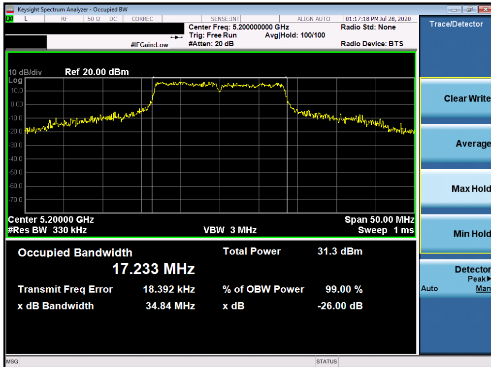
Plot 7-2. 26dB Bandwidth Plot ANT3 (802.11a (UNII Band 1) – Ch. 40)
