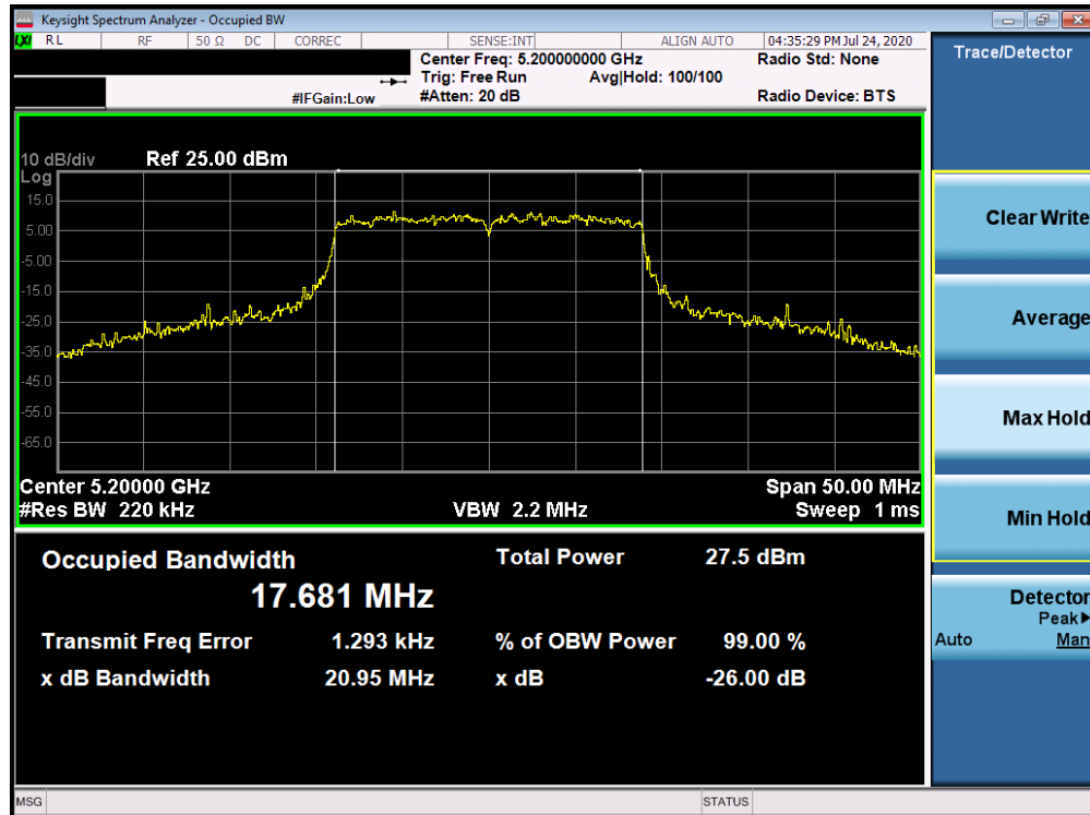
Plot 7-107. 26dB Bandwidth Plot ANT5 (20MHz BW 802.11n (UNII Band 1) – Ch. 40)
