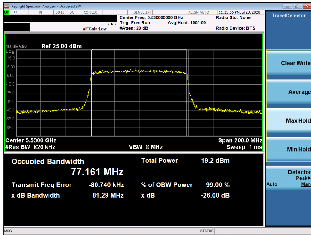
Plot 7-100. 26dB Bandwidth Plot ANT4 (80MHz BW 802.11ax (UNII Band 2C) – Ch. 106)
