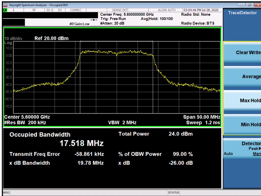
Plot 7-35. 26dB Bandwidth Plot ANT3 (20MHz BW 802.11n (UNII Band 2C) – Ch. 120)
