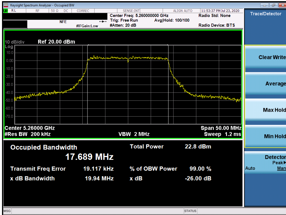
Plot 7-70. 26dB Bandwidth Plot ANT4 (20MHz BW 802.11n (UNII Band 2A) – Ch. 52)
