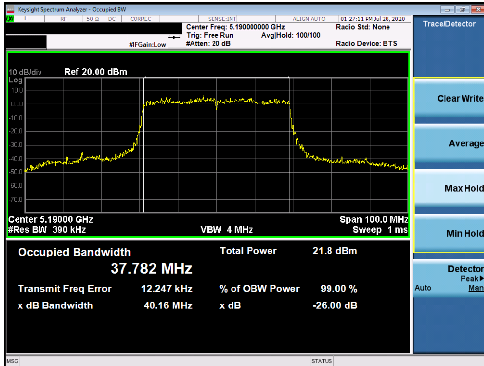
Plot 7-12. 26dB Bandwidth Plot ANT3 (40MHz BW 802.11ax (UNII Band 1) – Ch. 38)
