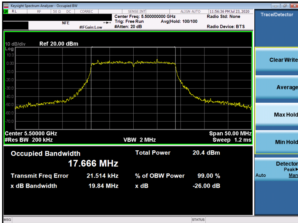
Plot 7-85. 26dB Bandwidth Plot ANT4 (20MHz BW 802.11n (UNII Band 2C) – Ch. 100)
