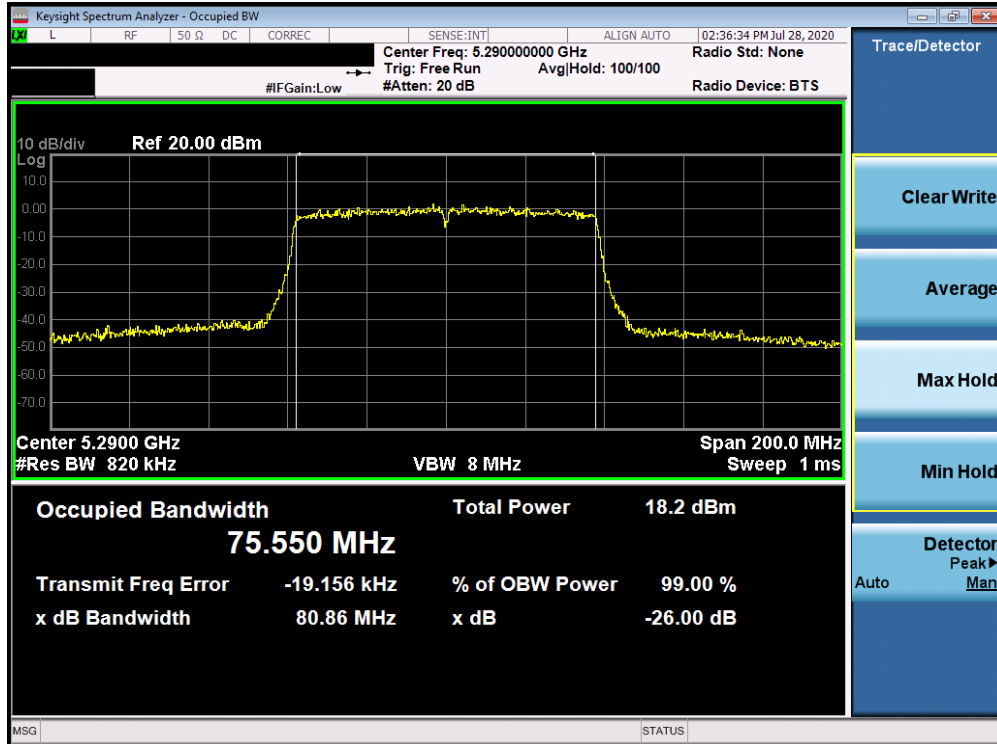
Plot 7-29. 26dB Bandwidth Plot ANT3 (80MHz BW 802.11ac (UNII Band 2A) – Ch. 58)
