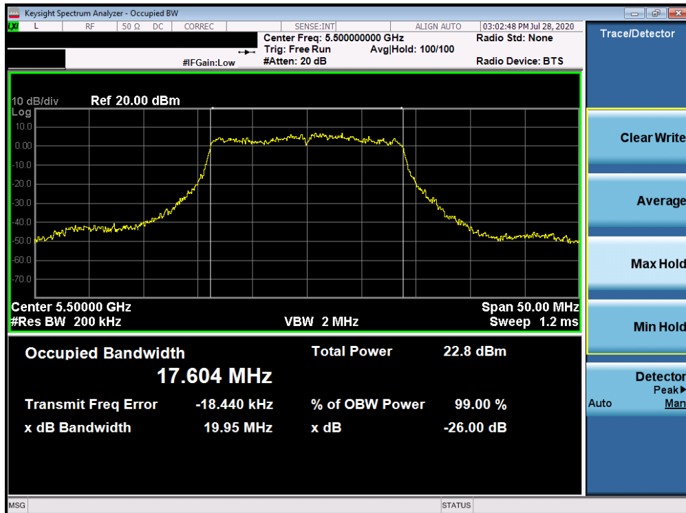
Plot 7-34. 26dB Bandwidth Plot ANT3 (20MHz BW 802.11n (UNII Band 2C) – Ch. 100)
