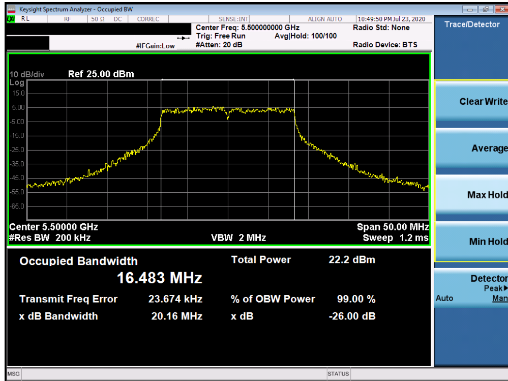
Plot 7-82. 26dB Bandwidth Plot ANT4 (802.11a (UNII Band 2C) – Ch. 100)
