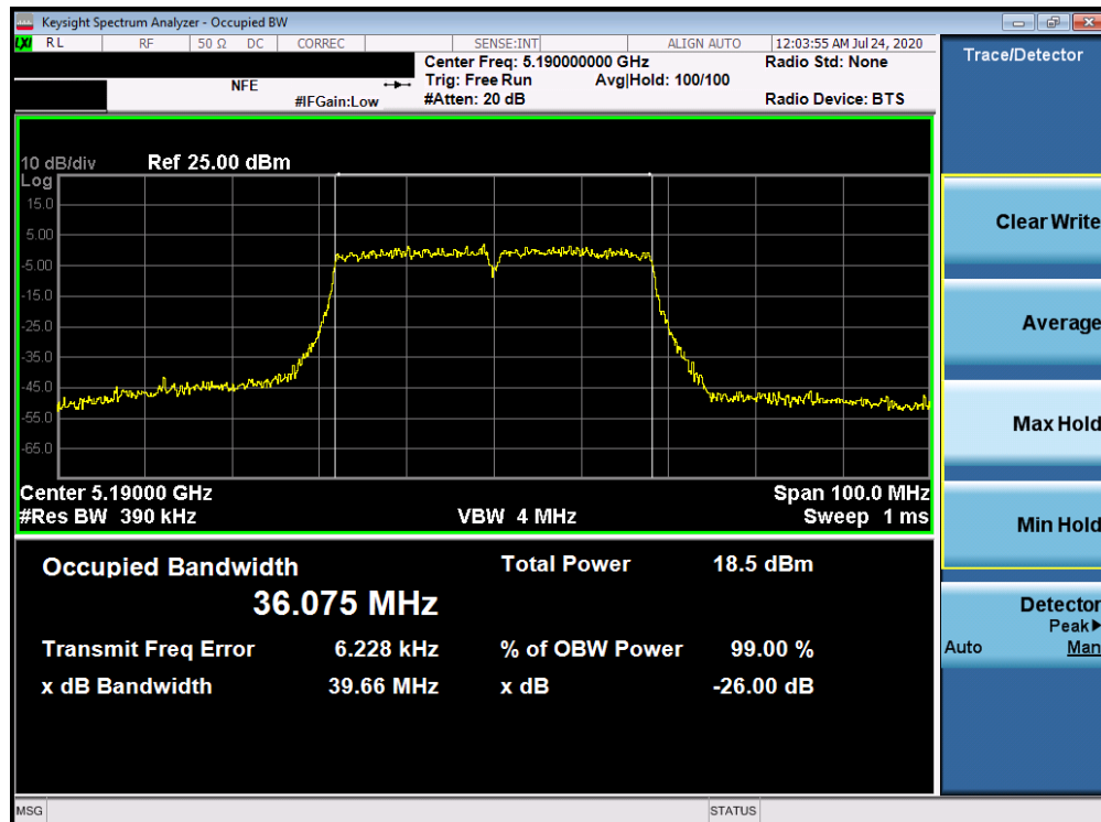
Plot 7-61. 26dB Bandwidth Plot ANT4 (40MHz BW 802.11n (UNII Band 1) – Ch. 38)
