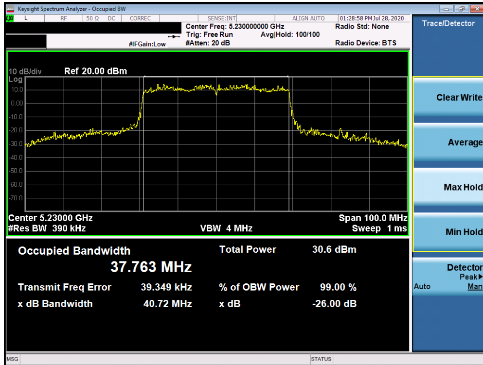
Plot 7-13. 26dB Bandwidth Plot ANT3 (40MHz BW 802.11ax (UNII Band 1) – Ch. 46)
