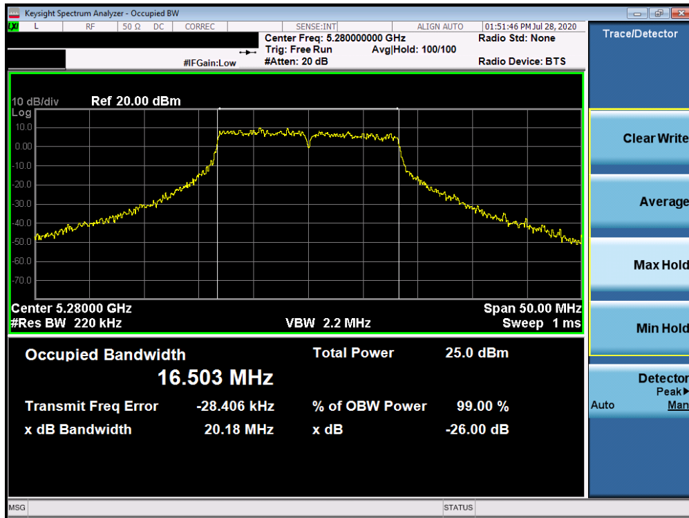
Plot 7-17. 26dB Bandwidth Plot ANT3 (802.11a (UNII Band 2A) – Ch. 56)
