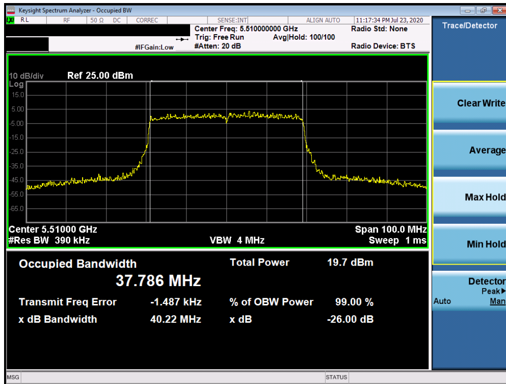
Plot 7-94. 26dB Bandwidth Plot ANT4 (40MHz BW 802.11ax (UNII Band 2C) – Ch. 102)
