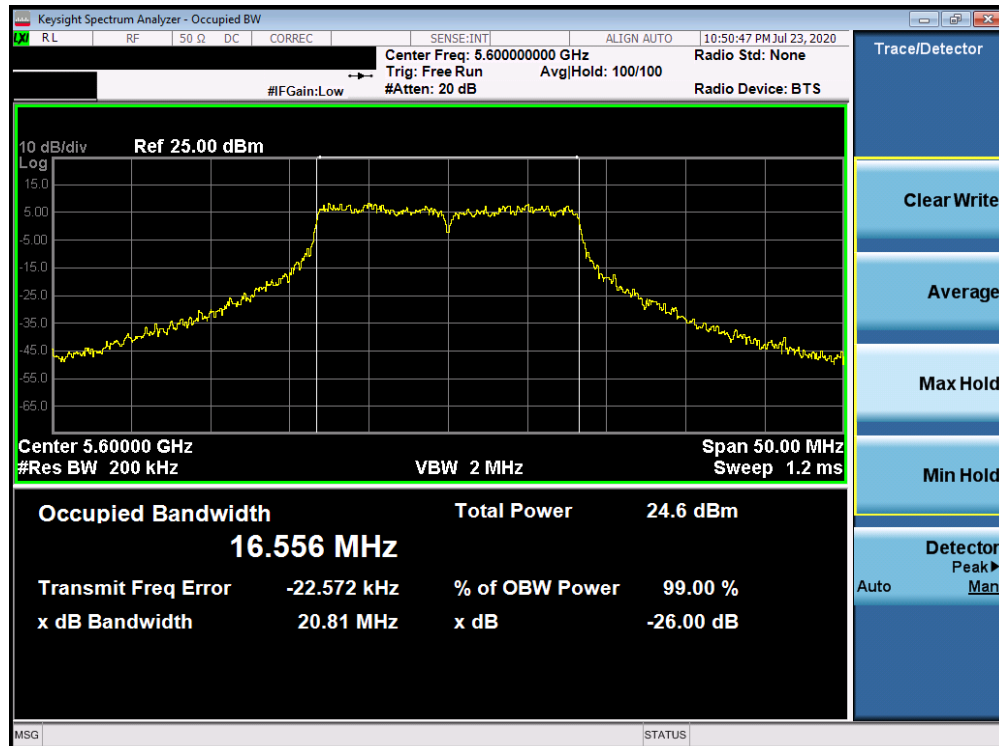
Plot 7-83. 26dB Bandwidth Plot ANT4 (802.11a (UNII Band 2C) – Ch. 120)
