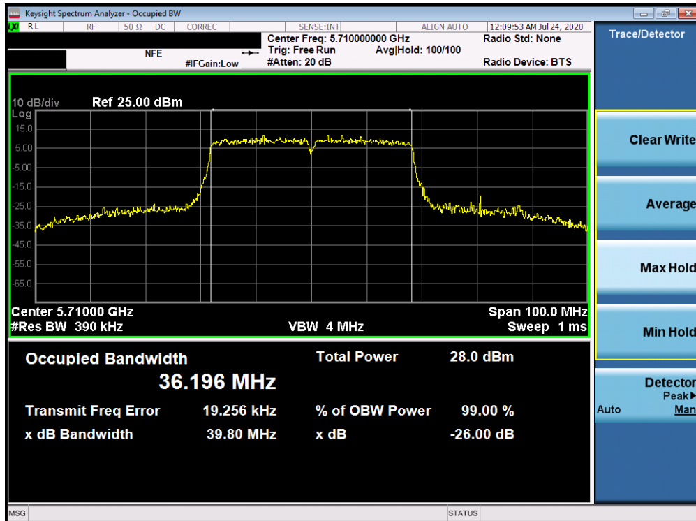
Plot 7-93. 26dB Bandwidth Plot ANT4 (40MHz BW 802.11n (UNII Band 2C) – Ch. 142)
