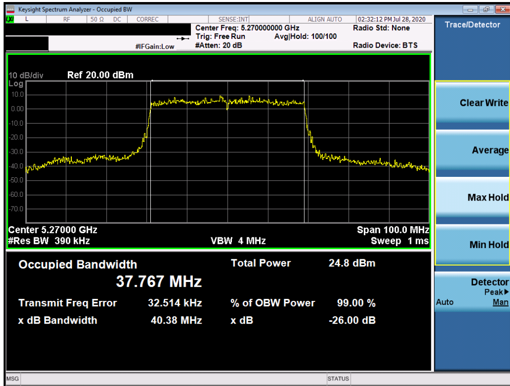
Plot 7-27. 26dB Bandwidth Plot ANT3 (40MHz BW 802.11ax (UNII Band 2A) – Ch. 54)
