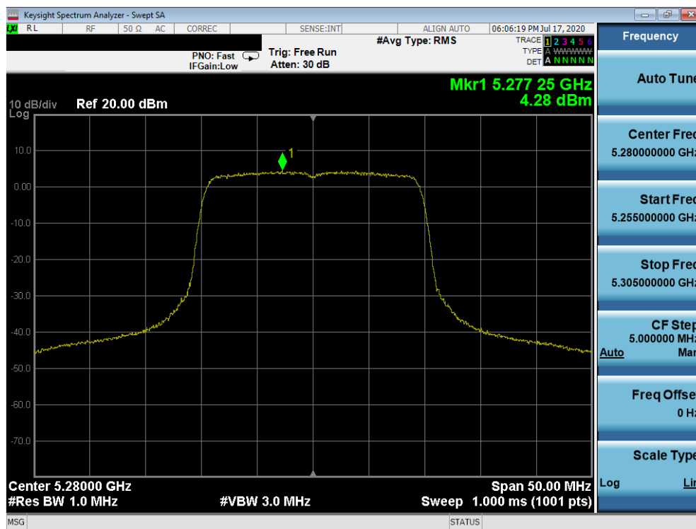
Plot 7-393. Power Spectral Density Plot ANT5 (20MHz BW 802.11ax (UNII Band 2A) – Ch. 56)
