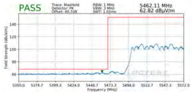
Plot 7-577. Radiated Lower Band Edge Plot MIMO (Peak – UNII Band 2C)
