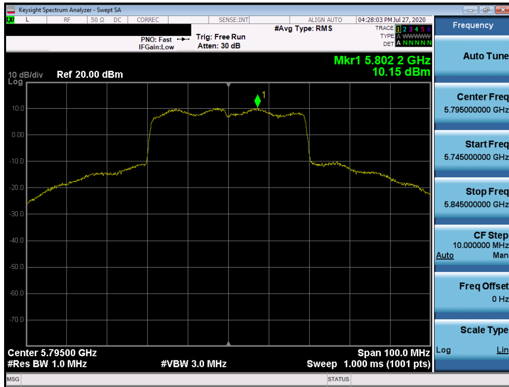
Plot 7-501. Power Spectral Density Plot ANT3 (40MHz BW 802.11ax (UNII Band 3) – Ch. 159)
