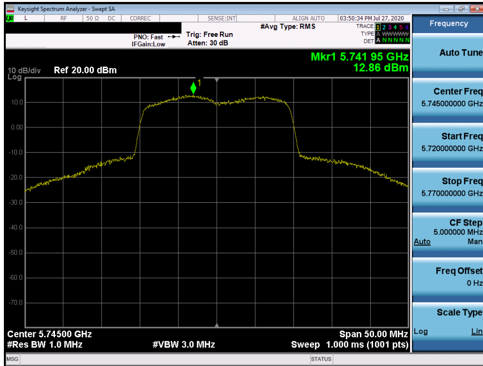
Plot 7-495. Power Spectral Density Plot ANT3 (20MHz BW 802.11ax (UNII Band 3) – Ch. 149)
