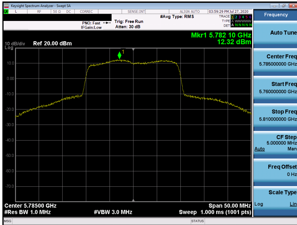
Plot 7-496. Power Spectral Density Plot ANT3 (20MHz BW 802.11ax (UNII Band 3) – Ch. 157)
