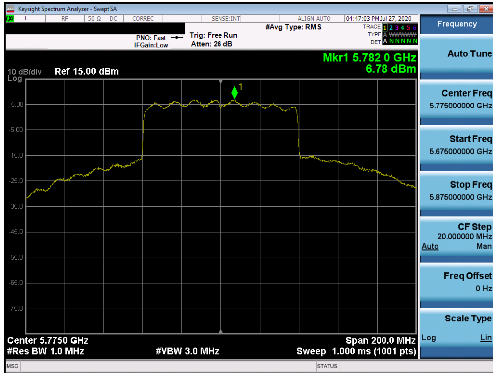
Plot 7-503. Power Spectral Density Plot ANT3 (80MHz BW 802.11ax (UNII Band 3) – Ch. 155)
