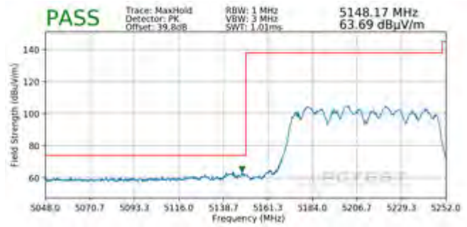
Plot 7-573. Radiated Lower Band Edge Plot MIMO (Peak – UNII Band 1)
