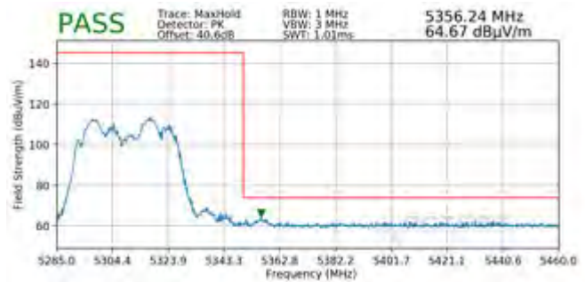
Plot 7-568. Radiated Upper Band Edge Plot MIMO (Peak – UNII Band 2A)
