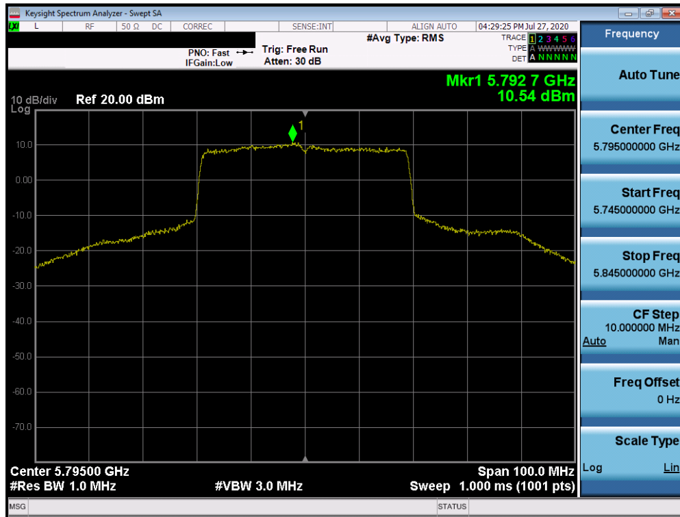
Plot 7-516. Power Spectral Density Plot ANT4 (40MHz BW 802.11ax (UNII Band 3) – Ch. 159)
