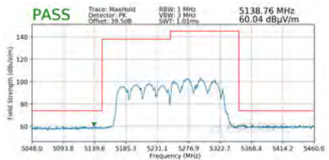
Plot 7-580. Radiated Lower Band Edge Plot MIMO (Peak – UNII Band 1)
