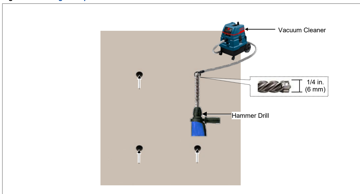
Figure 16. Drilling Example
