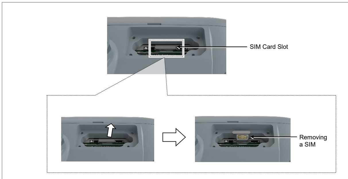
Figure 8. Replacing SIM (2)
