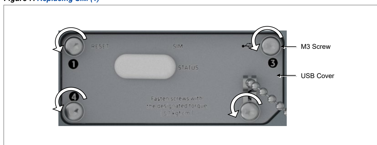
Figure 7. Replacing SIM (1)
