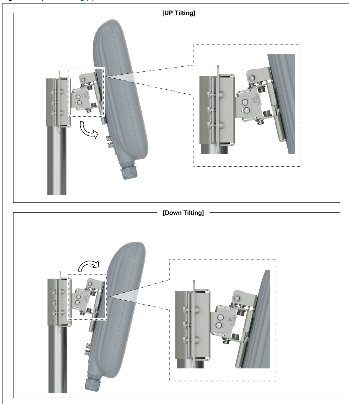
Figure 21. System Tilting (2)
