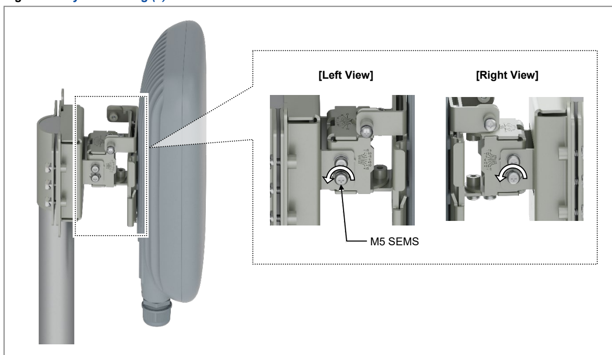
Figure 20. System Tilting (1)
