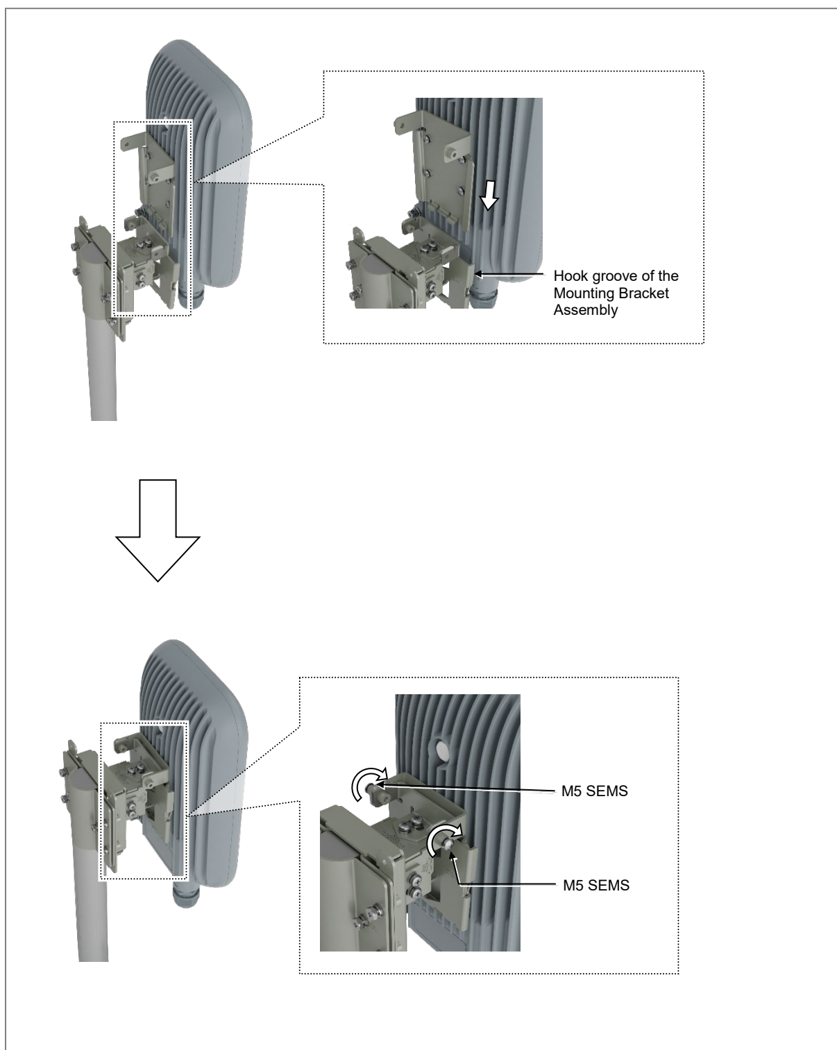
Figure 13. Fixing CPE Outdoor on the Pole Mounting Bracket Assembly
