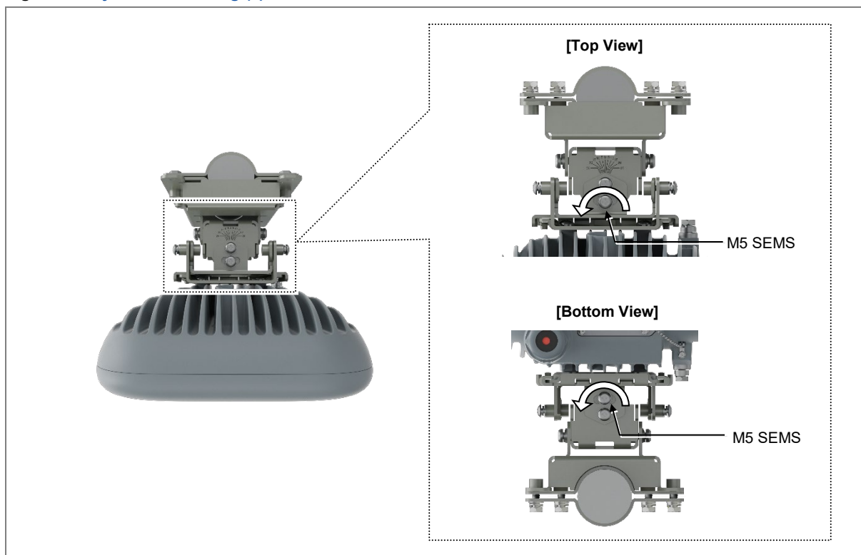
Figure 23. System Swivelling (1)
