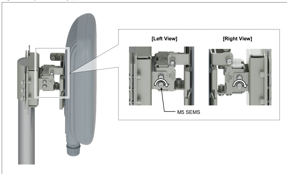
Figure 22. System Tilting (3)
