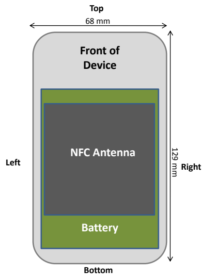
Figure F-1 DUT Antenna Locations
