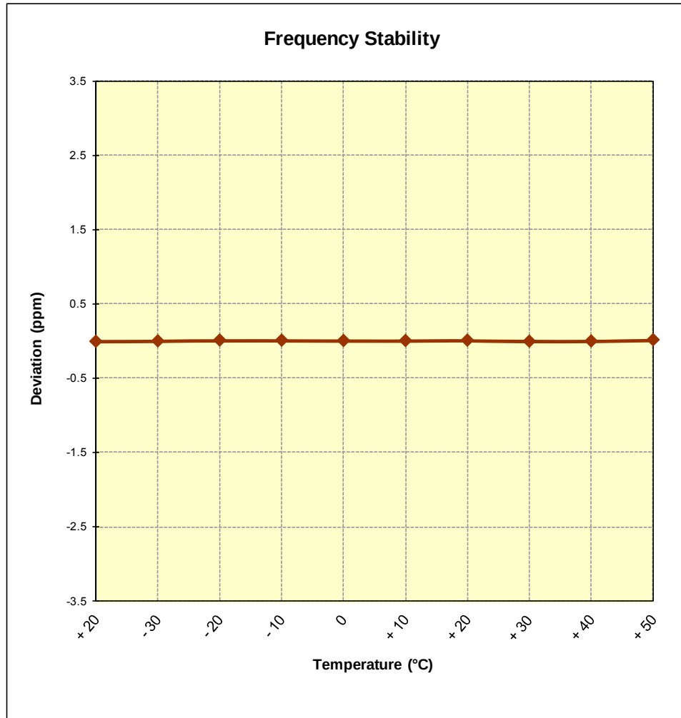
Figure 6-11. Frequency Stability Graph (PCS WCDMA Mode – Ch. 9400)
