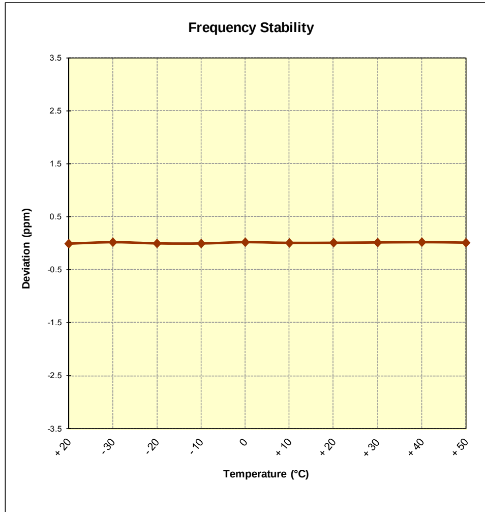
Figure 6-10. Frequency Stability Graph (PCS GSM Mode – Ch. 661)
