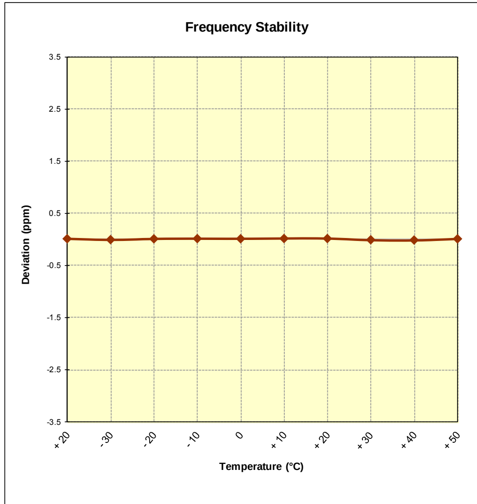
Figure 6-9. Frequency Stability Graph (AWS WCDMA Mode – Ch. 1412)
