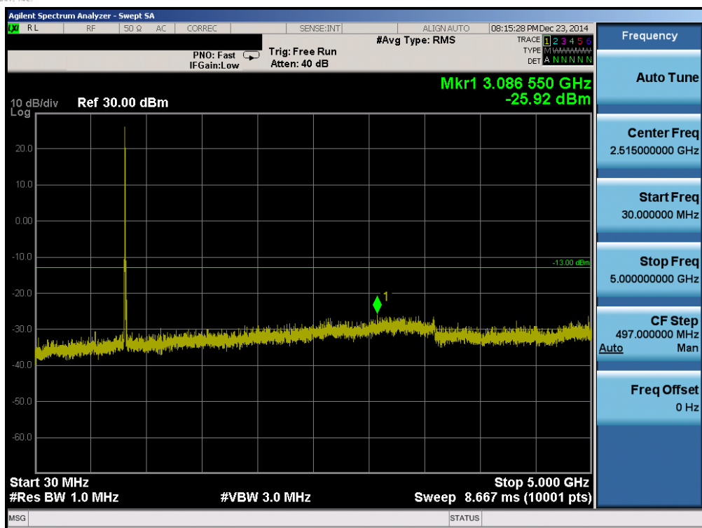
Plot 6-33. Conducted Spurious Plot (Band 5 – 10.0MHz QPSK – RB Size 1, RB Offset 0 – Mid Channel)
