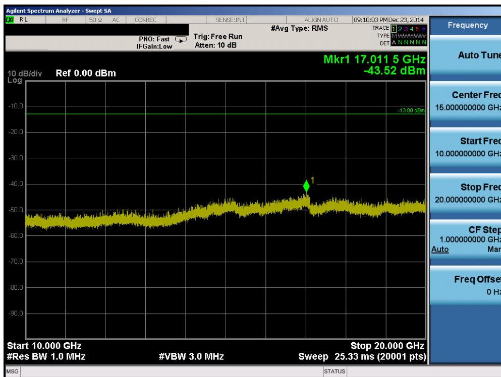
Plot 6-40. Conducted Spurious Plot (Band 4 – 20.0MHz QPSK – RB Size 1, RB Offset 0 – Mid Channel)
