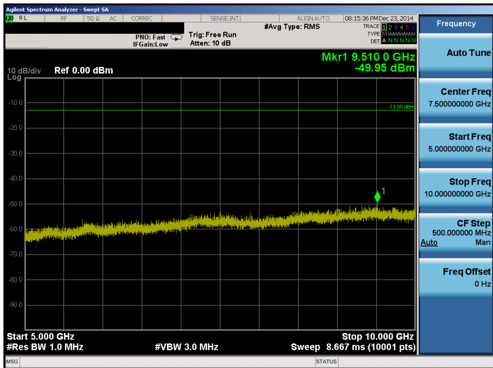
Plot 6-34. Conducted Spurious Plot (Band 5 – 10.0MHz QPSK – RB Size 1, RB Offset 0 – Mid Channel)
