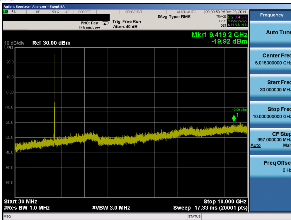
Plot 6-39. Conducted Spurious Plot (Band 4 – 20.0MHz QPSK – RB Size 1, RB Offset 0 – Mid Channel)
