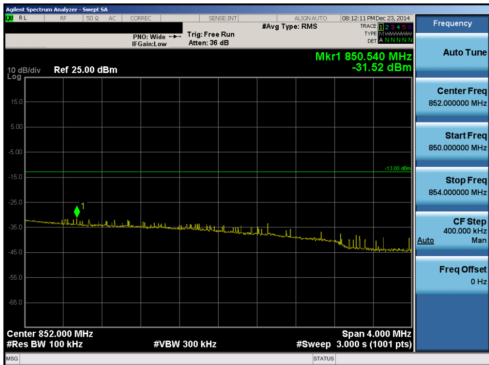
Plot 6-58. Upper Extended Band Edge Plot (Band 5 - 5.0MHz QPSK - RB Size 25)
