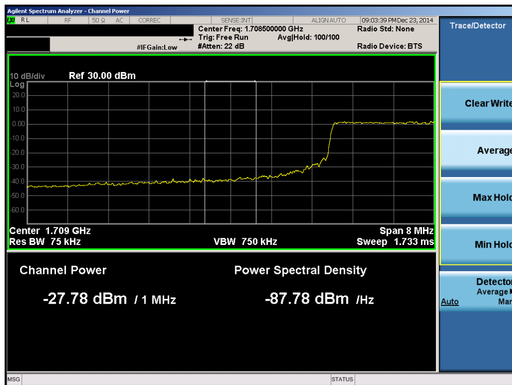
Plot 6-66. Lower Extended Band Edge Plot (Band 4 – 10.0MHz QPSK – RB Size 50)
