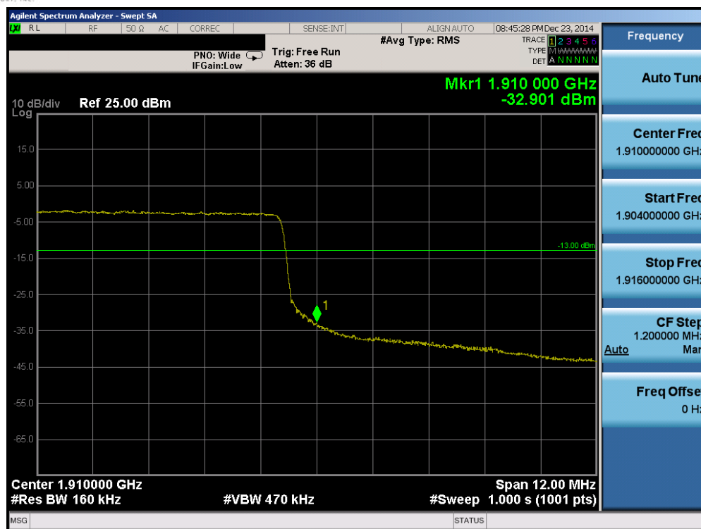
Plot 6-87. Upper Band Edge Plot (Band 2 – 15.0MHz QPSK – RB Size 75)
