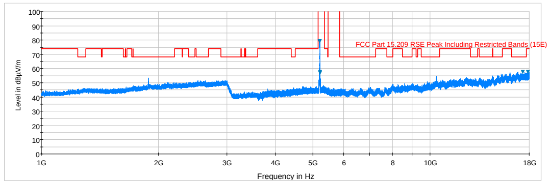
Plot 6-68. Radiated Spurious Plot above 1GHz (802.11a – U1 Ch. 40, Ant. Pol. V)
