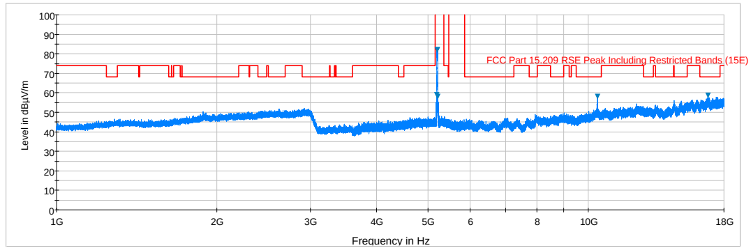
Plot 6-67. Radiated Spurious Plot above 1GHz (802.11a – U1 Ch. 40, Ant. Pol. H)
