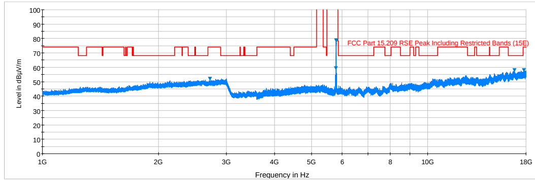
Plot 6-73. Radiated Spurious Plot above 1GHz (802.11a – U3 Ch. 157, Ant. Pol. H)
