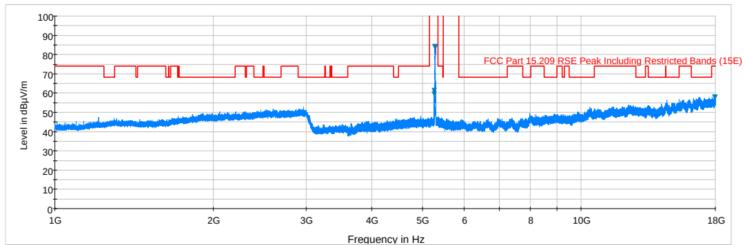
Plot 6-69. Radiated Spurious Plot above 1GHz (802.11a – U2A Ch. 56, Ant. Pol. H)
