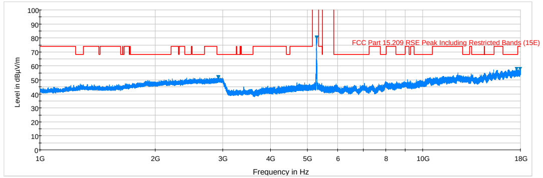
Plot 6-70. Radiated Spurious Plot above 1GHz (802.11a – U2A Ch. 56, Ant. Pol. V)
