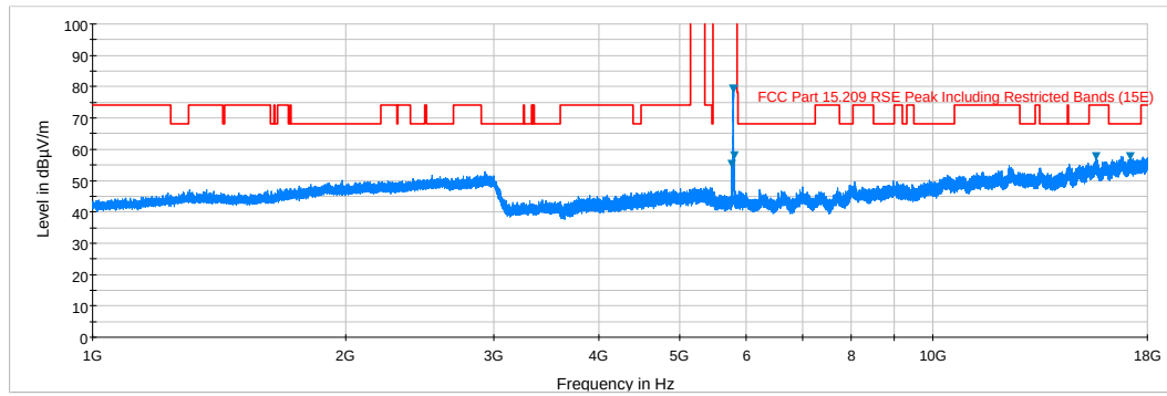
Plot 6-74. Radiated Spurious Plot above 1GHz (802.11a – U3 Ch. 157, Ant. Pol. V)
