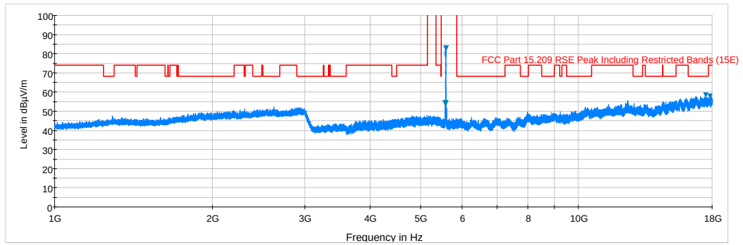
Plot 6-71. Radiated Spurious Plot above 1GHz (802.11a – U2C Ch. 116, Ant. Pol. H)
