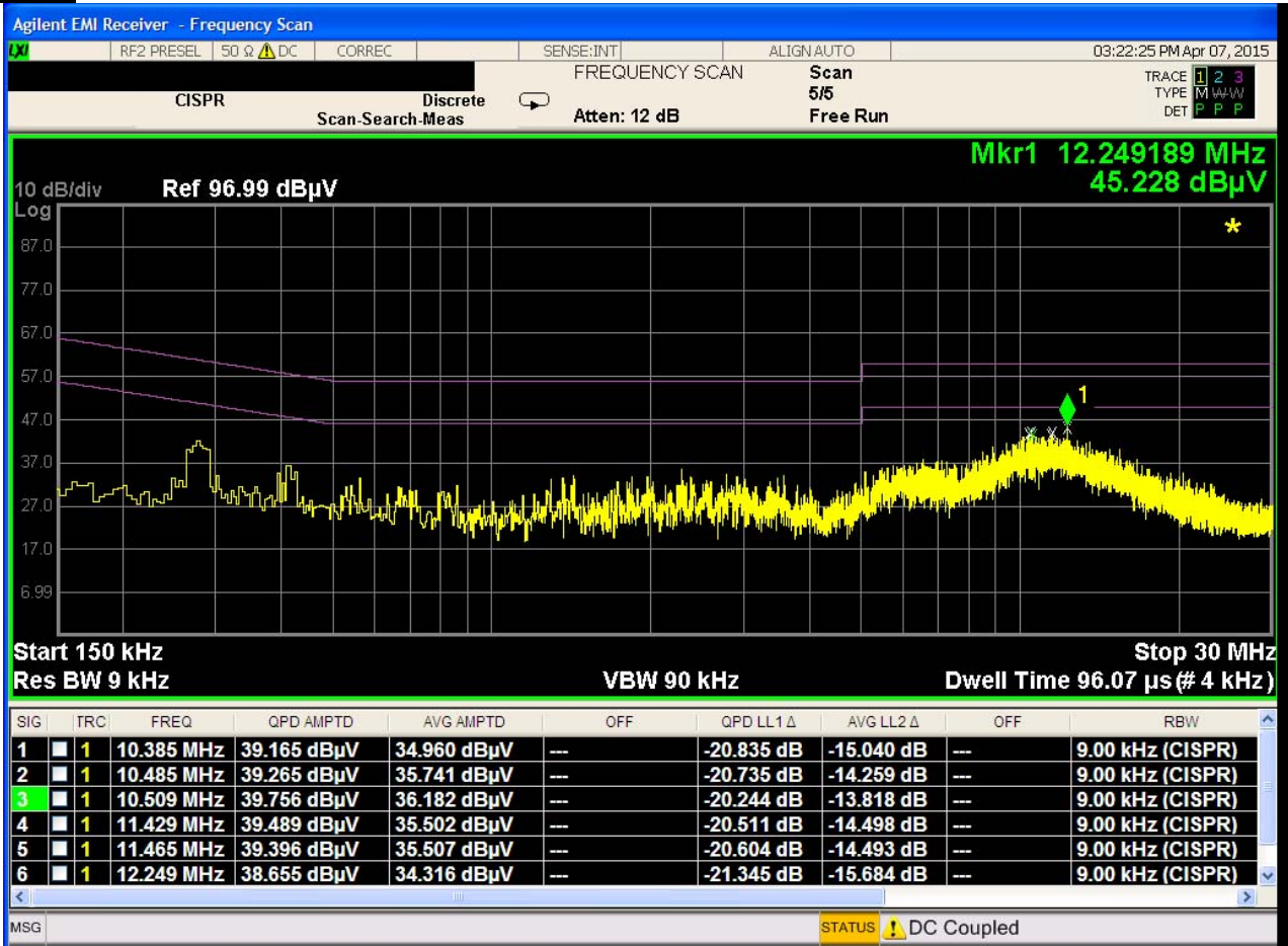
Plot 6-99. Line Conducted Plot with 802.11a UNII Band 2C (L1)
