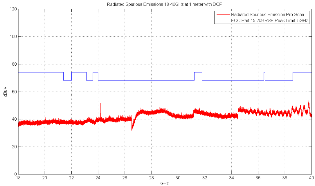
Plot 6-75. Radiated Spurious Plot above 18GHz (802.11a – Ant. Pol. H)
