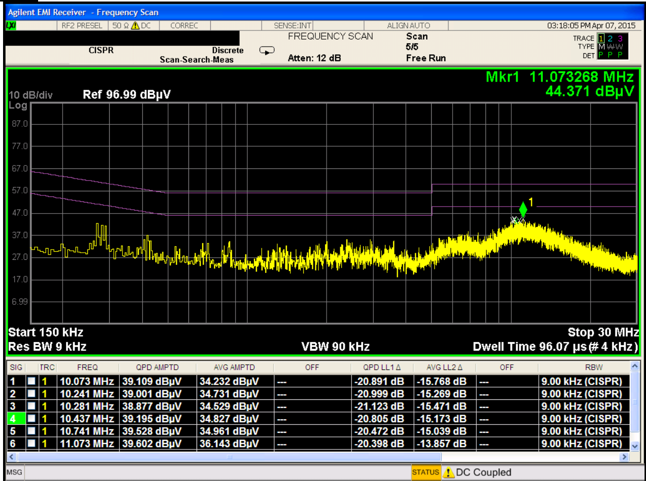
Plot 6-97. Line Conducted Plot with 802.11a UNII Band 2A (L1)
