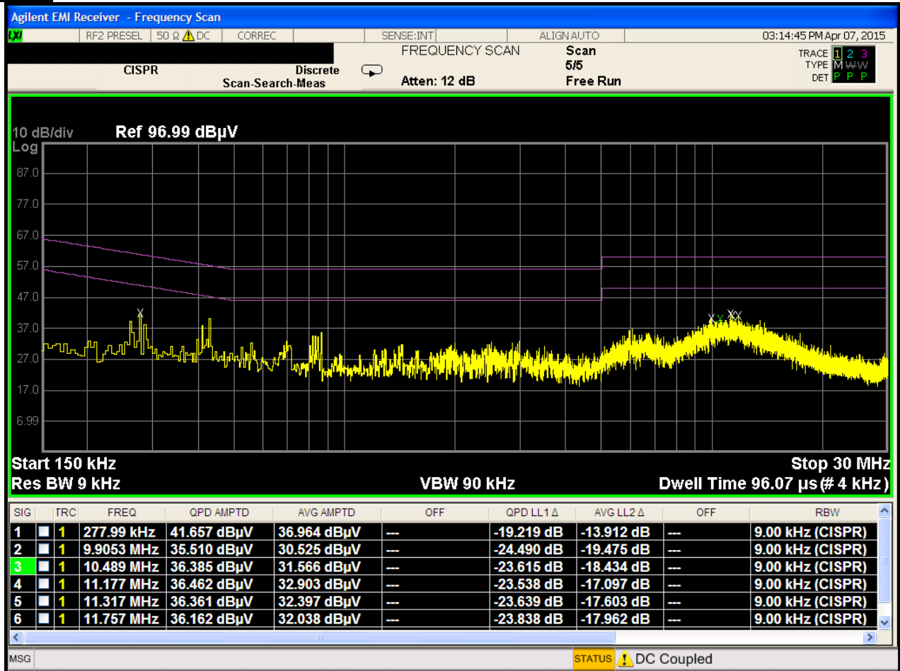
Plot 6-98. Line Conducted Plot with 802.11a UNII Band 2A (N)
