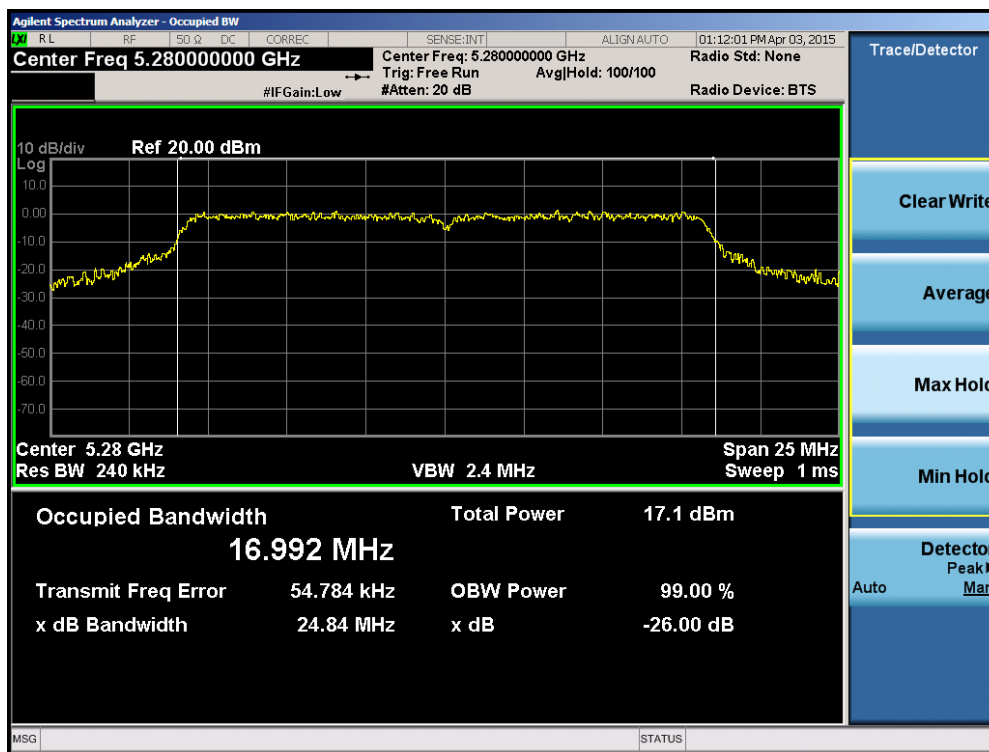
Plot 6-10. 26dB Bandwidth Plot (802.11a (UNII Band 2A) – Ch. 56)
