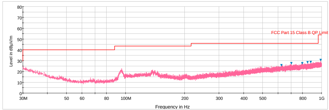
Plot 6-93. Radiated Spurious Plot below 1GHz (802.11a – U3 Ch. 157, Ant. Pol. H)
