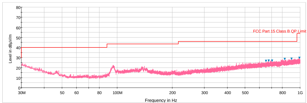
Plot 6-94. Radiated Spurious Plot below 1GHz (802.11a – U3 Ch. 157, Ant. Pol. V)
