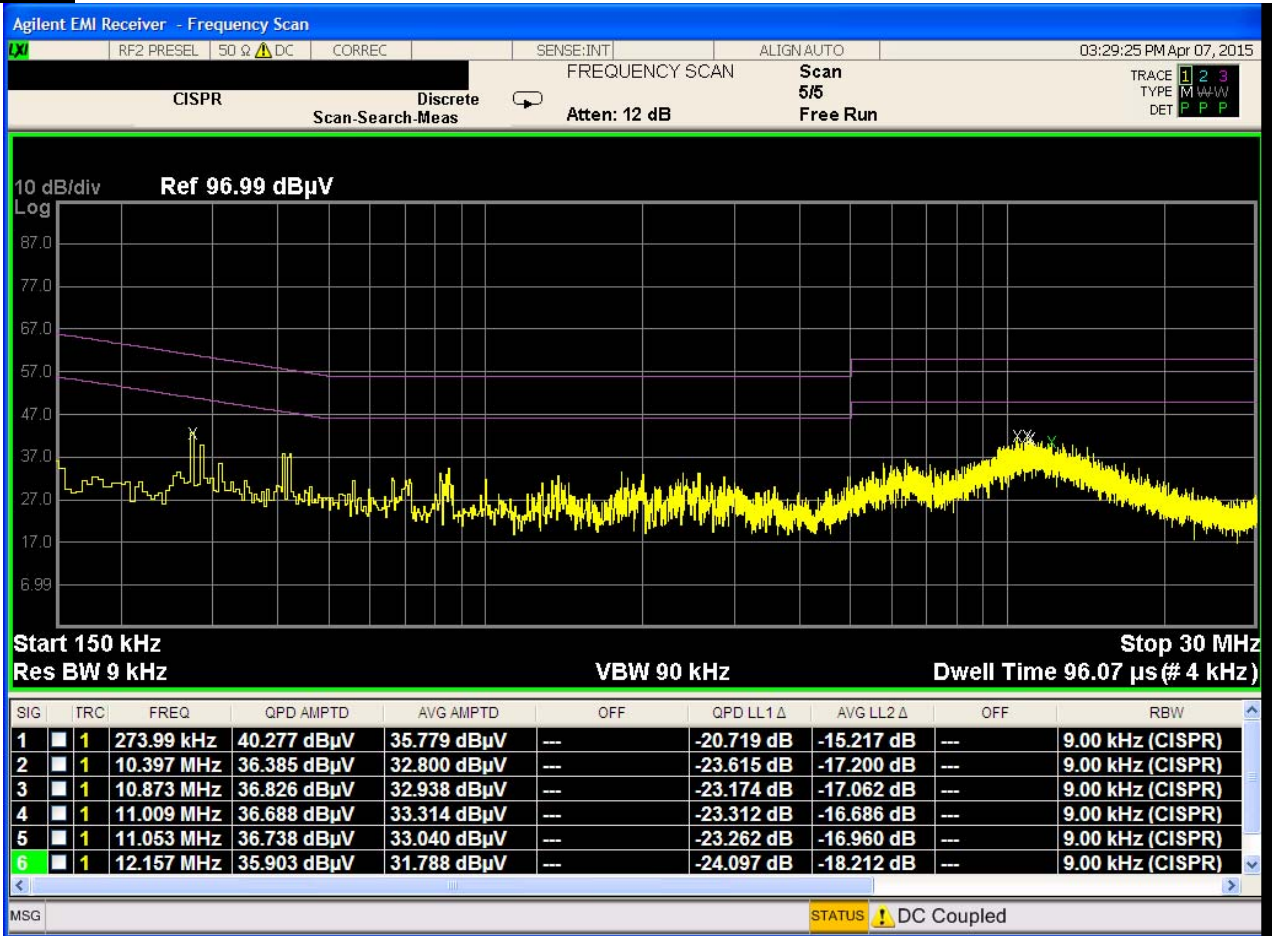
Plot 6-102. Line Conducted Plot with 802.11a UNII Band 3 (N)
