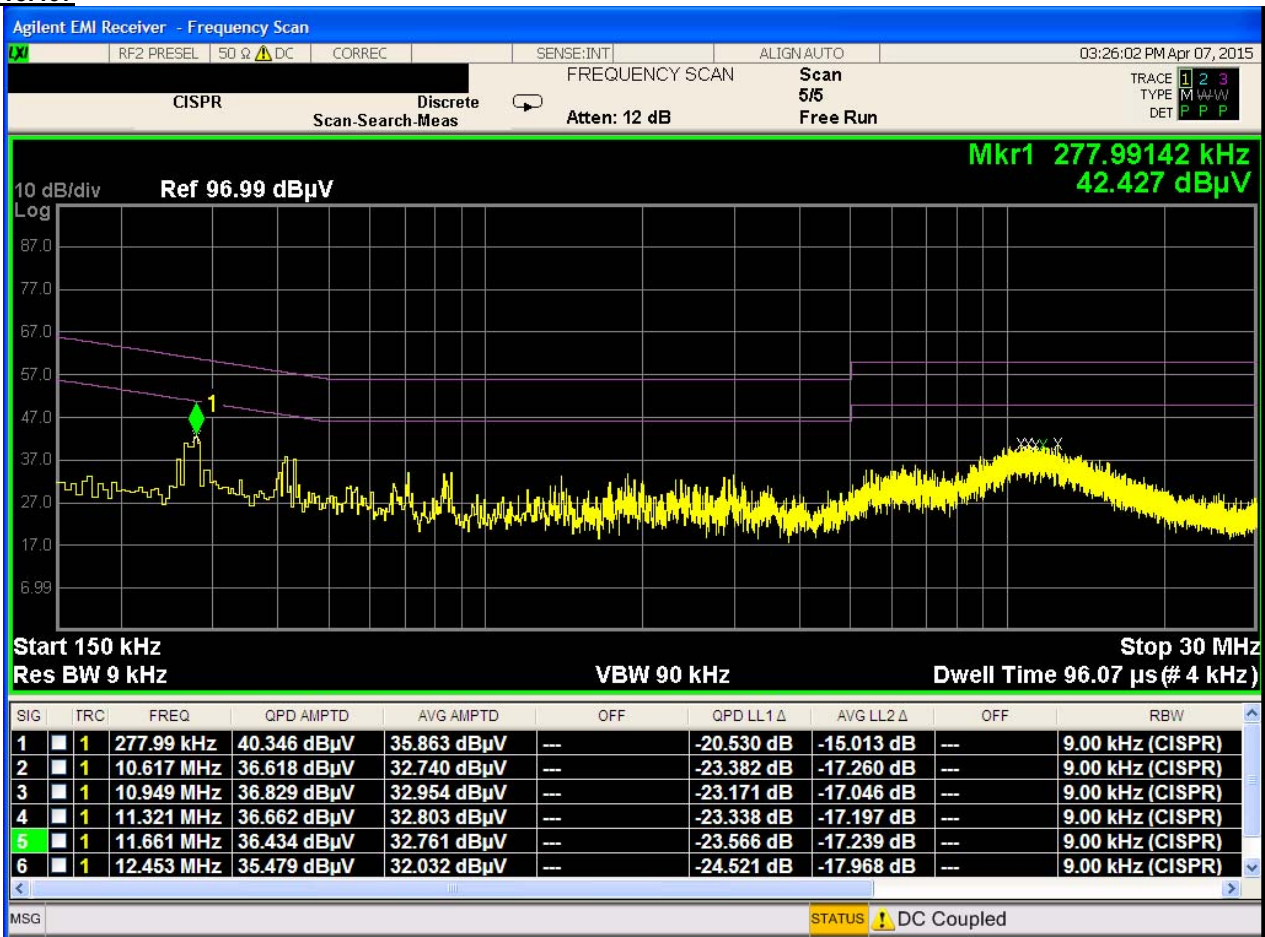
Plot 6-100. Line Conducted Plot with 802.11a UNII Band 2C (N)
