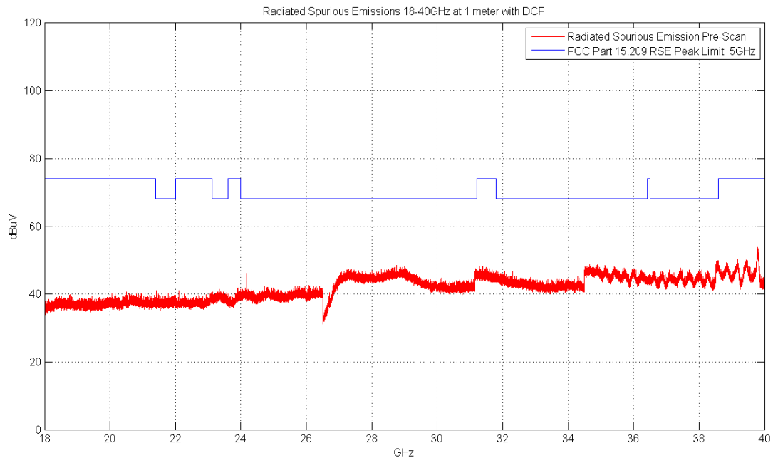
Plot 6-76. Radiated Spurious Plot above 18GHz (802.11a – Ant. Pol. V)
