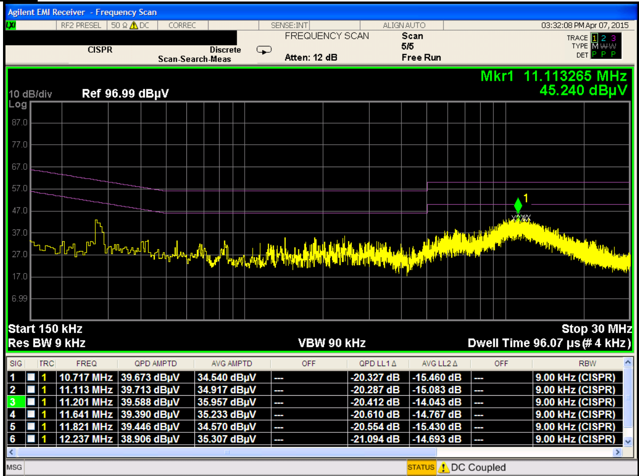
Plot 6-101. Line Conducted Plot with 802.11a UNII Band 3 (L1)
