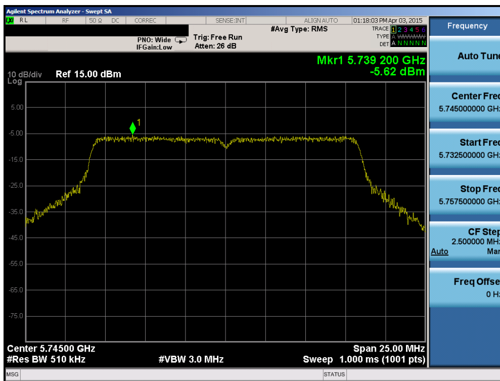
Plot 6-59. Power Spectral Density Plot (802.11a (UNII Band 3) – Ch. 149)
