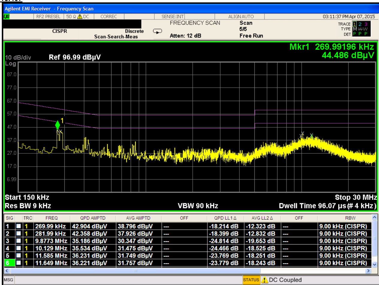
Plot 6-96. Line Conducted Plot with 802.11a UNII Band 1 (N)
