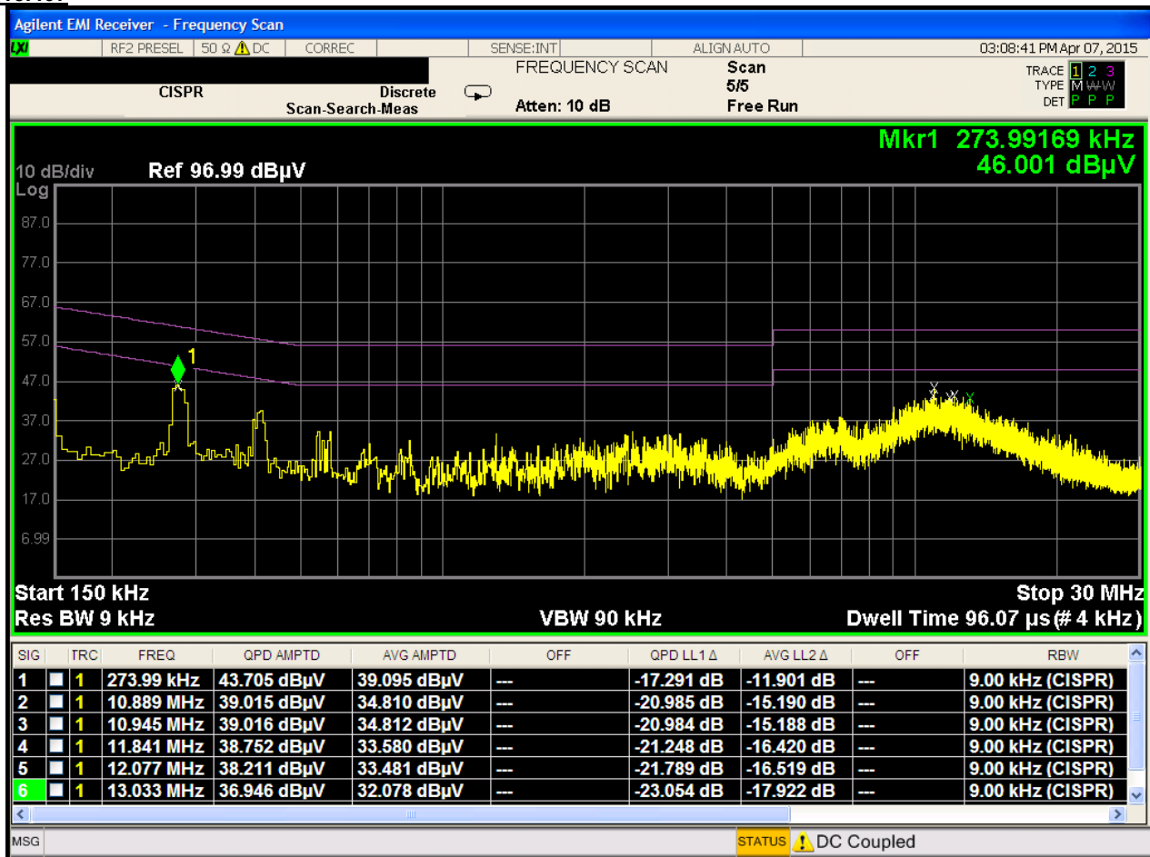
Plot 6-95. Line Conducted Plot with 802.11a UNII Band 1 (L1)
