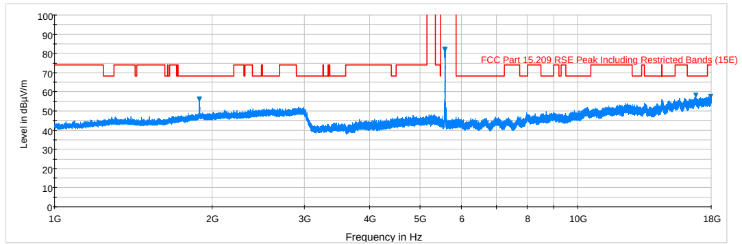
Plot 6-72. Radiated Spurious Plot above 1GHz (802.11a – U2C Ch. 116, Ant. Pol. V)
