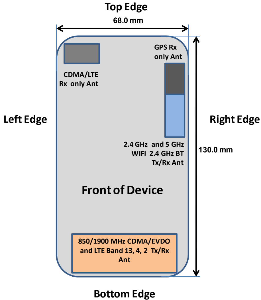
Figure F-1 DUT Antenna Locations
