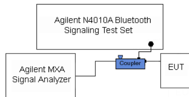
Figure 6-2. Test Instrument & Measurement Setup
