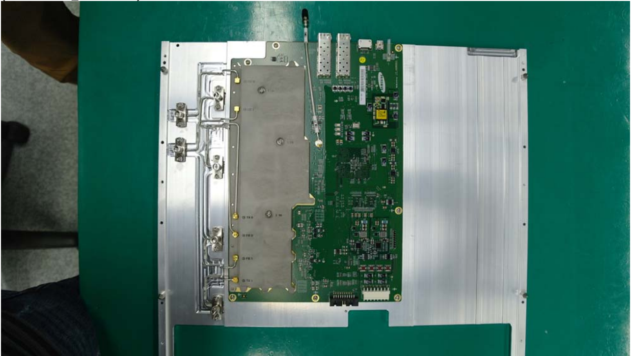
(L9VU-E2M_Cold Plate)
