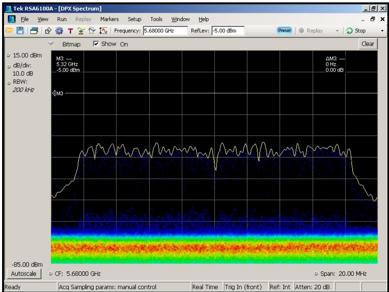
Figure 6-3. Real-Time Spectrum Display, WLAN Traffic (Streaming Video)
