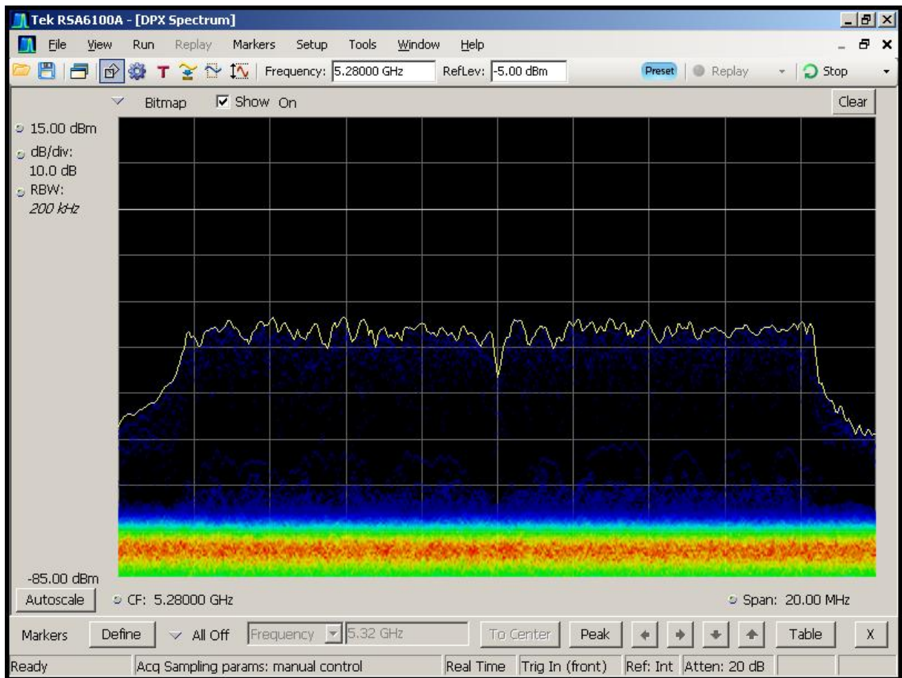
Figure 5-3. Real-Time Spectrum Display, WLAN Traffic (Streaming Video)
