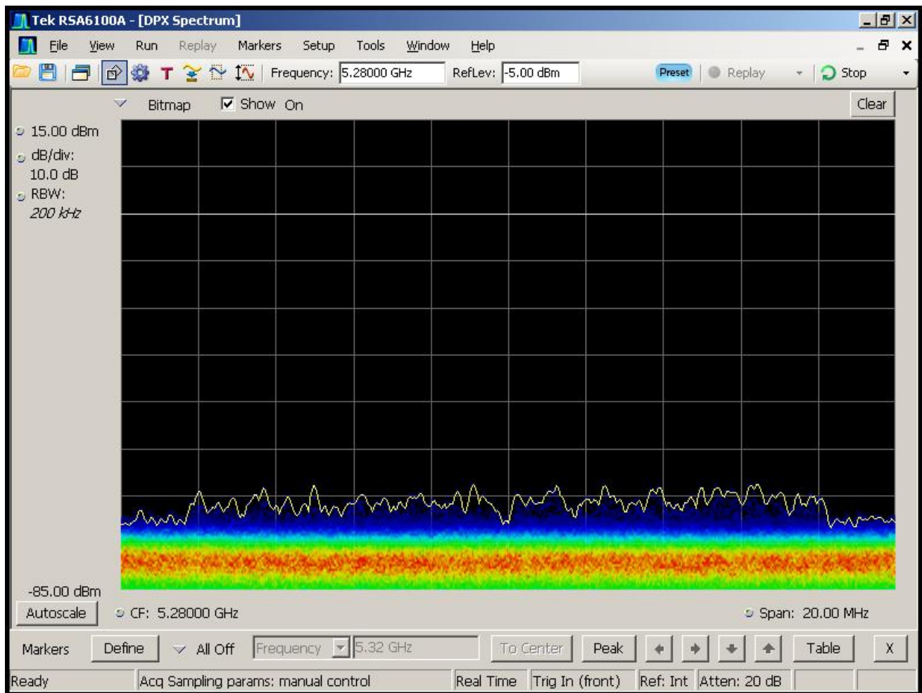
Figure 5-2. Real-Time Spectrum Display, No WLAN Traffic
