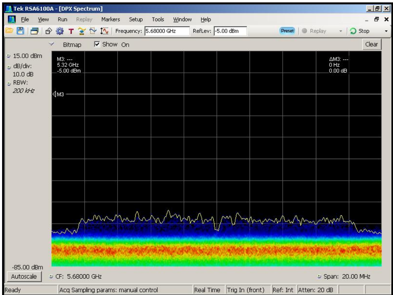
Figure 6-2. Real-Time Spectrum Display, No WLAN Traffic
