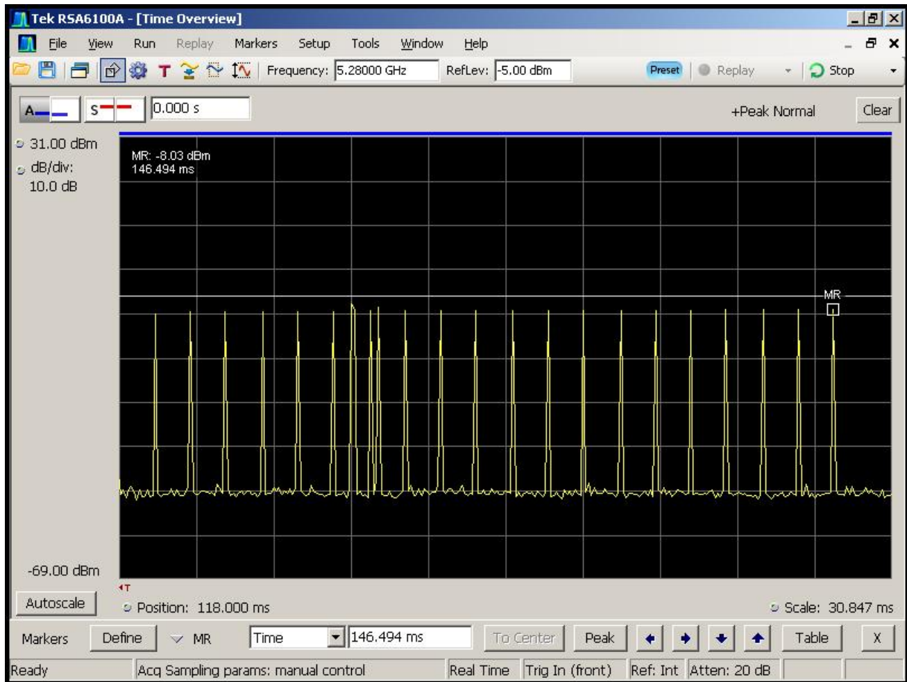
Figure 5-1. Type 1 Radar Pulse
