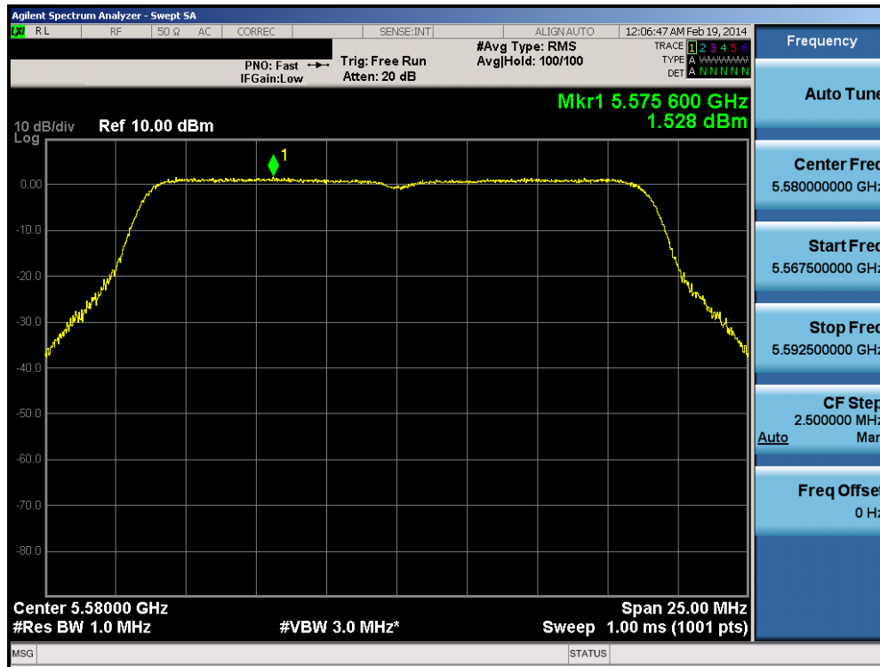
Plot 6-58. Peak Power Spectral Density Plot (20MHz BW 802.11n (UNII Band 2C) – Ch. 116)
