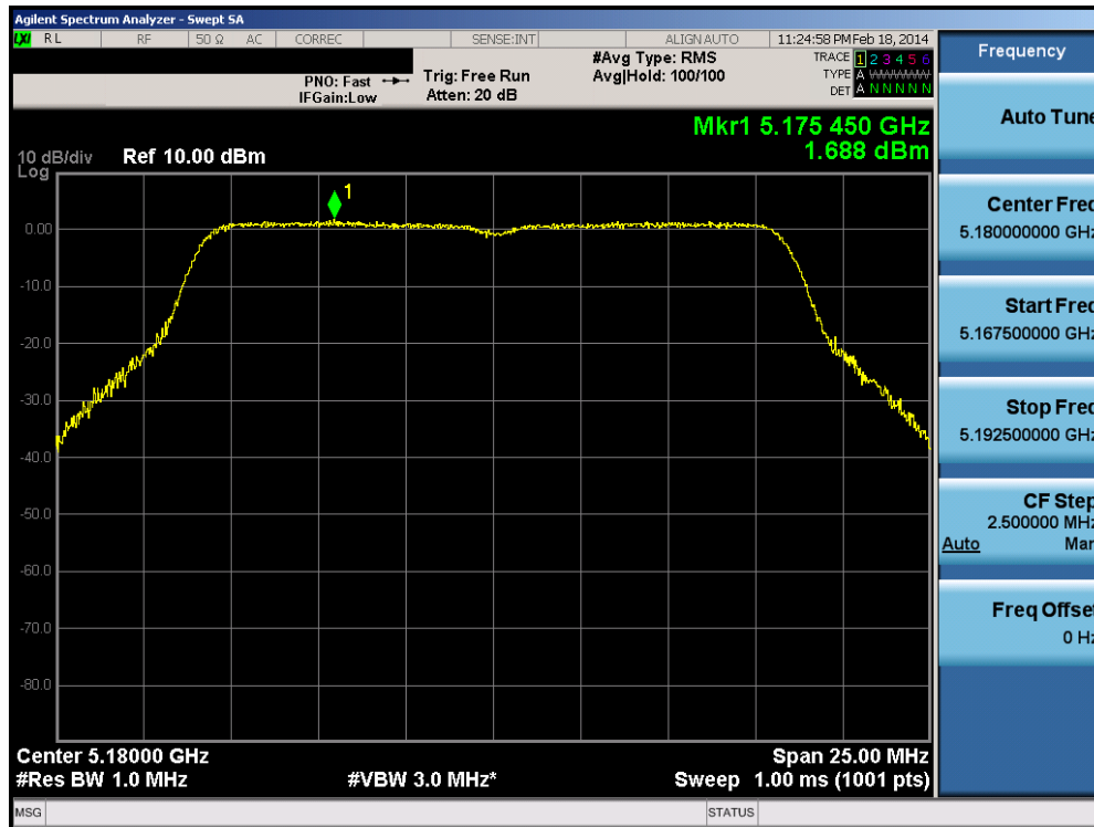
Plot 6-36. Peak Power Spectral Density Plot (802.11a (UNII Band 1) – Ch. 36)
