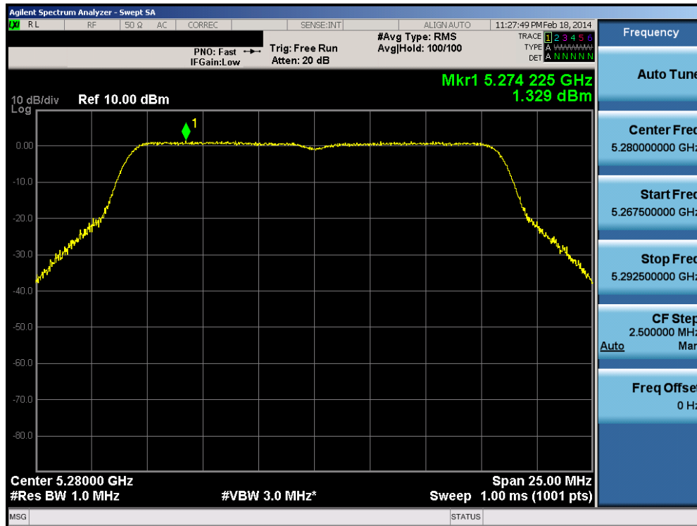
Plot 6-46. Peak Power Spectral Density Plot (802.11a (UNII Band 2A) – Ch. 56)
