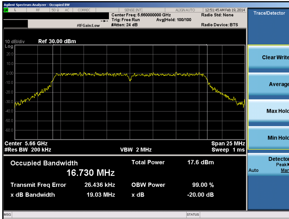
Plot 6-33. 20dB Bandwidth Plot (20MHz BW 802.11a (UNII Band 2A) – Ch. 132)
