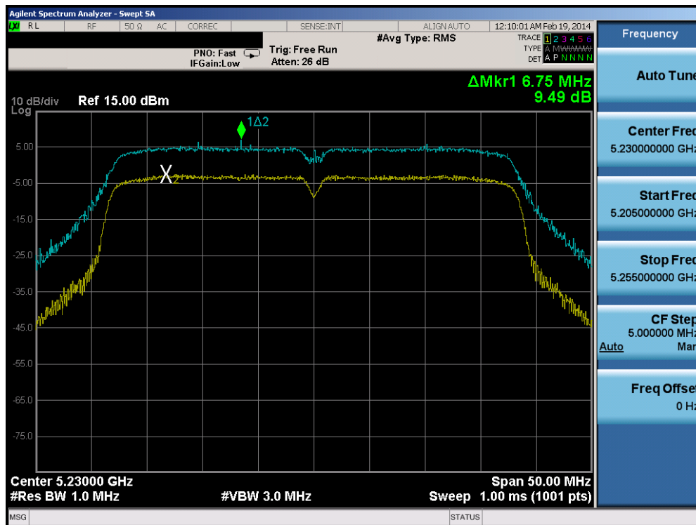
Plot 6-66. Peak Excursion Ratio Plot (40MHz BW 802.11n)
