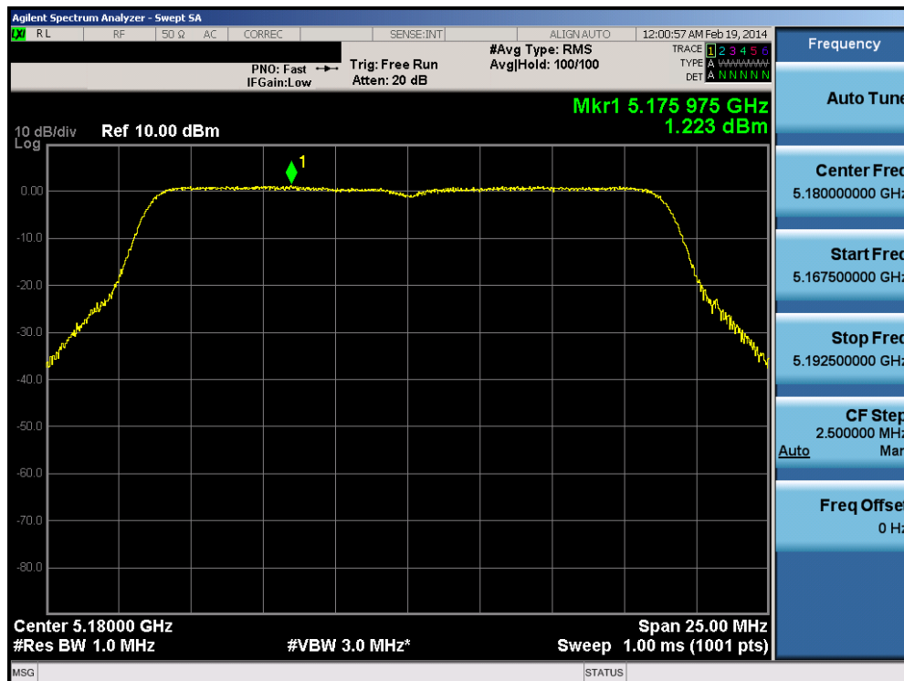
Plot 6-39. Peak Power Spectral Density Plot (20MHz BW 802.11n (UNII Band 1) – Ch. 36)
