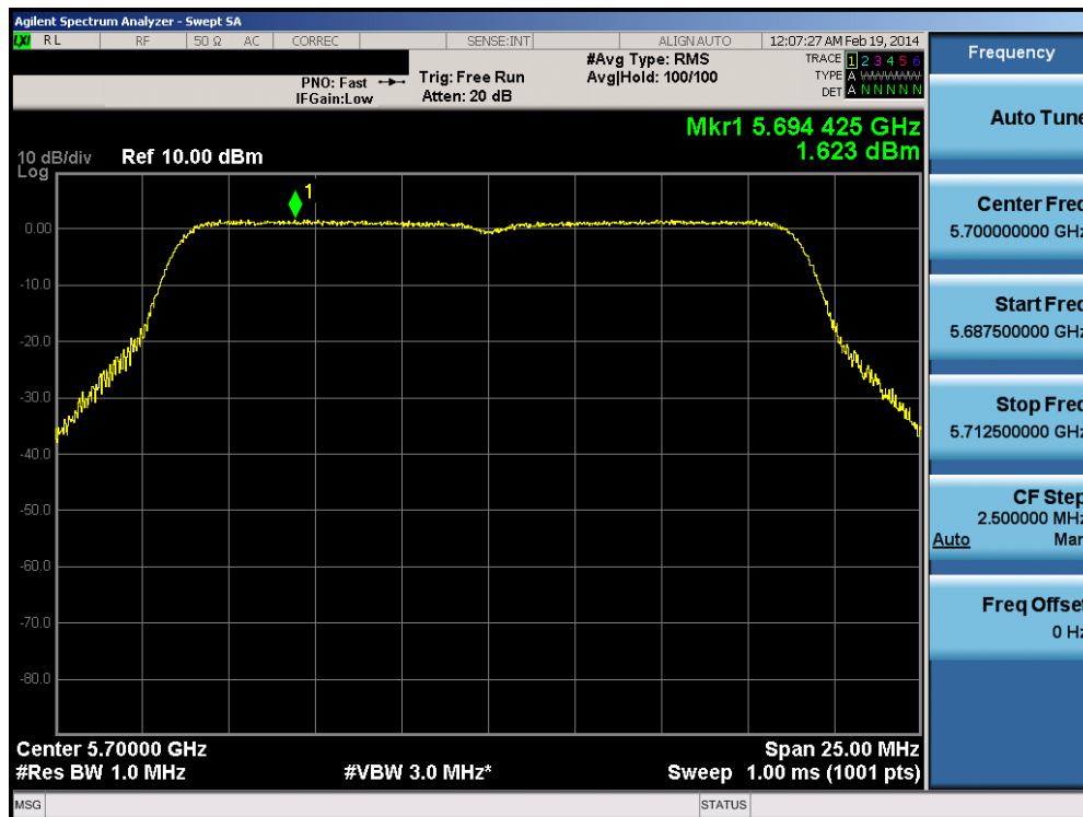
Plot 6-59. Peak Power Spectral Density Plot (20MHz BW 802.11n (UNII Band 2C) – Ch. 140)
