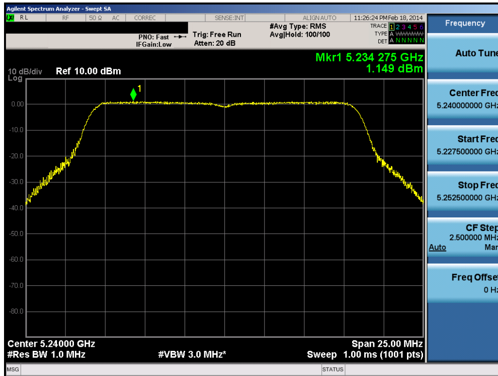
Plot 6-38. Peak Power Spectral Density Plot (802.11a (UNII Band 1) – Ch. 48)
