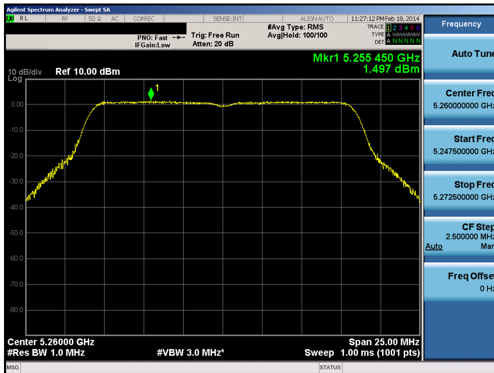
Plot 6-45. Peak Power Spectral Density Plot (802.11a (UNII Band 2A) – Ch. 52)
