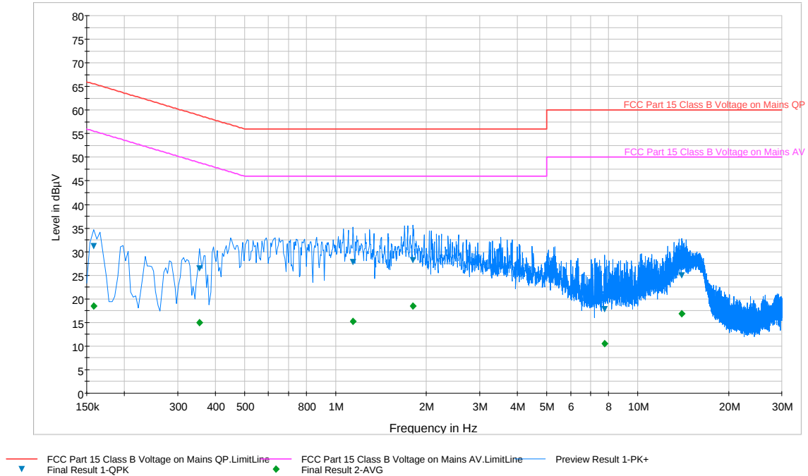
Plot 6-88. Line Conducted Plot with 802.11a UNII Band 1 (L1)
