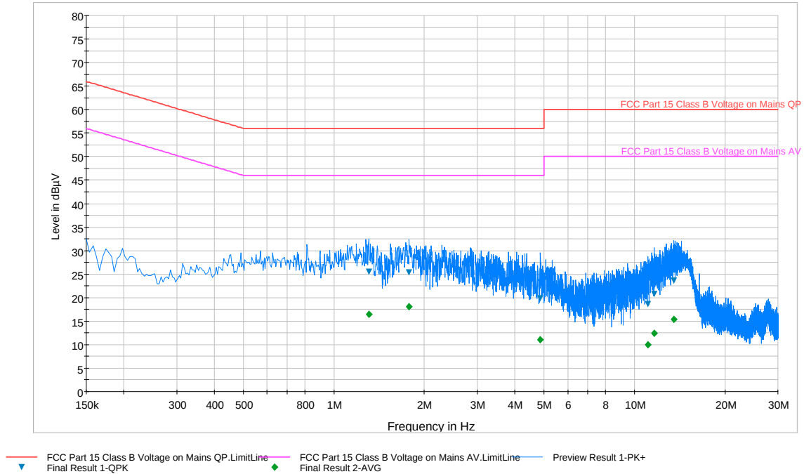
Plot 6-92. Line Conducted Plot with 802.11a UNII Band 2C (L1)
