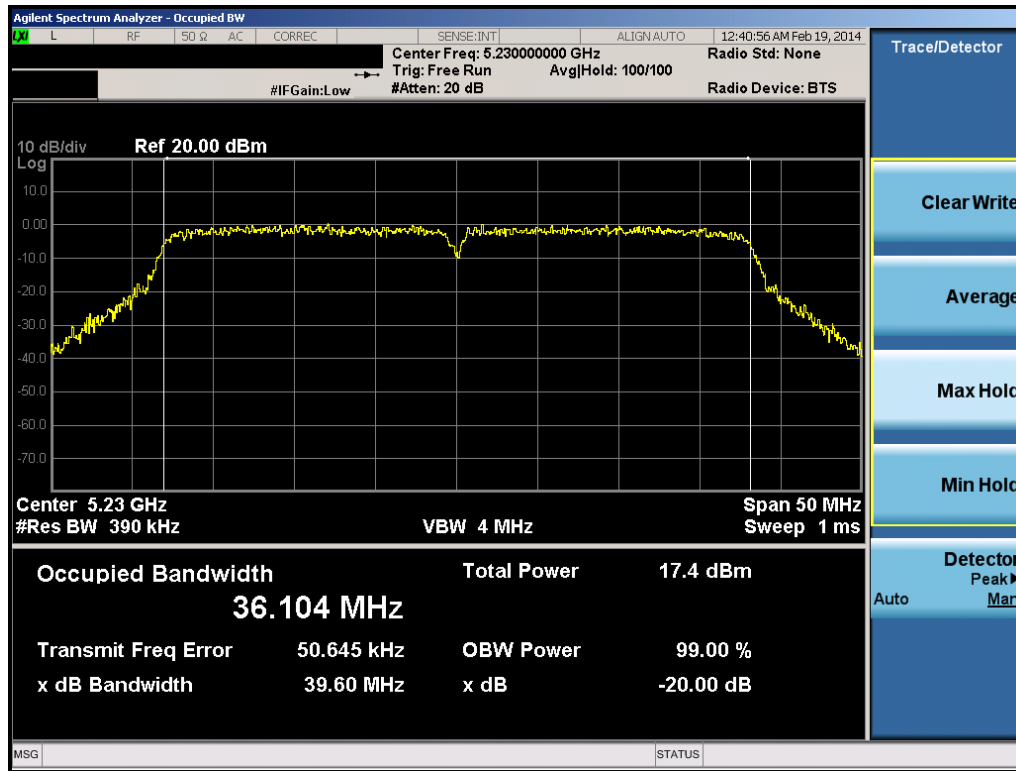
Plot 6-31. 20dB Bandwidth Plot (40MHz BW 802.11n (UNII Band 2A) – Ch. 46)
