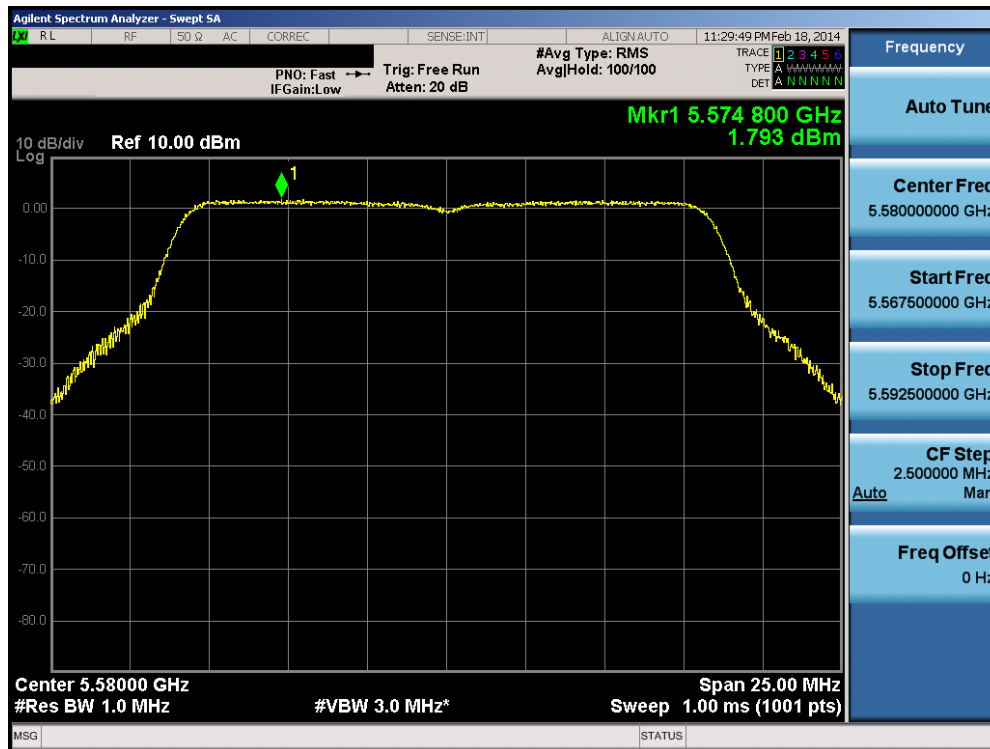
Plot 6-55. Peak Power Spectral Density Plot (802.11a (UNII Band 2C) – Ch. 116)
