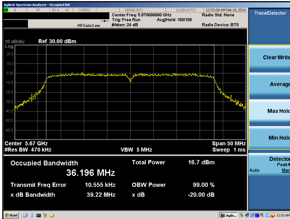
Plot 6-35. 20dB Bandwidth Plot (40MHz BW 802.11n (UNII Band 2A) – Ch. 134)
