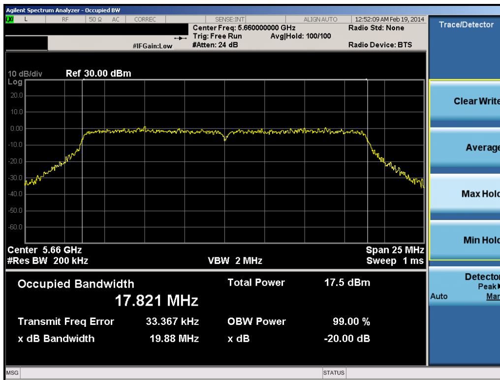
Plot 6-34. 20dB Bandwidth Plot (20MHz BW 802.11n (UNII Band 2A) – Ch. 132)
