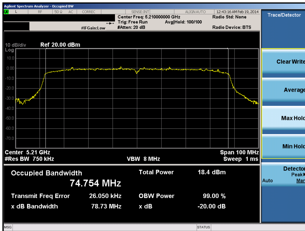
Plot 6-32. 20dB Bandwidth Plot (80MHz BW 802.11ac (UNII Band 2A) – Ch. 42)
