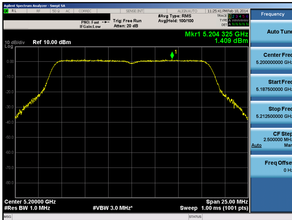
Plot 6-37. Peak Power Spectral Density Plot (802.11a (UNII Band 1) – Ch. 40)
