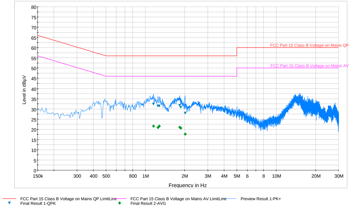
Plot 6-93. Line Conducted Plot with 802.11a UNII Band 2C (N)
