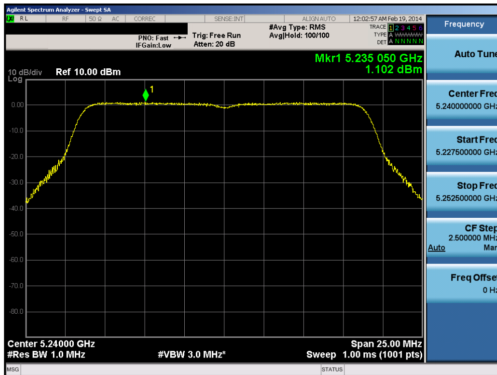
Plot 6-41. Peak Power Spectral Density Plot (20MHz BW 802.11n (UNII Band 1) – Ch. 48)
