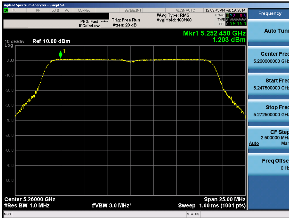
Plot 6-48. Peak Power Spectral Density Plot (20MHz BW 802.11n (UNII Band 2A) – Ch. 52)
