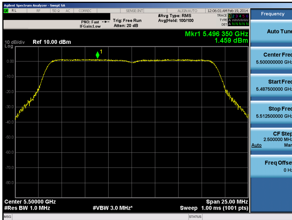
Plot 6-57. Peak Power Spectral Density Plot (20MHz BW 802.11n (UNII Band 2C) – Ch. 100)
