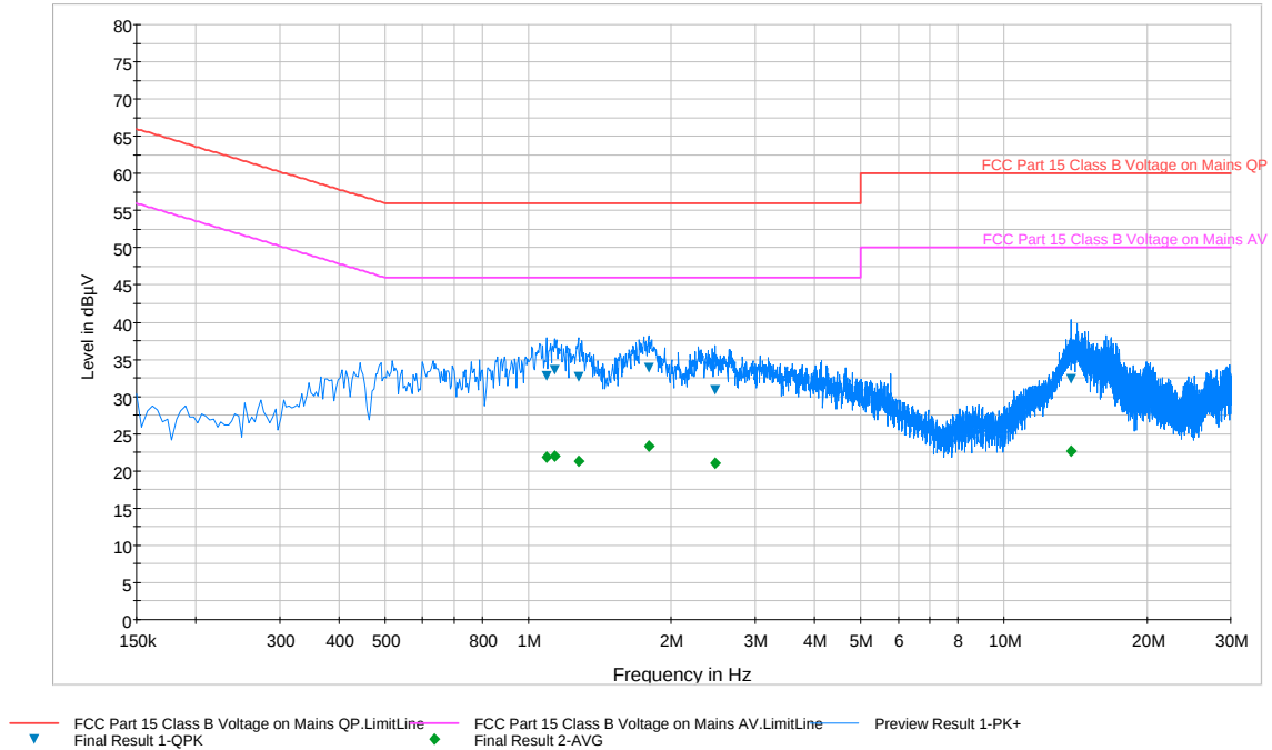
Plot 6-91. Line Conducted Plot with 802.11a UNII Band 2A (N)
