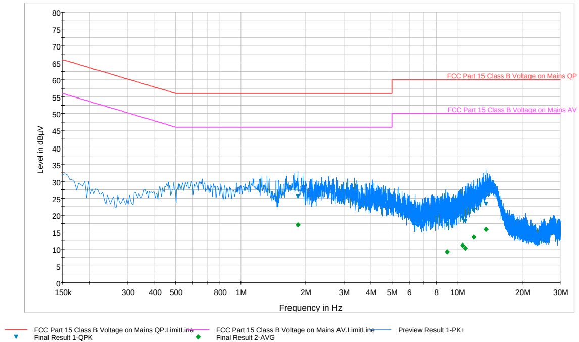
Plot 6-90. Line Conducted Plot with 802.11a UNII Band 2A (L1)
