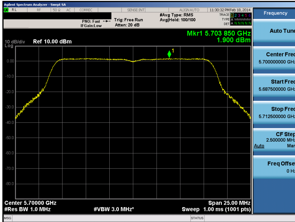
Plot 6-56. Peak Power Spectral Density Plot (802.11a (UNII Band 2C) – Ch. 140)
