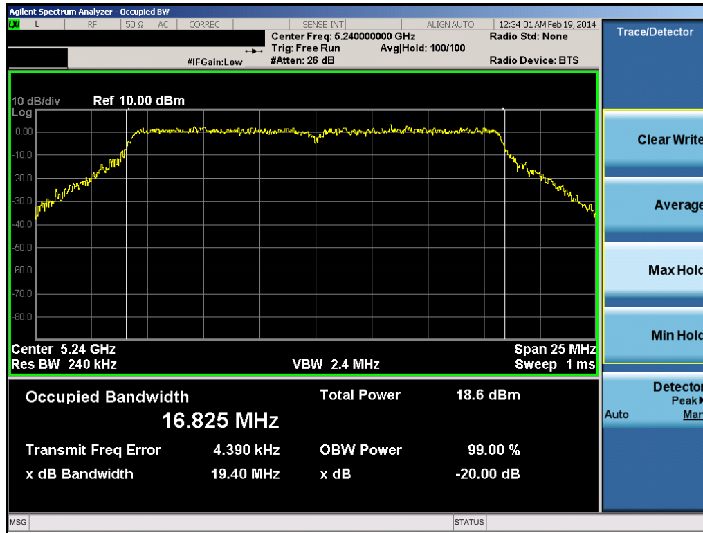
Plot 6-29. 20dB Bandwidth Plot (20MHz BW 802.11a (UNII Band 2A) – Ch. 48)
