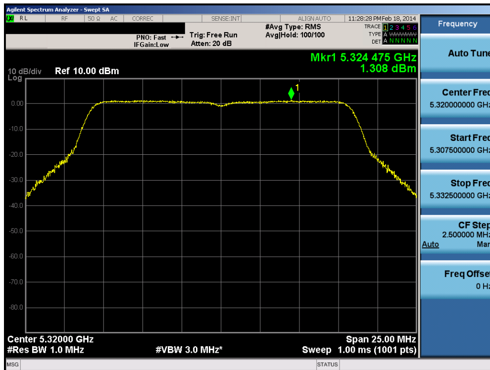
Plot 6-47. Peak Power Spectral Density Plot (802.11a (UNII Band 2A) – Ch. 64)
