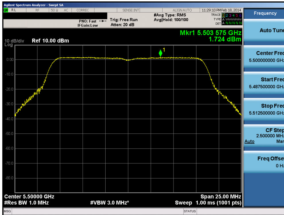
Plot 6-54. Peak Power Spectral Density Plot (802.11a (UNII Band 2C) – Ch. 100)
