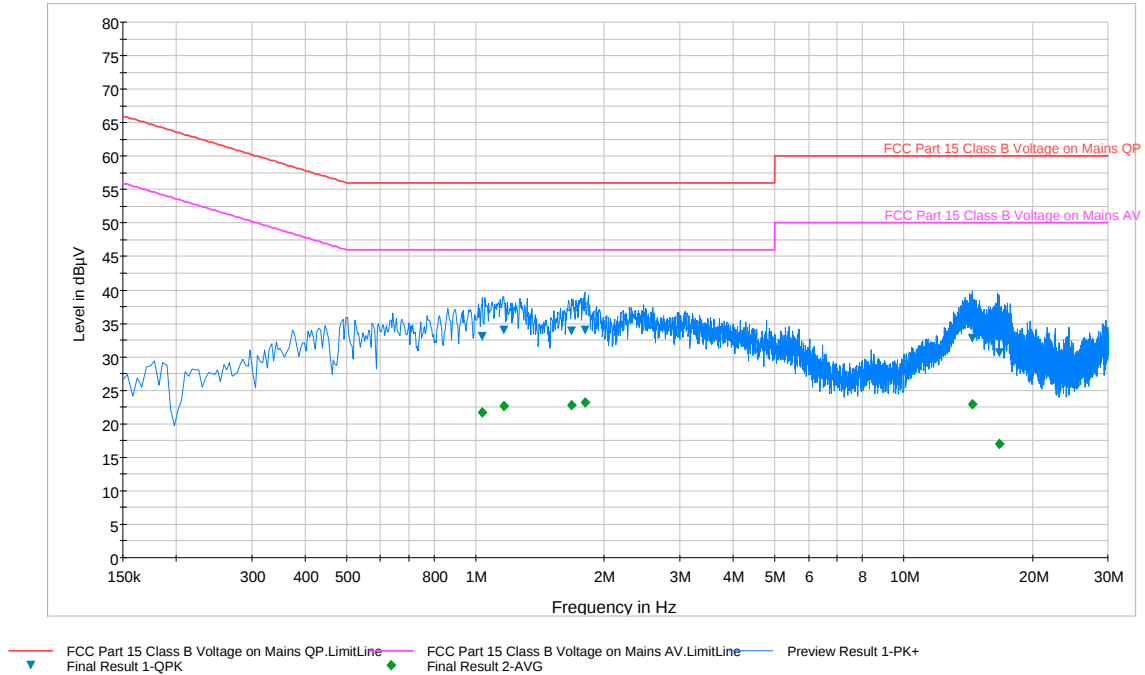
Plot 6-89. Line Conducted Plot with 802.11a UNII Band 1 (N)
