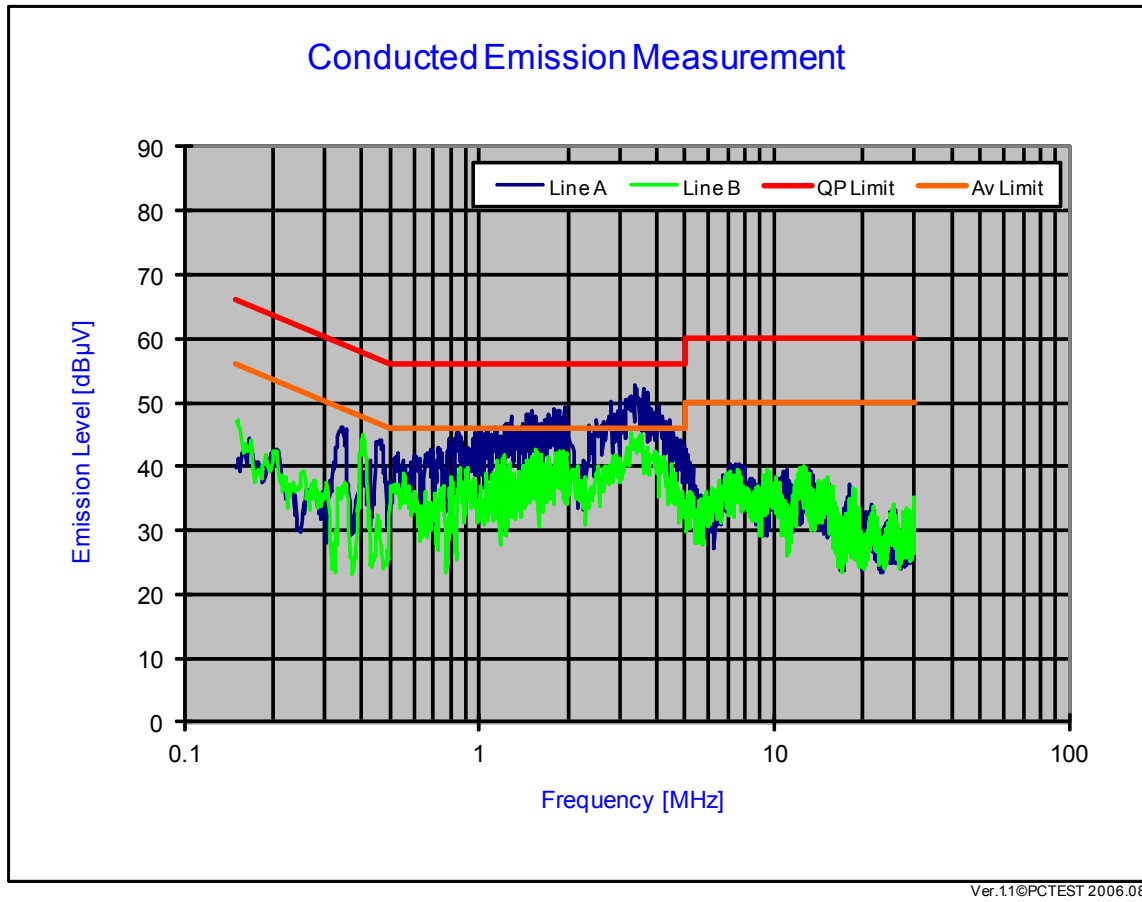
Plot 6-44. Line Conducted Plot with Bluetooth
