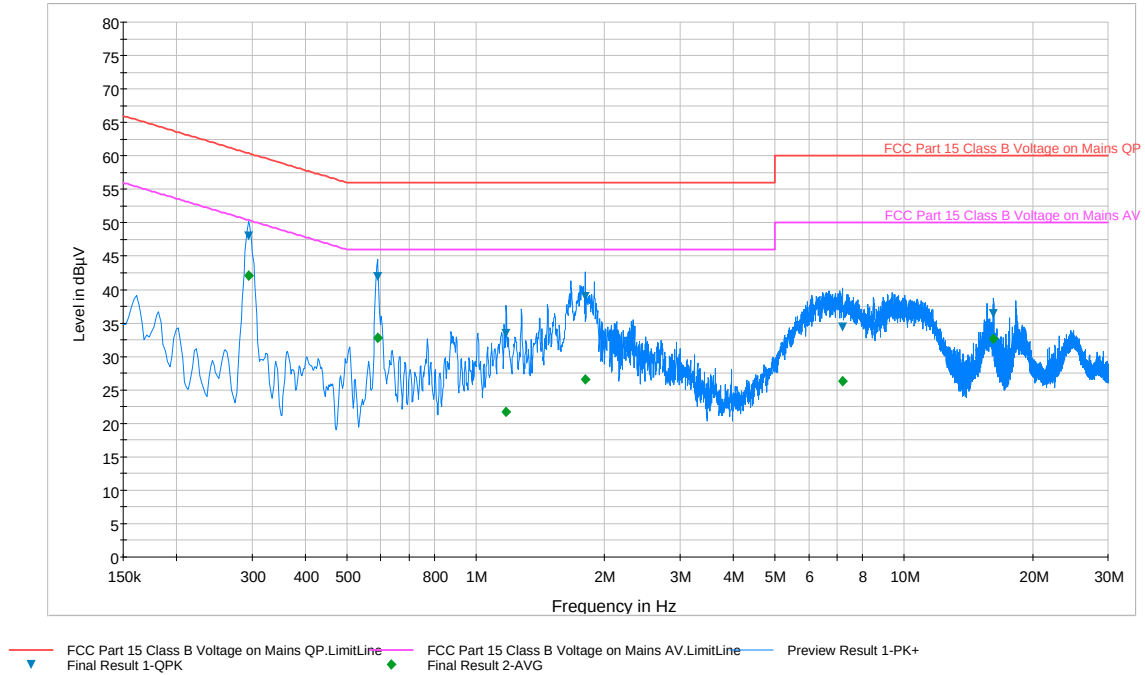
Plot 6-85. Line Conducted Plot with 802.11a UNII Band 2A (L1)
