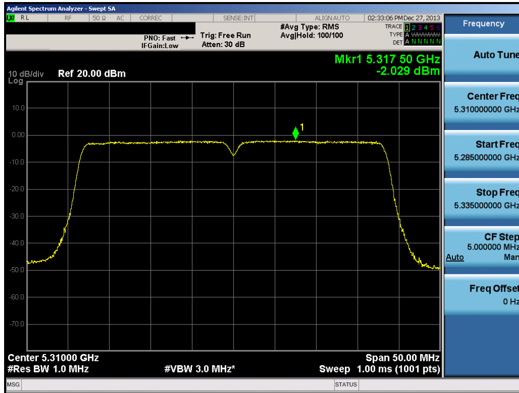
Plot 6-48. Peak Power Spectral Density Plot (40MHz BW 802.11n (UNII Band 2A) – Ch. 62)
