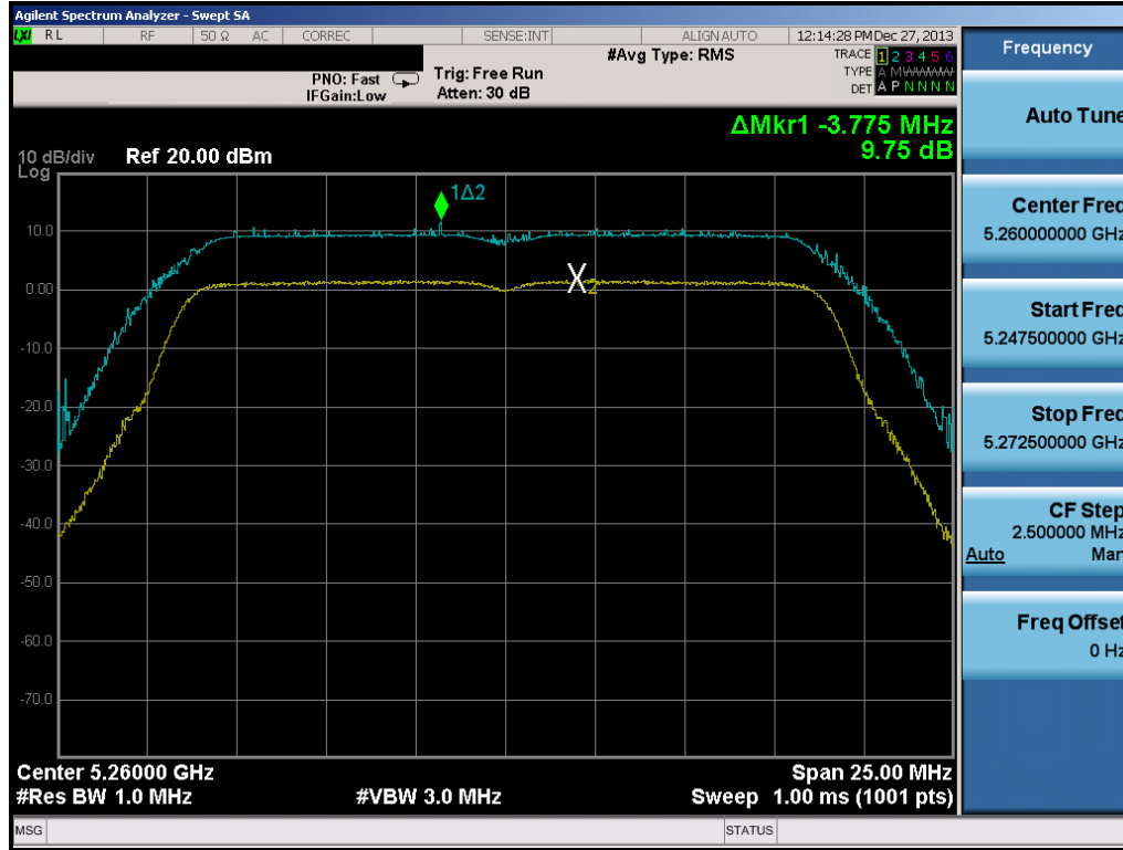
Plot 6-61. Peak Excursion Ratio Plot (20MHz BW 802.11n)
