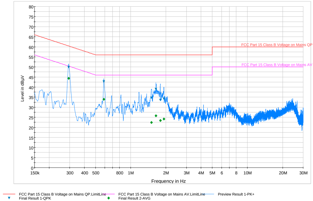
Plot 6-88. Line Conducted Plot with 802.11a UNII Band 2C (N)
