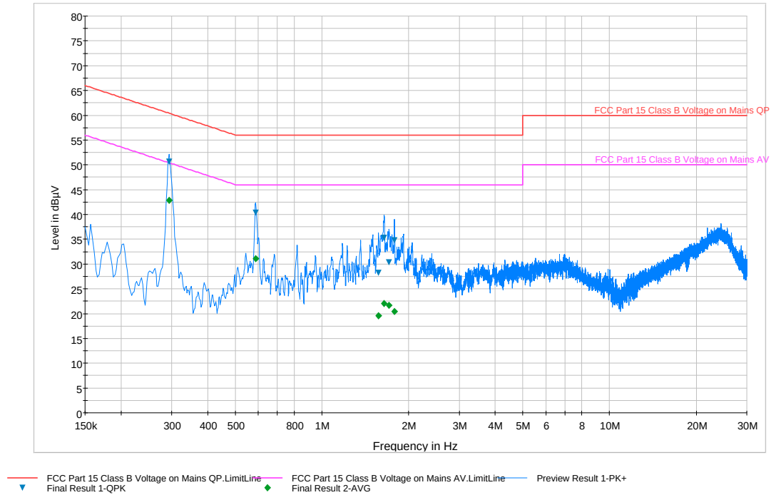
Plot 6-84. Line Conducted Plot with 802.11a UNII Band 1 (N)
