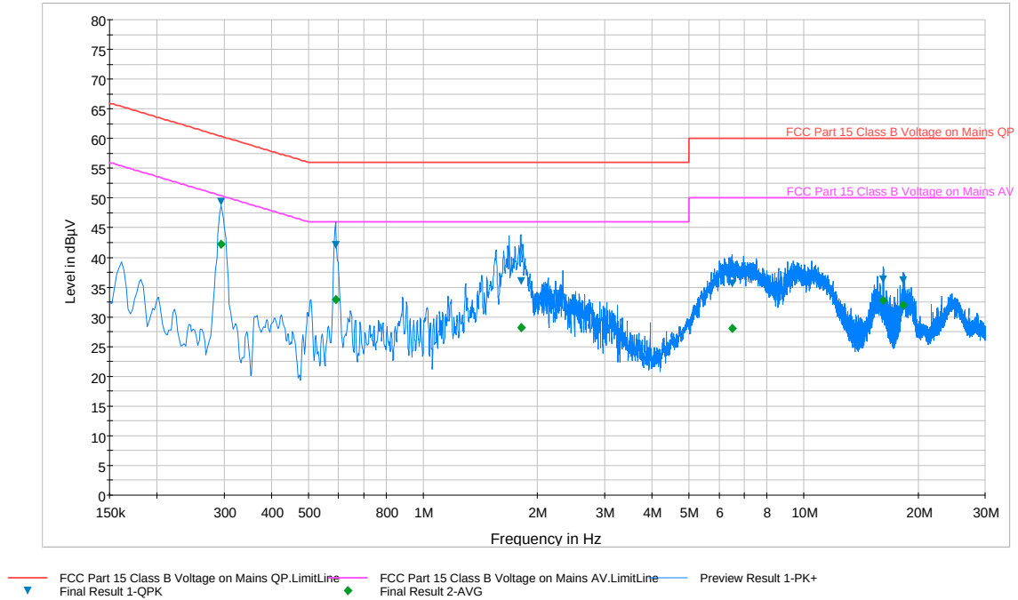
Plot 6-87. Line Conducted Plot with 802.11a UNII Band 2C (L1)
