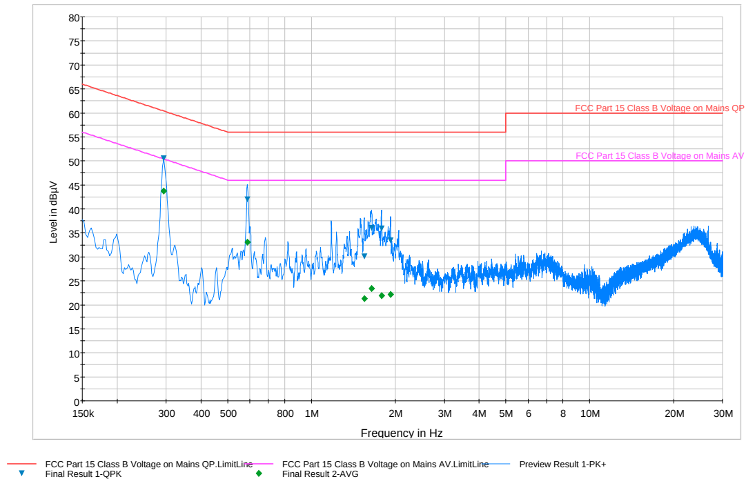
Plot 6-86. Line Conducted Plot with 802.11a UNII Band 2A (N)
