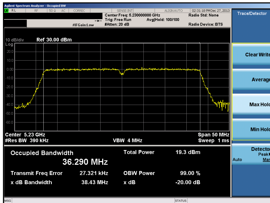
Plot 6-30. 20dB Bandwidth Plot (40MHz BW 802.11n (UNII Band 1) – Ch. 46)
