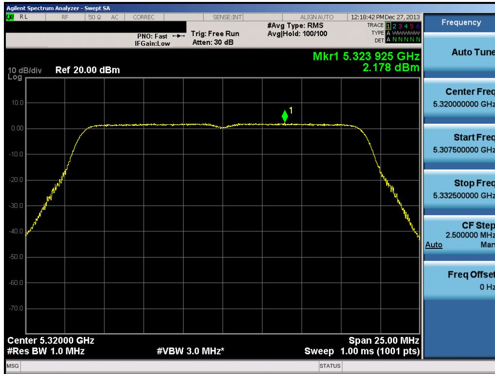
Plot 6-46. Peak Power Spectral Density Plot (20MHz BW 802.11n (UNII Band 2A) – Ch. 64)
