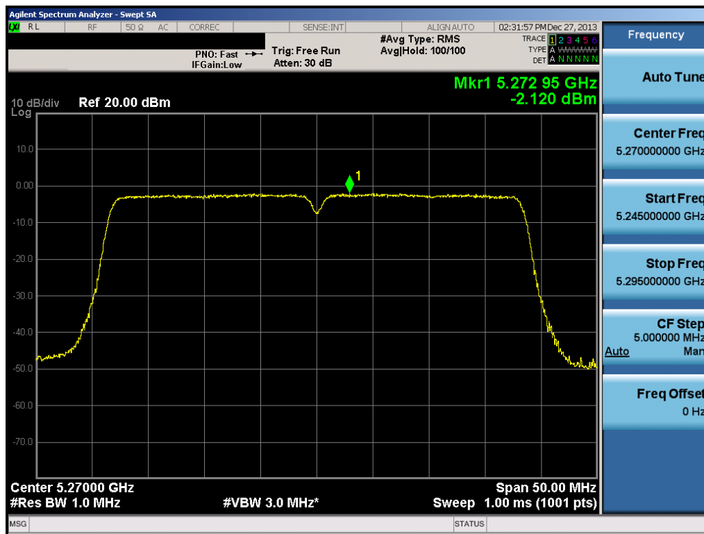
Plot 6-47. Peak Power Spectral Density Plot (40MHz BW 802.11n (UNII Band 2A) – Ch. 54)
