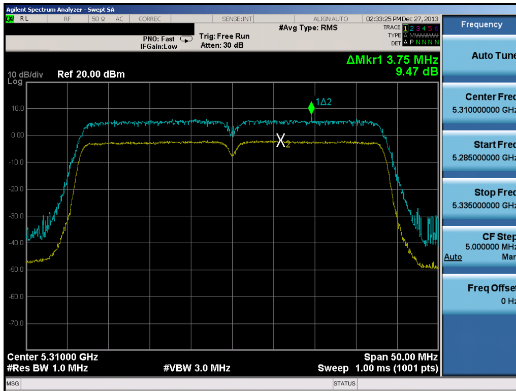
Plot 6-62. Peak Excursion Ratio Plot (40MHz BW 802.11n)
