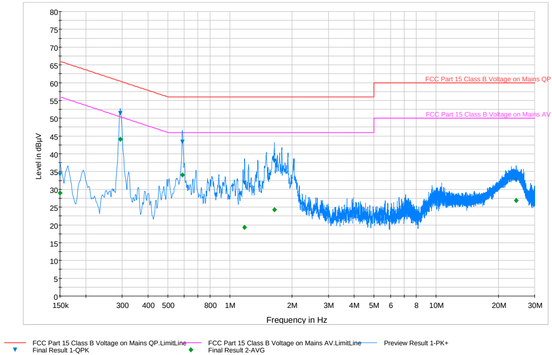
Plot 6-83. Line Conducted Plot with 802.11a UNII Band 1 (L1)
