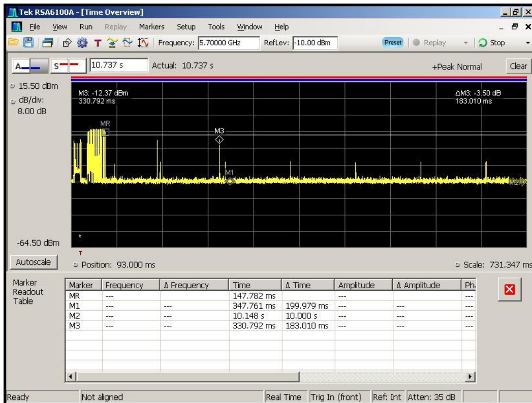
Figure 6-6. Channel Move Time Zoomed In
