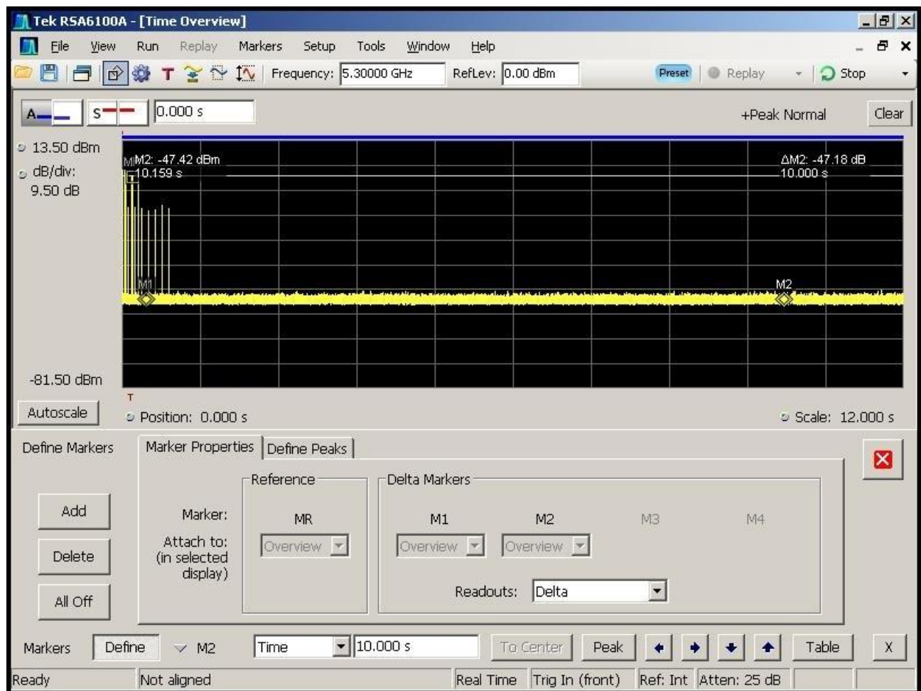
Figure 5-3. Channel Move Time (< 10sec)
