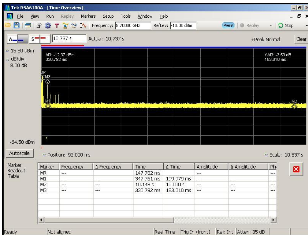
Figure 6-3. Channel Move Time (< 10sec)
