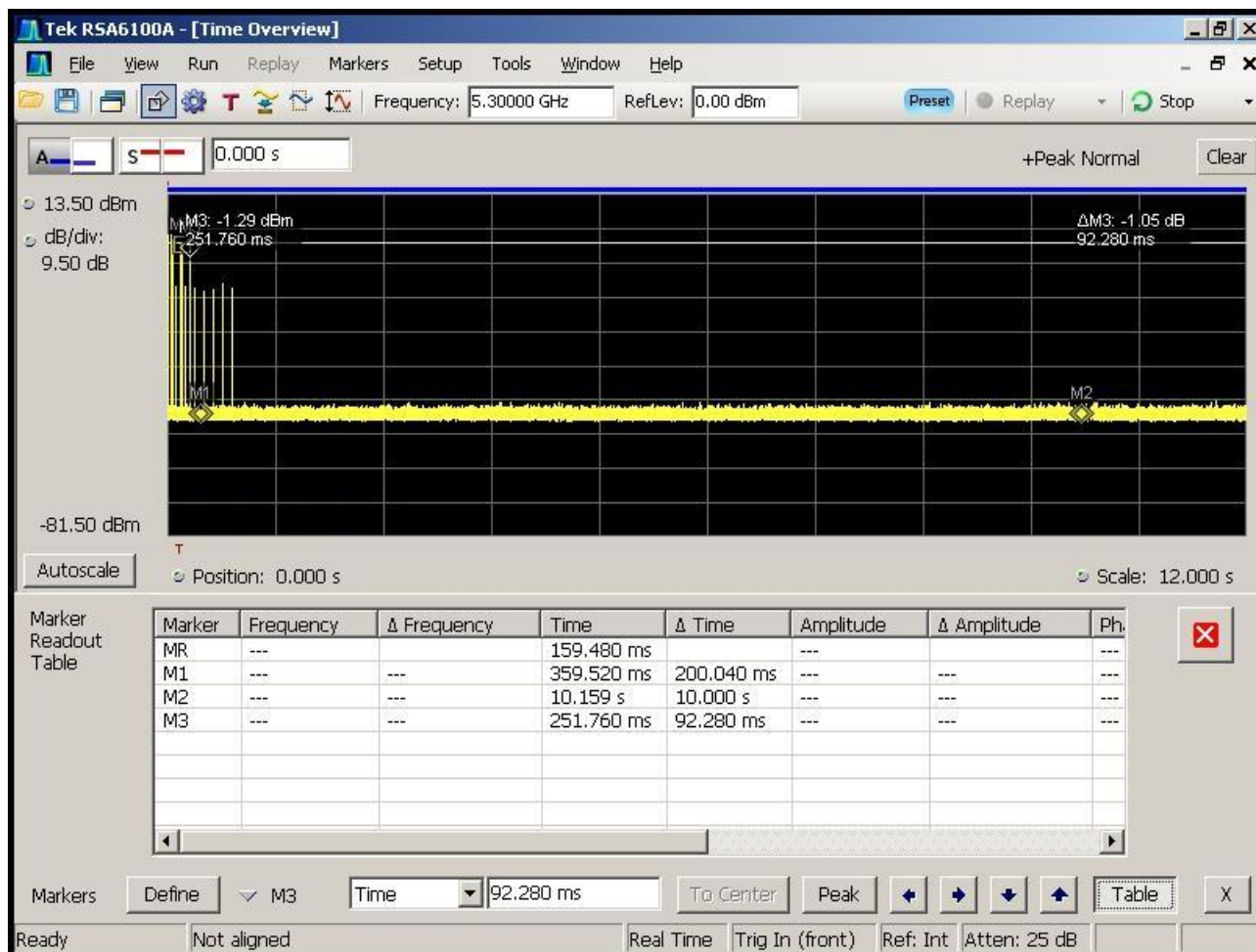
Figure 5-4. Aggregate Time using Pulse Table Capability
