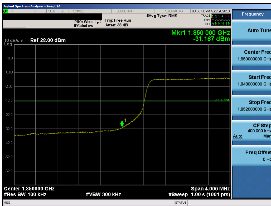
Plot 7-15. Lower Band Edge Plot (10.0MHz QPSK - RB Size 50)
