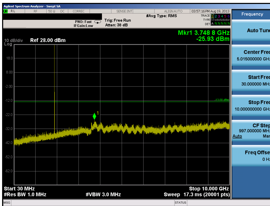
Plot 7-23. Conducted Spurious Plot (10.0MHz QPSK – RB Size 1, RB Offset 0 – High Channel)
