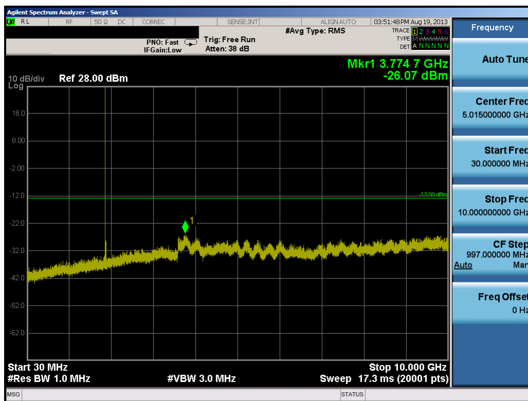
Plot 7-21. Conducted Spurious Plot (10.0MHz QPSK – RB Size 1, RB Offset 0 – Mid Channel)
