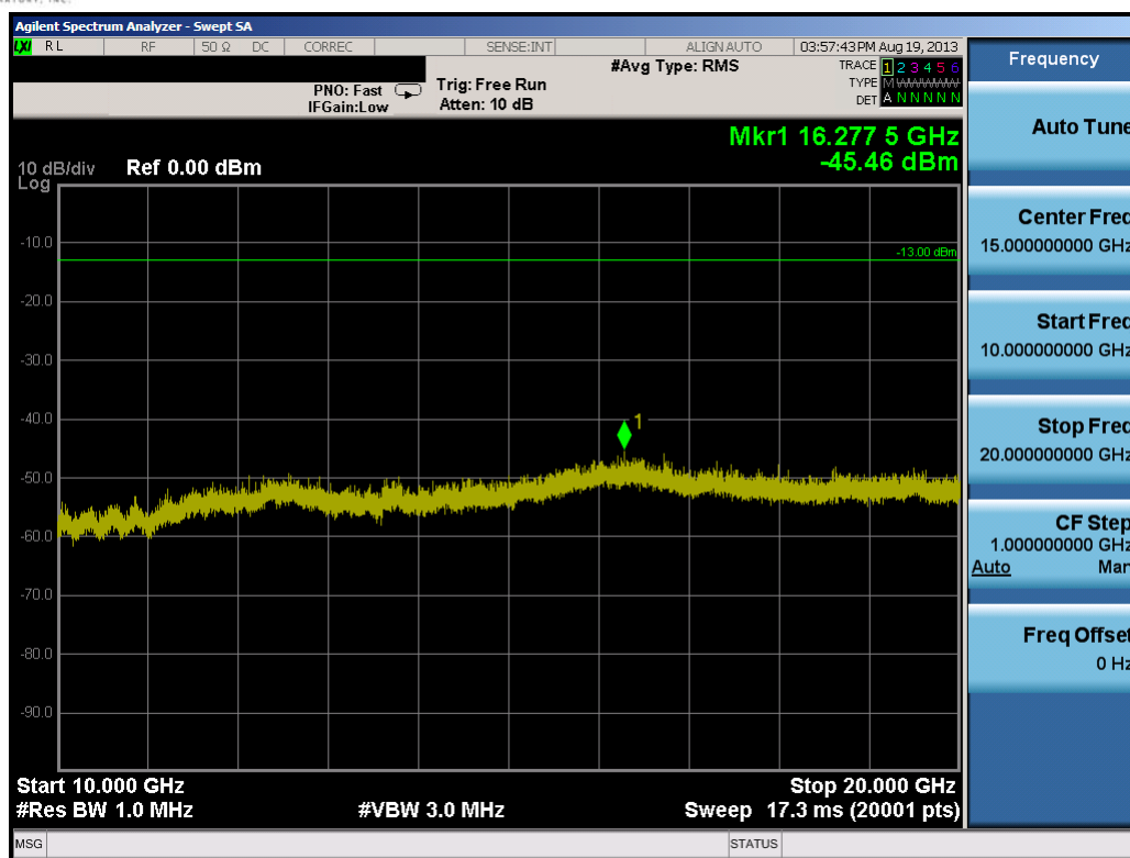
Plot 7-24. Conducted Spurious Plot (10.0MHz QPSK – RB Size 1, RB Offset 0 – High Channel)
