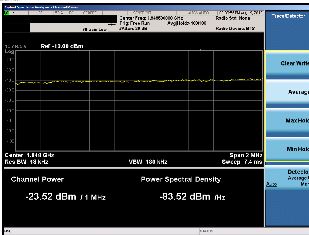
Plot 7-2. Lower Extended Band Edge Plot (5.0MHz QPSK – RB Size 25)
