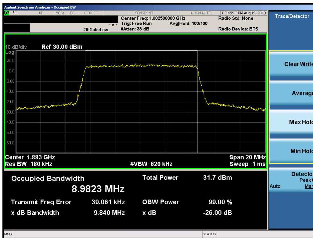
Plot 7-17. Occupied Bandwidth Plot (10.0MHz QPSK – RB Size 50)
