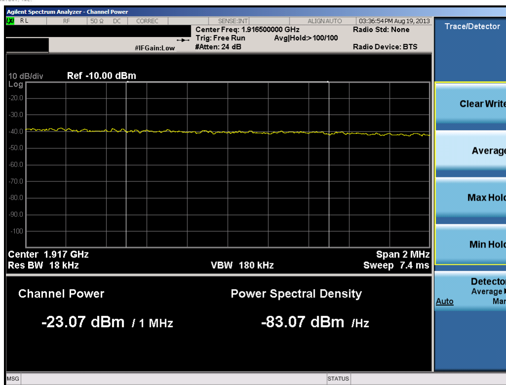
Plot 7-12. Upper Extended Band Edge Plot (5.0MHz QPSK – RB Size 25)
