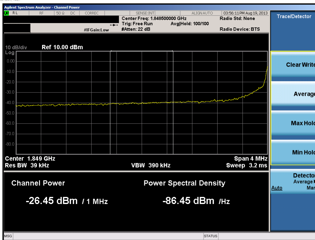
Plot 7-16. Lower Extended Band Edge Plot (10.0MHz QPSK – RB Size 50)
