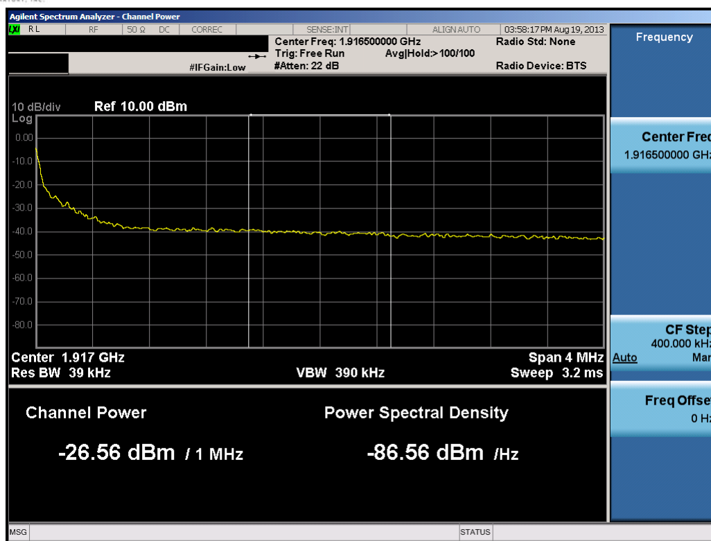
Plot 7-26. Upper Extended Band Edge Plot (10.0MHz QPSK – RB Size 50)
