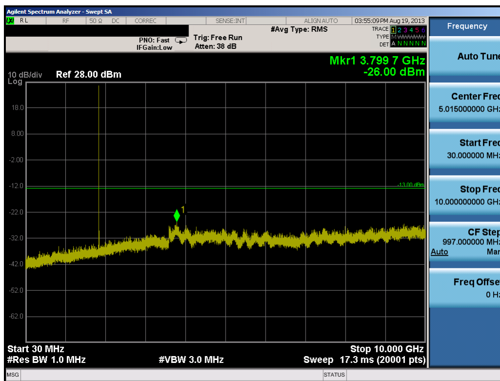
Plot 7-19. Conducted Spurious Plot (10.0MHz QPSK – RB Size 1, RB Offset 0– Low Channel)
