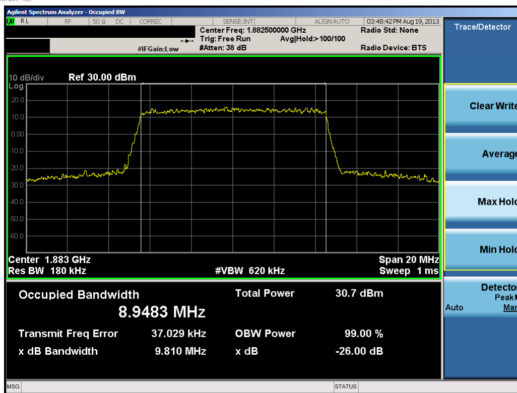
Plot 7-18. Occupied Bandwidth Plot (10.0MHz 16-QAM – RB Size 50)
