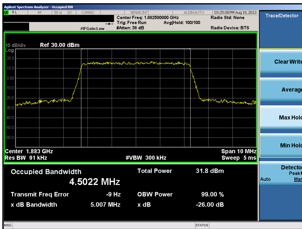
Plot 7-3. Occupied Bandwidth Plot (5.0MHz QPSK – RB Size 25)
