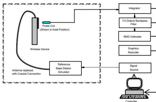
Figure 5-14 Audio Magnetic Field Test Setup
