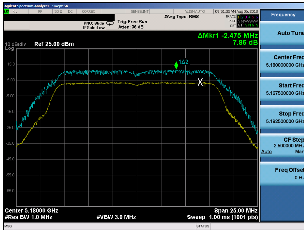
Plot 6-58. Peak Excursion Ratio Plot (802.11a)
