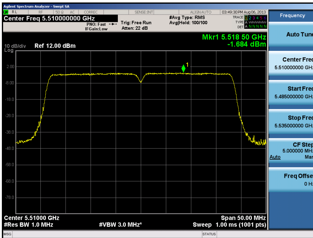
Plot 6-54. Peak Power Spectral Density Plot (40MHz BW 802.11n (UNII Band 3) – Ch. 102)
