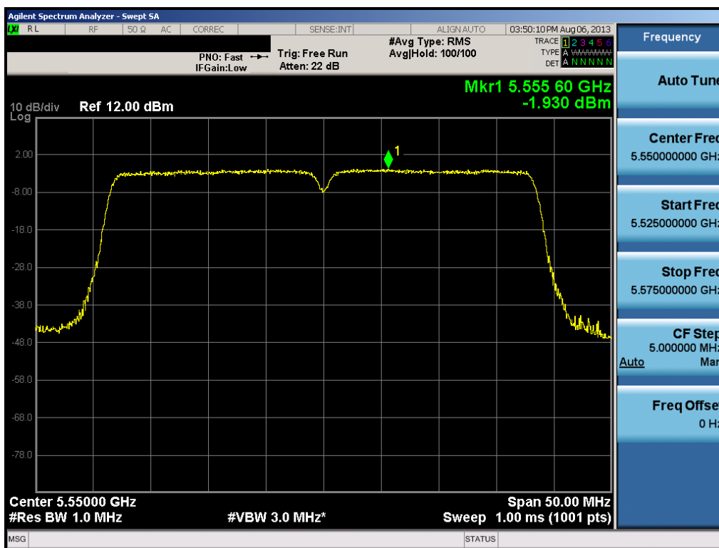
Plot 6-55. Peak Power Spectral Density Plot (40MHz BW 802.11n (UNII Band 3) – Ch. 110)
